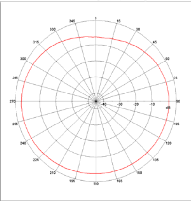
Far-field Power Distribution(H+V) on X-Y Plane Plot AvgGain(H+V)=-0.48dB @2.44000 GHz
