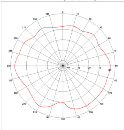
Far-field Power Distribution(H+V) on Y-Z Plane Plot AvgGain(H+V)=-2.99dB @2.44000 GHz
