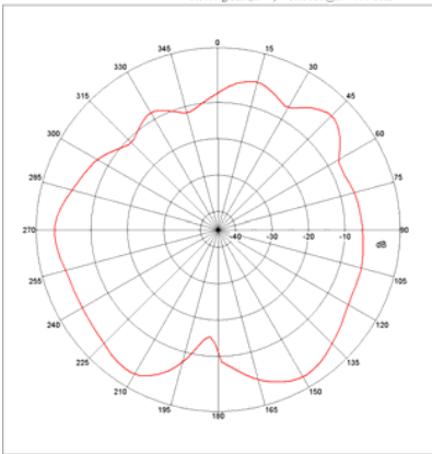
Far-field Power Distribution(H+V) on X-Z Plane Plot AvgGain(H+V)=-3.83dB @2.44000 GHz
