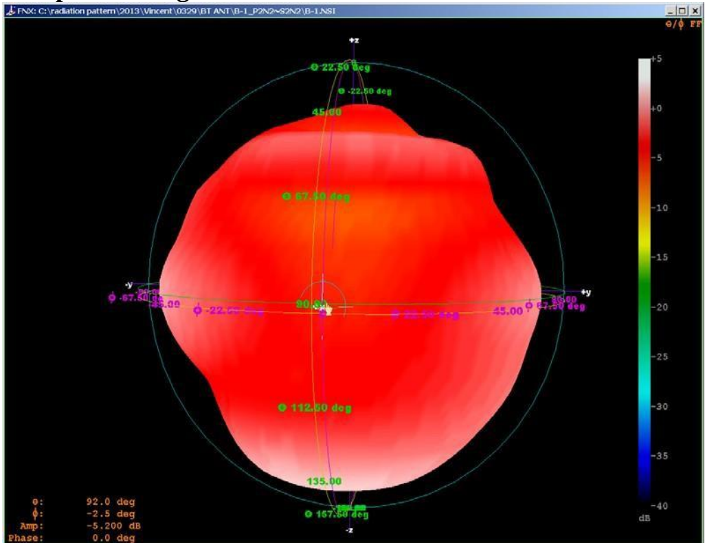
Far-field Power Distribution(H+V) on X-Y Plane Plot AvgGain(H+V)=-0.48dB @2.44000 GHz
