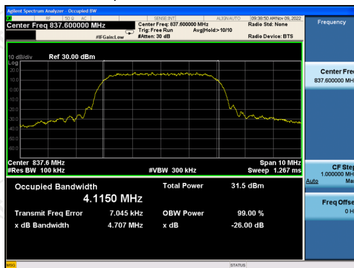
26dB&99% Occupied Bandwidth Plot on Channel 437
