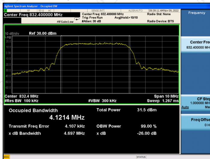
26dB&99% Occupied Bandwidth Plot on Channel 338
