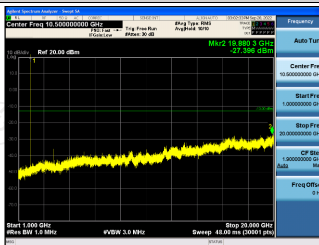
Band25-20MHz-16QAM-26590-1RB#0-Range2:1000~20000MHz
