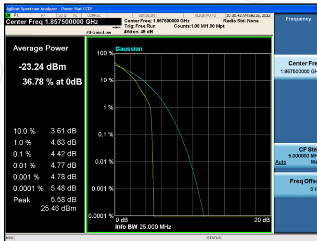
Band2-15MHz-QPSK-18675-75RB#0
