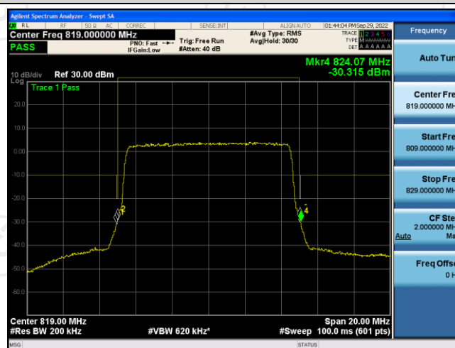
Band26-10MHz-16QAM-26740-50RB#0
