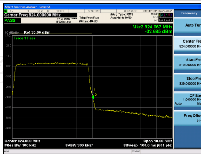
Band26-10MHz-QPSK-26740-50RB#0
