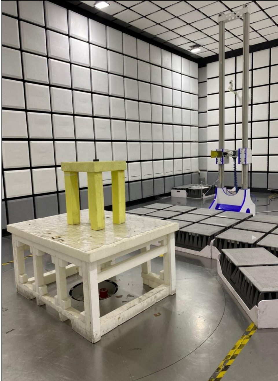
RADIATED EMISSION AND BANDEGE TEST (Above1GHz)
