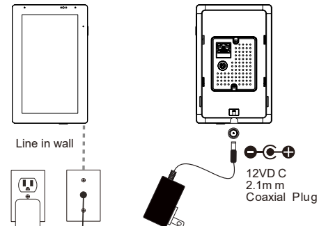
12VDC Power Supply Cabling
