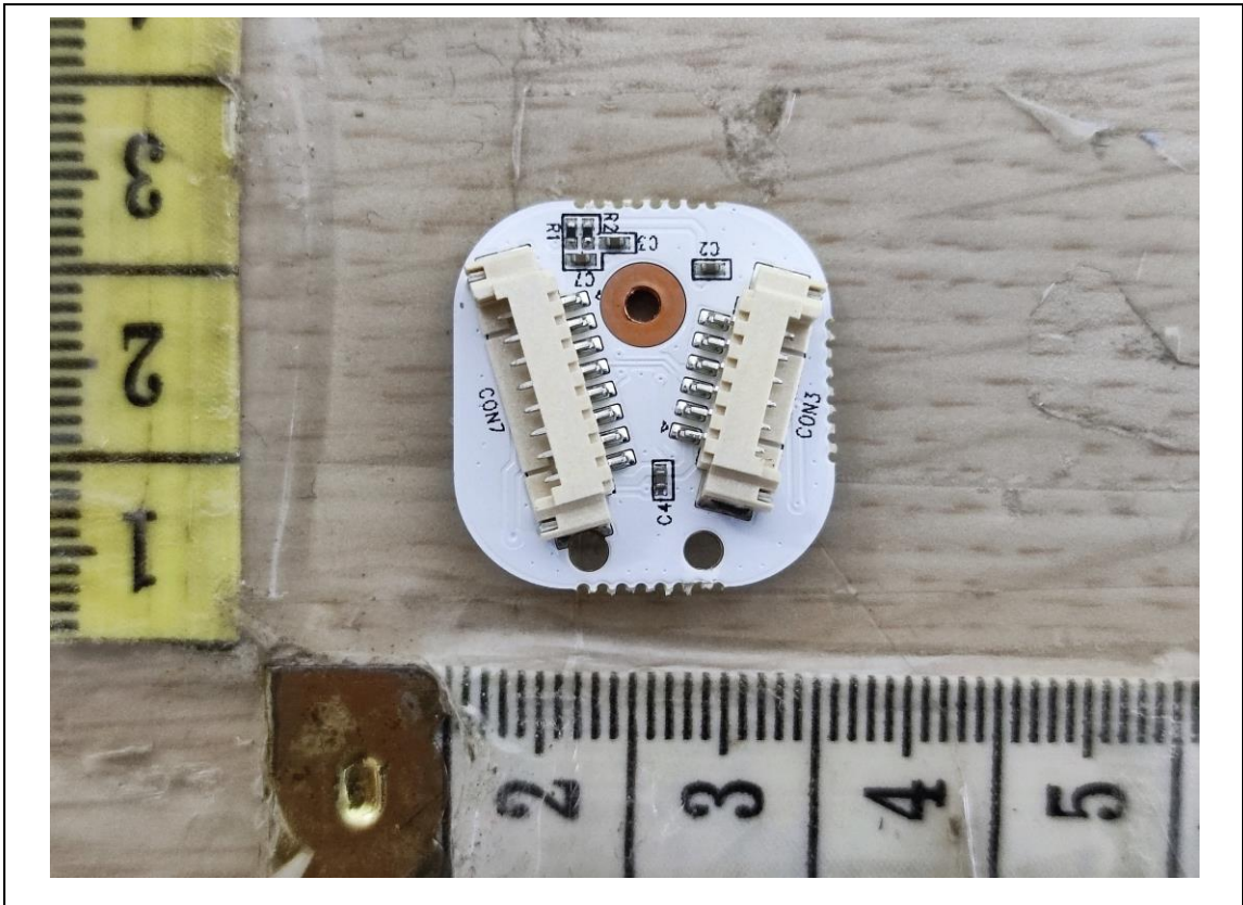
Sub Board
