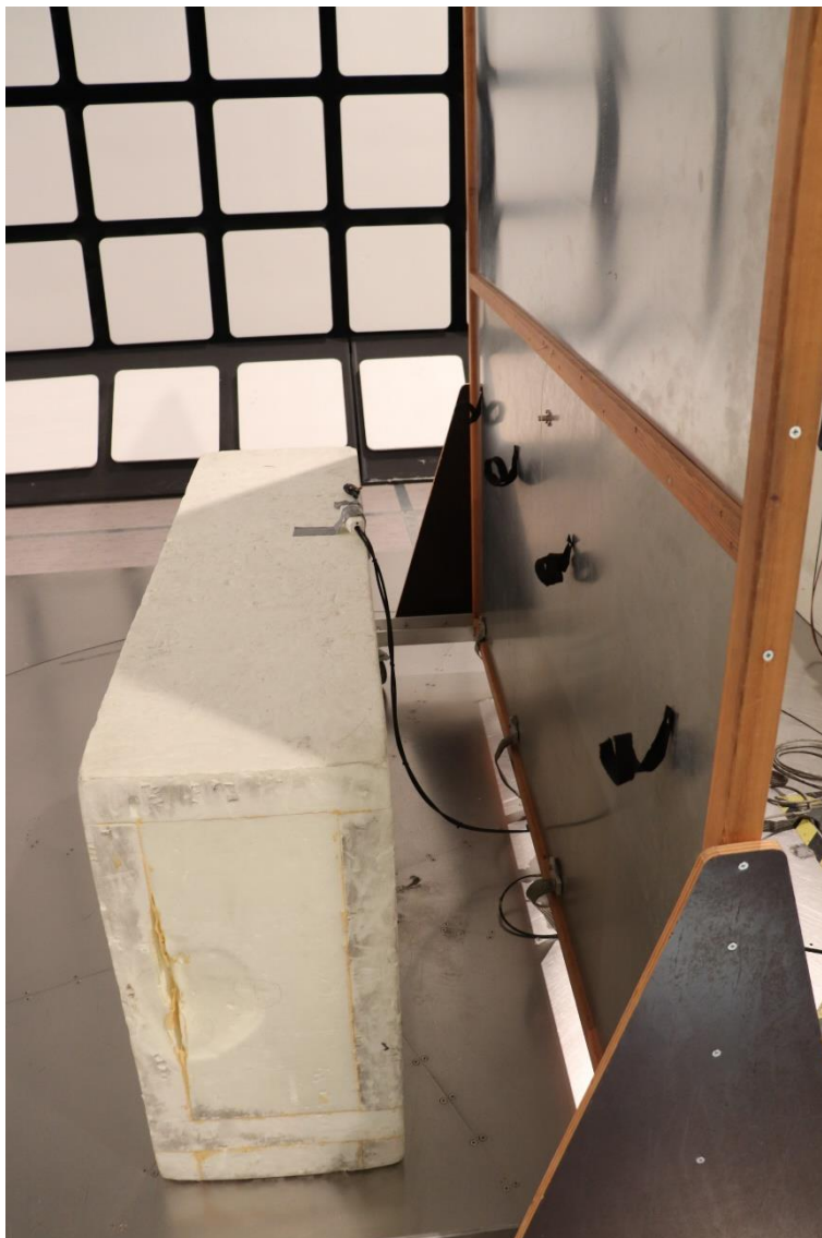
Photograph 1. Test setup for AC Power-Line Conducted Emissions
