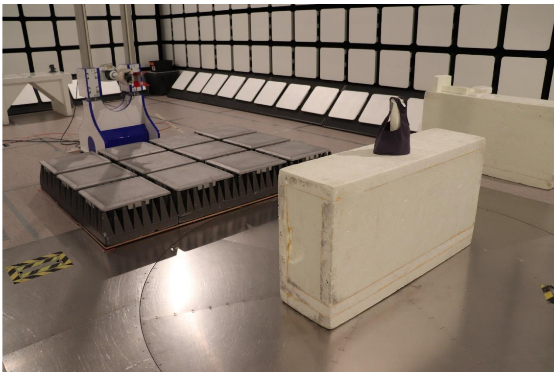
Photograph 4: Test setup for Radiated Emissions (1-12.5 GHz), Operation Mode 1
