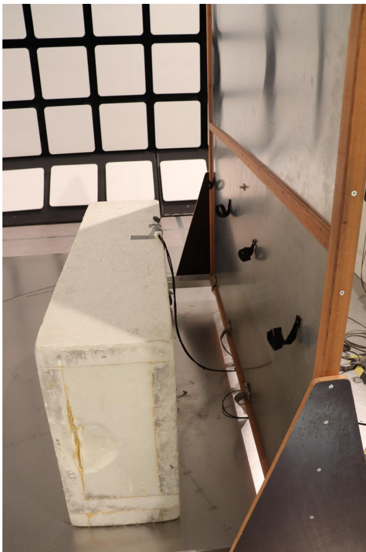
Photograph 1: Test setup for Conducted Emissions
