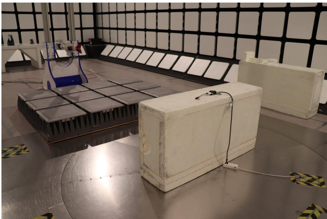
Photograph 7: Test setup for Radiated Emissions (1-12.5 GHz), Operation Mode 2
