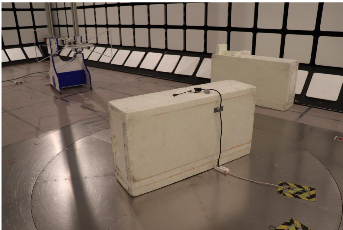
Photograph 6: Test setup for Radiated Emissions (30-1000 MHz), Operation Mode 2
