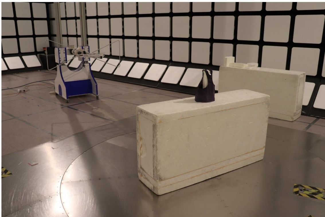
Photograph 3: Test setup for Radiated Emissions (30-1000 MHz), Operation Mode 1
