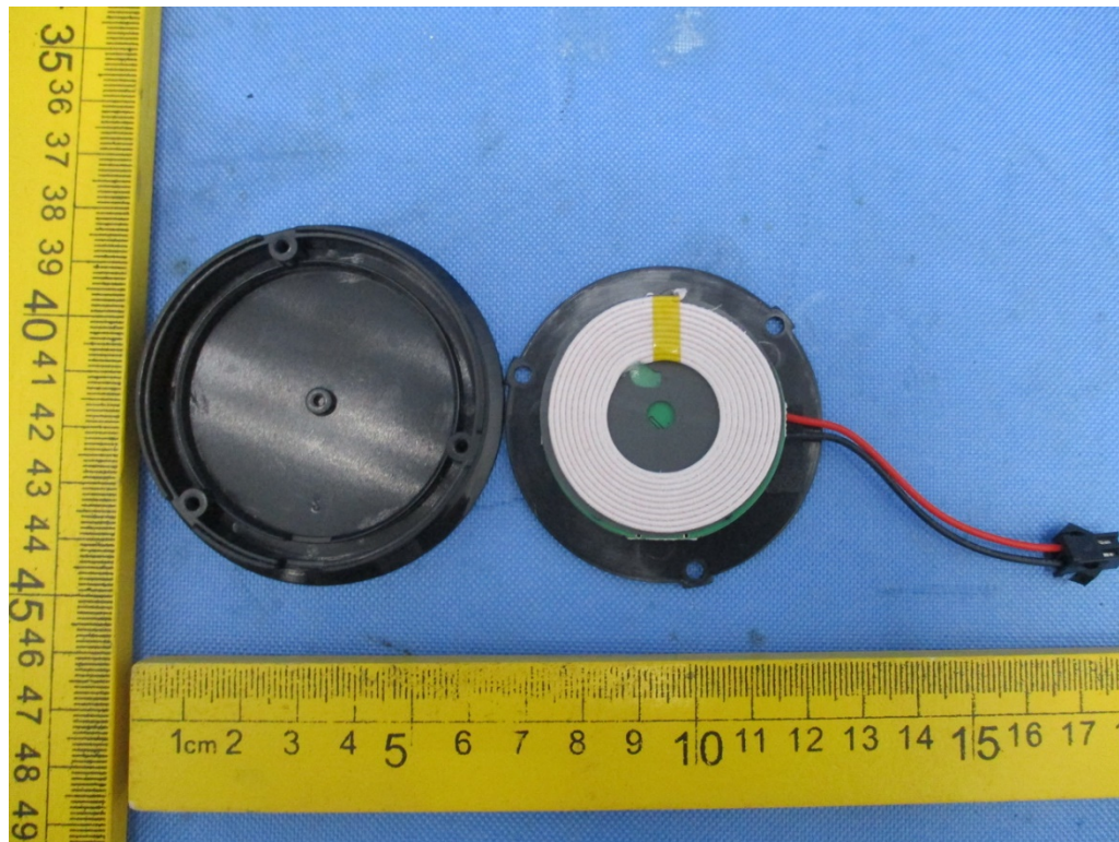
Internal Photo FCC ID: 2A8RMJP-21005A
