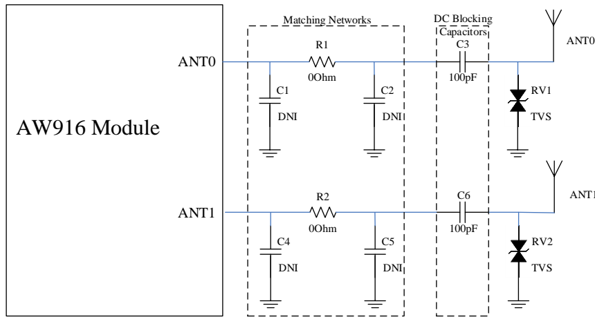
Figure 4-1 Reference design of WiFi/BT antenna interface
