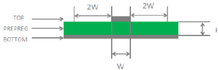
Microstrip Design on a 2-layer PCB
