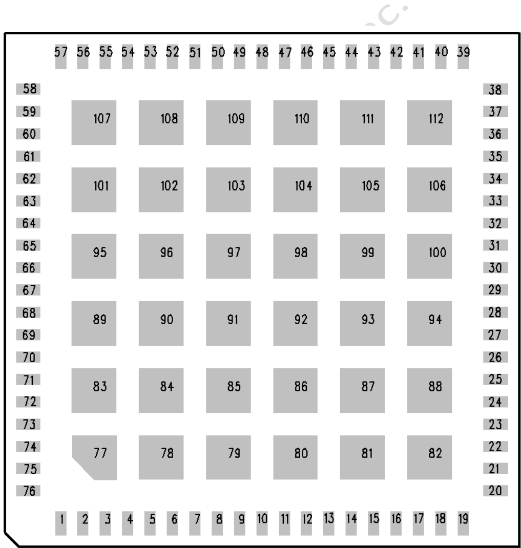
Figure 3-1 Pin distribution (Top perspective)
