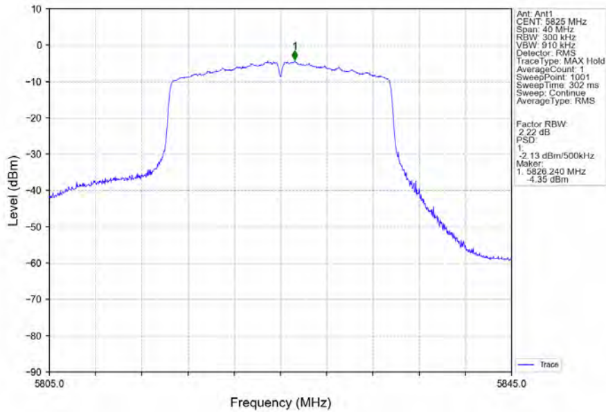
802.11ax(HEW20)_HCH_5825MHz_RU242_Left_Ant1_NTNV
