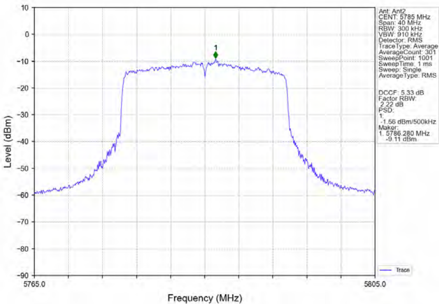
802.11ax(HEW20)_MCH_5785MHz_RU242_Left_Ant2_NTNV
