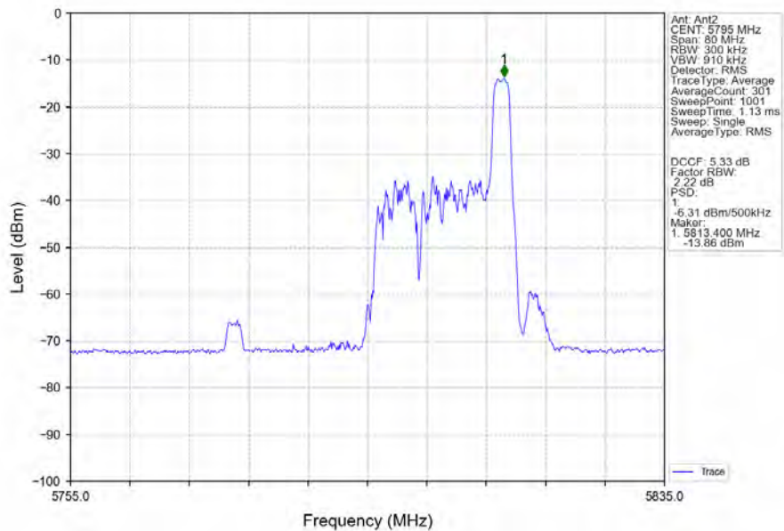
802.11ax(HEW40)_HCH_5795MHz_RU26_Right_Ant2_NTNV
