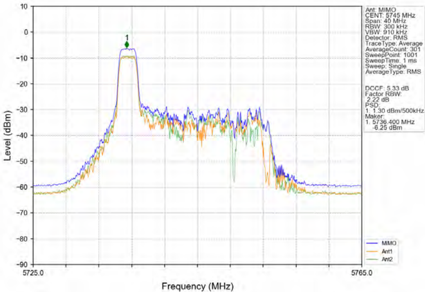
802.11ax(HEW20)_LCH_5745MHz_RU26_Left_MIMO_NTNV
