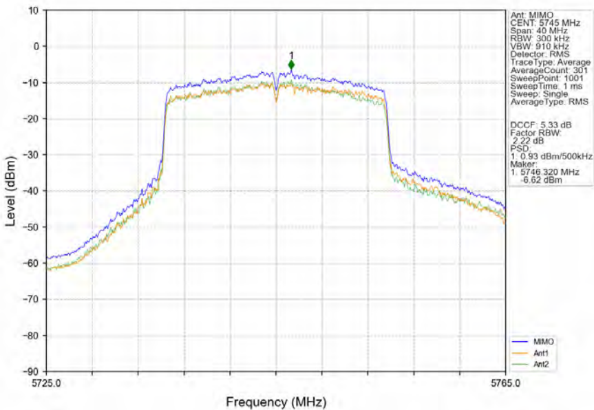
802.11ax(HEW20)_LCH_5745MHz_RU242_Left_MIMO_NTNV
