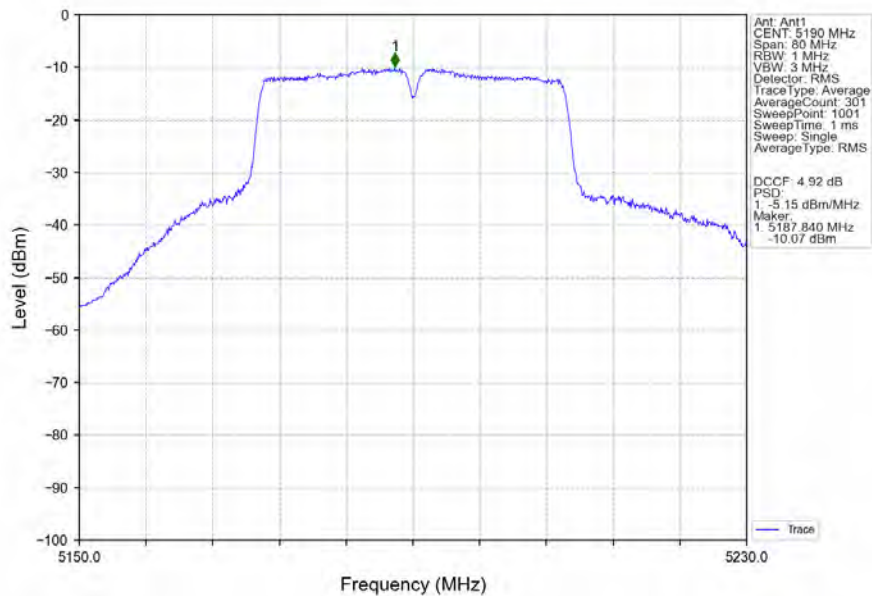
802.11ac(VHT40)_LCH_5190MHz_Ant1_NTNV
