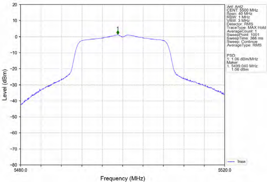
802.11ac(VHT20)_LCH_5500MHz_Ant2_NTNV
