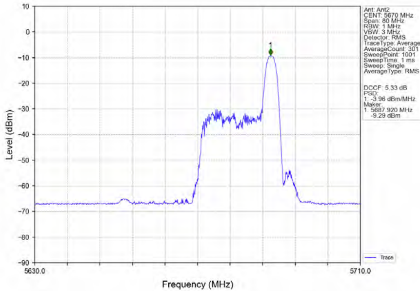
802.11ax(HEW40)_HCH_5670MHz_RU26_Right_Ant2_NTNV
