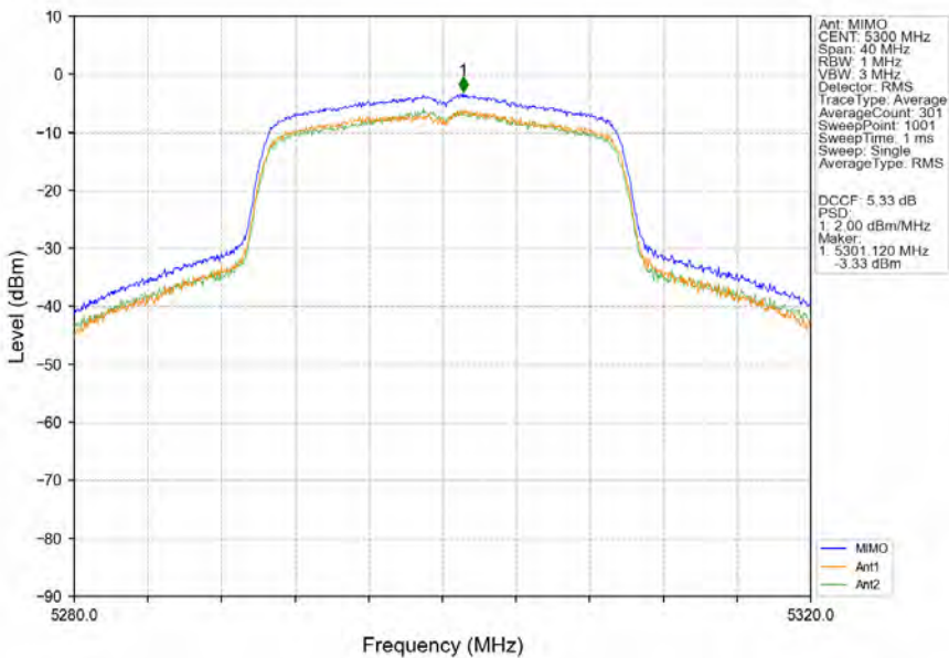
802.11ax(HEW20)_MCH_5300MHz_RU242_Left_MIMO_NTNV
