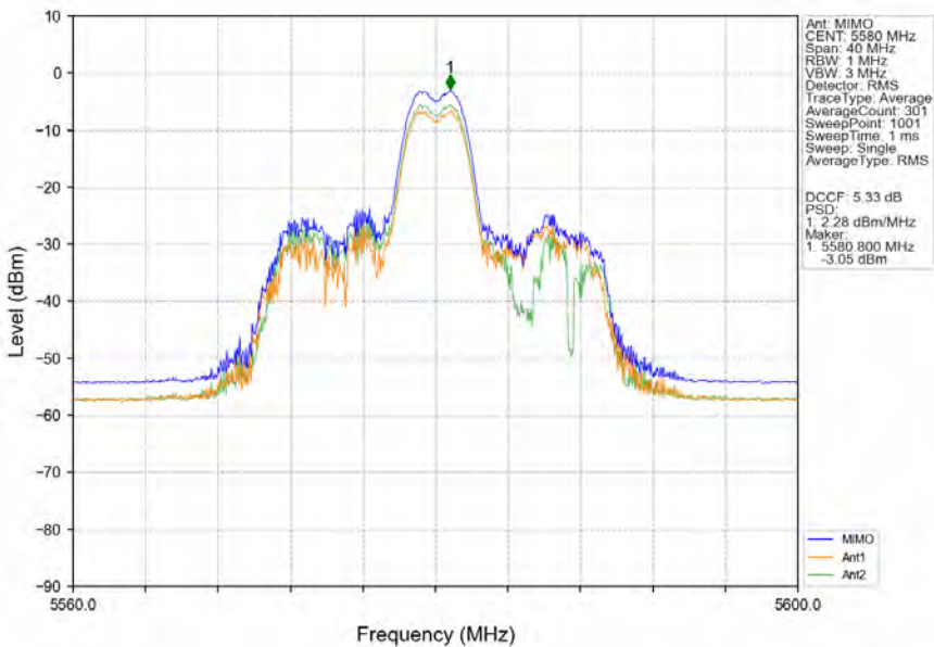
802.11ax(HEW20)_MCH_5580MHz_RU26_Mid_MIMO_NTNV
