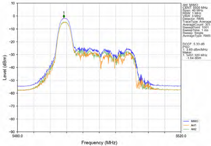
802.11ax(HEW20)_LCH_5500MHz_RU26_Left_MIMO_NTNV
