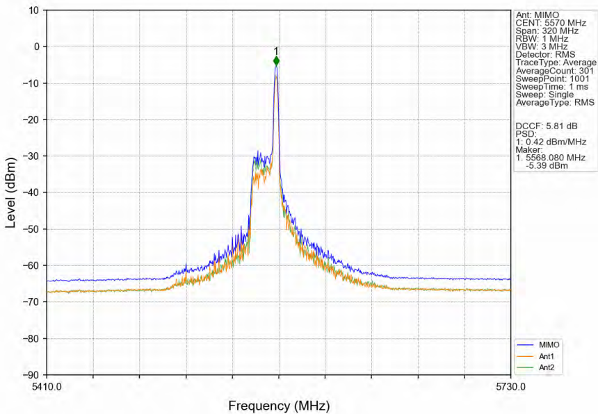
802.11ax(HEW160)_MCH_5570MHz_RU26_Right_MIMO_NTNV
