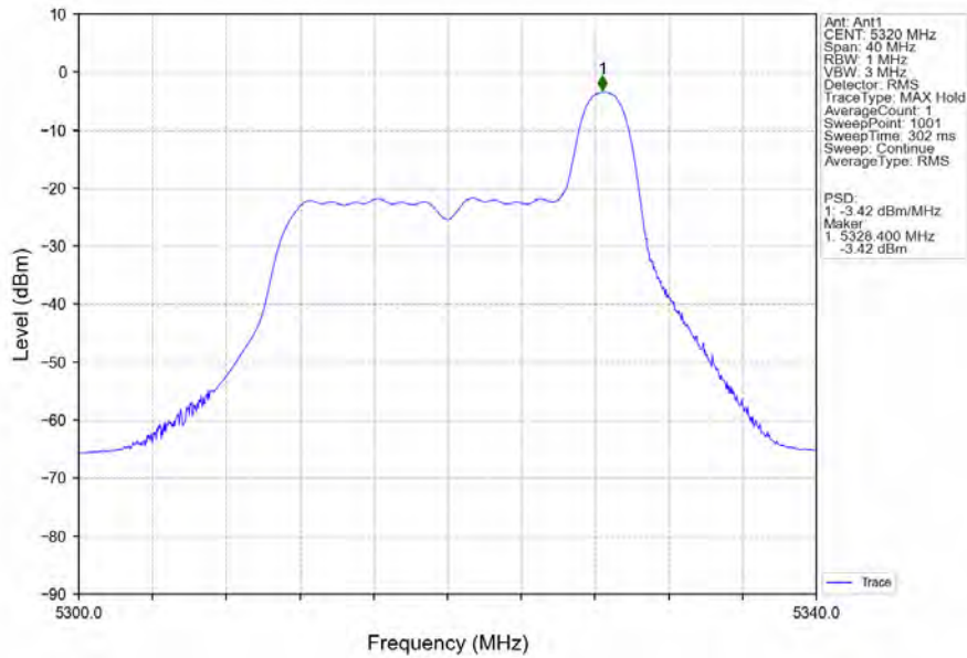
802.11ax(HEW20)_HCH_5320MHz_RU26_Right_Ant1_NTNV
