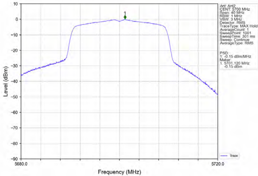
802.11ax(HEW20)_HCH_5700MHz_RU242_Left_Ant2_NTNV
