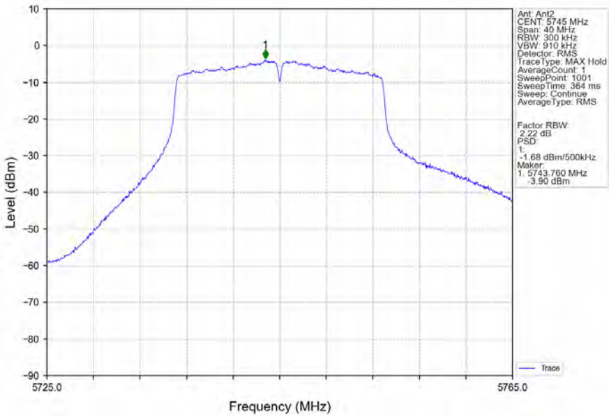
802.11ac(VHT20)_LCH_5745MHz_Ant2_NTNV
