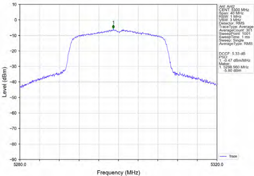
802.11ax(HEW20)_MCH_5300MHz_RU242_Left_Ant2_NTNV
