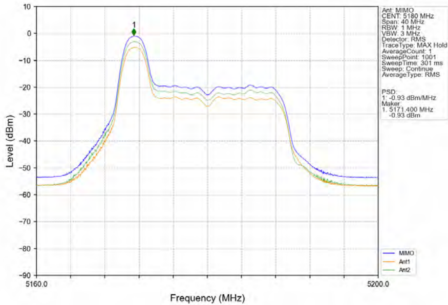
802.11ax(HEW20)_LCH_5180MHz_RU26_Left_MIMO_NTNV
