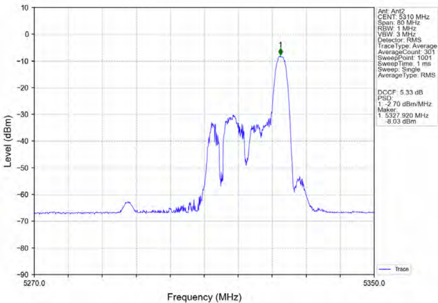
802.11ax(HEW40)_HCH_5310MHz_RU26_Right_Ant2_NTNV
