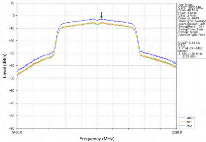
802.11ax(HEW20)_LCH_5500MHz_RU242_Left_MIMO_NTNV
