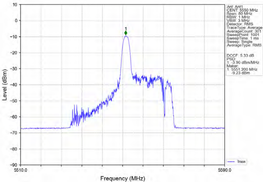
802.11ax(HEW40)_MCH_5550MHz_RU26_Mid_Ant1_NTNV
