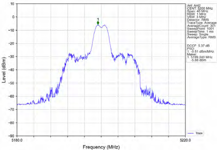
802.11ax(HEW20)_MCH_5200MHz_RU26_Mid_Ant2_NTNV
