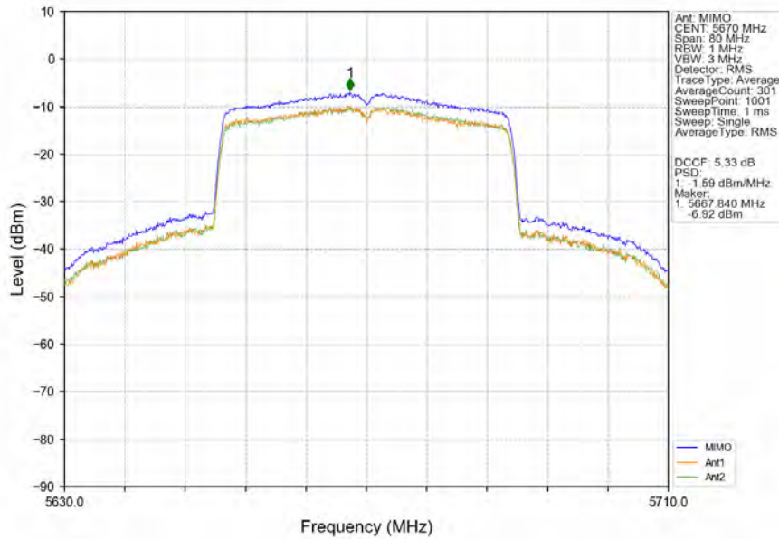
802.11ax(HEW40)_HCH_5670MHz_RU484_Left_MIMO_NTNV
