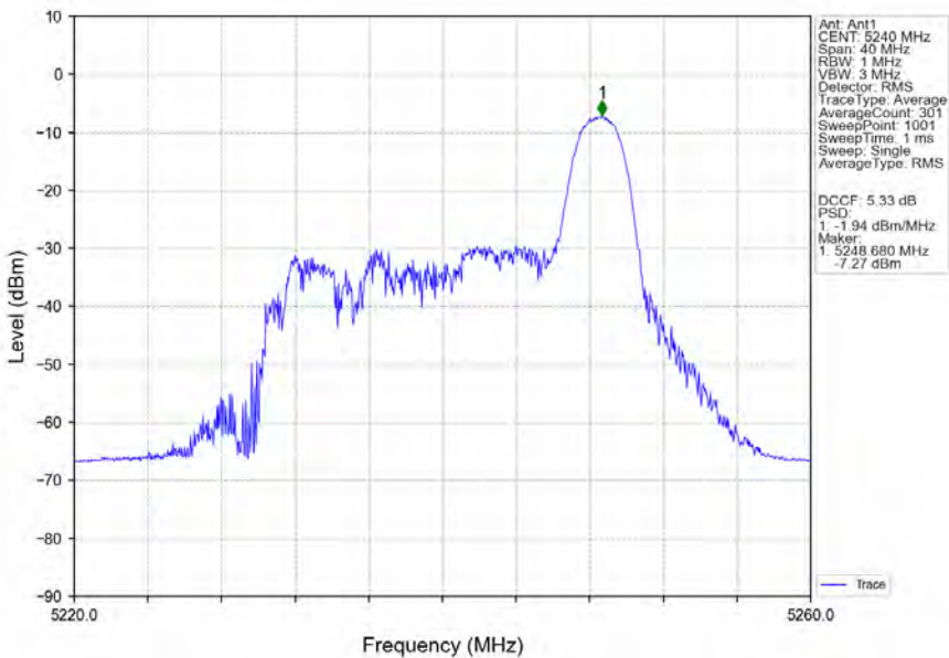
802.11ax(HEW20)_HCH_5240MHz_RU26_Right_Ant1_NTNV
