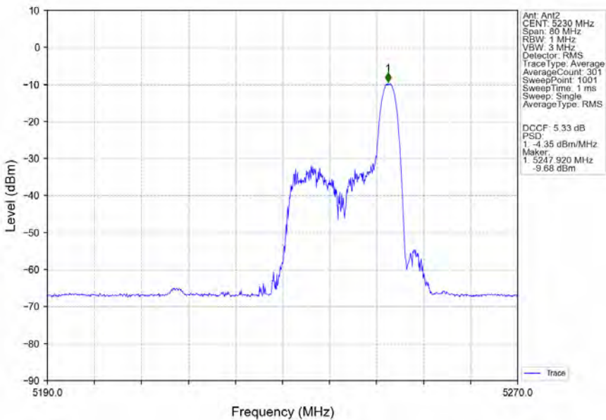
802.11ax(HEW40)_HCH_5230MHz_RU26_Right_Ant2_NTNV
