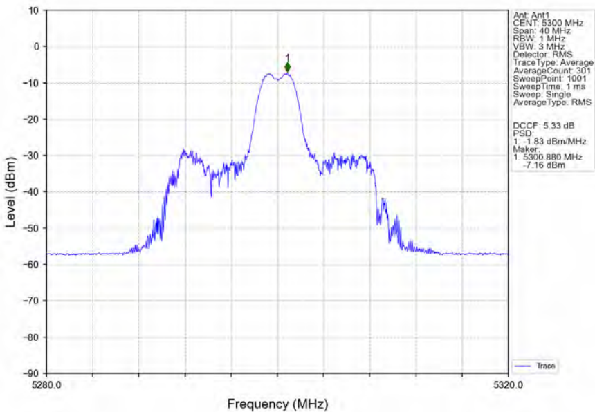
802.11ax(HEW20)_MCH_5300MHz_RU26_Mid_Ant1_NTNV
