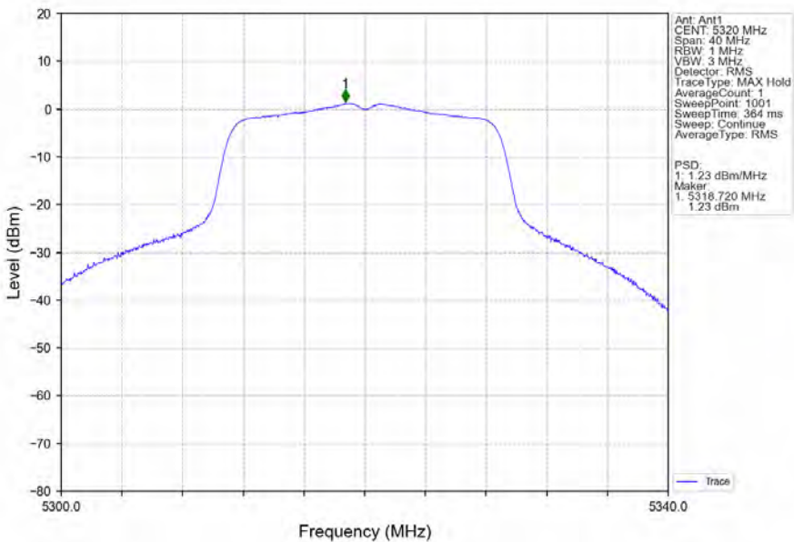
802.11ac(VHT20)_HCH_5320MHz_Ant1_NTNV
