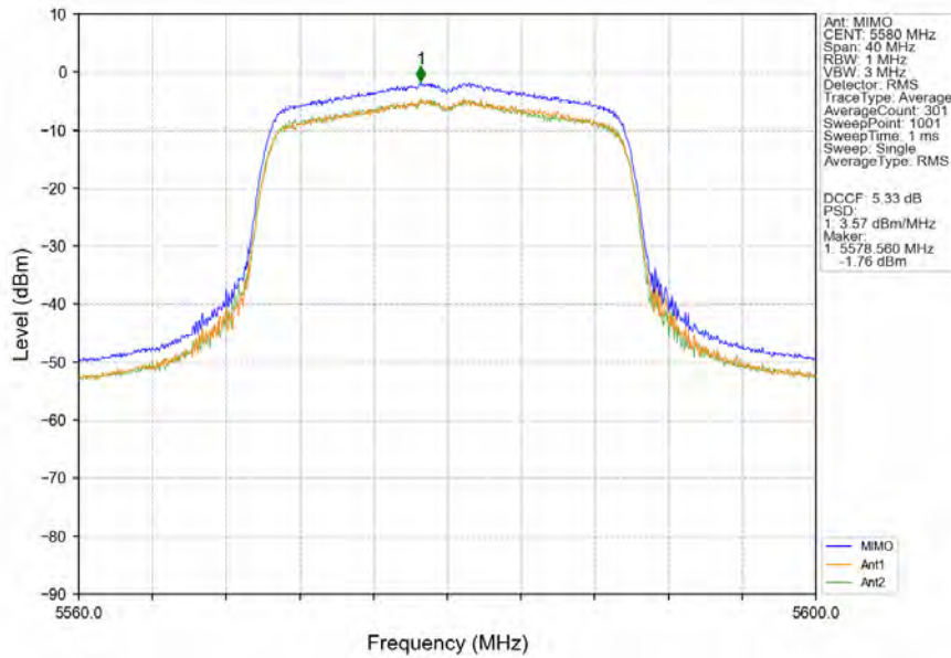
802.11ax(HEW20)_MCH_5580MHz_RU242_Left_MIMO_NTNV
