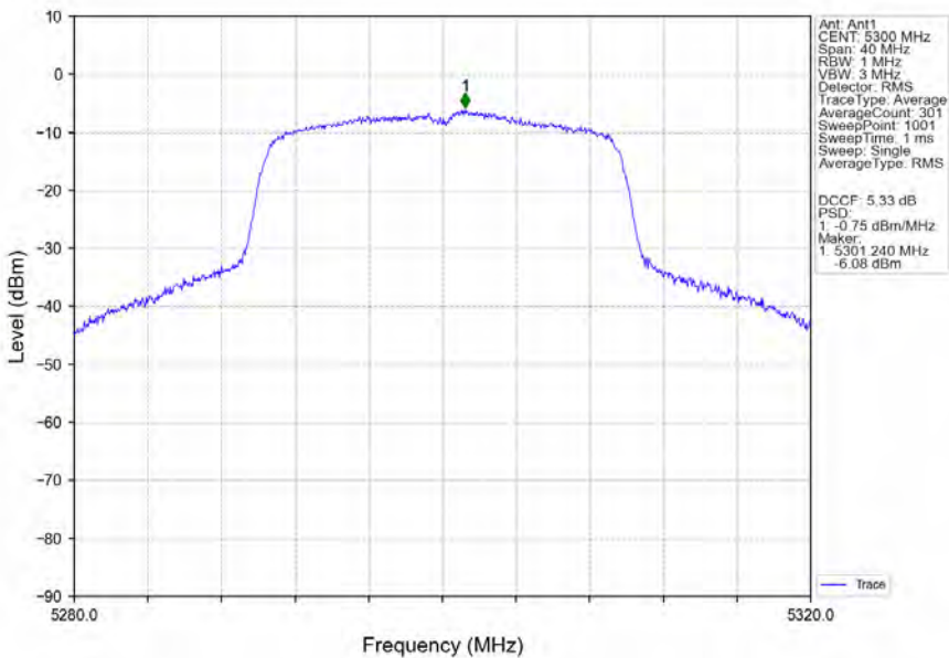
802.11ax(HEW20)_MCH_5300MHz_RU242_Left_Ant1_NTNV
