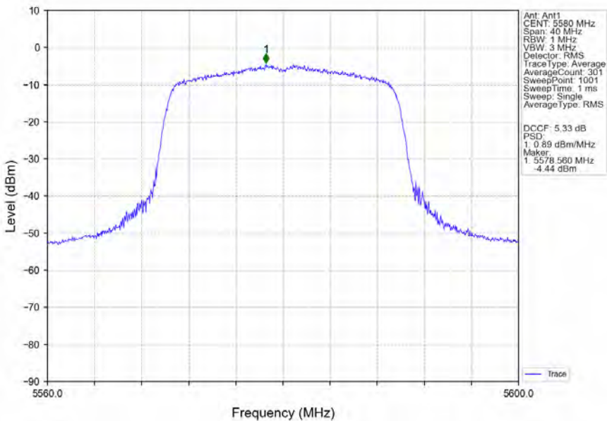
802.11ax(HEW20)_MCH_5580MHz_RU242_Left_Ant1_NTNV
