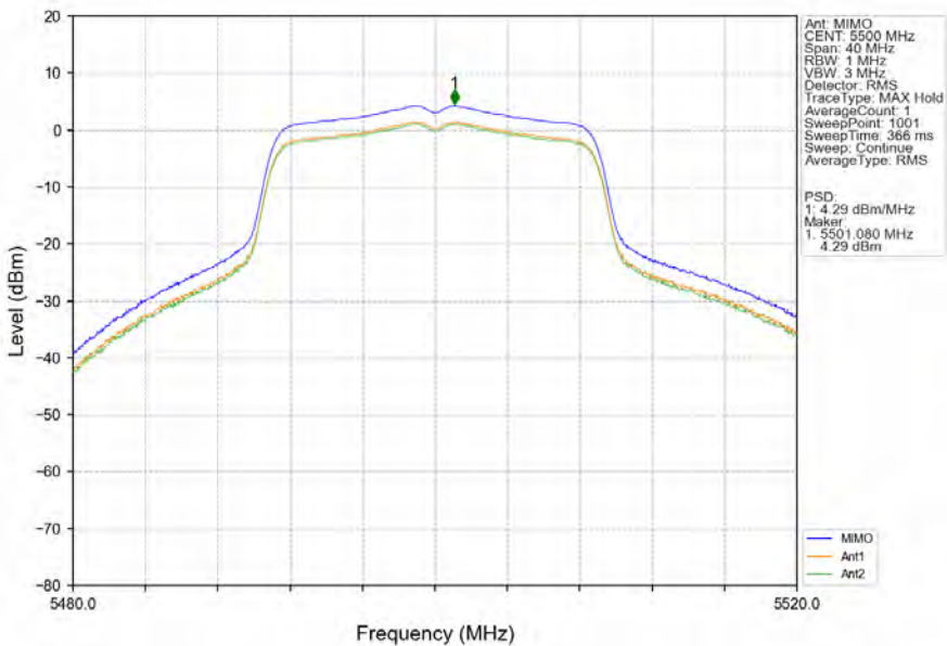
802.11ac(VHT20)_LCH_5500MHz_MIMO_NTNV
