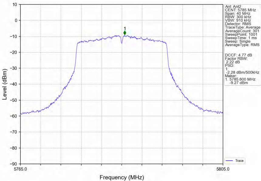
802.11ac(VHT20)_MCH_5785MHz_Ant2_NTNV
