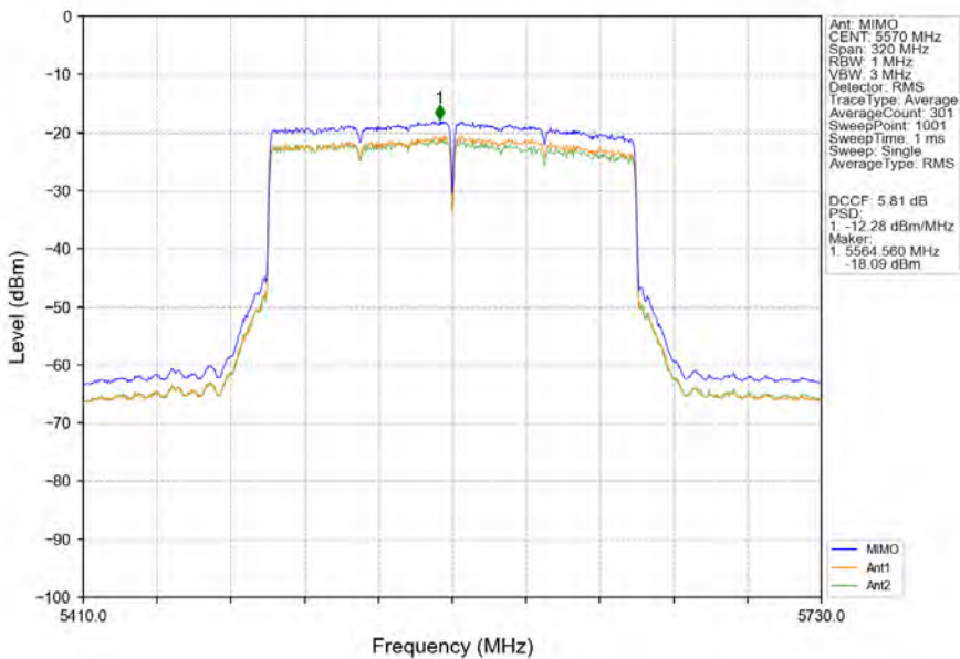
802.11ax(HEW160)_MCH_5570MHz_2xRU996_Left_MIMO_NTNV
