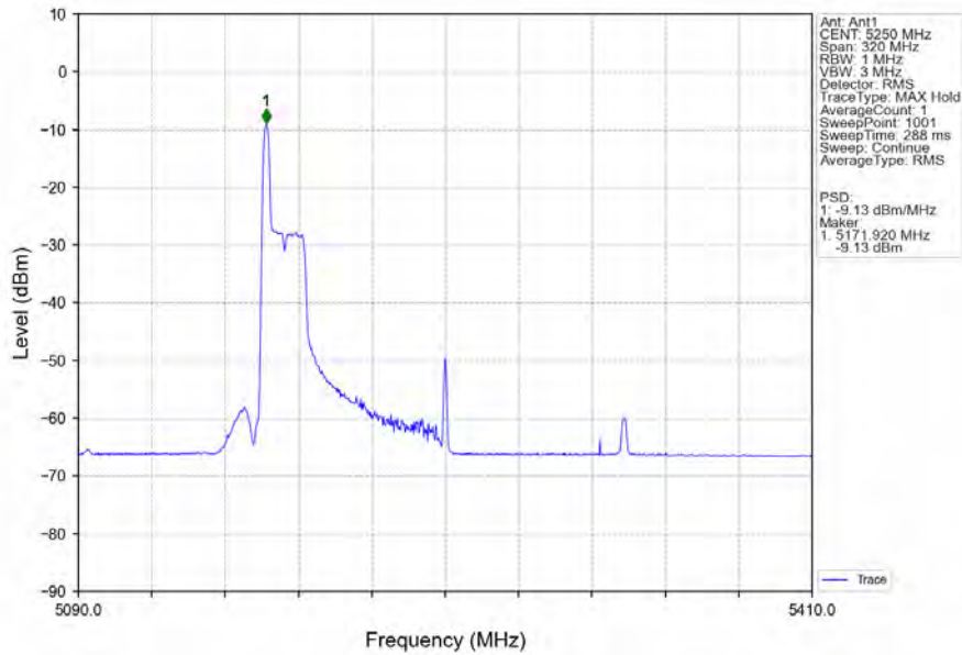
802.11ax(HEW160)_MCH_5250MHz_RU26_Left_Ant1_NTNV
