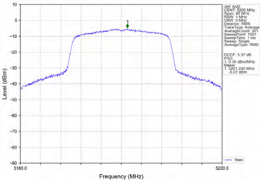
802.11ax(HEW20)_MCH_5200MHz_RU242_Left_Ant2_NTNV
