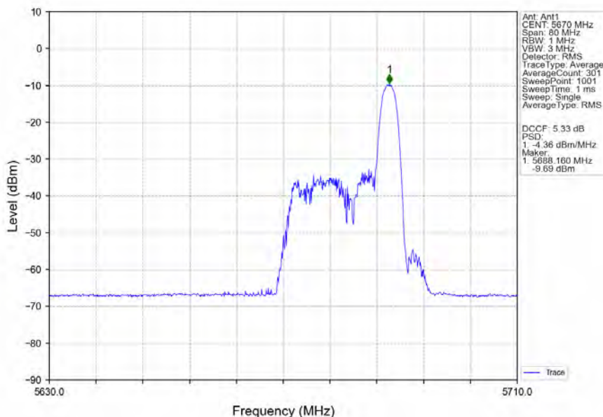
802.11ax(HEW40)_HCH_5670MHz_RU26_Right_Ant1_NTNV
