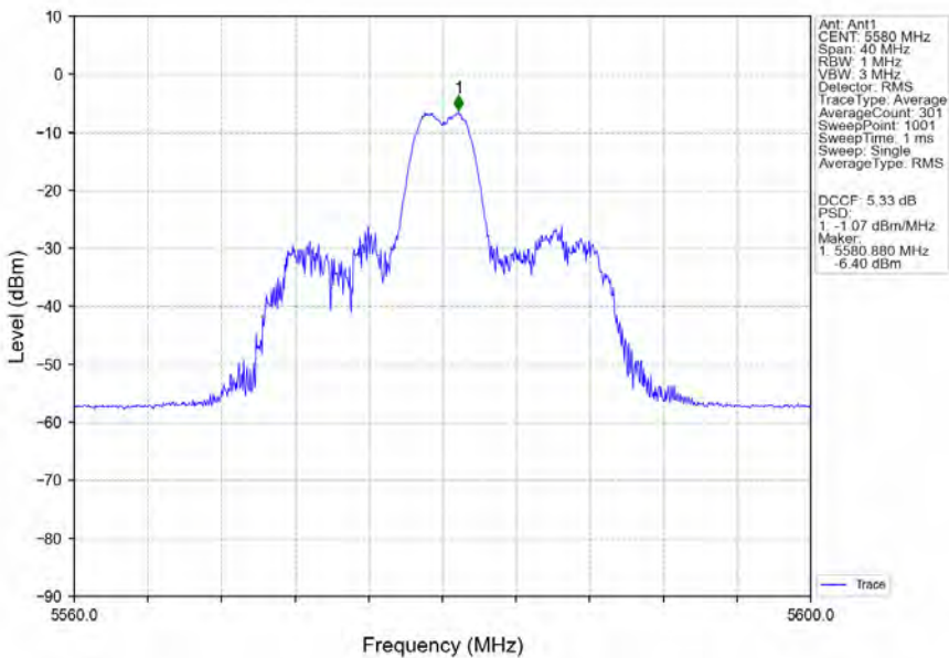
802.11ax(HEW20)_MCH_5580MHz_RU26_Mid_Ant1_NTNV
