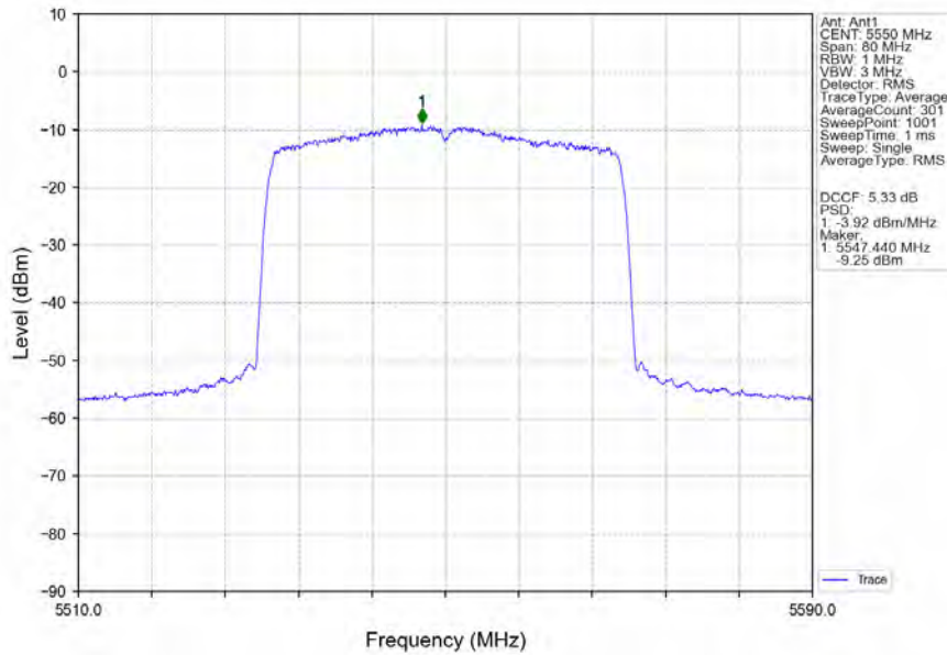
802.11ax(HEW40)_MCH_5550MHz_RU484_Left_Ant1_NTNV
