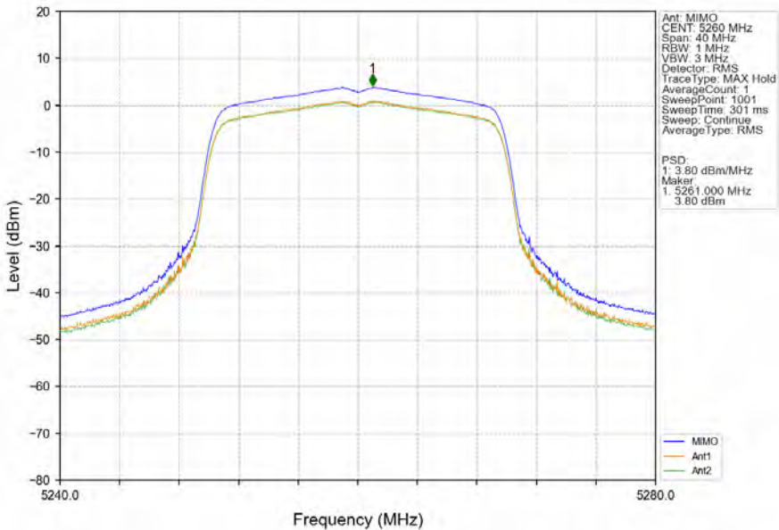
802.11ax(HEW20)_LCH_5260MHz_RU242_Left_MIMO_NTNV
