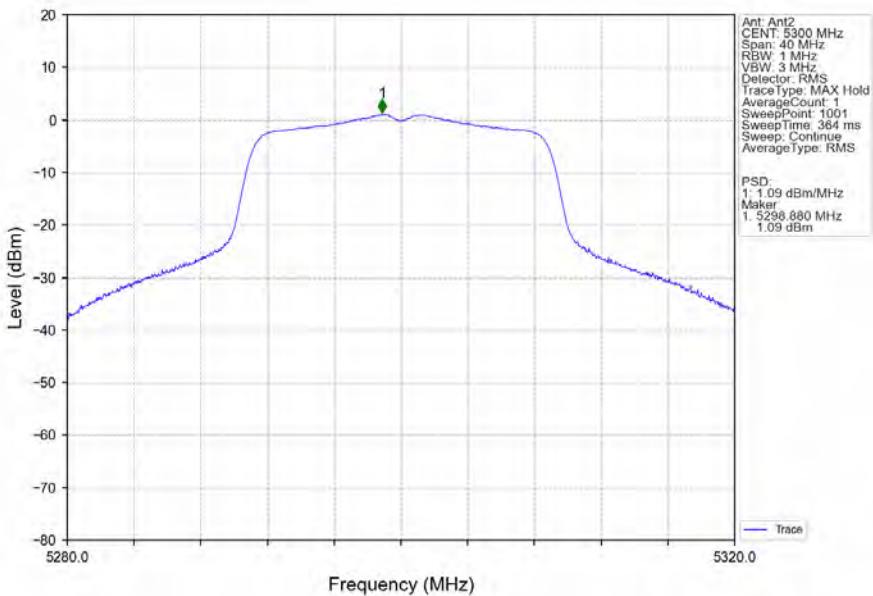
802.11ac(VHT20)_MCH_5300MHz_Ant2_NTNV
