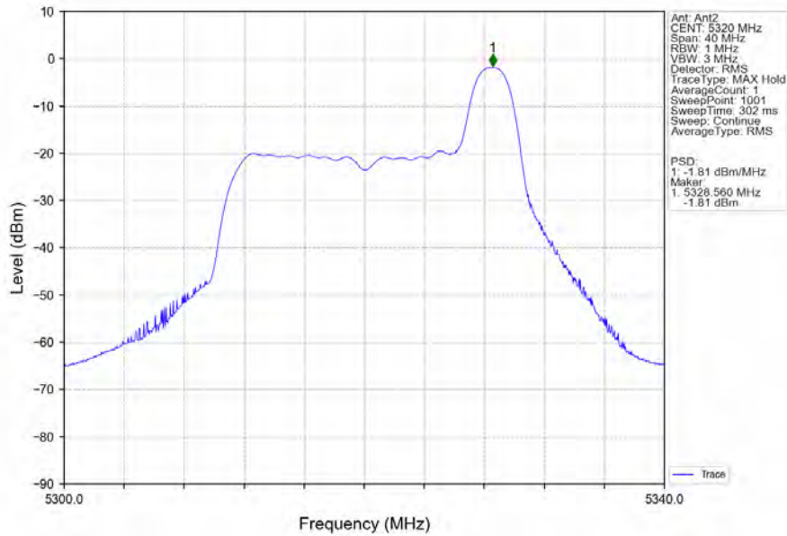
802.11ax(HEW20)_HCH_5320MHz_RU26_Right_Ant2_NTNV
