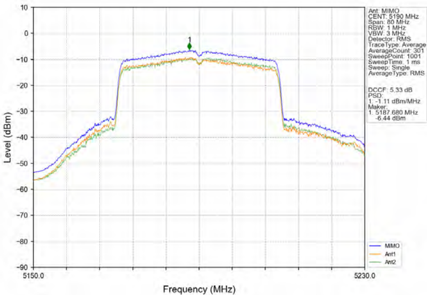
802.11ax(HEW40)_LCH_5190MHz_RU484_Left_MIMO_NTNV
