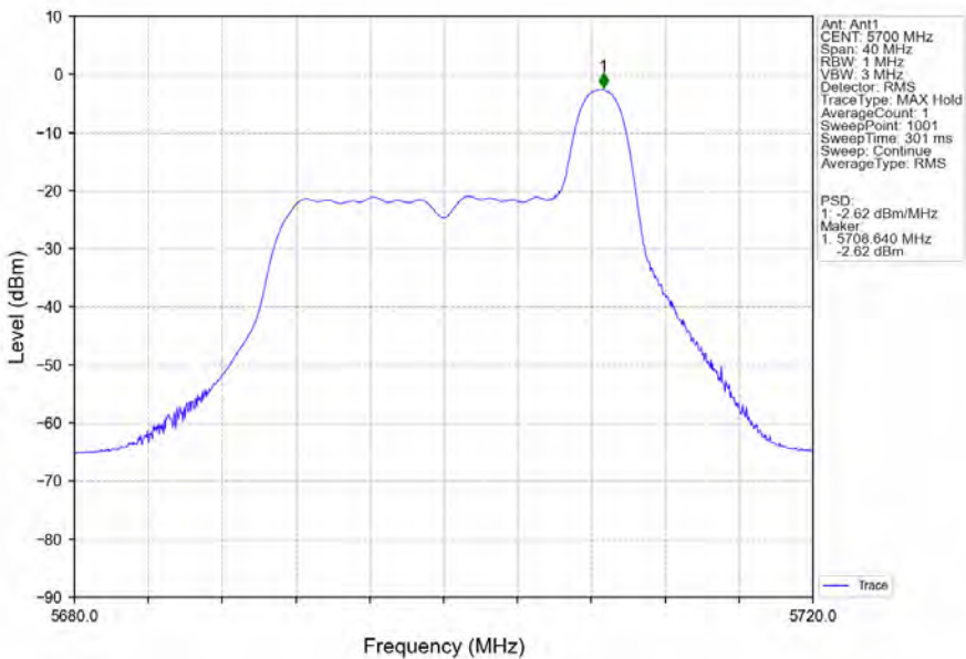
802.11ax(HEW20)_HCH_5700MHz_RU26_Right_Ant1_NTNV
