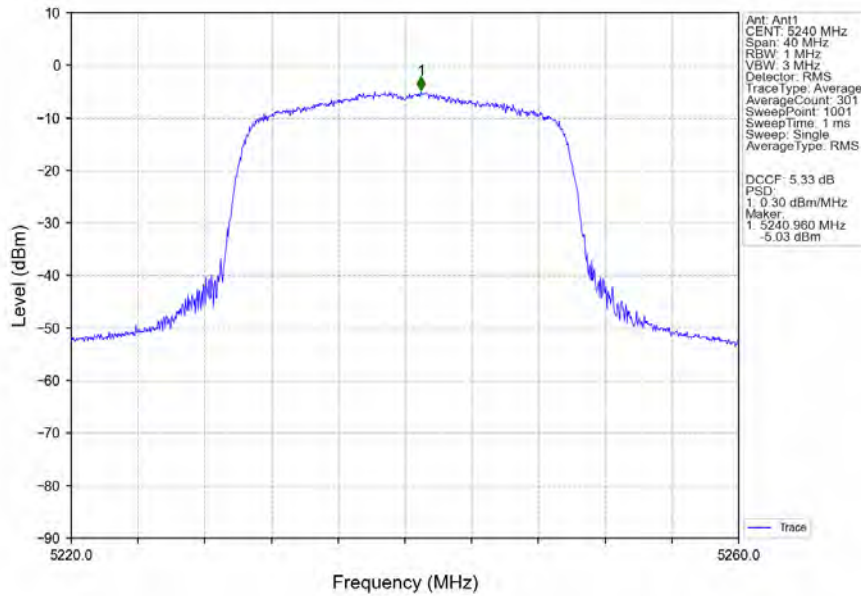
802.11ax(HEW20)_HCH_5240MHz_RU242_Left_Ant1_NTNV
