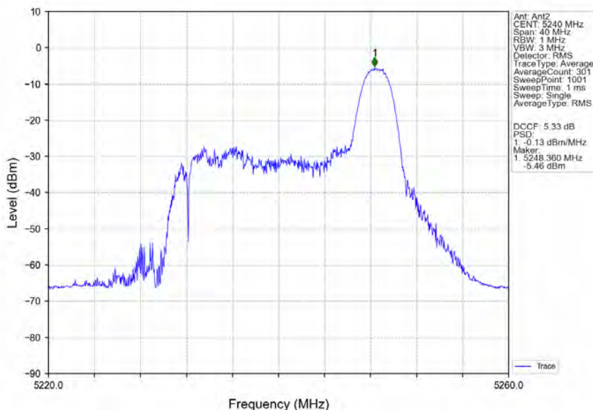
802.11ax(HEW20)_HCH_5240MHz_RU26_Right_Ant2_NTNV
