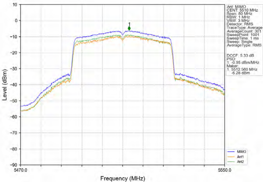
802.11ax(HEW40)_LCH_5510MHz_RU484_Left_MIMO_NTNV
