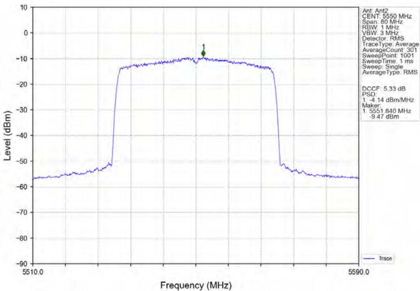
802.11ax(HEW40)_MCH_5550MHz_RU484_Left_Ant2_NTNV
