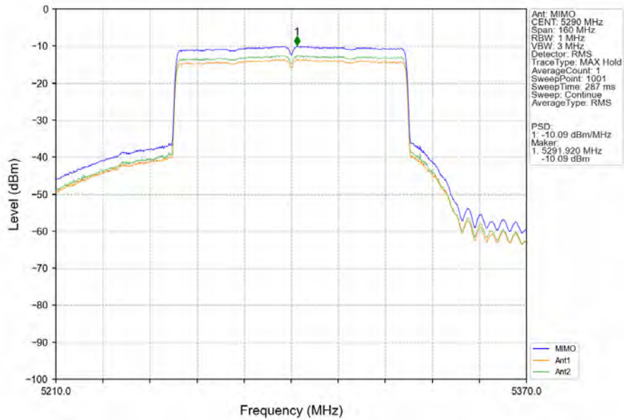
802.11ax(HEW80)_MCH_5290MHz_RU996_Left_MIMO_NTNV
