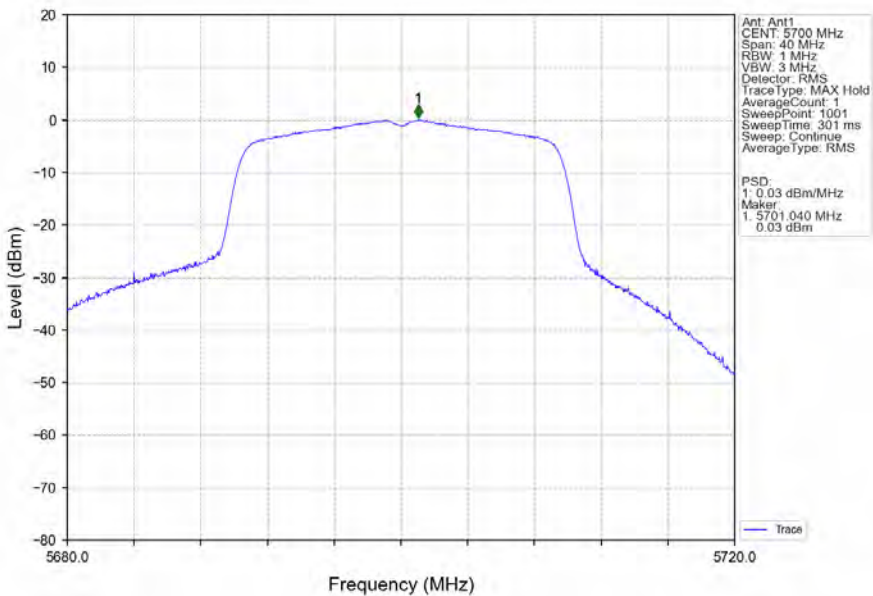
802.11ax(HEW20)_HCH_5700MHz_RU242_Left_Ant1_NTNV
