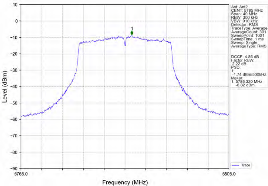
802.11n(HT20)_MCH_5785MHz_Ant2_NTNV
