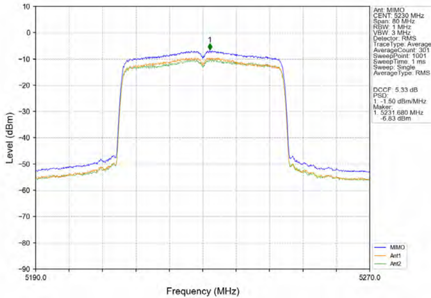
802.11ax(HEW40)_HCH_5230MHz_RU484_Left_MIMO_NTNV
