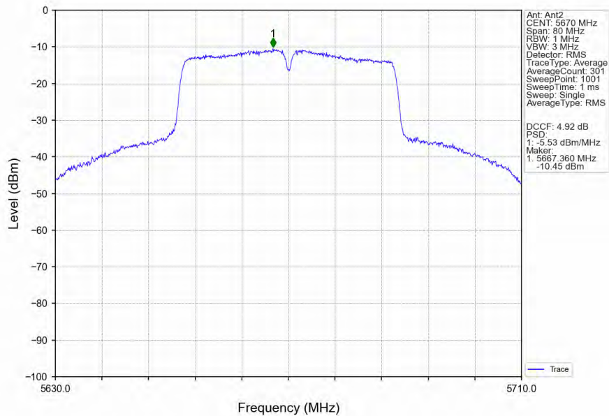
802.11ac(VHT40)_HCH_5670MHz_Ant2_NTNV
