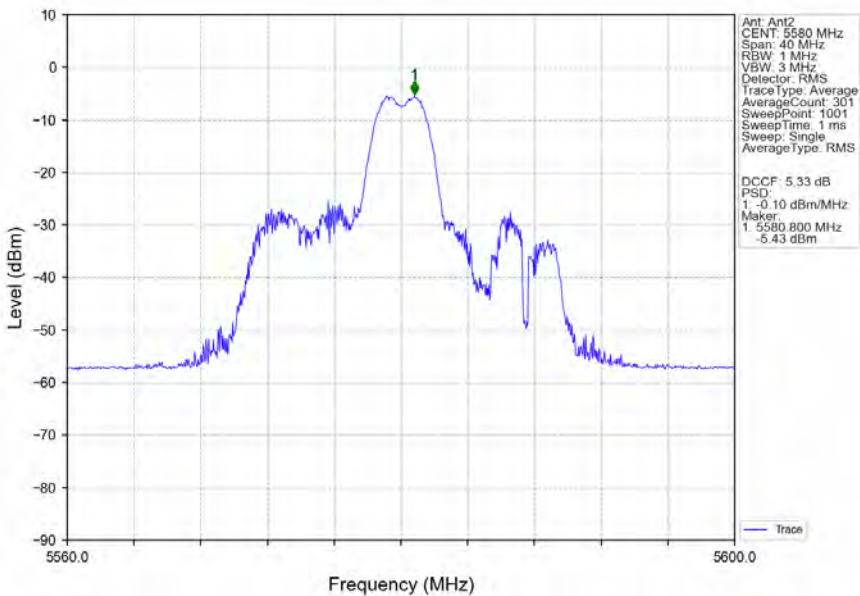
802.11ax(HEW20)_MCH_5580MHz_RU26_Mid_Ant2_NTNV
