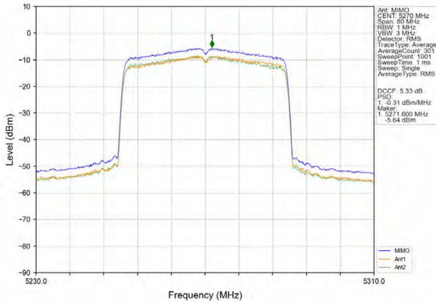
802.11ax(HEW40)_LCH_5270MHz_RU484_Left_MIMO_NTNV
