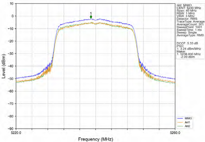
802.11ax(HEW20)_HCH_5240MHz_RU242_Left_MIMO_NTNV
