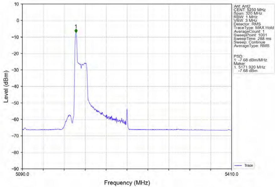
802.11ax(HEW160)_MCH_5250MHz_RU26_Left_Ant2_NTNV
