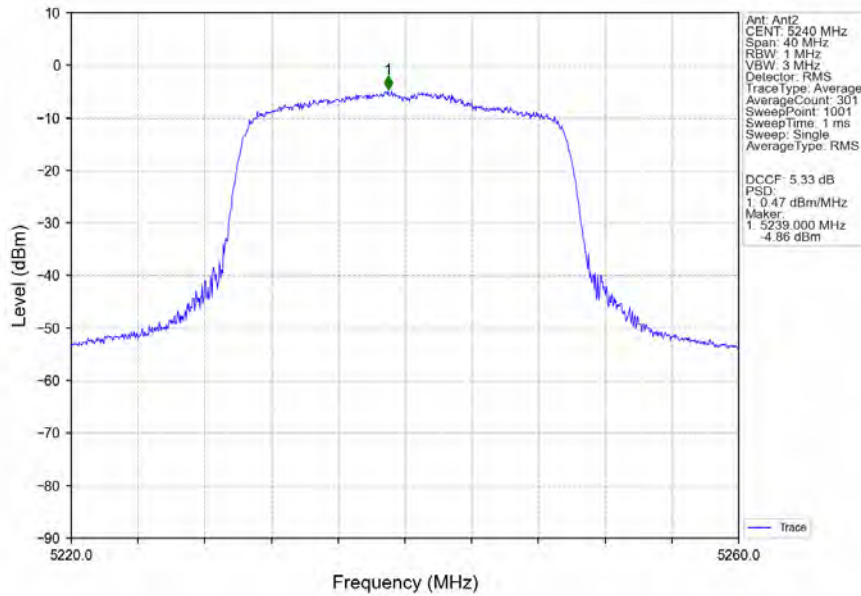
802.11ax(HEW20)_HCH_5240MHz_RU242_Left_Ant2_NTNV
