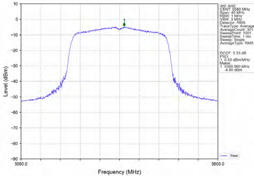
802.11ax(HEW20)_MCH_5580MHz_RU242_Left_Ant2_NTNV
