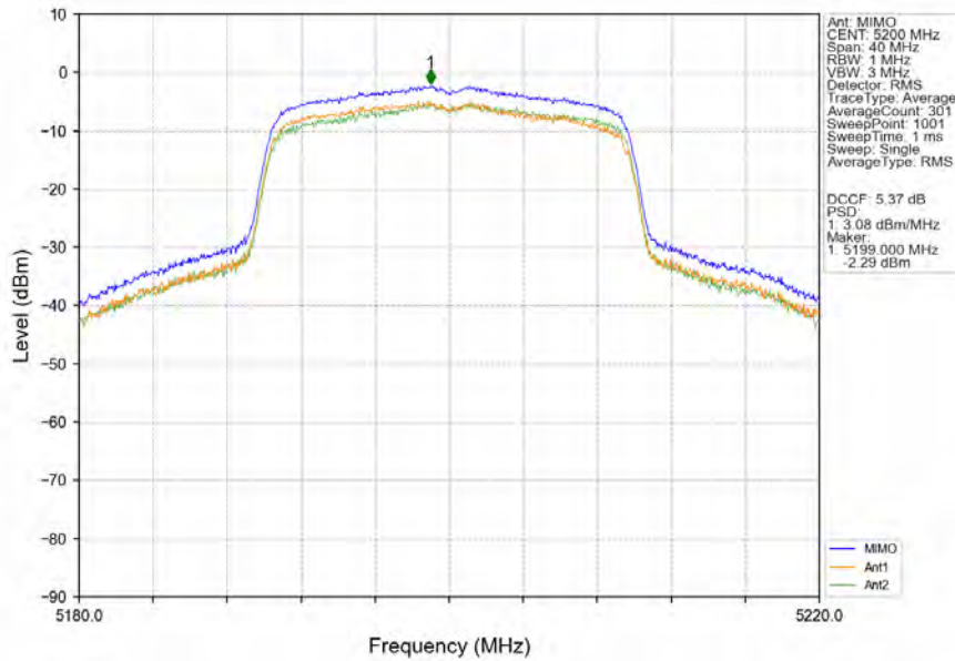
802.11ax(HEW20)_MCH_5200MHz_RU242_Left_MIMO_NTNV
