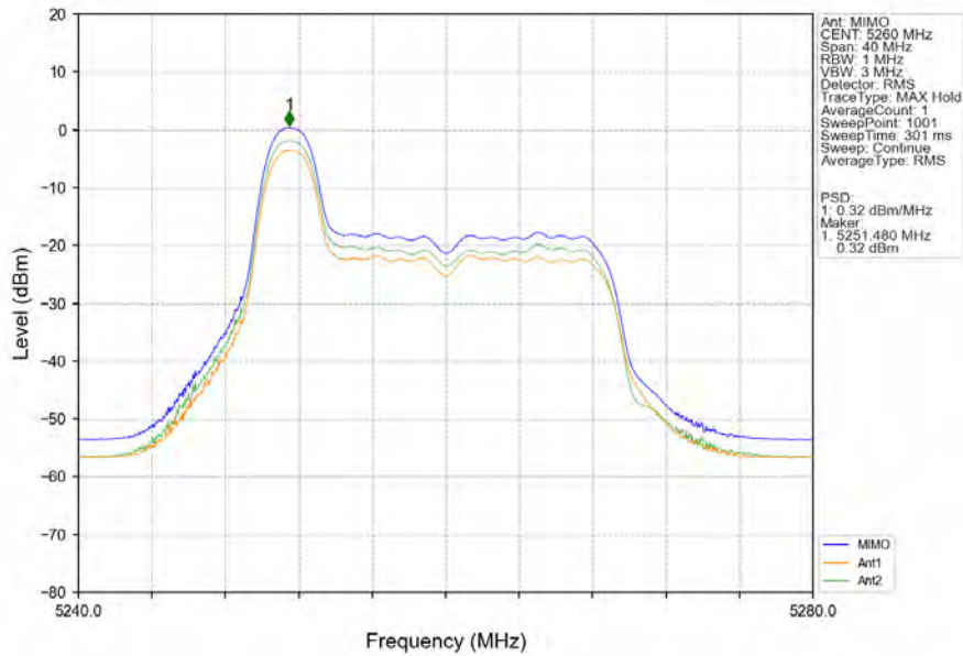
802.11ax(HEW20)_LCH_5260MHz_RU26_Left_MIMO_NTNV
