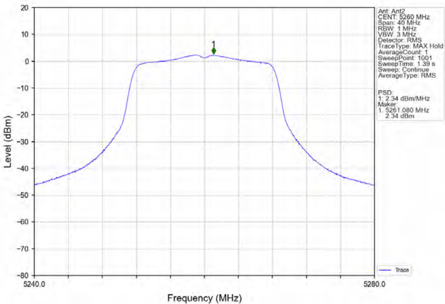
802.11a_LCH_5260MHz_Ant2_NTNV
