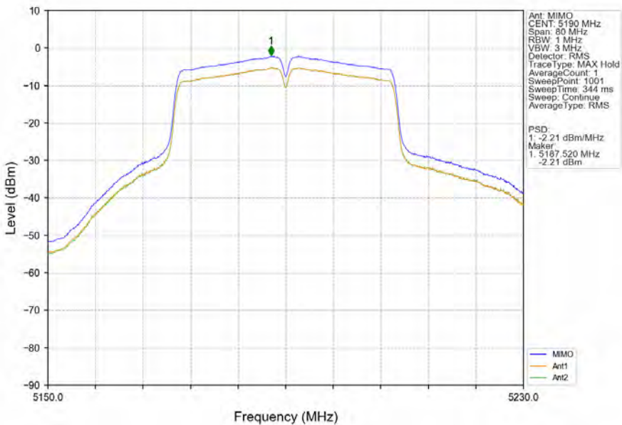
802.11n(HT40)_LCH_5190MHz_MIMO_NTNV
