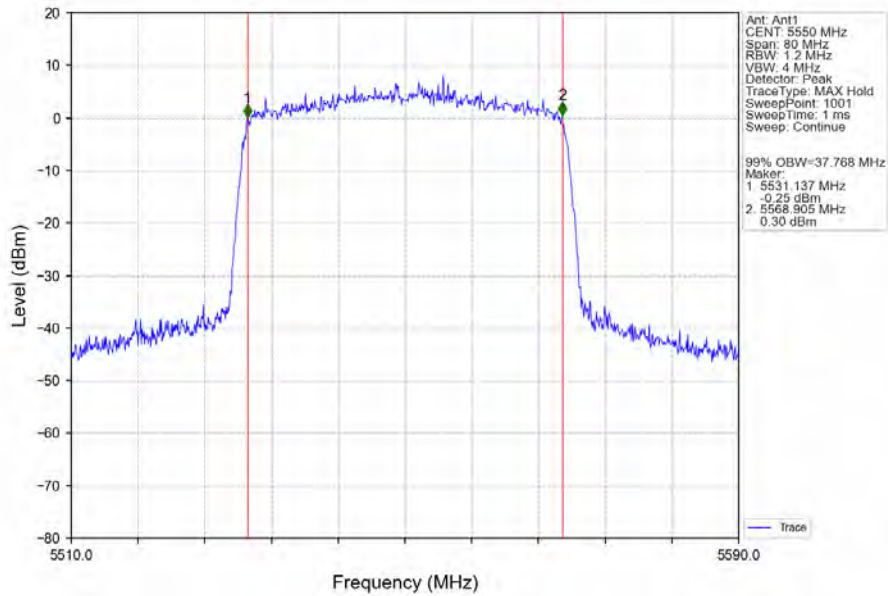
802.11ax(HEW40)_MCH_5550MHz_RU484_Left_Ant1_NTNV
