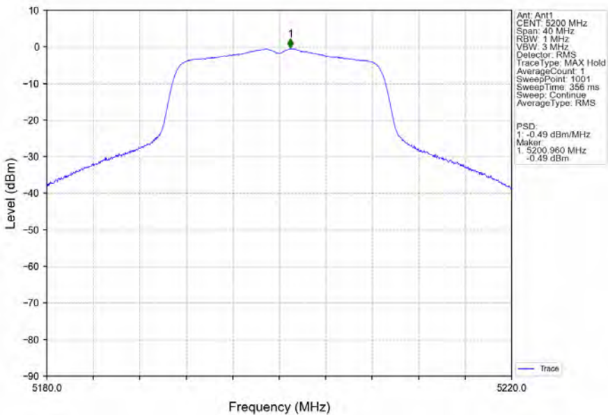
802.11n(HT20)_MCH_5200MHz_Ant1_NTNV
