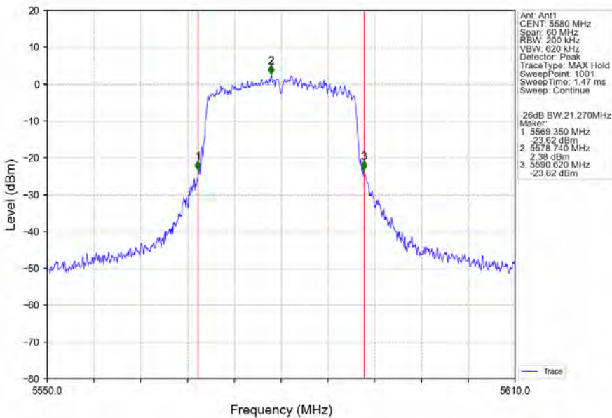
802.11ax(HEW20)_MCH_5580MHz_RU242_Left_Ant1_NTNV
