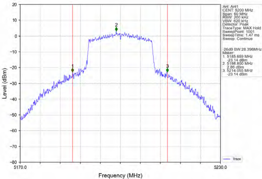
802.11ax(HEW20)_MCH_5200MHz_RU242_Left_Ant1_NTNV
