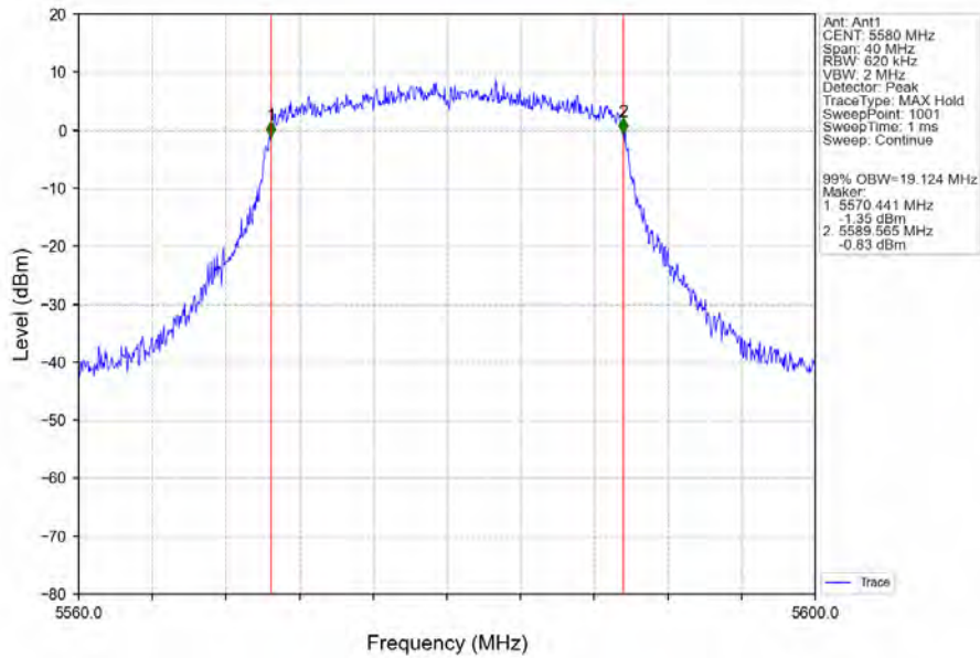
802.11ax(HEW20)_MCH_5580MHz_RU242_Left_Ant1_NTNV
