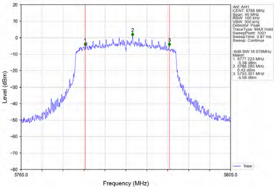
802.11ax(HEW20)_MCH_5785MHz_RU242_Left_Ant1_NTNV
