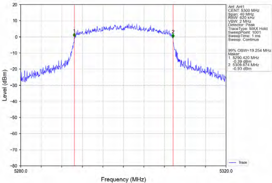
802.11ax(HEW20)_MCH_5300MHz_RU242_Left_Ant1_NTNV
