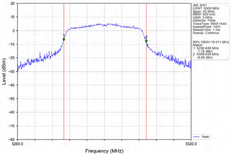
802.11n(HT20)_MCH_5300MHz_Ant1_NTNV
