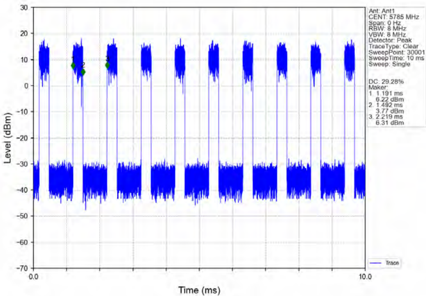
802.11ax(HEW20)_MCH_5785MHz_RU242_Left_Ant1_NTNV
