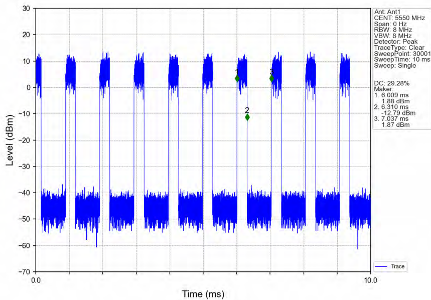
802.11ax(HEW40)_MCH_5550MHz_RU484_Left_Ant1_NTNV
