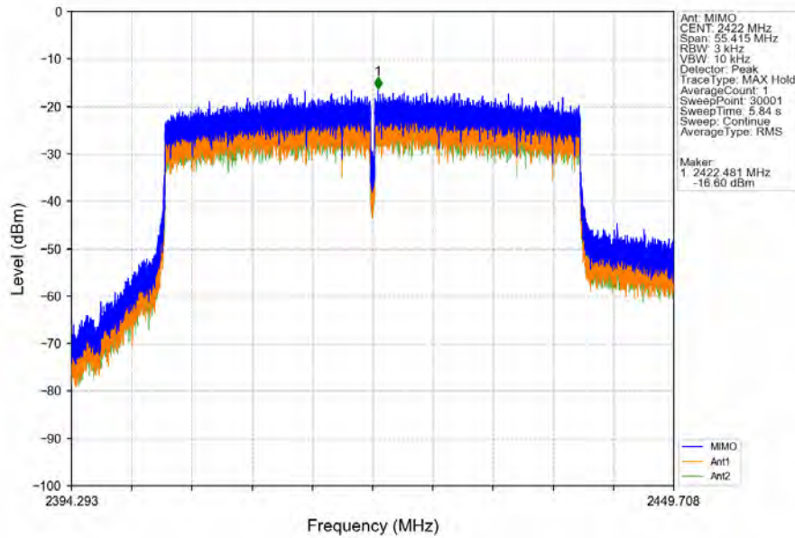
802.11ax(HEW40)_LCH_2422MHz_RU484_Left_MIMO_NTNV
