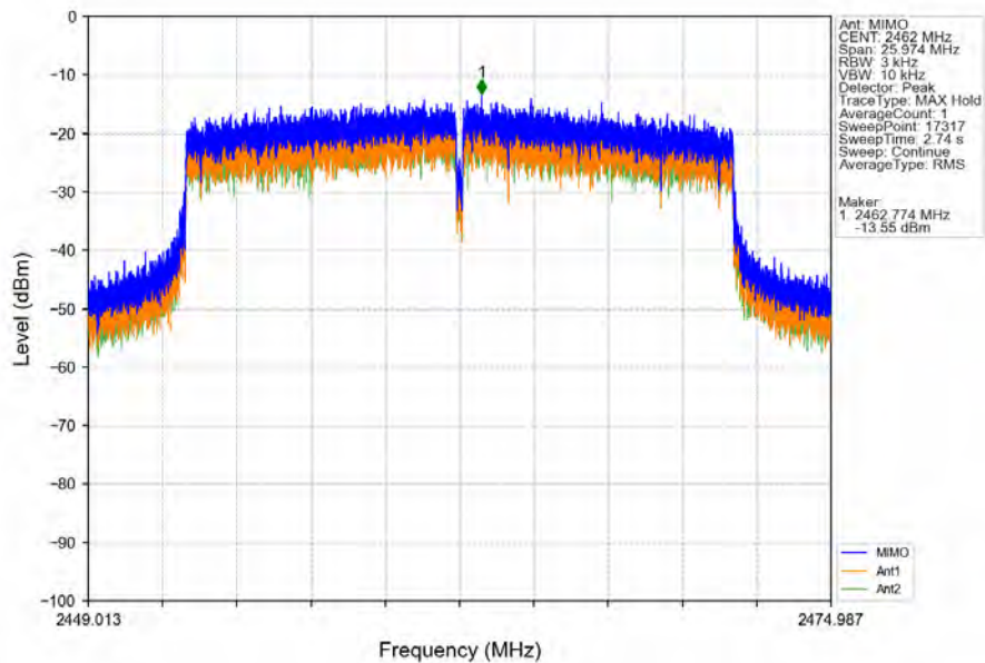
802.11ax(HEW20)_HCH_2462MHz_RU242_Left_MIMO_NTNV
