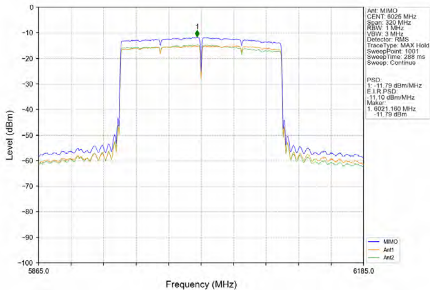
802.11ax(HEW160)_LCH_6025MHz_2xRU996_Left_MIMO_NTNV
