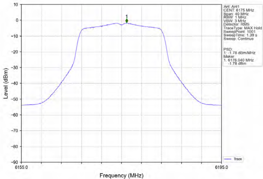
802.11a_MCH_6175MHz_Ant1_NTNV
