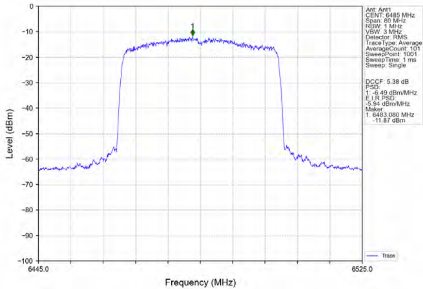
802.11ax(HEW40)_MCH_6485MHz_RU484_Left_Ant1_NTNV
