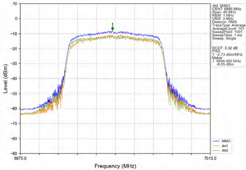
802.11ax(HEW20)_MCH_6995MHz_RU242_Left_MIMO_NTNV
