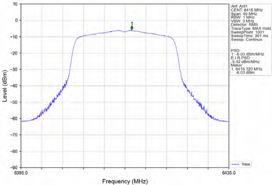
802.11ax(HEW20)_HCH_6415MHz_RU242_Left_Ant1_NTNV
