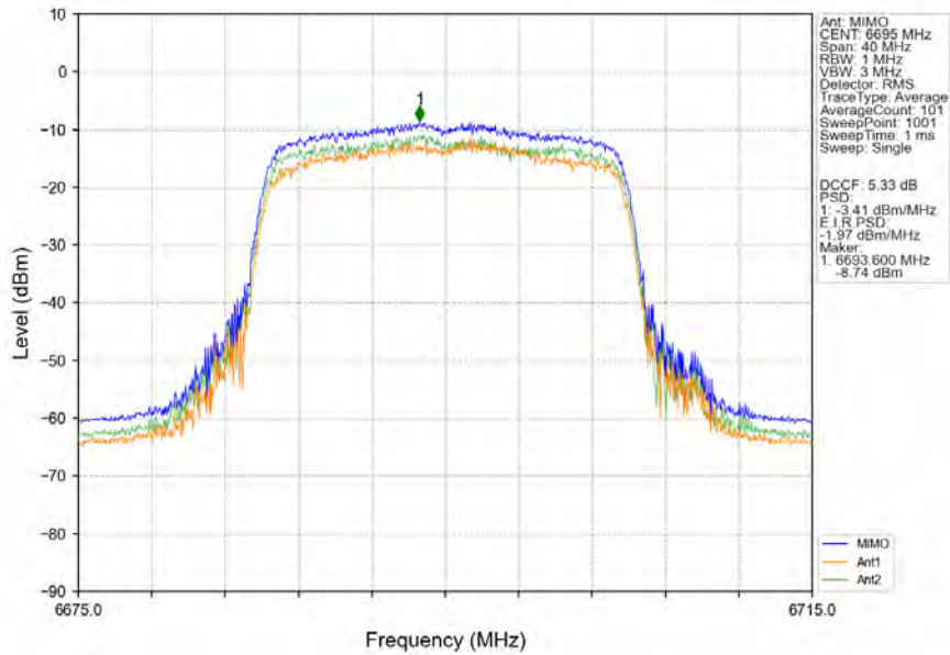
802.11ax(HEW20)_MCH_6695MHz_RU242_Left_MIMO_NTNV
