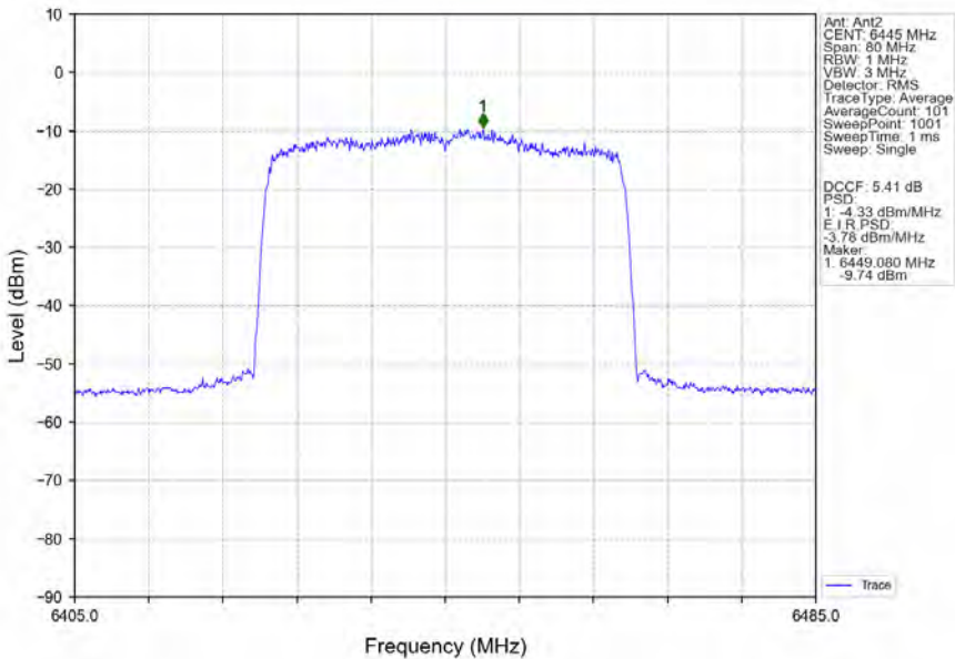
802.11ax(HEW40)_LCH_6445MHz_RU484_Left_Ant2_NTNV
