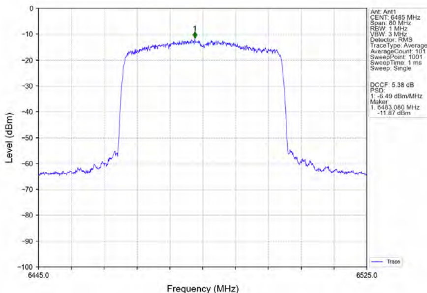
802.11ax(HEW40)_MCH_6485MHz_RU484_Left_Ant1_NTNV
