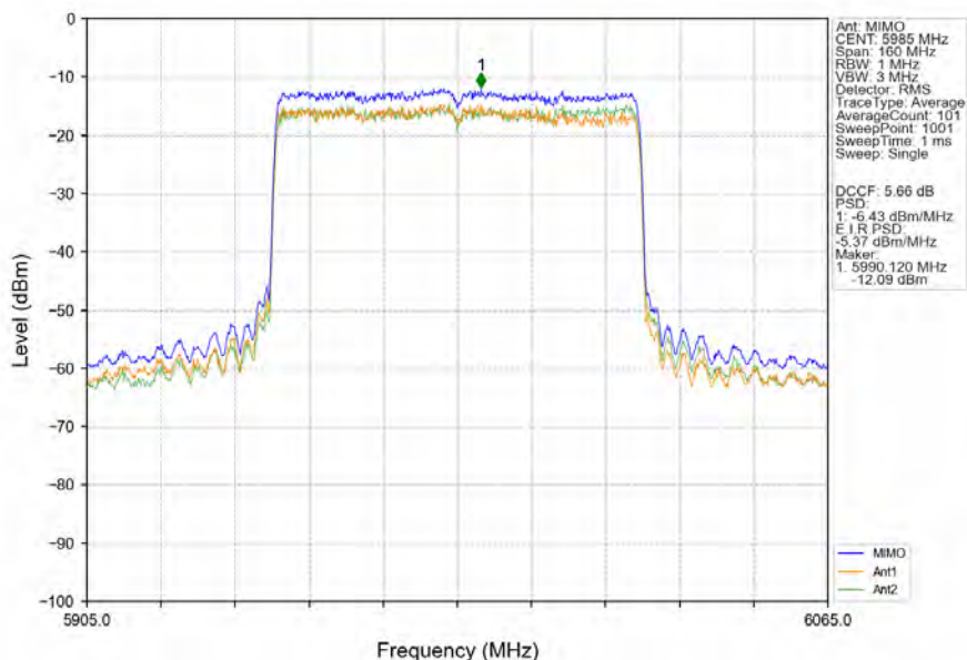
802.11ax(HEW80)_LCH_5985MHz_RU996_Left_MIMO_NTNV
