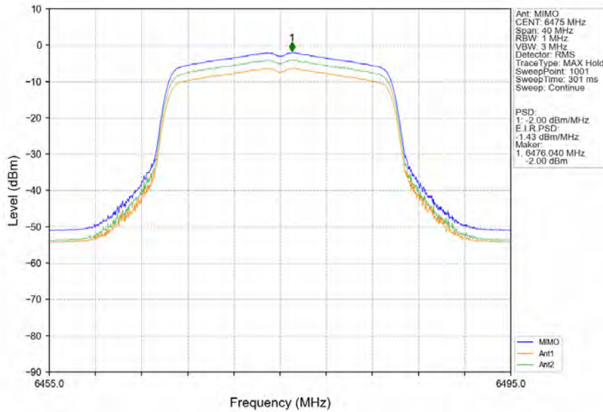
802.11ax(HEW20)_MCH_6475MHz_RU242_Left_MIMO_NTNV
