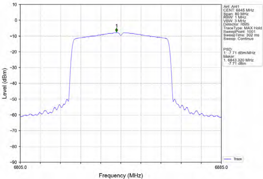
802.11ax(HEW40)_HCH_6845MHz_RU484_Left_Ant1_NTNV
