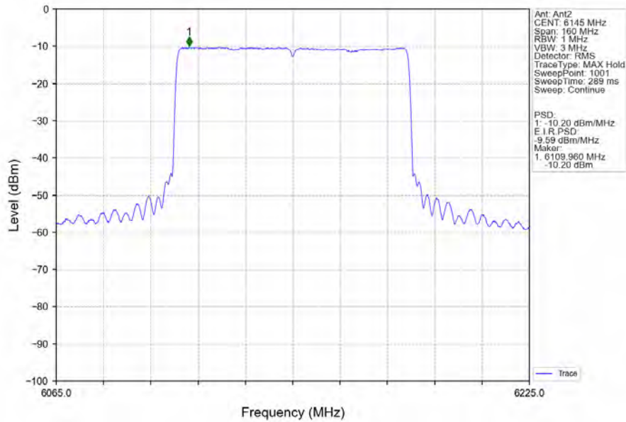
802.11ax(HEW80)_MCH_6145MHz_RU996_Left_Ant2_NTNV
