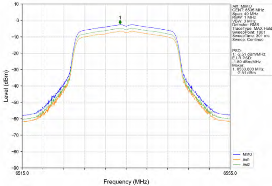
802.11ax(HEW20)_LCH_6535MHz_RU242_Left_MIMO_NTNV
