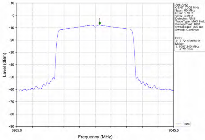
802.11ax(HEW40)_MCH_7005MHz_RU484_Left_Ant2_NTNV
