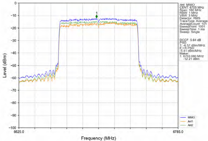
802.11ax(HEW80)_MCH_6705MHz_RU996_Left_MIMO_NTNV
