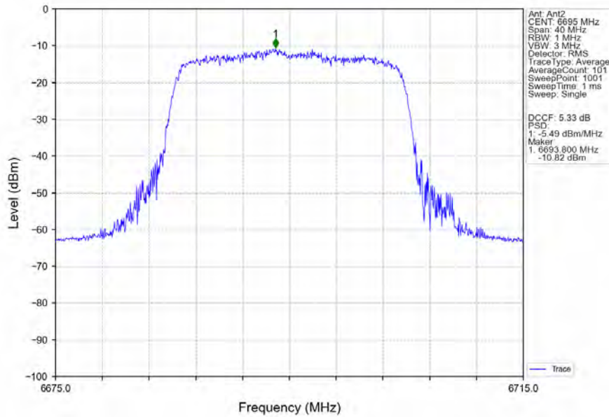
802.11ax(HEW20)_MCH_6695MHz_RU242_Left_Ant2_NTNV
