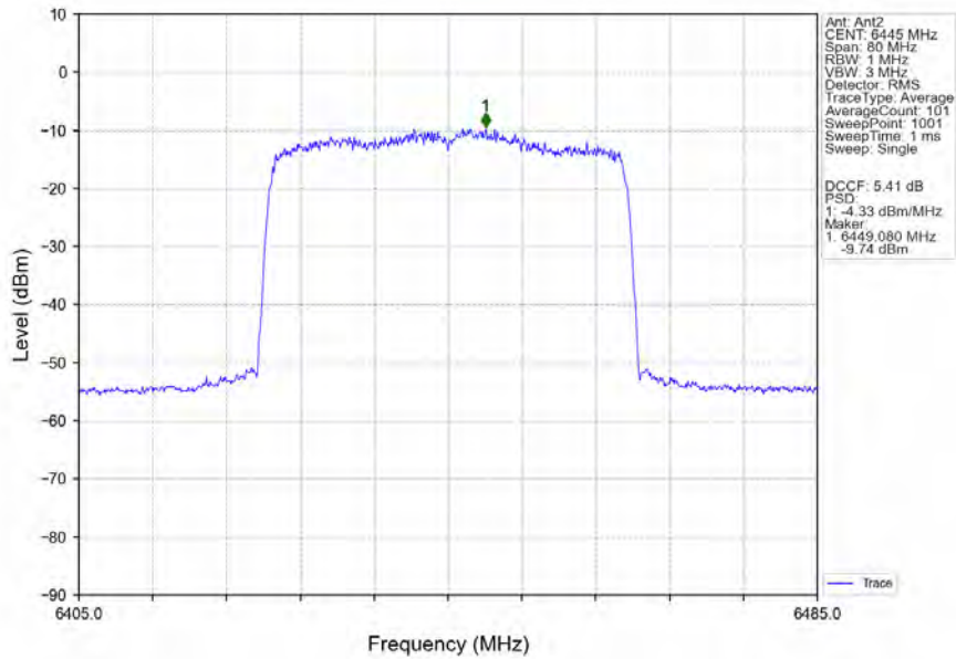
802.11ax(HEW40)_LCH_6445MHz_RU484_Left_Ant2_NTNV
