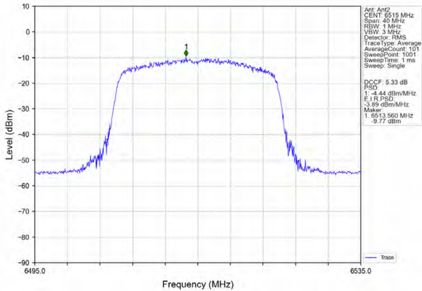
802.11ax(HEW20)_HCH_6515MHz_RU242_Left_Ant2_NTNV
