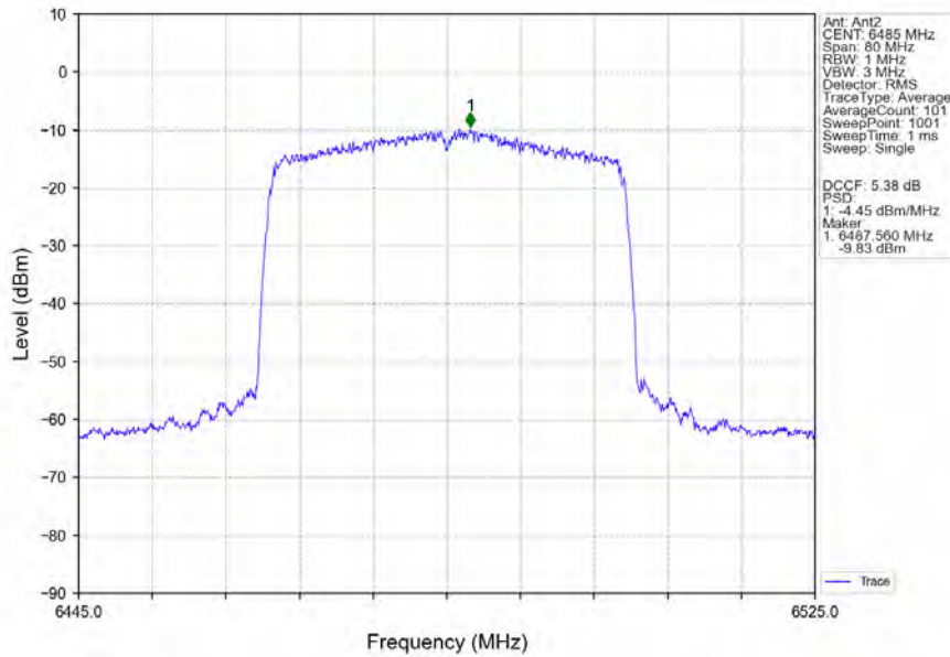
802.11ax(HEW40)_MCH_6485MHz_RU484_Left_Ant2_NTNV
