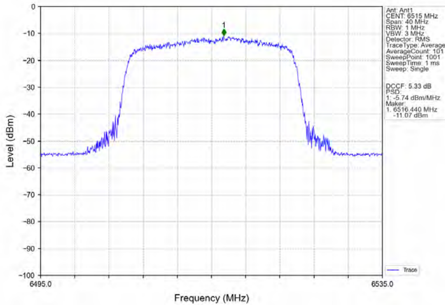
802.11ax(HEW20)_HCH_6515MHz_RU242_Left_Ant1_NTNV
