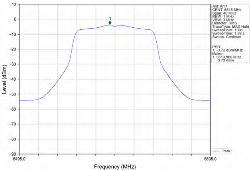
802.11a_HCH_6515MHz_Ant1_NTNV
