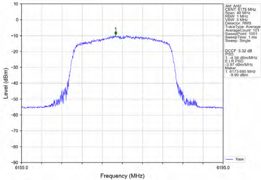
802.11ax(HEW20)_MCH_6175MHz_RU242_Left_Ant2_NTNV
