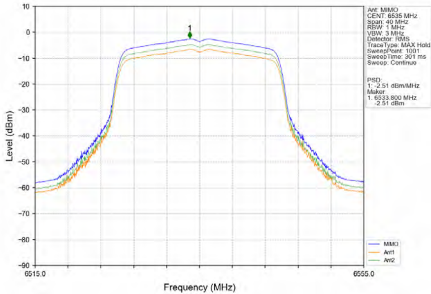
802.11ax(HEW20)_LCH_6535MHz_RU242_Left_MIMO_NTNV
