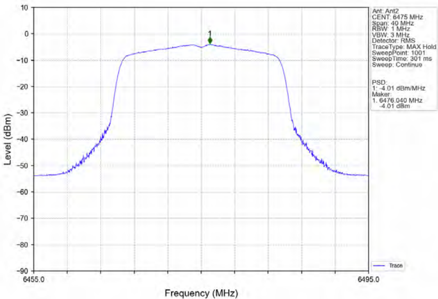
802.11ax(HEW20)_MCH_6475MHz_RU242_Left_Ant2_NTNV
