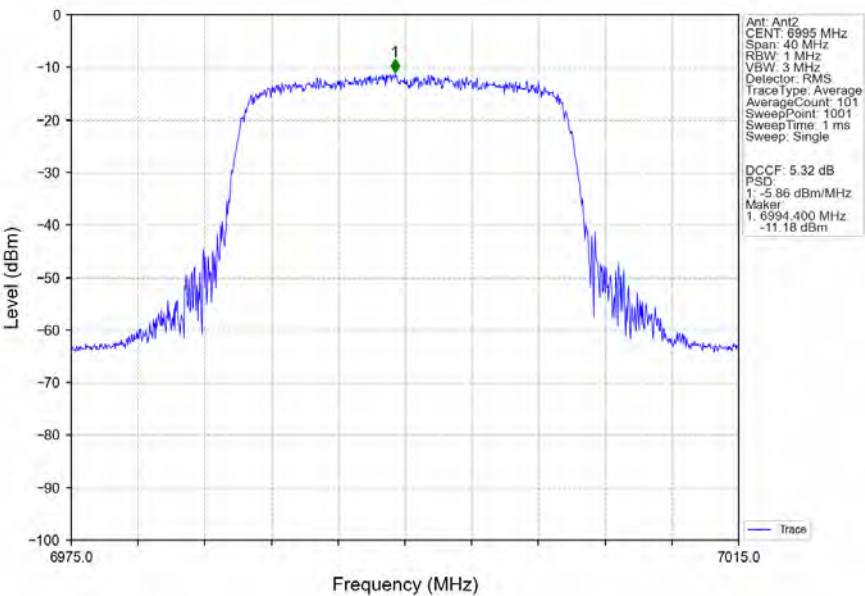
802.11ax(HEW20)_MCH_6995MHz_RU242_Left_Ant2_NTNV
