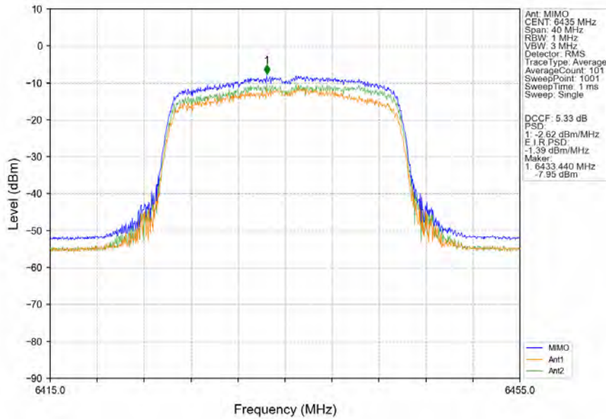
802.11ax(HEW20)_LCH_6435MHz_RU242_Left_MIMO_NTNV
