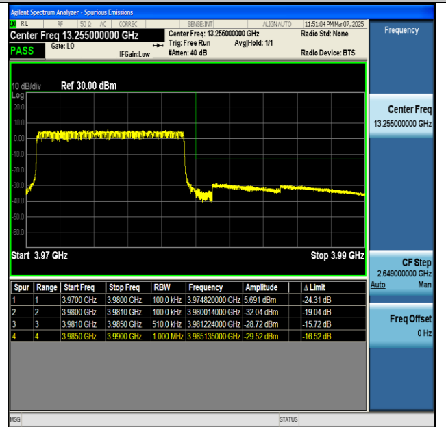
NNTV-n77(3700-3980)-PC2-30-10-H-CP-QPSK- Outer_Full-PASS
