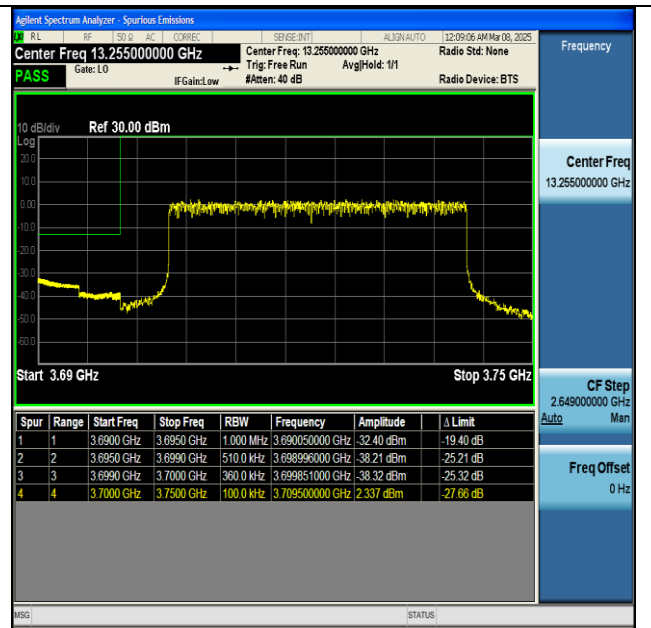
NTNV-n77(3700-3980)-PC2-30-50-L-DFT-BPSK- Outer_Full-PASS
