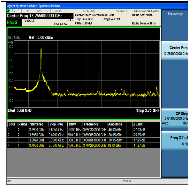
NTNV-n77(3700-3980)-PC2-30-50-L-DFT-BPSK- Edge_1RB_Left-PASS
