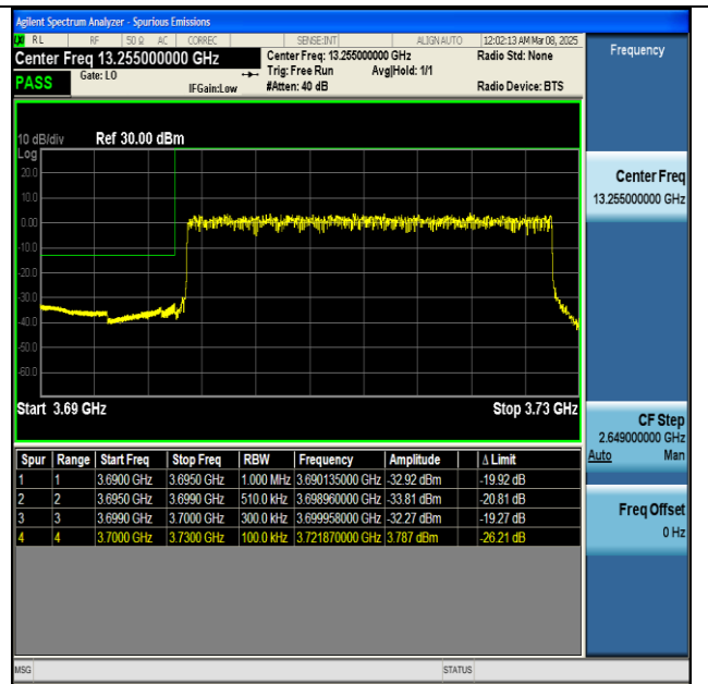
NTNV-n77(3700-3980)-PC2-30-30-L-DFT-BPSK- Outer_Full-PASS
