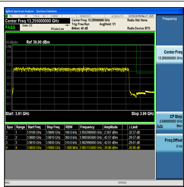
NTNV-n77(3700-3980)-PC2-30-70-H-DFT-BPSK- Outer_Full-PASS
