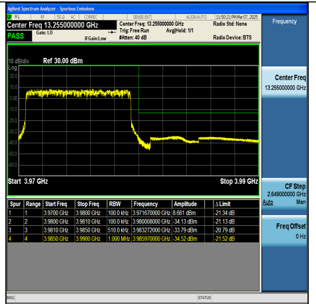
NNTV-n77(3700-3980)-PC2-30-10-H-DFT-BPSK- Outer_Full-PASS
