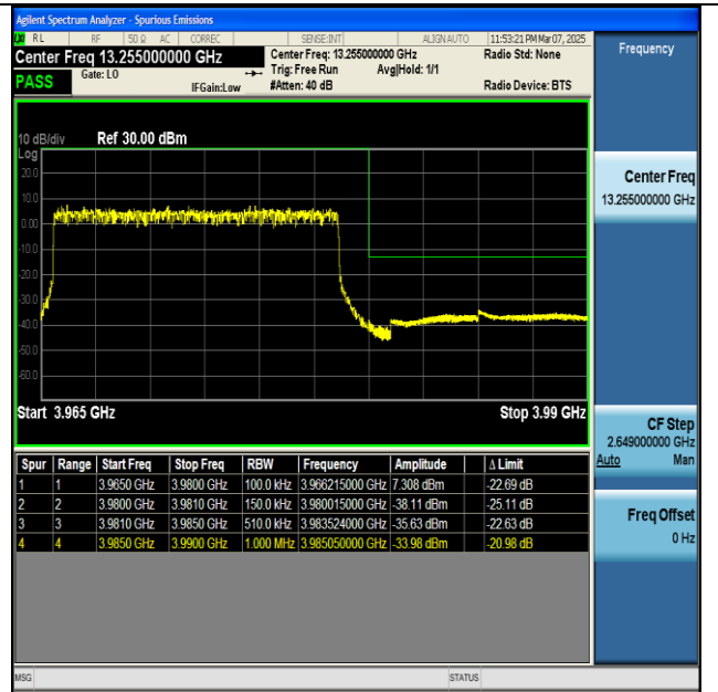
NTVN-n77(3700-3980)-PC2-30-15-H-DFT-BPSK- Outer_Full-PASS
