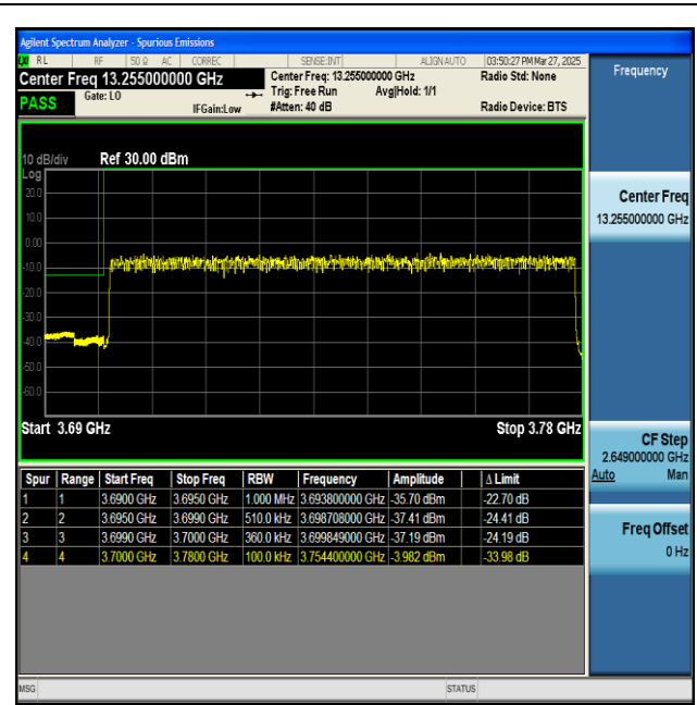
NTNV-n77(3700-3980)-PC2-30-80-L-DFT-BPSK- Outer_Full-PASS
