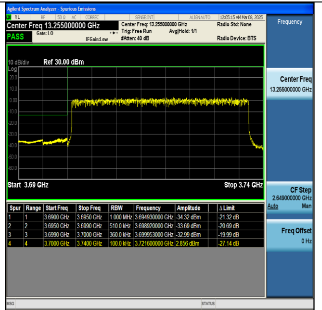
NTNV-n77(3700-3980)-PC2-30-40-L-DFT-BPSK- Outer_Full-PASS
