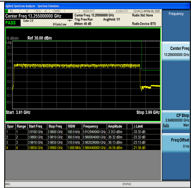
NTNV-n77(3700-3980)-PC2-30-70-H-CP-QPSK- Outer_Full-PASS
