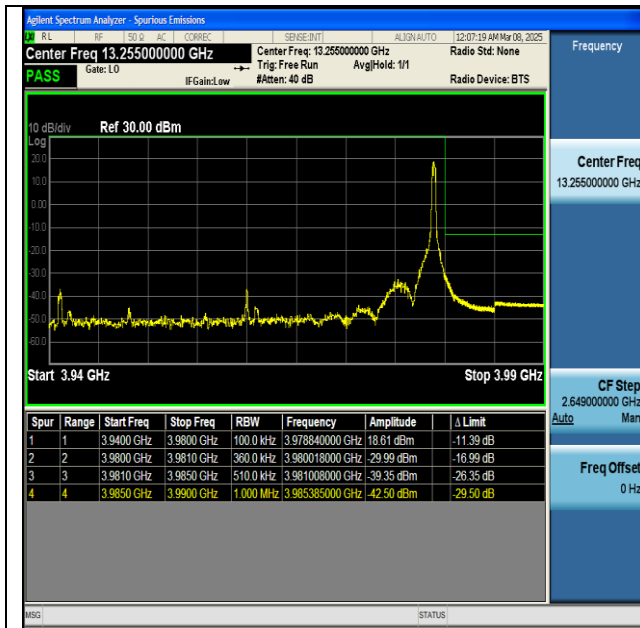
NNTV-n77(3700-3980)-PC2-30-40-H-DFT-BPSK- Edge_1RB_Right-PASS
