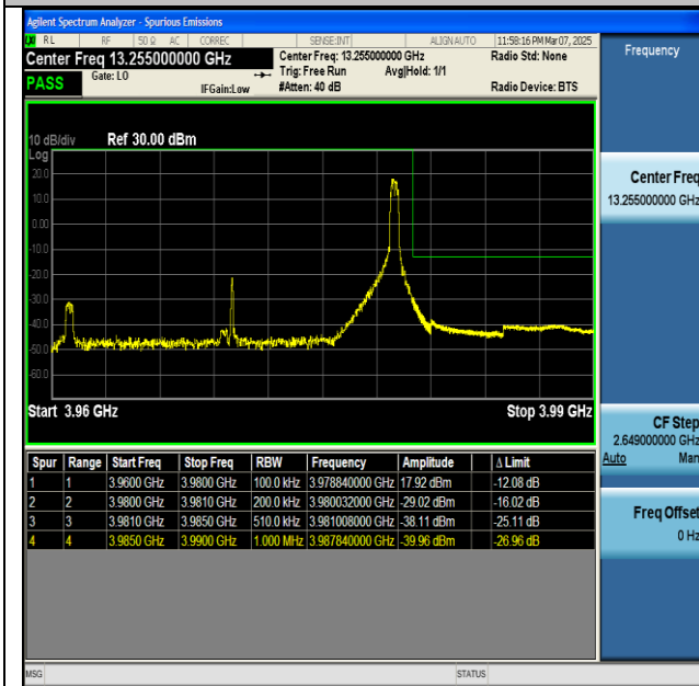
NNTV-n77(3700-3980)-PC2-30-20-H-CP-QPSK- Edge_1RB_Right-PASS
