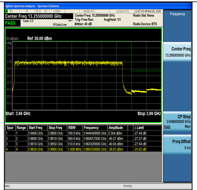
NNTV-n77(3700-3980)-PC2-30-40-H-DFT-BPSK- Outer_Full-PASS
