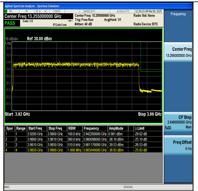
NTVN-n77(3700-3980)-PC2-30-60-H-DFT-BPSK- Outer_Full-PASS
