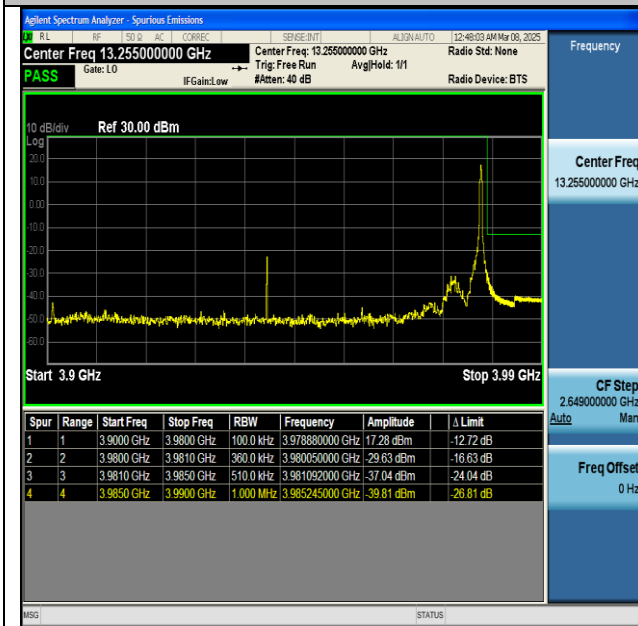
NTVN-n77(3700-3980)-PC2-30-80-H-CP-QPSK- Edge_1RB_Right-PASS
