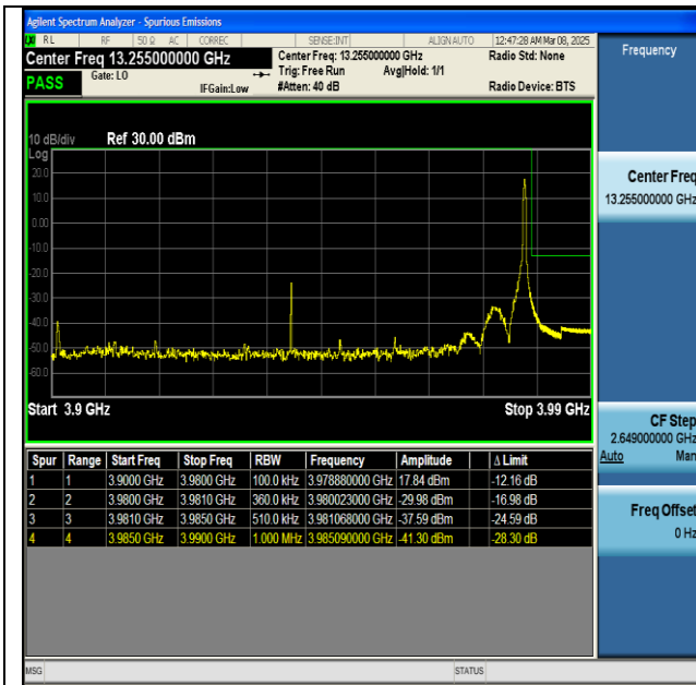
NTVN-n77(3700-3980)-PC2-30-80-H-DFT-BPSK- Edge_1RB_Right-PASS
