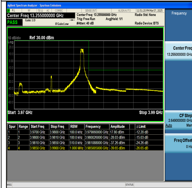
NNTV-n77(3700-3980)-PC2-30-10-H-CP-QPSK- Edge_1RB_Right-PASS
