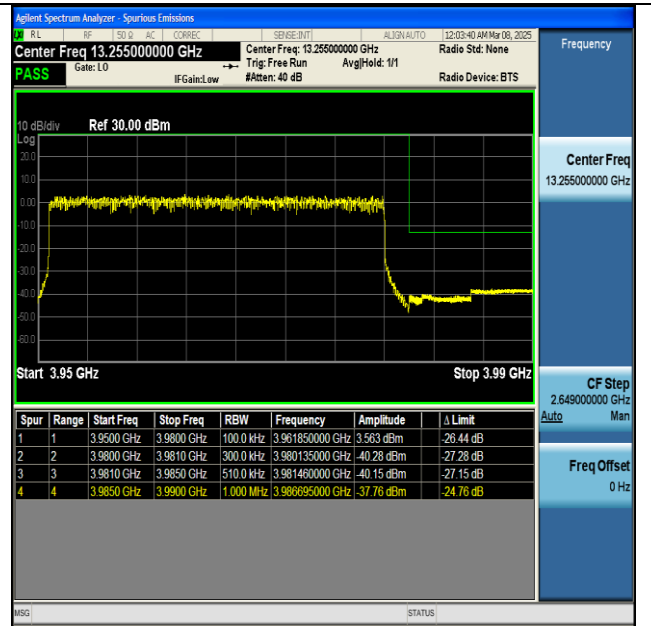
NNTV-n77(3700-3980)-PC2-30-30-H-DFT-BPSK- Outer_Full-PASS
