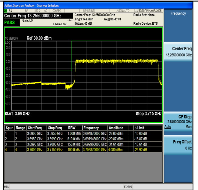
NTVN-n77(3700-3980)-PC2-30-15-L-CP-QPSK- Outer_Full-PASS
