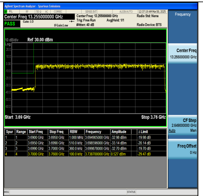
NTVN-n77(3700-3980)-PC2-30-60-L-DFT-BPSK- Outer_Full-PASS
