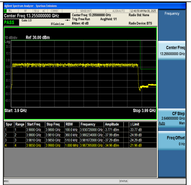
NTVN-n77(3700-3980)-PC2-30-80-H-DFT-BPSK- Outer_Full-PASS
