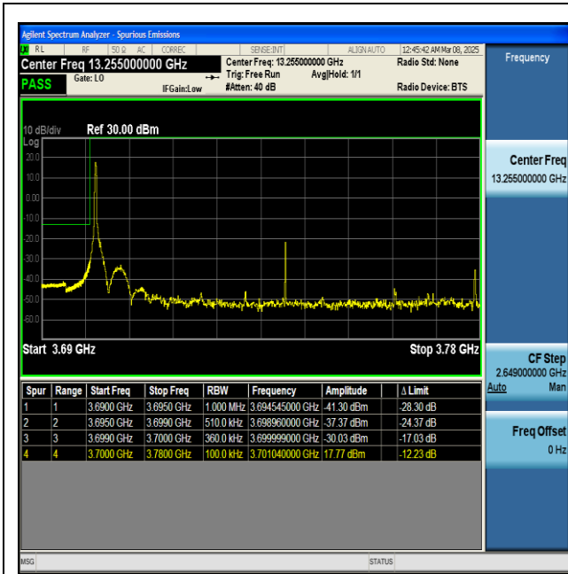
NTNV-n77(3700-3980)-PC2-30-80-L-DFT-BPSK- Edge_1RB_Left-PASS
