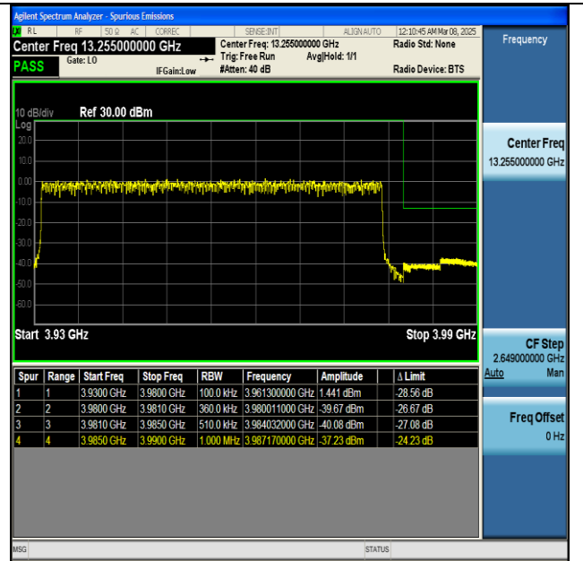
NTNV-n77(3700-3980)-PC2-30-50-H-DFT-BPSK- Outer_Full-PASS
