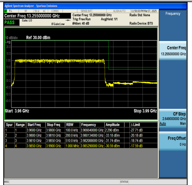
NNTV-n77(3700-3980)-PC2-30-20-H-CP-QPSK- Outer_Full-PASS
