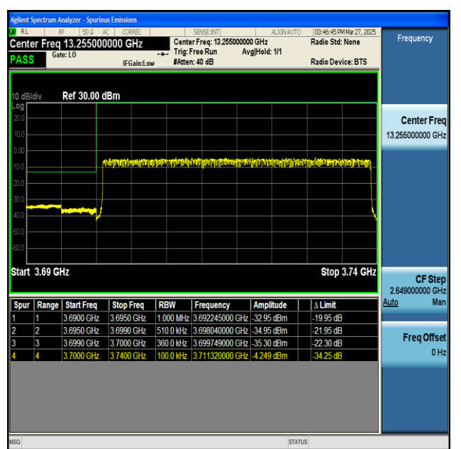
NTNV-n77(3700-3980)-PC2-30-40-L-CP-QPSK- Outer_Full-PASS
