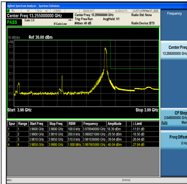
NNTV-n77(3700-3980)-PC2-30-20-H-DFT-BPSK- Edge_1RB_Right-PASS
