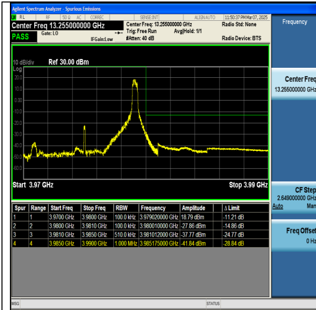
NNTV-n77(3700-3980)-PC2-30-10-H-DFT-BPSK- Edge_1RB_Right-PASS
