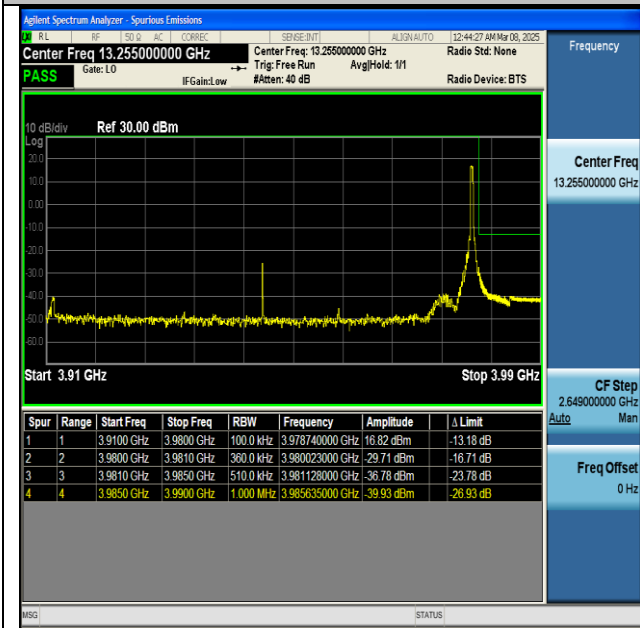
NTNV-n77(3700-3980)-PC2-30-70-H-CP-QPSK- Edge_1RB_Right-PASS
