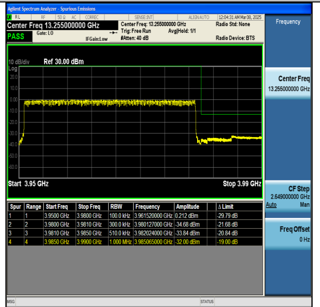
NNTV-n77(3700-3980)-PC2-30-30-H-CP-QPSK- Outer_Full-PASS
