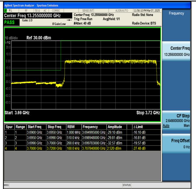
NTNV-n77(3700-3980)-PC2-30-20-L-CP-QPSK- Outer_Full-PASS
