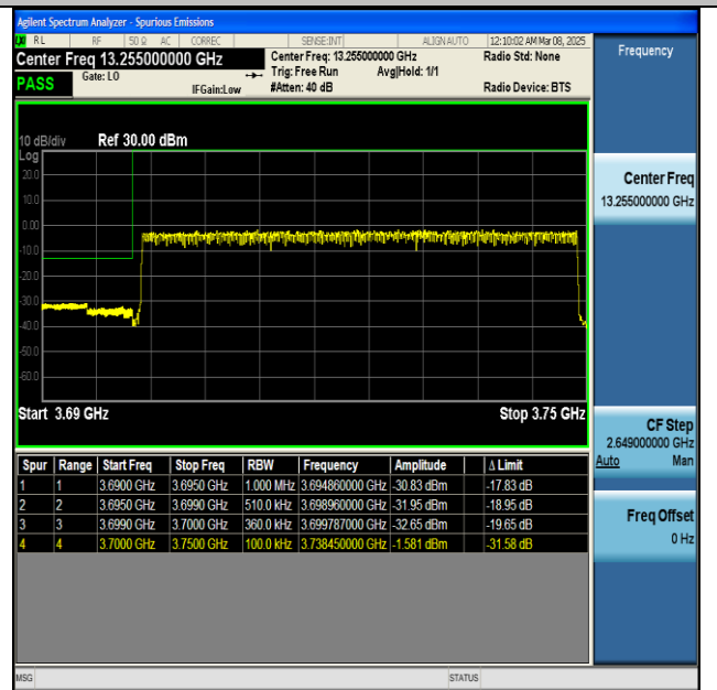
NTNV-n77(3700-3980)-PC2-30-50-L-CP-QPSK- Outer_Full-PASS
