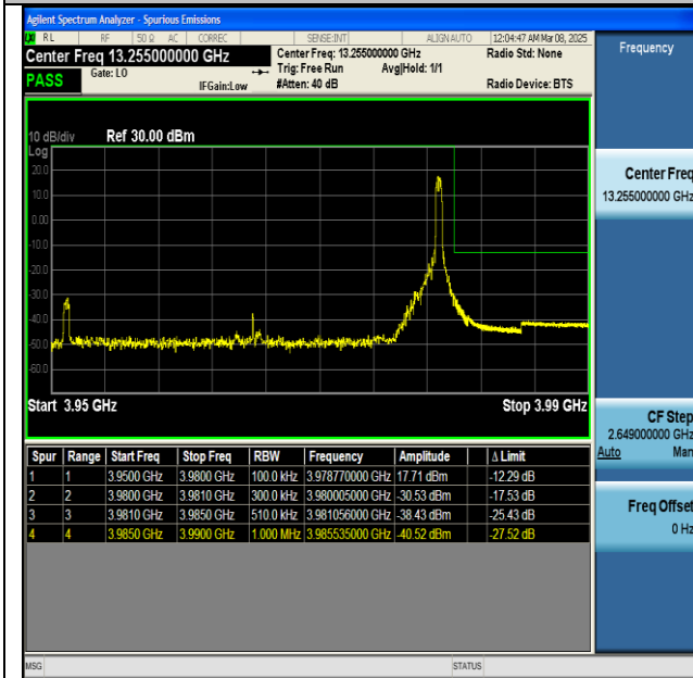
NNTV-n77(3700-3980)-PC2-30-30-H-CP-QPSK- Edge_1RB_Right-PASS
