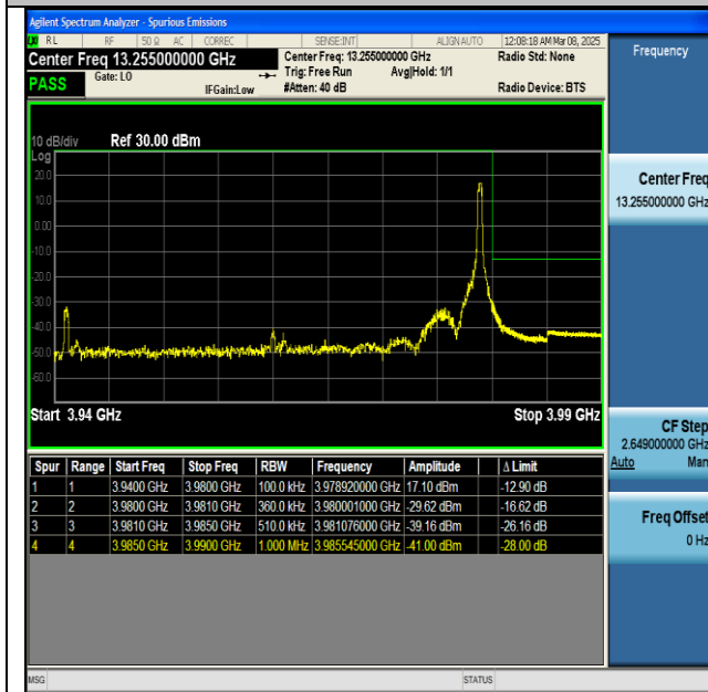
NNTV-n77(3700-3980)-PC2-30-40-H-CP-QPSK- Edge_1RB_Right-PASS
