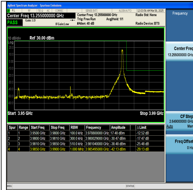
NNTV-n77(3700-3980)-PC2-30-30-H-DFT-BPSK- Edge_1RB_Right-PASS
