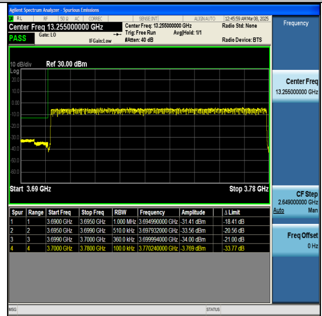
NTNV-n77(3700-3980)-PC2-30-80-L-CP-QPSK- Outer_Full-PASS
