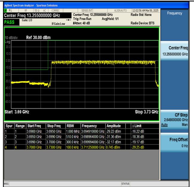
NTNV-n77(3700-3980)-PC2-30-30-L-CP-QPSK- Outer_Full-PASS
