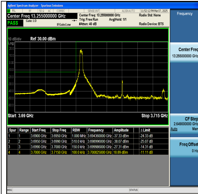
NTVN-n77(3700-3980)-PC2-30-15-L-DFT-BPSK- Edge_1RB_Left-PASS
