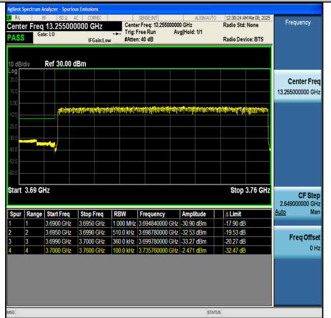
NTVN-n77(3700-3980)-PC2-30-60-L-CP-QPSK- Outer_Full-PASS
