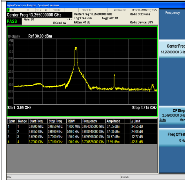
NTVN-n77(3700-3980)-PC2-30-15-L-CP-QPSK- Edge_1RB_Left-PASS
