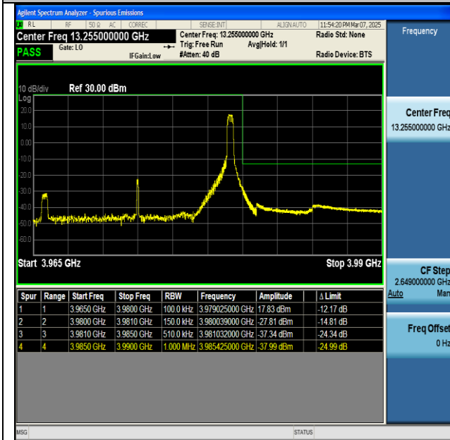
NTVN-n77(3700-3980)-PC2-30-15-H-CP-QPSK- Edge_1RB_Right-PASS
