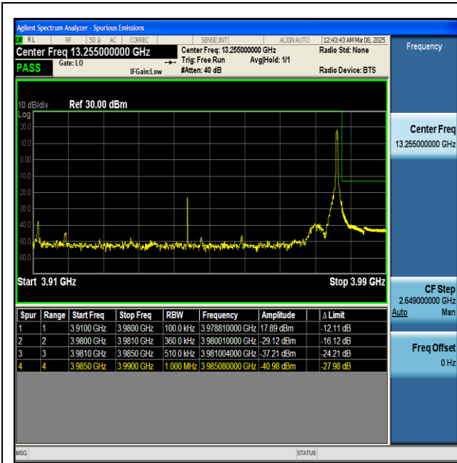
NTNV-n77(3700-3980)-PC2-30-70-H-DFT-BPSK- Edge_1RB_Right-PASS
