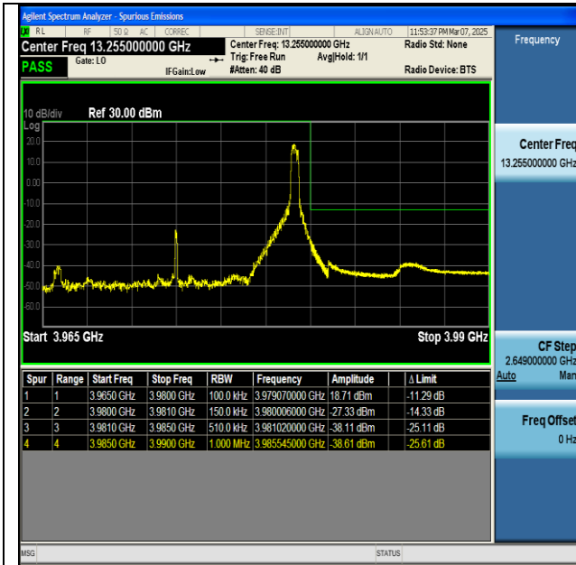
NTVN-n77(3700-3980)-PC2-30-15-H-DFT-BPSK- Edge_1RB_Right-PASS
