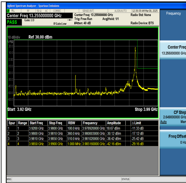
NTVN-n77(3700-3980)-PC2-30-60-H-DFT-BPSK- Edge_1RB_Right-PASS
