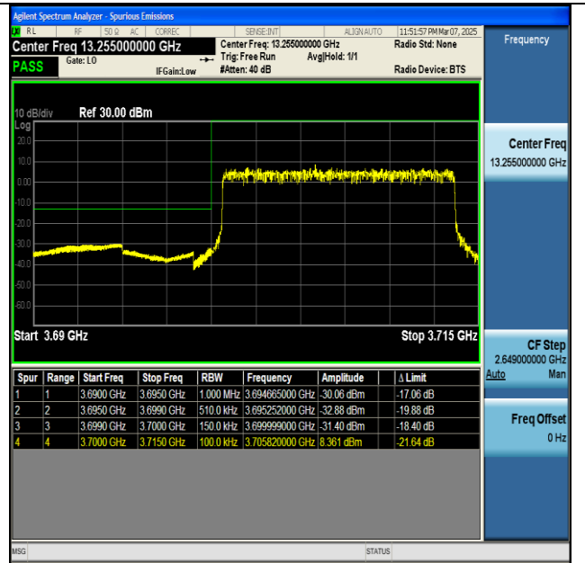
NTVN-n77(3700-3980)-PC2-30-15-L-DFT-BPSK- Outer_Full-PASS
