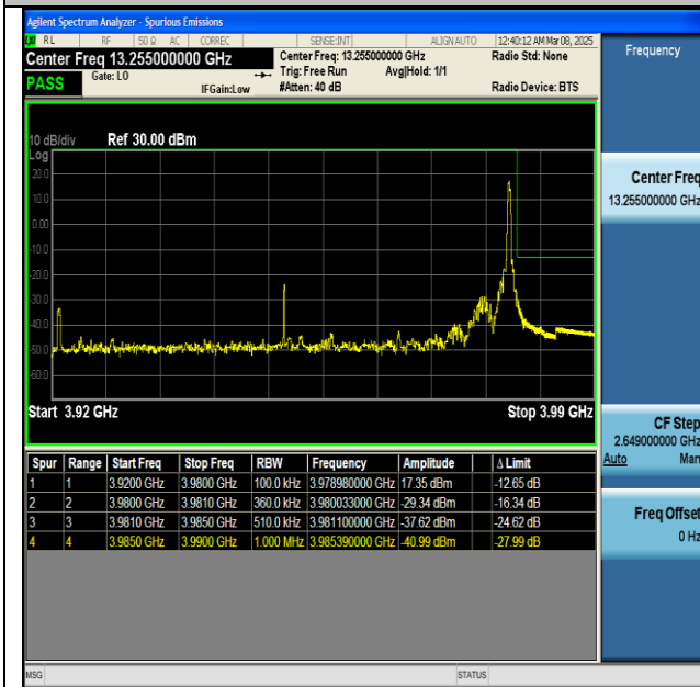
NTVN-n77(3700-3980)-PC2-30-60-H-CP-QPSK- Edge_1RB_Right-PASS
