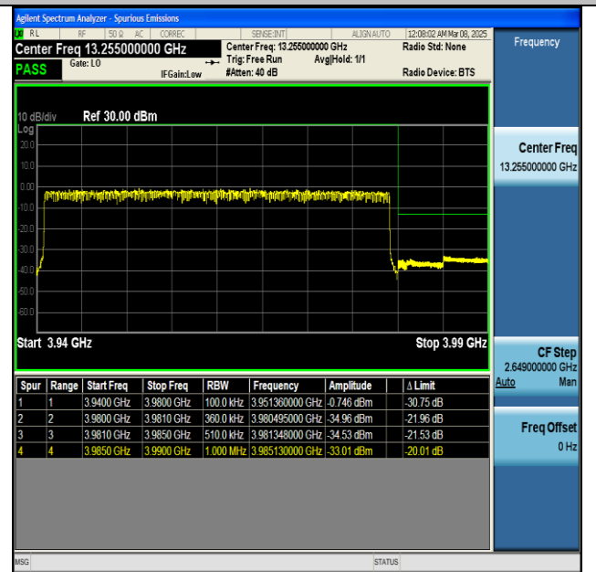
NNTV-n77(3700-3980)-PC2-30-40-H-CP-QPSK- Outer_Full-PASS
