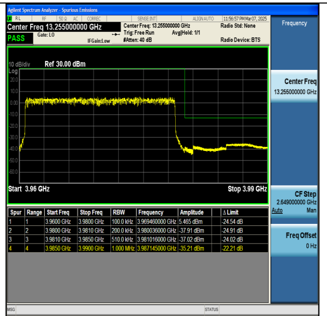
NNTV-n77(3700-3980)-PC2-30-20-H-DFT-BPSK- Outer_Full-PASS
