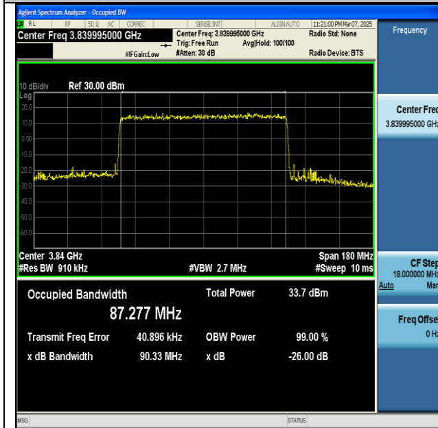
NTNV-n77(3700-3980)-PC2-30-90-M-CP-QPSK- Outer_Full-Ant1-PASS
