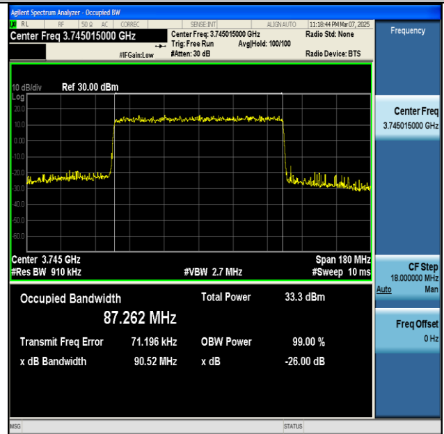
NTVN-n77(3700-3980)-PC2-30-90-L-CP-64QAM- Outer_Full-Ant1-PASS
