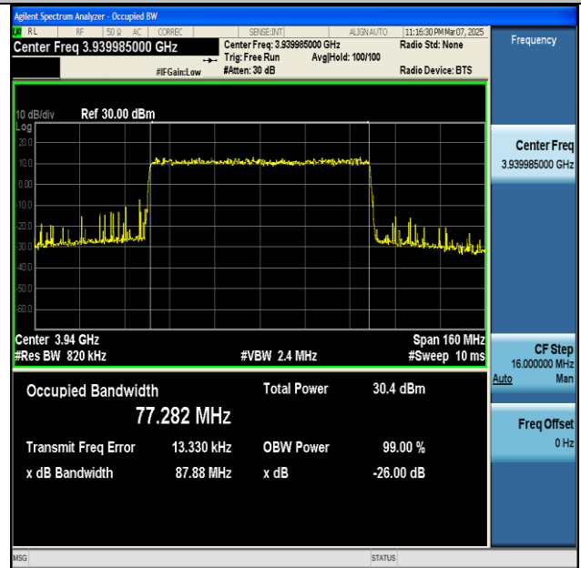
NTNV-n77(3700-3980)-PC2-30-80-H-CP-256QAM-Outer_Full-Ant1-PASS
