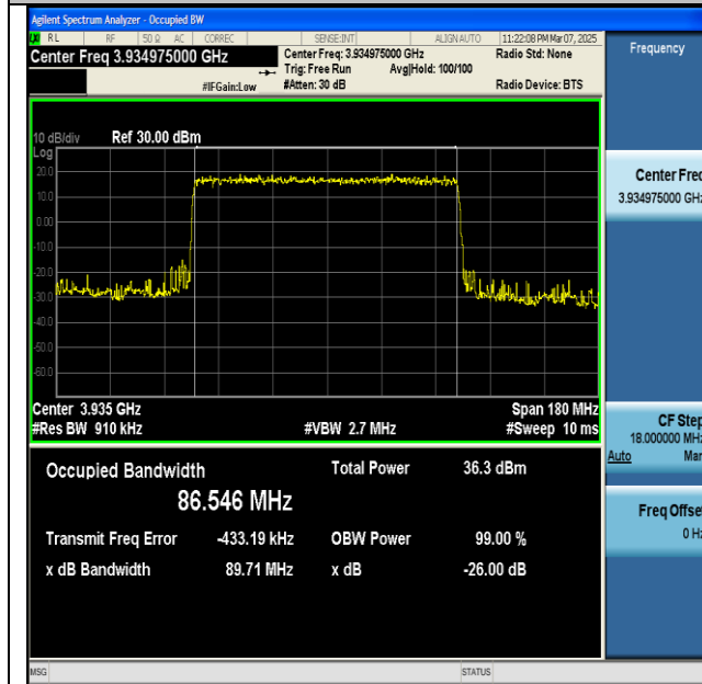
NTNV-n77(3700-3980)-PC2-30-90-H-DFT-BPSK- Outer_Full-Ant1-PASS
