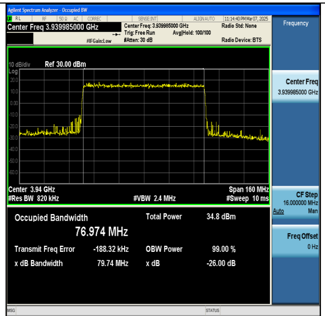
NTNV-n77(3700-3980)-PC2-30-80-H-DFT-16QAM- Outer_Full-Ant1-PASS
