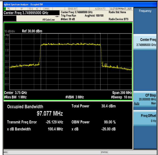
NTNV-n77(3700-3980)-PC2-30-100-L-CP-256QAM- Outer_Full-Ant1-PASS
