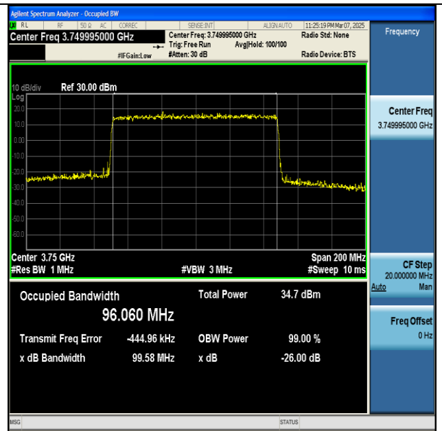
NTNV-n77(3700-3980)-PC2-30-100-L-DFT-16QAM- Outer_Full-Ant1-PASS
