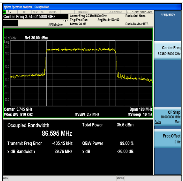
NTNV-n77(3700-3980)-PC2-30-90-L-DFT-QPSK- Outer_Full-Ant1-PASS
