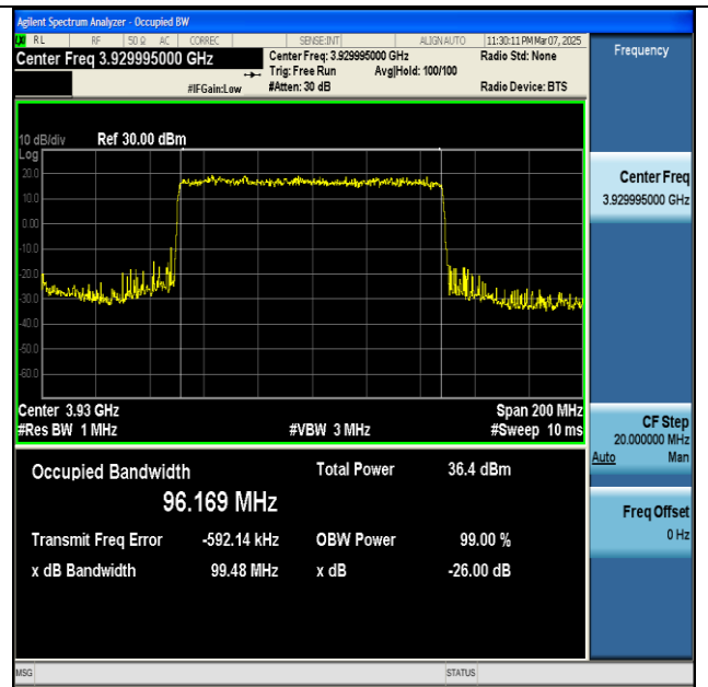
NTNV-n77(3700-3980)-PC2-30-100-H-DFT-BPSK- Outer_Full-Ant1-PASS
