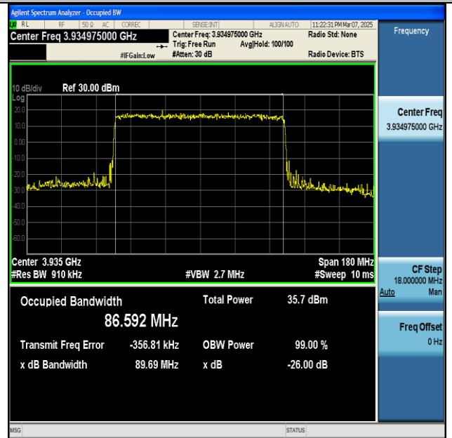
NTNV-n77(3700-3980)-PC2-30-90-H-DFT-QPSK- Outer_Full-Ant1-PASS
