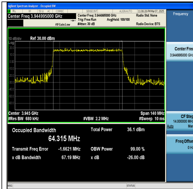
NTNV-n77(3700-3980)-PC2-30-70-H-DFT-BPSK- Outer_Full-Ant1-PASS
