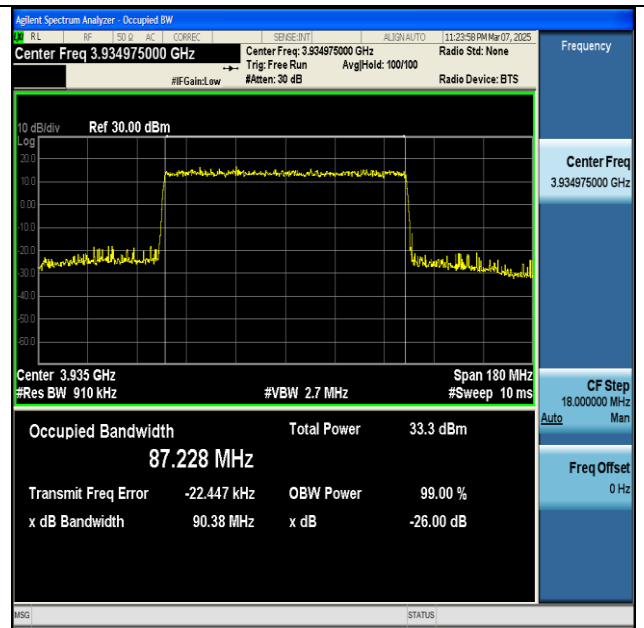
NTNV-n77(3700-3980)-PC2-30-90-H-CP-64QAM- Outer_Full-Ant1-PASS
