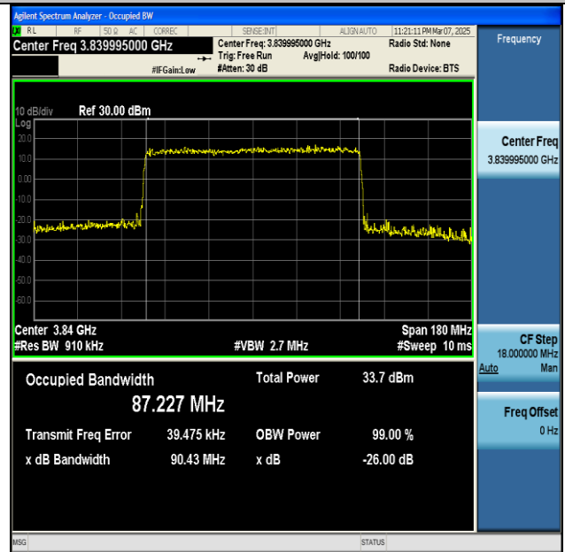
NTNV-n77(3700-3980)-PC2-30-90-M-CP-16QAM- Outer_Full-Ant1-PASS
