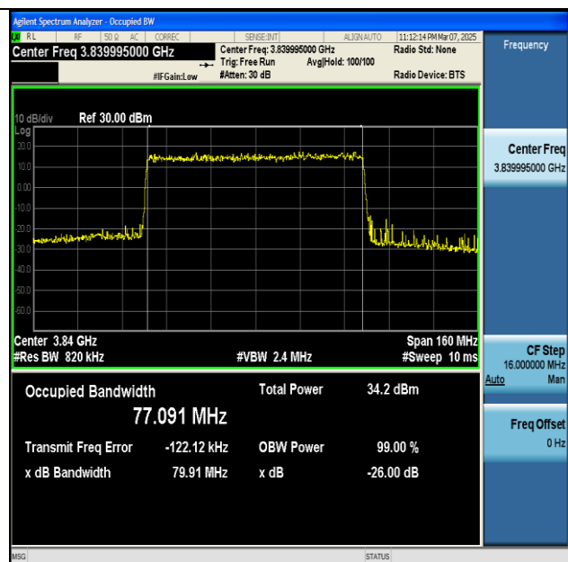
NTNV-n77(3700-3980)-PC2-30-80-M-DFT-64QAM- Outer_Full-Ant1-PASS
