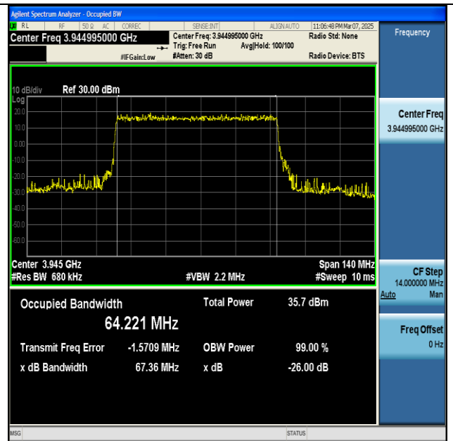
NTNV-n77(3700-3980)-PC2-30-70-H-DFT-QPSK- Outer_Full-Ant1-PASS
