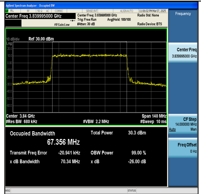
NTNV-n77(3700-3980)-PC2-30-70-M-CP-256QAM- Outer_Full-Ant1-PASS
