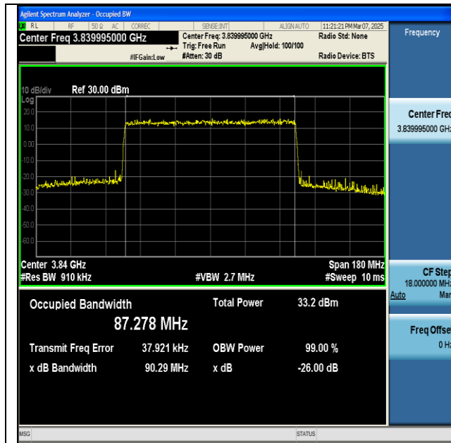
NTNV-n77(3700-3980)-PC2-30-90-M-CP-64QAM- Outer_Full-Ant1-PASS
