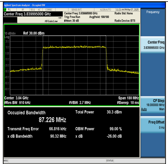
NTNV-n77(3700-3980)-PC2-30-90-M-CP-256QAM- Outer_Full-Ant1-PASS
