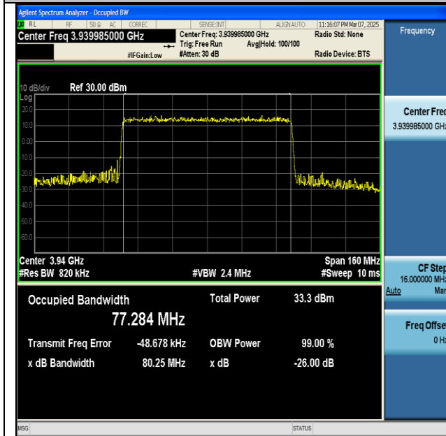
NTNV-n77(3700-3980)-PC2-30-80-H-CP-64QAM-Outer_Full-Ant1-PASS
