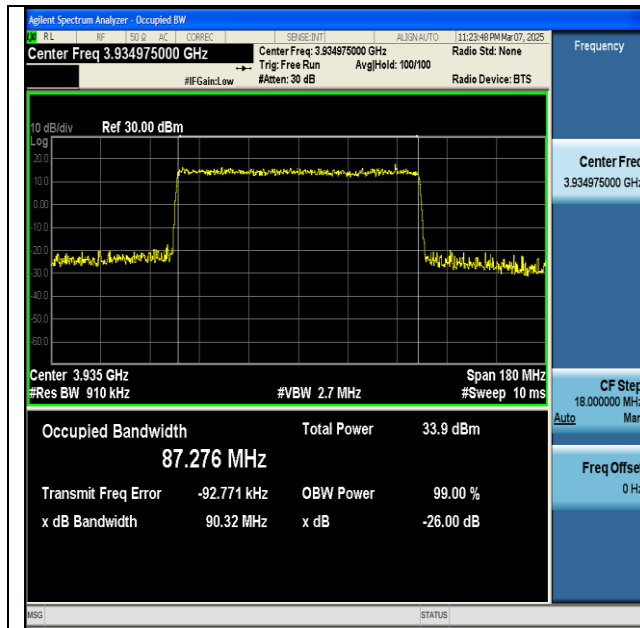
NTNV-n77(3700-3980)-PC2-30-90-H-CP-16QAM- Outer_Full-Ant1-PASS
