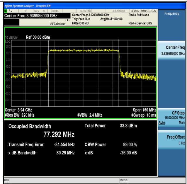
NTNV-n77(3700-3980)-PC2-30-80-H-CP-16QAM-Outer_Full-Ant1-PASS
