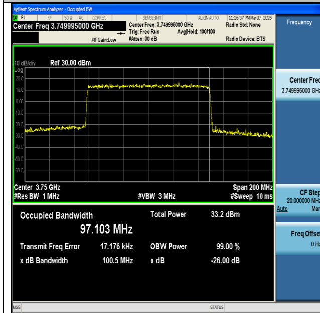
NTNV-n77(3700-3980)-PC2-30-100-L-CP-64QAM- Outer_Full-Ant1-PASS
