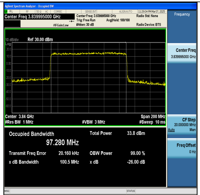
NTNV-n77(3700-3980)-PC2-30-100-M-CP-QPSK-Outer_Full-Ant1-PASS
