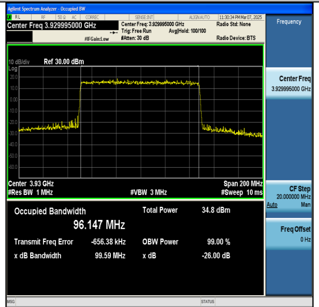
NTNV-n77(3700-3980)-PC2-30-100-H-DFT-16QAM- Outer_Full-Ant1-PASS
