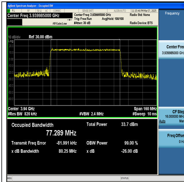
NTNV-n77(3700-3980)-PC2-30-80-H-CP-QPSK-Outer_Full-Ant1-PASS
