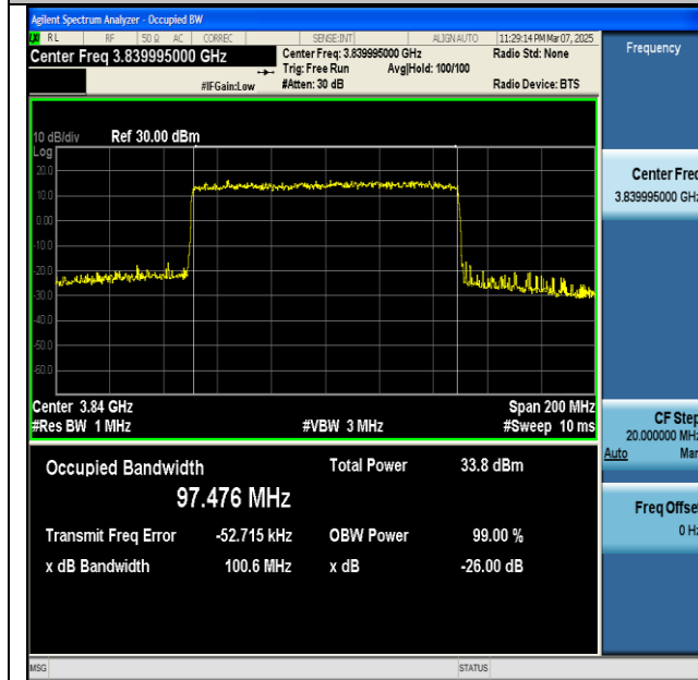
NTNV-n77(3700-3980)-PC2-30-100-M-CP-16QAM-Outer_Full-Ant1-PASS
