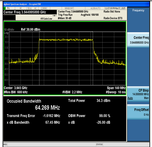
NTNV-n77(3700-3980)-PC2-30-70-H-DFT-64QAM- Outer_Full-Ant1-PASS
