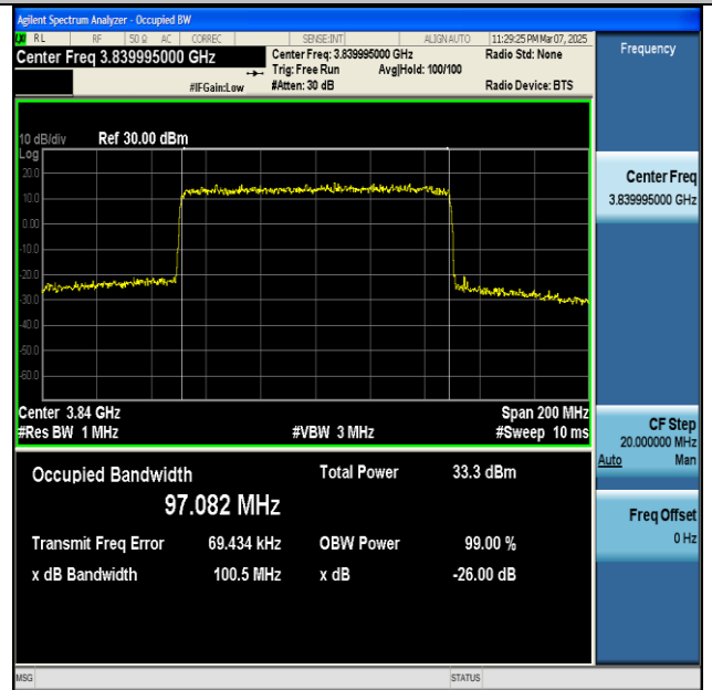
NTNV-n77(3700-3980)-PC2-30-100-M-CP-64QAM-Outer_Full-Ant1-PASS
