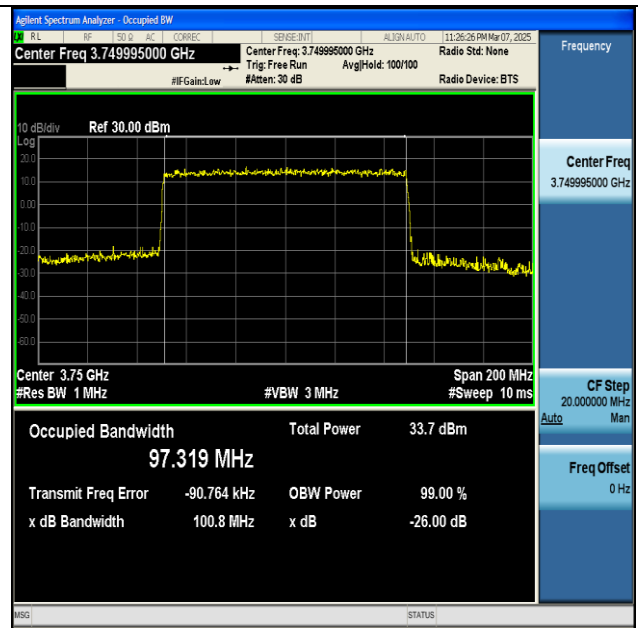
NTNV-n77(3700-3980)-PC2-30-100-L-CP-16QAM- Outer_Full-Ant1-PASS
