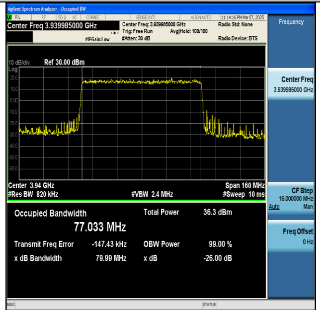
NTNV-n77(3700-3980)-PC2-30-80-H-DFT-BPSK- Outer_Full-Ant1-PASS
