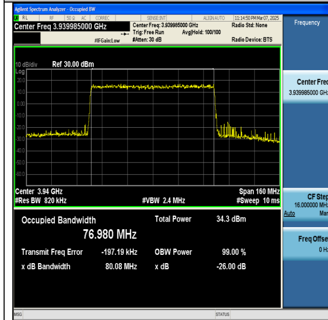
NTNV-n77(3700-3980)-PC2-30-80-H-DFT-64QAM- Outer_Full-Ant1-PASS
