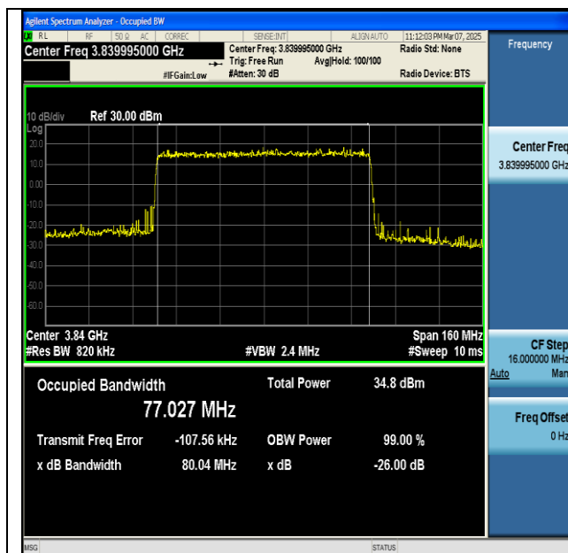
NTNV-n77(3700-3980)-PC2-30-80-M-DFT-16QAM- Outer_Full-Ant1-PASS
