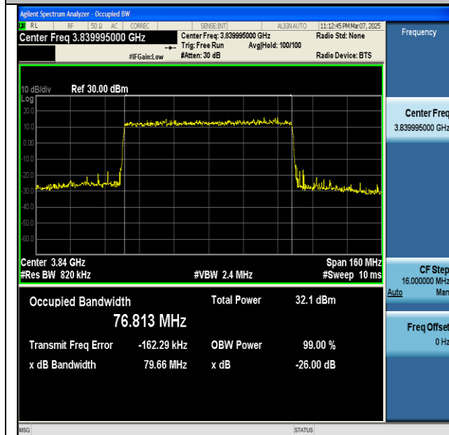
NTNV-n77(3700-3980)-PC2-30-80-M-DFT-256QAM- Outer_Full-Ant1-PASS
