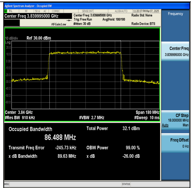
NTNV-n77(3700-3980)-PC2-30-90-M-DFT-256QAM- Outer_Full-Ant1-PASS
