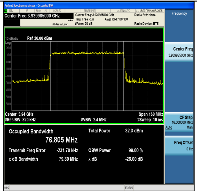
NTNV-n77(3700-3980)-PC2-30-80-H-DFT-256QAM- Outer_Full-Ant1-PASS
