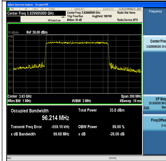
NTNV-n77(3700-3980)-PC2-30-100-H-DFT-QPSK- Outer_Full-Ant1-PASS
