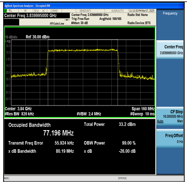
NTNV-n77(3700-3980)-PC2-30-80-M-CP-64QAM- Outer_Full-Ant1-PASS
