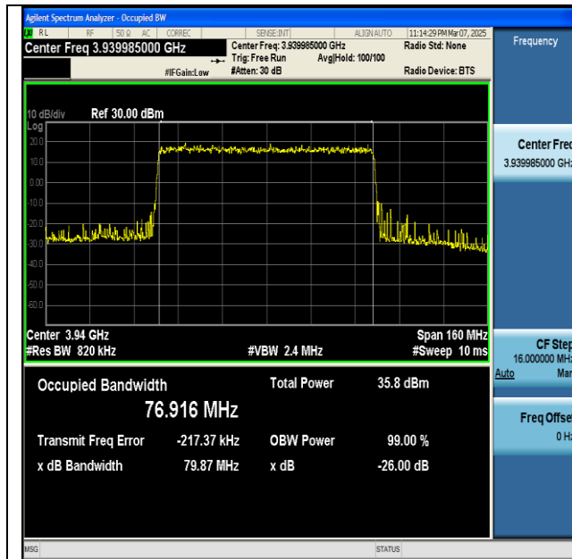
NTNV-n77(3700-3980)-PC2-30-80-H-DFT-QPSK- Outer_Full-Ant1-PASS
