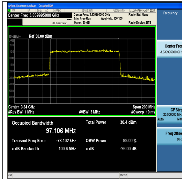
NTNV-n77(3700-3980)-PC2-30-100-M-CP-256QAM- Outer_Full-Ant1-PASS
