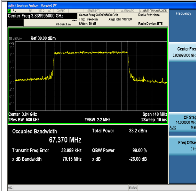
NTNV-n77(3700-3980)-PC2-30-70-M-CP-64QAM- Outer_Full-Ant1-PASS
