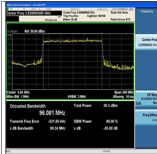
NTNV-n77(3700-3980)-PC2-30-100-M-DFT-BPSK- Outer_Full-Ant1-PASS
