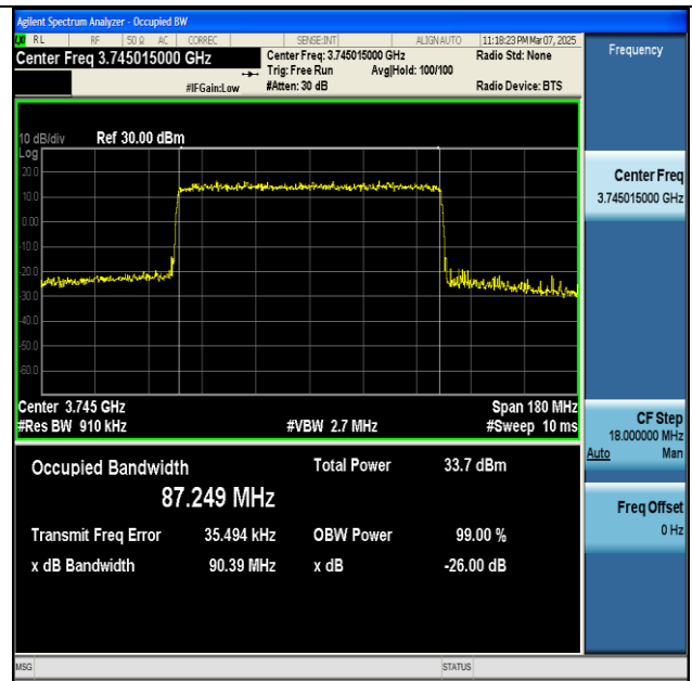
NTVN-n77(3700-3980)-PC2-30-90-L-CP-QPSK- Outer_Full-Ant1-PASS
