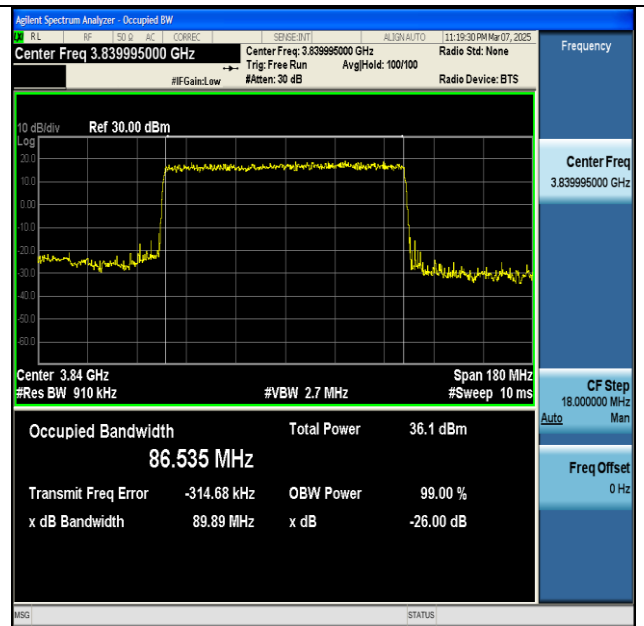
NTNV-n77(3700-3980)-PC2-30-90-M-DFT-BPSK- Outer_Full-Ant1-PASS
