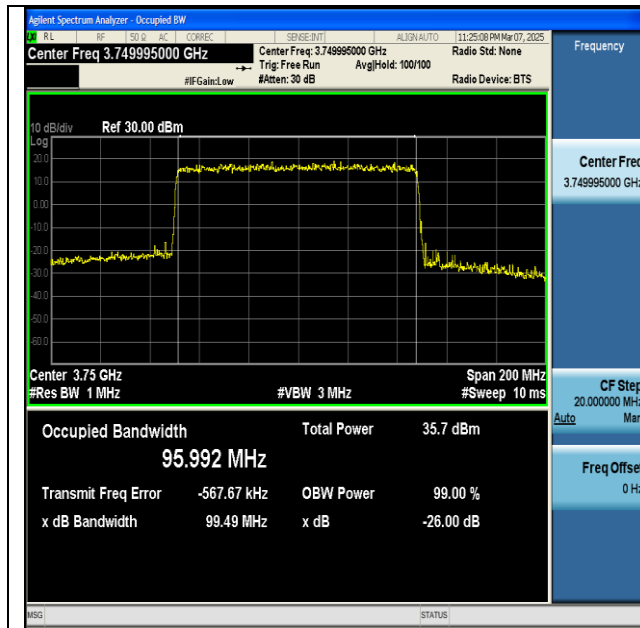
NTNV-n77(3700-3980)-PC2-30-100-L-DFT-QPSK- Outer_Full-Ant1-PASS
