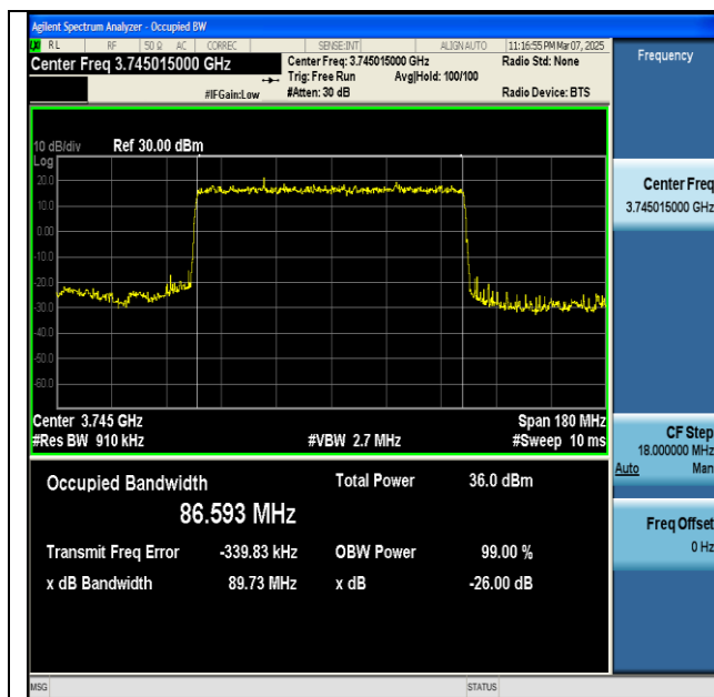
NTNV-n77(3700-3980)-PC2-30-90-L-DFT-BPSK- Outer_Full-Ant1-PASS
