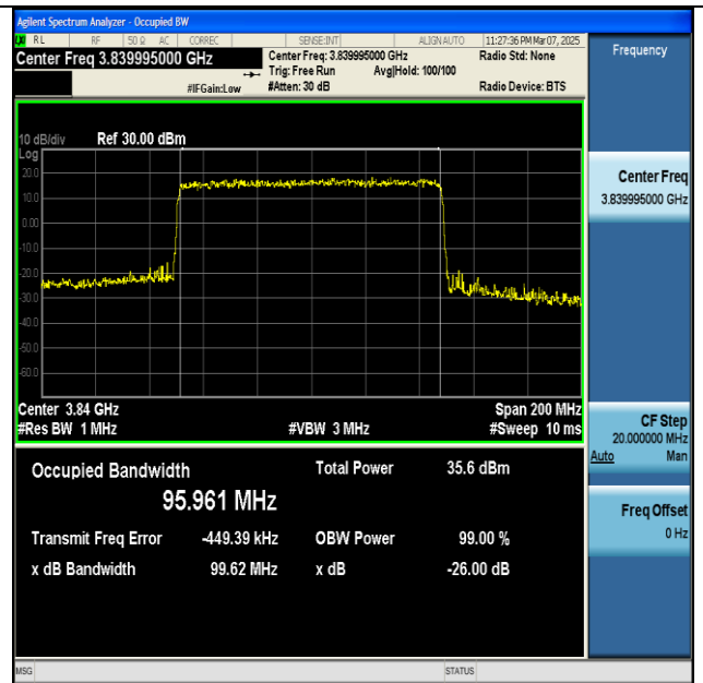
NTNV-n77(3700-3980)-PC2-30-100-M-DFT-QPSK- Outer_Full-Ant1-PASS
