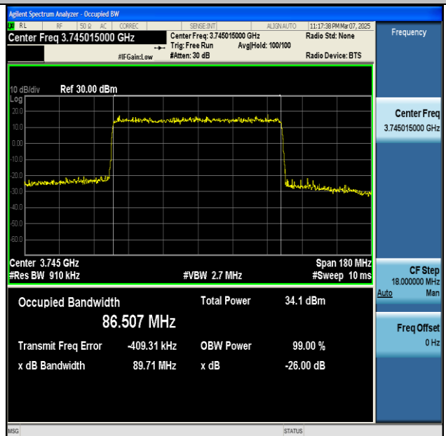
NTNV-n77(3700-3980)-PC2-30-90-L-DFT-64QAM- Outer_Full-Ant1-PASS
