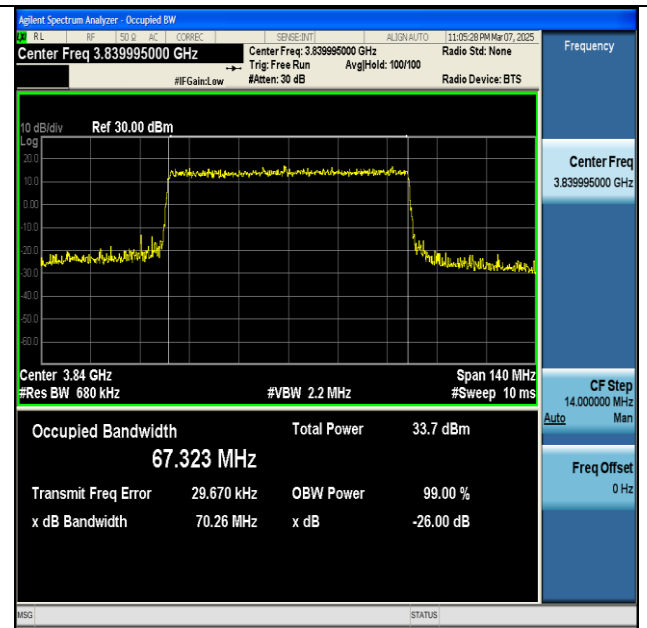
NTNV-n77(3700-3980)-PC2-30-70-M-CP-16QAM- Outer_Full-Ant1-PASS
