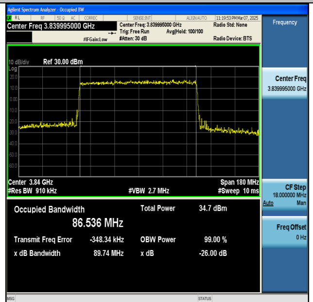
NTNV-n77(3700-3980)-PC2-30-90-M-DFT-16QAM- Outer_Full-Ant1-PASS
