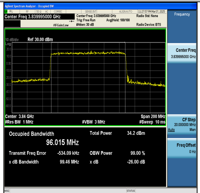
NTNV-n77(3700-3980)-PC2-30-100-M-DFT-64QAM- Outer_Full-Ant1-PASS
