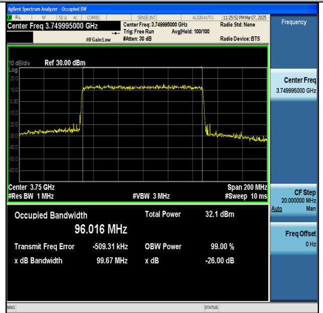
NTNV-n77(3700-3980)-PC2-30-100-L-DFT-256QAM- Outer_Full-Ant1-PASS
