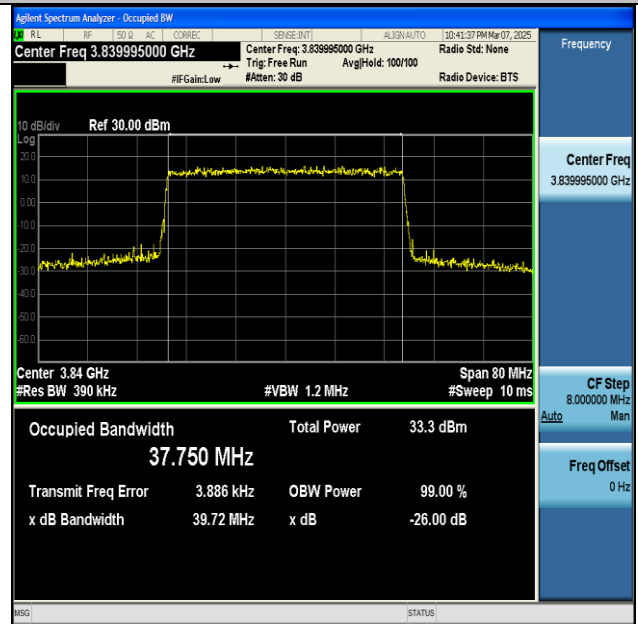
NTNV-n77(3700-3980)-PC2-30-40-M-CP-QPSK- Outer_Full-Ant1-PASS
