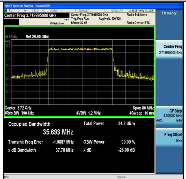
NTNV-n77(3700-3980)-PC2-30-40-L-DFT-16QAM- Outer_Full-Ant1-PASS
