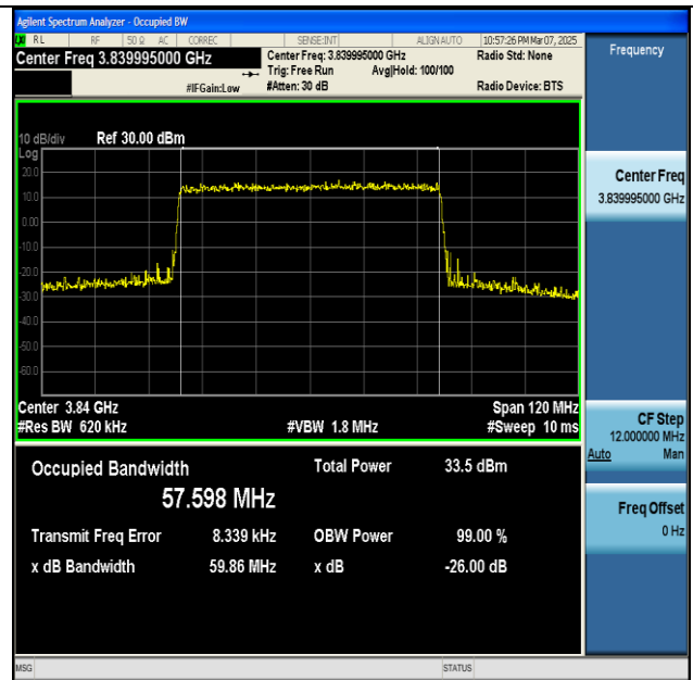
NTNV-n77(3700-3980)-PC2-30-60-M-CP-QPSK- Outer_Full-Ant1-PASS
