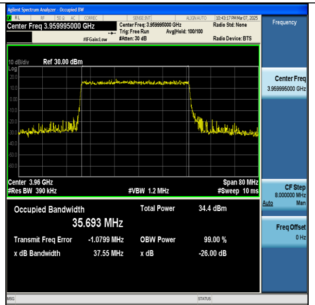
NTNV-n77(3700-3980)-PC2-30-40-H-DFT-16QAM- Outer_Full-Ant1-PASS
