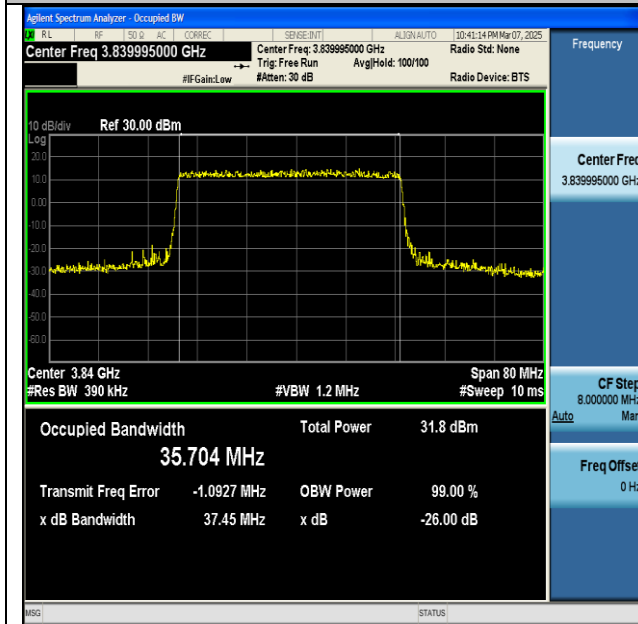
NTNV-n77(3700-3980)-PC2-30-40-M-DFT-256QAM- Outer_Full-Ant1-PASS
