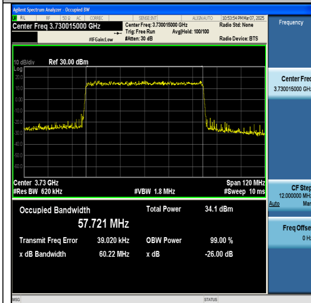
NTNV-n77(3700-3980)-PC2-30-60-L-DFT-64QAM- Outer_Full-Ant1-PASS
