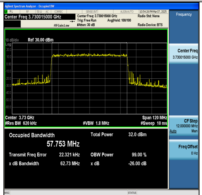
NTNV-n77(3700-3980)-PC2-30-60-L-DFT-256QAM- Outer_Full-Ant1-PASS
