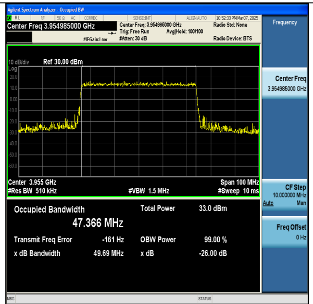
NTNV-n77(3700-3980)-PC2-30-50-H-CP-64QAM- Outer_Full-Ant1-PASS
