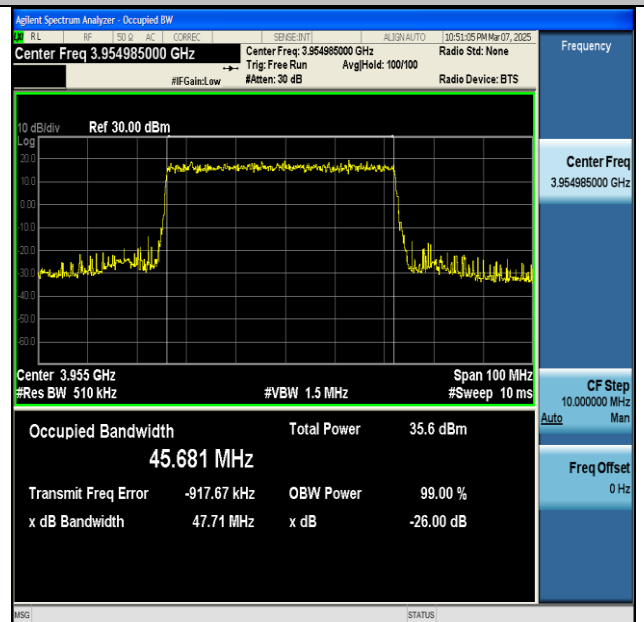
NTNV-n77(3700-3980)-PC2-30-50-H-DFT-QPSK- Outer_Full-Ant1-PASS
