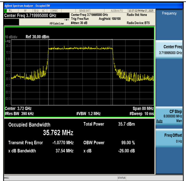
NTNV-n77(3700-3980)-PC2-30-40-L-DFT-BPSK- Outer_Full-Ant1-PASS
