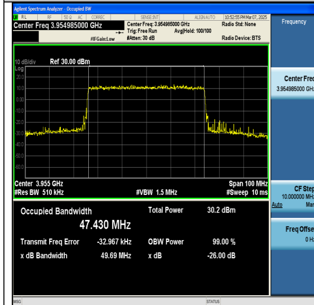
NTNV-n77(3700-3980)-PC2-30-50-H-CP-256QAM- Outer_Full-Ant1-PASS
