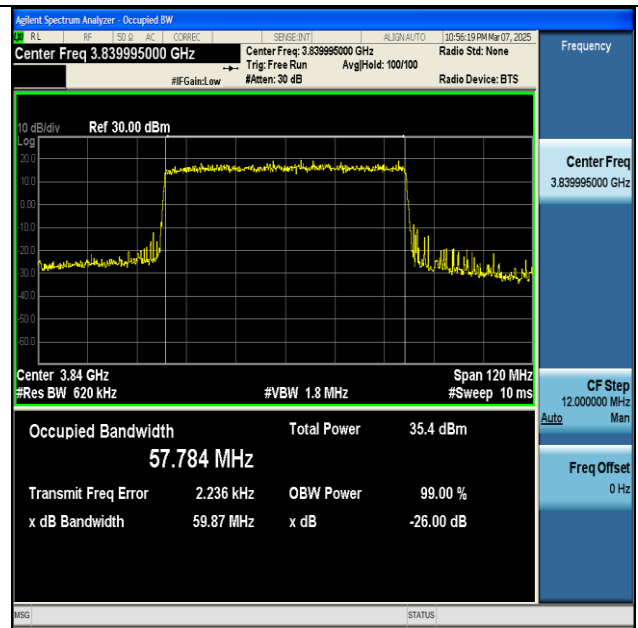
NTNV-n77(3700-3980)-PC2-30-60-M-DFT-QPSK- Outer_Full-Ant1-PASS
