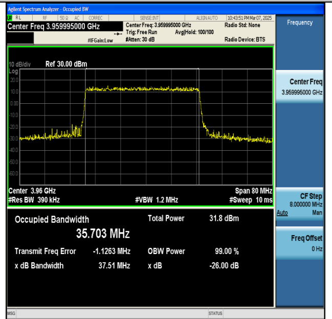
NTNV-n77(3700-3980)-PC2-30-40-H-DFT-256QAM- Outer_Full-Ant1-PASS
