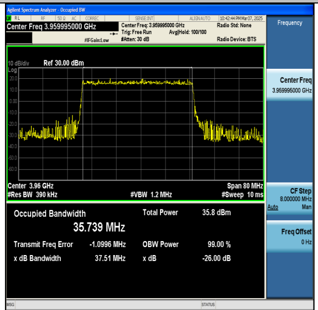
NTNV-n77(3700-3980)-PC2-30-40-H-DFT-BPSK-Outer_Full-Ant1-PASS
