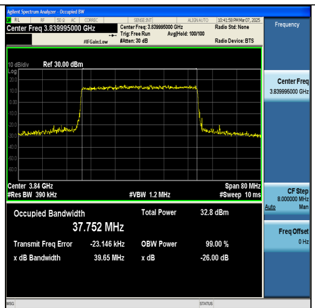
NTNV-n77(3700-3980)-PC2-30-40-M-CP-64QAM-Outer_Full-Ant1-PASS
