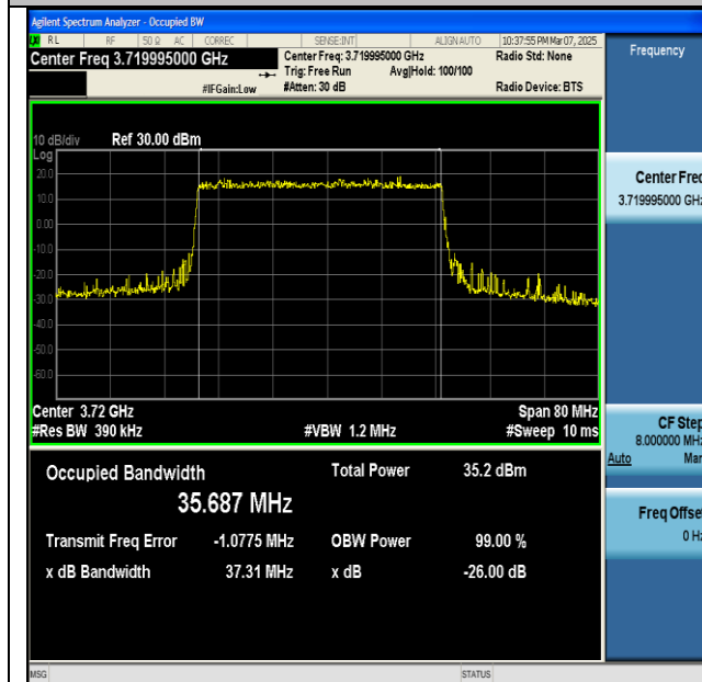
NTNV-n77(3700-3980)-PC2-30-40-L-DFT-QPSK- Outer_Full-Ant1-PASS
