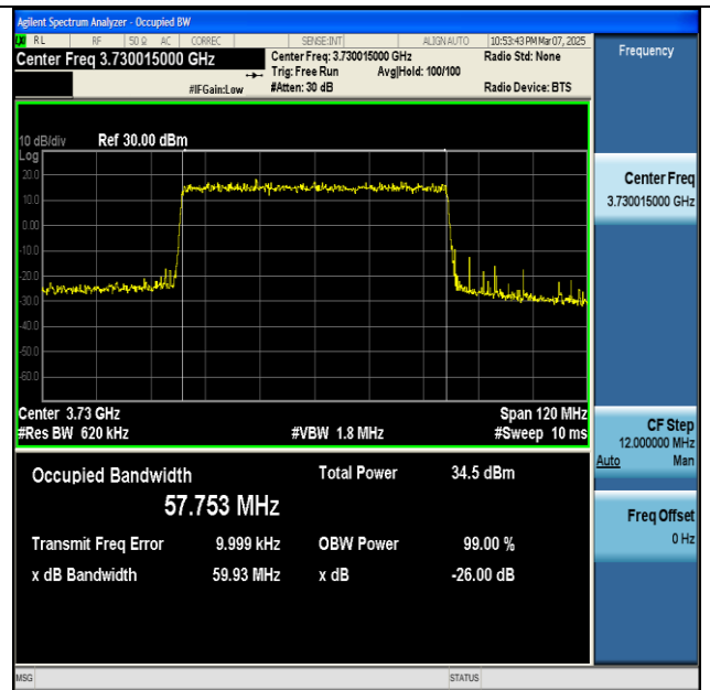
NTNV-n77(3700-3980)-PC2-30-60-L-DFT-16QAM- Outer_Full-Ant1-PASS
