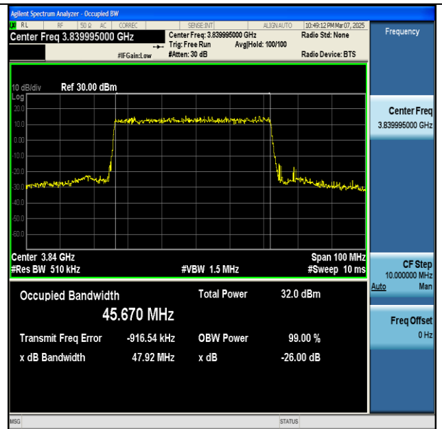
NTNV-n77(3700-3980)-PC2-30-50-M-DFT-256QAM- Outer_Full-Ant1-PASS
