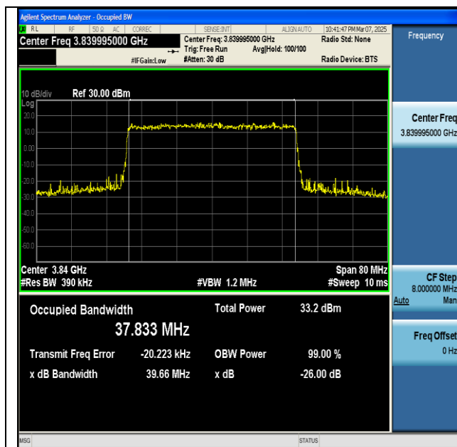
NTNV-n77(3700-3980)-PC2-30-40-M-CP-16QAM-Outer_Full-Ant1-PASS
