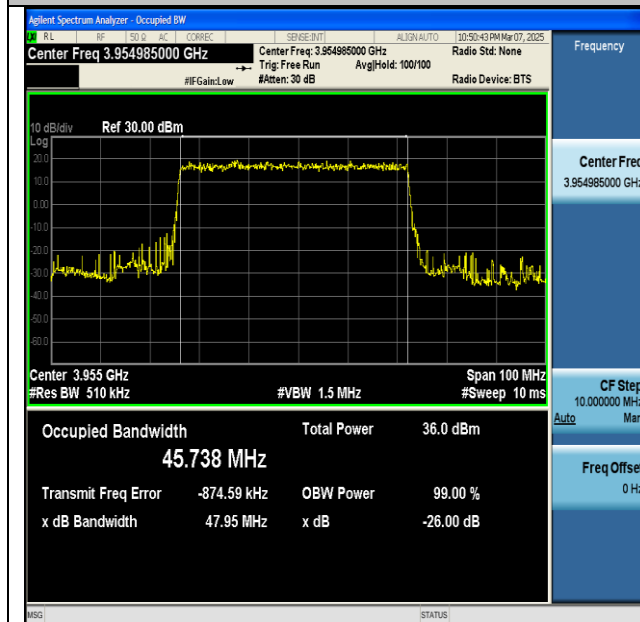
NTNV-n77(3700-3980)-PC2-30-50-H-DFT-BPSK- Outer_Full-Ant1-PASS
