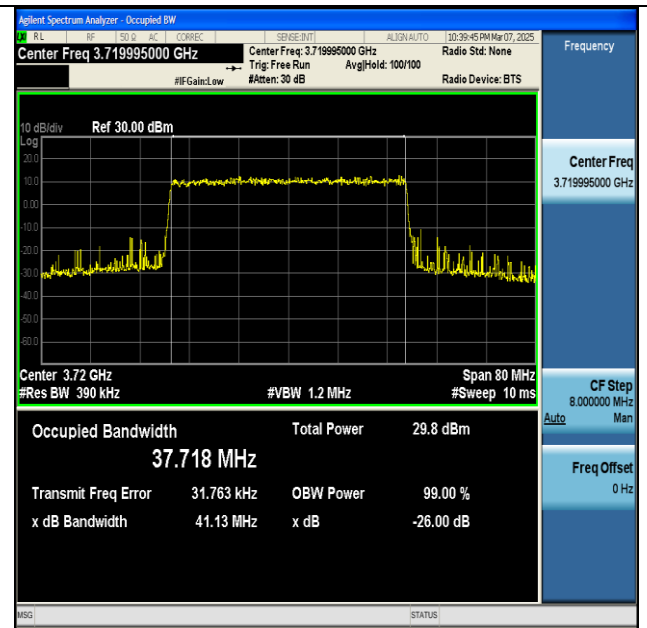
NTNV-n77(3700-3980)-PC2-30-40-L-CP-256QAM- Outer_Full-Ant1-PASS
