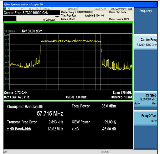
NTNV-n77(3700-3980)-PC2-30-60-L-DFT-BPSK- Outer_Full-Ant1-PASS
