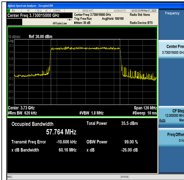
NTNV-n77(3700-3980)-PC2-30-60-L-DFT-QPSK- Outer_Full-Ant1-PASS
