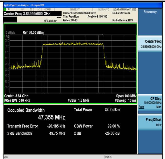
NTNV-n77(3700-3980)-PC2-30-50-M-CP-16QAM- Outer_Full-Ant1-PASS
