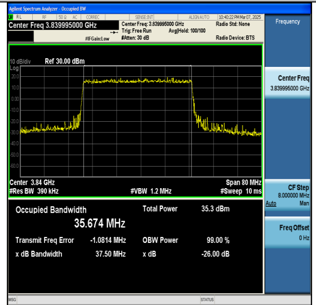
NTNV-n77(3700-3980)-PC2-30-40-M-DFT-QPSK- Outer_Full-Ant1-PASS
