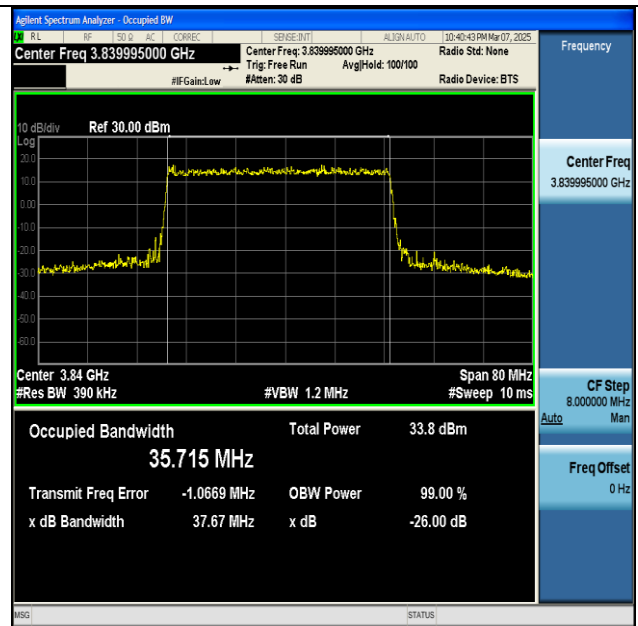
NTNV-n77(3700-3980)-PC2-30-40-M-DFT-64QAM- Outer_Full-Ant1-PASS
