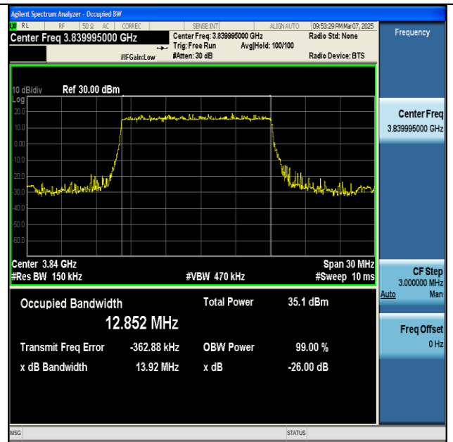
NTNV-n77(3700-3980)-PC2-30-15-M-DFT-QPSK- Outer_Full-Ant1-PASS
