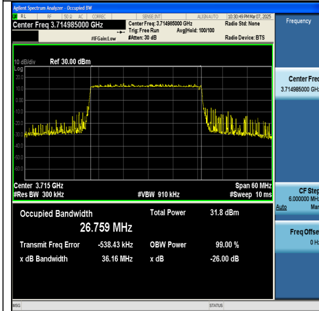
NTNV-n77(3700-3980)-PC2-30-30-L-DFT-256QAM- Outer_Full-Ant1-PASS
