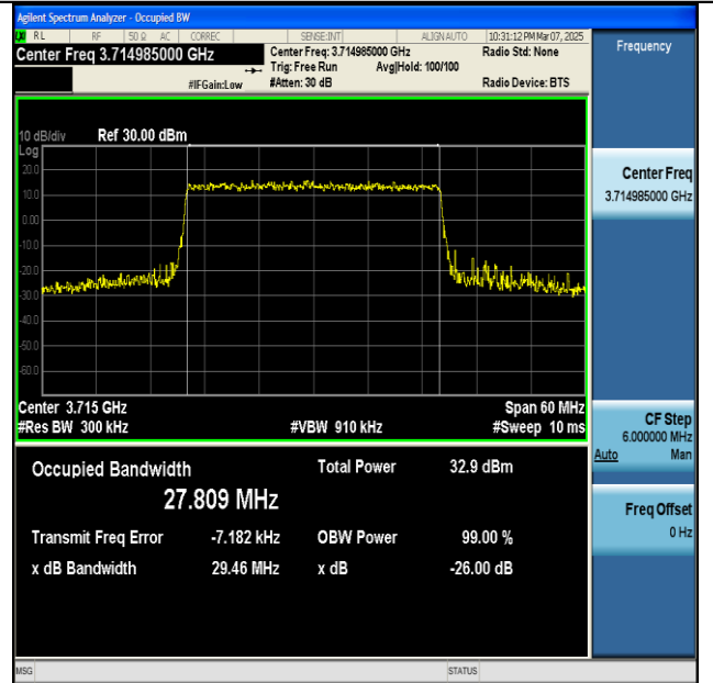
NTNV-n77(3700-3980)-PC2-30-30-L-CP-QPSK- Outer_Full-Ant1-PASS
