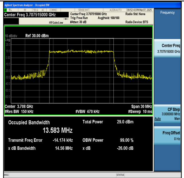
NTNV-n77(3700-3980)-PC2-30-15-L-CP-256QAM- Outer_Full-Ant1-PASS
