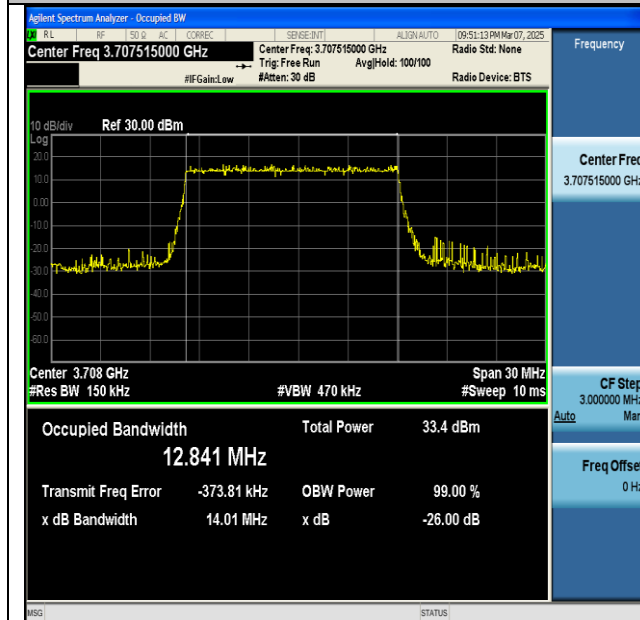
NTNV-n77(3700-3980)-PC2-30-15-L-DFT-64QAM- Outer_Full-Ant1-PASS
