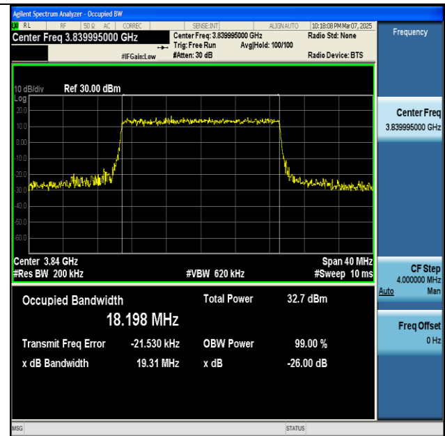
NTNV-n77(3700-3980)-PC2-30-20-M-CP-16QAM-Outer_Full-Ant1-PASS
