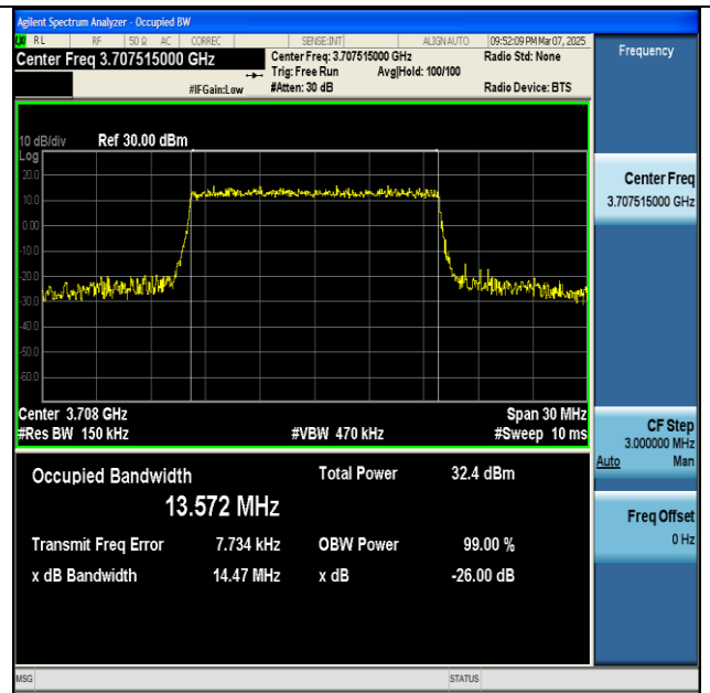
NTNV-n77(3700-3980)-PC2-30-15-L-CP-16QAM- Outer_Full-Ant1-PASS
