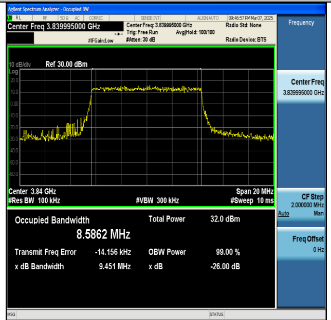
NTNV-n77(3700-3980)-PC2-30-10-M-CP-16QAM- Outer_Full-Ant1-PASS
