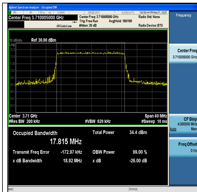
NTNV-n77(3700-3980)-PC2-30-20-L-DFT-16QAM- Outer_Full-Ant1-PASS
