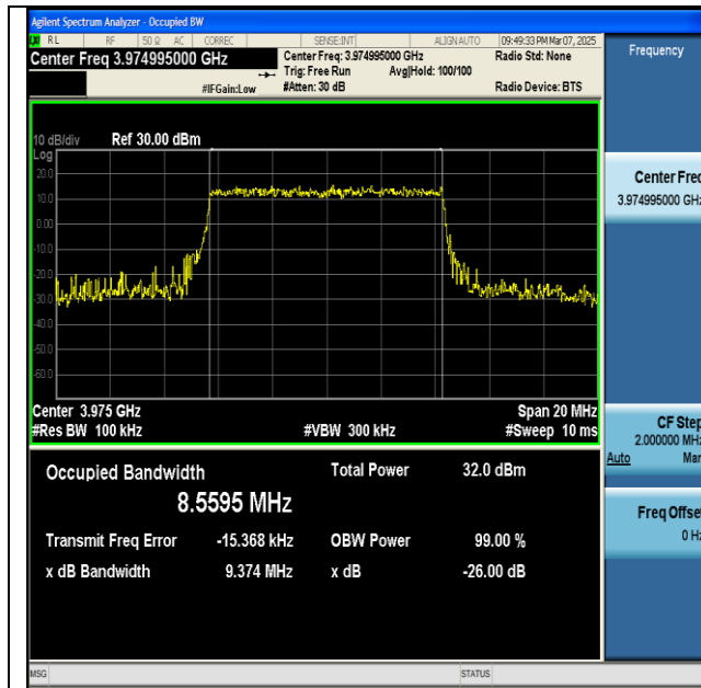
NTNV-n77(3700-3980)-PC2-30-10-H-CP-16QAM- Outer_Full-Ant1-PASS
