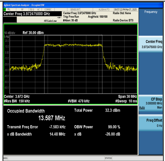
NTNV-n77(3700-3980)-PC2-30-15-H-CP-16QAM- Outer_Full-Ant1-PASS
