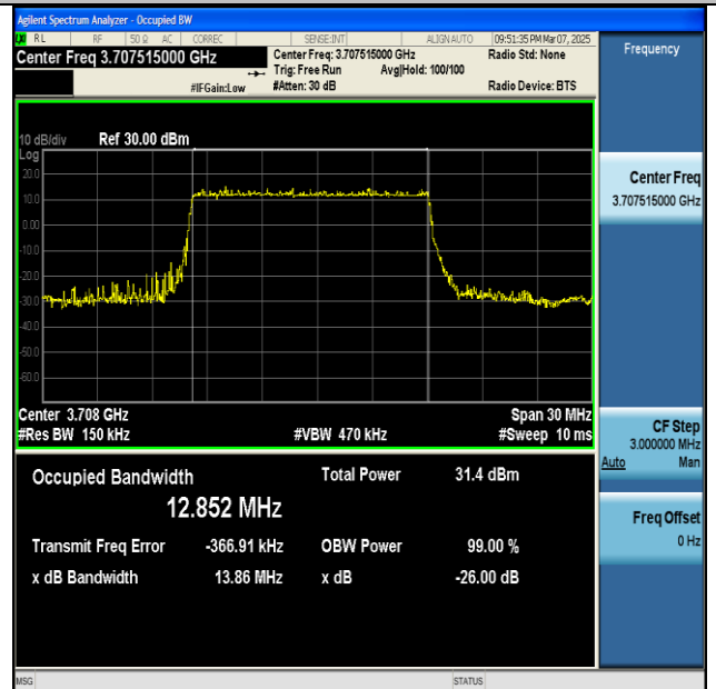
NTNV-n77(3700-3980)-PC2-30-15-L-DFT-256QAM- Outer_Full-Ant1-PASS
