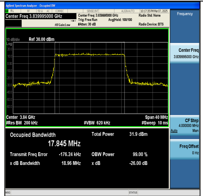
NTNV-n77(3700-3980)-PC2-30-20-M-DFT-256QAM- Outer_Full-Ant1-PASS
