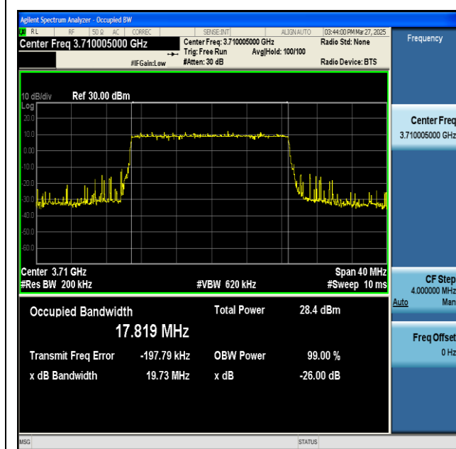
NTNV-n77(3700-3980)-PC2-30-20-L-DFT-256QAM- Outer_Full-Ant1-PASS
