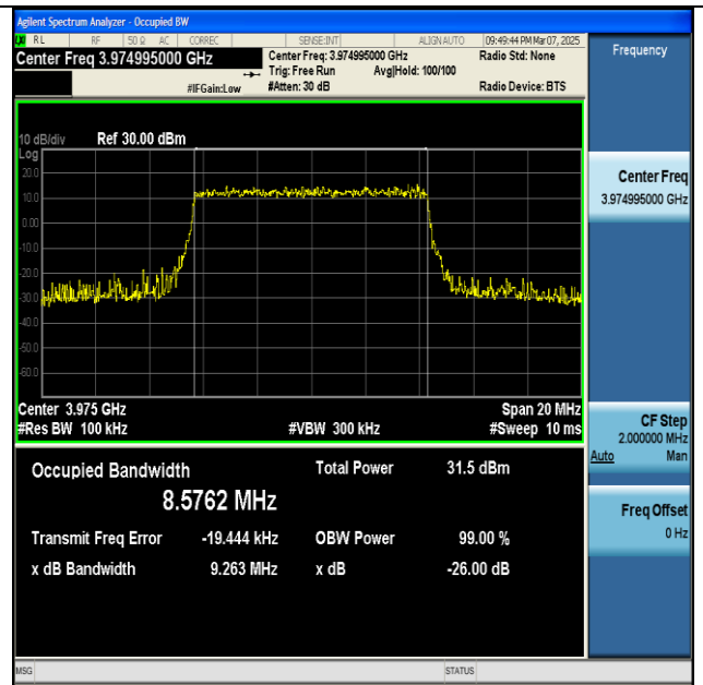
NTNV-n77(3700-3980)-PC2-30-10-H-CP-64QAM- Outer_Full-Ant1-PASS
