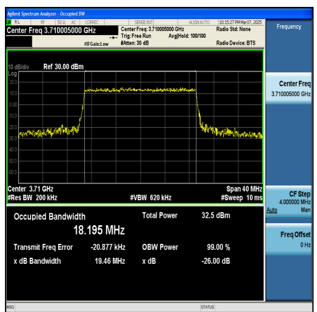
NTNV-n77(3700-3980)-PC2-30-20-L-CP-QPSK- Outer_Full-Ant1-PASS
