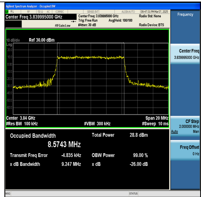
NTNV-n77(3700-3980)-PC2-30-10-M-CP-256QAM- Outer_Full-Ant1-PASS
