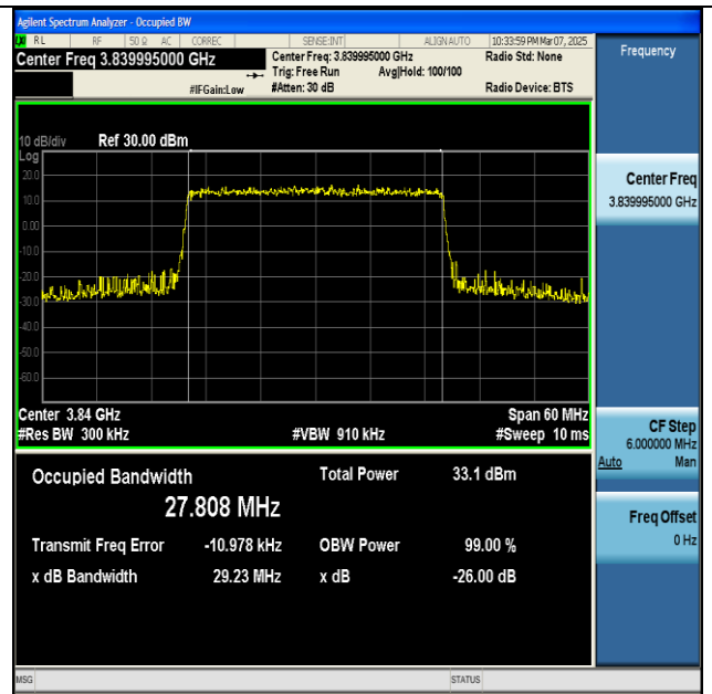
NTNV-n77(3700-3980)-PC2-30-30-M-CP-16QAM- Outer_Full-Ant1-PASS
