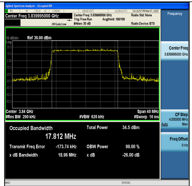
NTNV-n77(3700-3980)-PC2-30-20-M-DFT-16QAM- Outer_Full-Ant1-PASS
