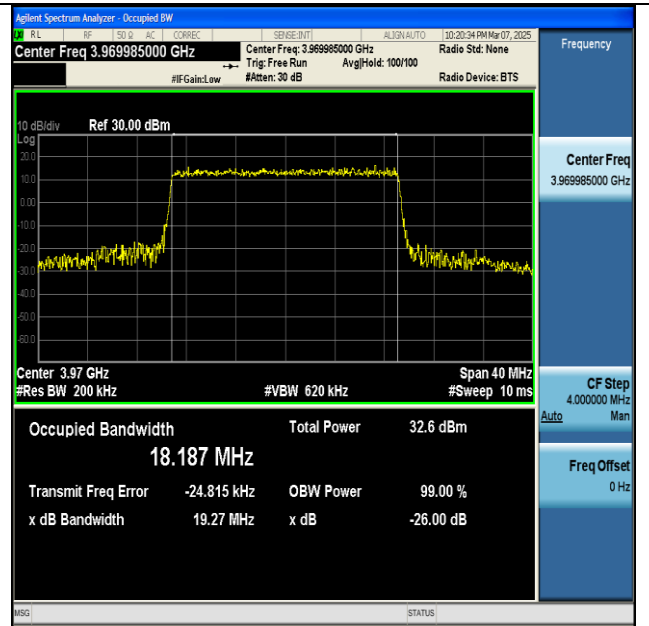
NTVN-n77(3700-3980)-PC2-30-20-H-CP-QPSK- Outer_Full-Ant1-PASS
