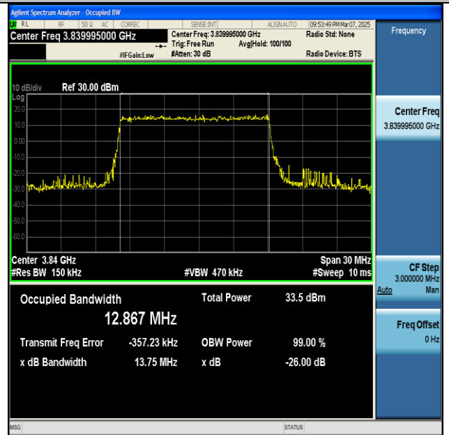
NTNV-n77(3700-3980)-PC2-30-15-M-DFT-64QAM- Outer_Full-Ant1-PASS
