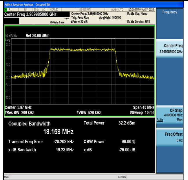
NTVN-n77(3700-3980)-PC2-30-20-H-CP-64QAM- Outer_Full-Ant1-PASS
