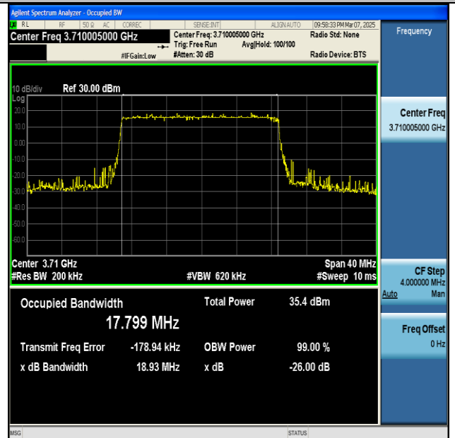
NTNV-n77(3700-3980)-PC2-30-20-L-DFT-QPSK- Outer_Full-Ant1-PASS
