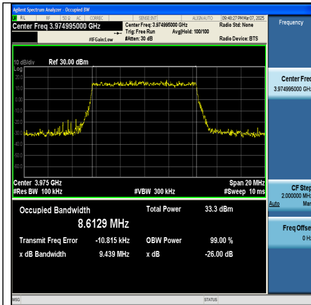
NTNV-n77(3700-3980)-PC2-30-10-H-DFT-16QAM-Outer_Full-Ant1-PASS
