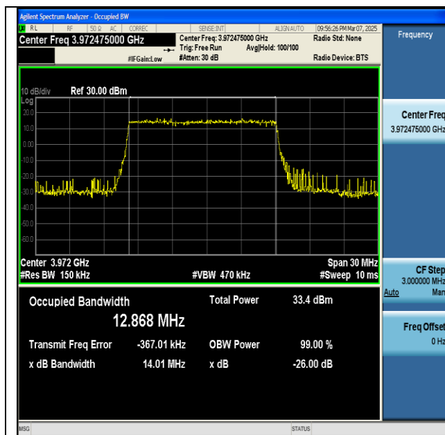
NTNV-n77(3700-3980)-PC2-30-15-H-DFT-64QAM- Outer_Full-Ant1-PASS
