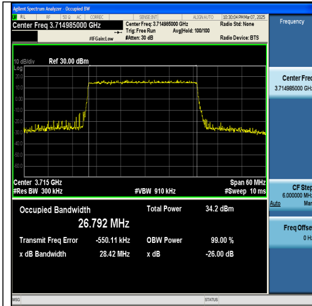
NTNV-n77(3700-3980)-PC2-30-30-L-DFT-16QAM- Outer_Full-Ant1-PASS
