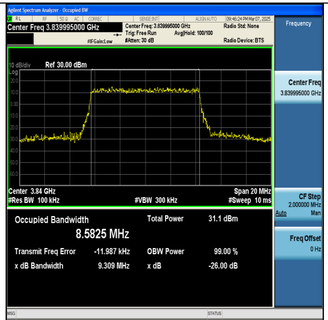
NTNV-n77(3700-3980)-PC2-30-10-M-DFT-256QAM- Outer_Full-Ant1-PASS
