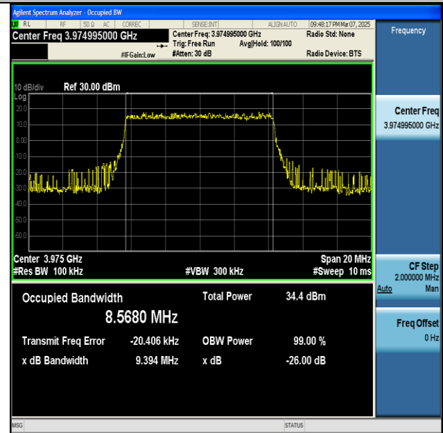
NTNV-n77(3700-3980)-PC2-30-10-H-DFT-QPSK- Outer_Full-Ant1-PASS
