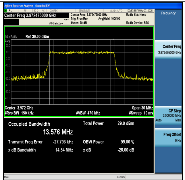
NTNV-n77(3700-3980)-PC2-30-15-H-CP-256QAM- Outer_Full-Ant1-PASS
