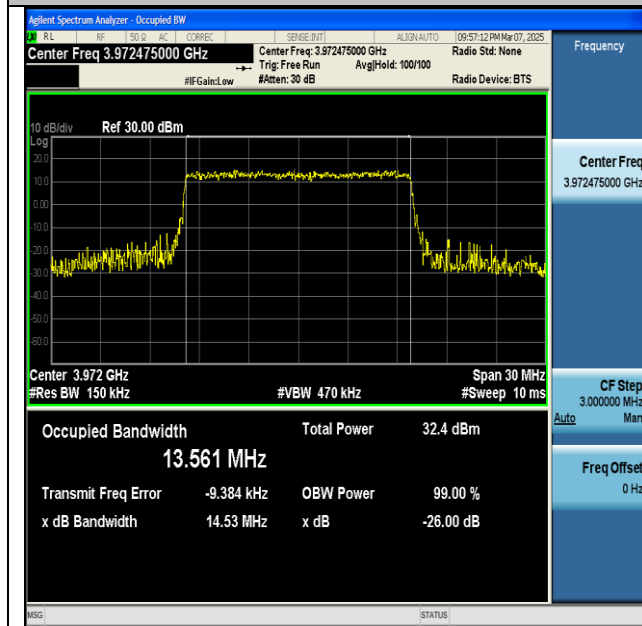
NTNV-n77(3700-3980)-PC2-30-15-H-CP-QPSK- Outer_Full-Ant1-PASS
