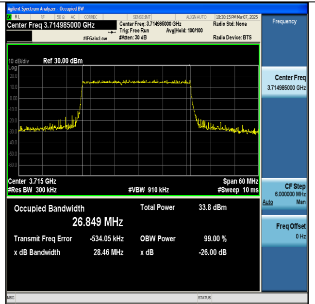
NTNV-n77(3700-3980)-PC2-30-30-L-DFT-64QAM- Outer_Full-Ant1-PASS
