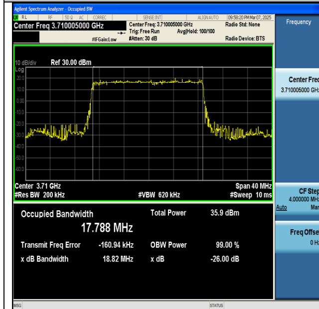
NTNV-n77(3700-3980)-PC2-30-20-L-DFT-BPSK- Outer_Full-Ant1-PASS
