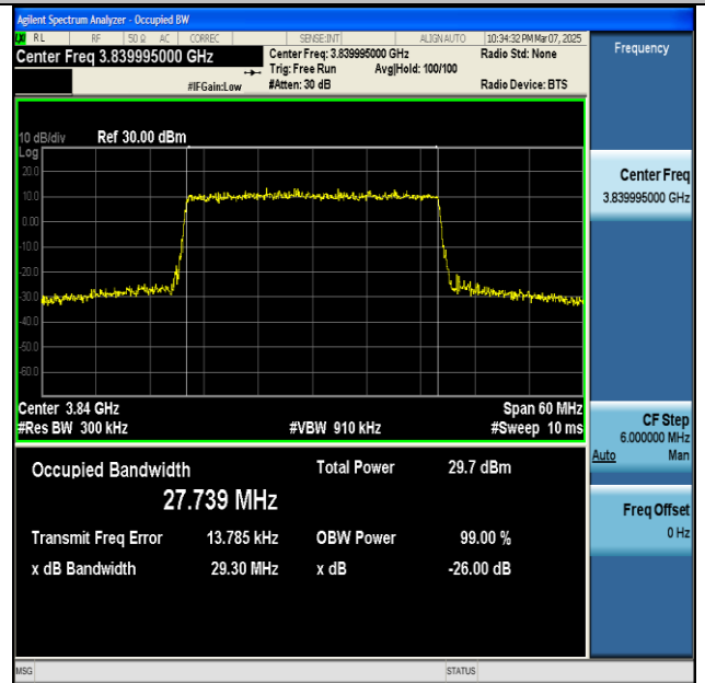
NTNV-n77(3700-3980)-PC2-30-30-M-CP-256QAM- Outer_Full-Ant1-PASS
