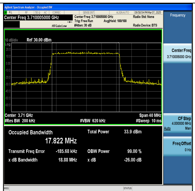
NTNV-n77(3700-3980)-PC2-30-20-L-DFT-64QAM- Outer_Full-Ant1-PASS
