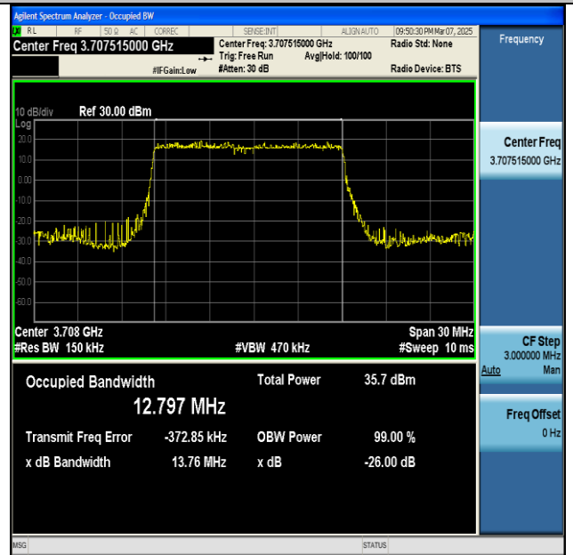
NTNV-n77(3700-3980)-PC2-30-15-L-DFT-BPSK- Outer_Full-Ant1-PASS
