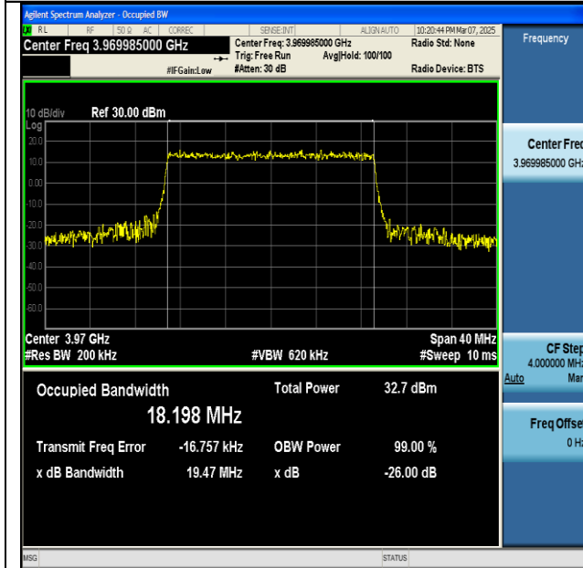
NTVN-n77(3700-3980)-PC2-30-20-H-CP-16QAM- Outer_Full-Ant1-PASS
