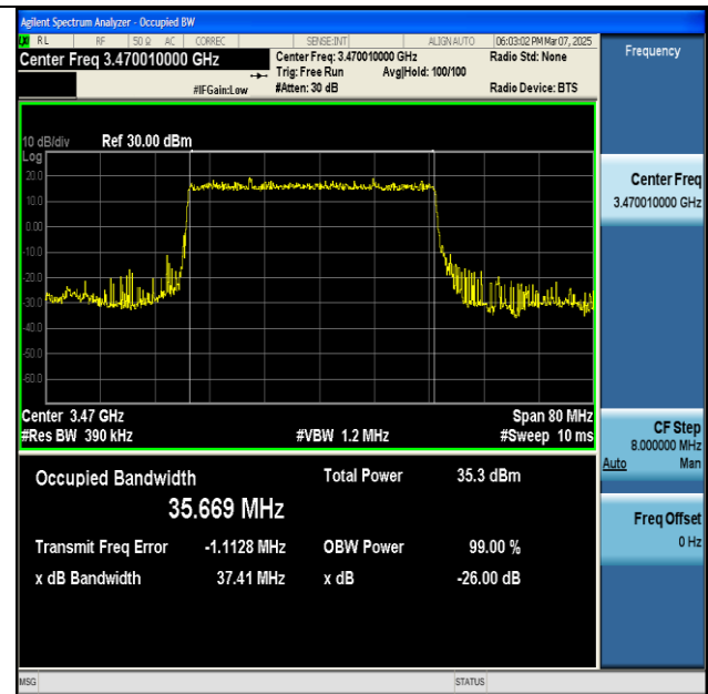
NTNV-n77(3450-3550)-PC2-30-40-L-DFT-BPSK-Outer_Full-Ant1-PASS
