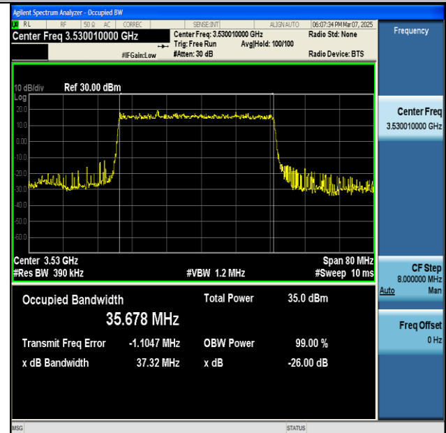
NTNV-n77(3450-3550)-PC2-30-40-H-DFT-BPSK- Outer_Full-Ant1-PASS
