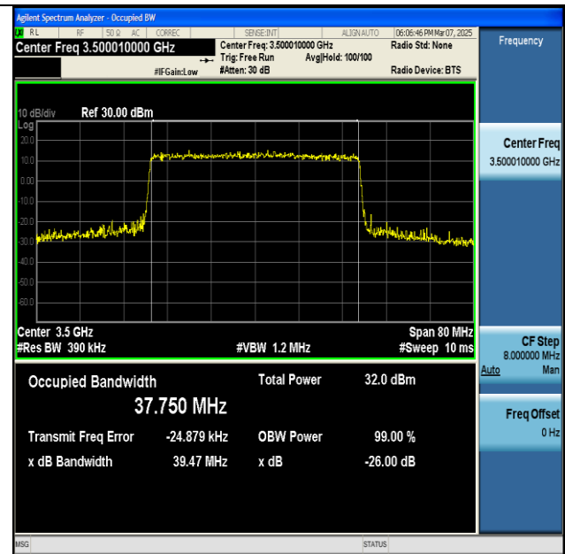
NTNV-n77(3450-3550)-PC2-30-40-M-CP-64QAM- Outer_Full-Ant1-PASS
