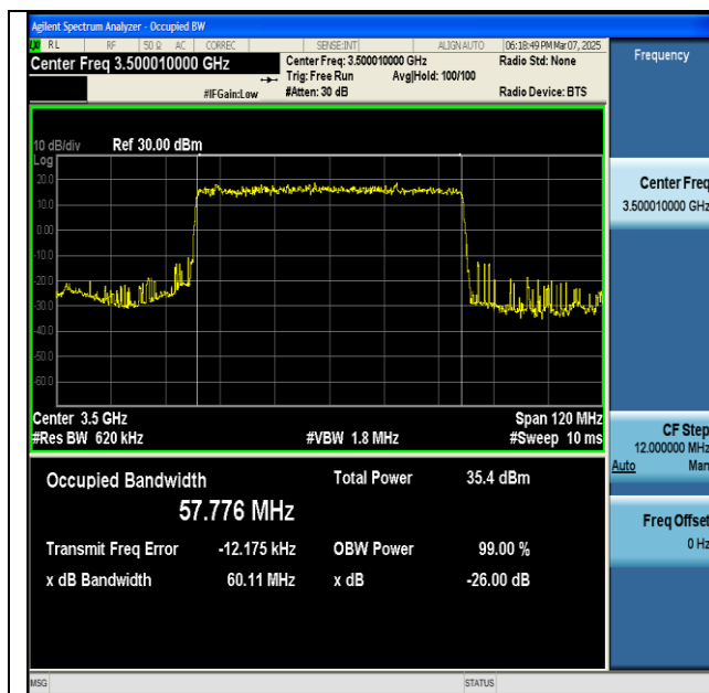
NTNV-n77(3450-3550)-PC2-30-60-M-DFT-BPSK-Outer_Full-Ant1-PASS
