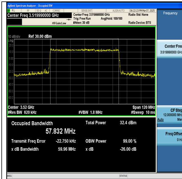
NTNV-n77(3450-3550)-PC2-30-60-H-CP-64QAM- Outer_Full-Ant1-PASS
