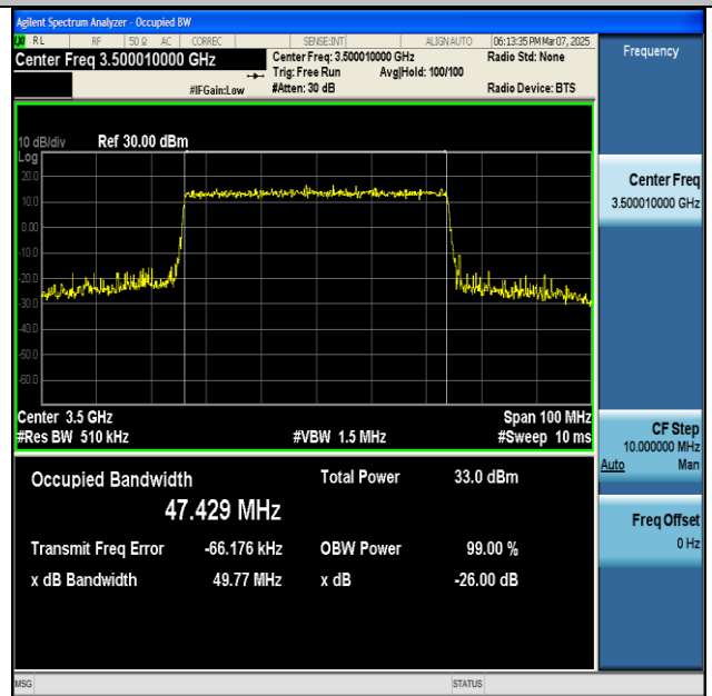
NTNV-n77(3450-3550)-PC2-30-50-M-CP-16QAM- Outer_Full-Ant1-PASS
