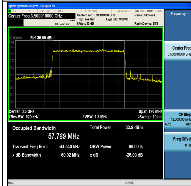
NTNV-n77(3450-3550)-PC2-30-60-M-DFT-16QAM-Outer_Full-Ant1-PASS
