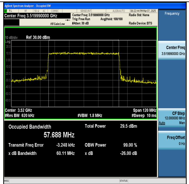
NTNV-n77(3450-3550)-PC2-30-60-H-CP-256QAM- Outer_Full-Ant1-PASS
