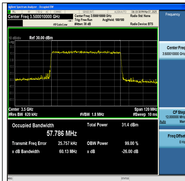
NTNV-n77(3450-3550)-PC2-30-60-M-DFT-256QAM- Outer_Full-Ant1-PASS
