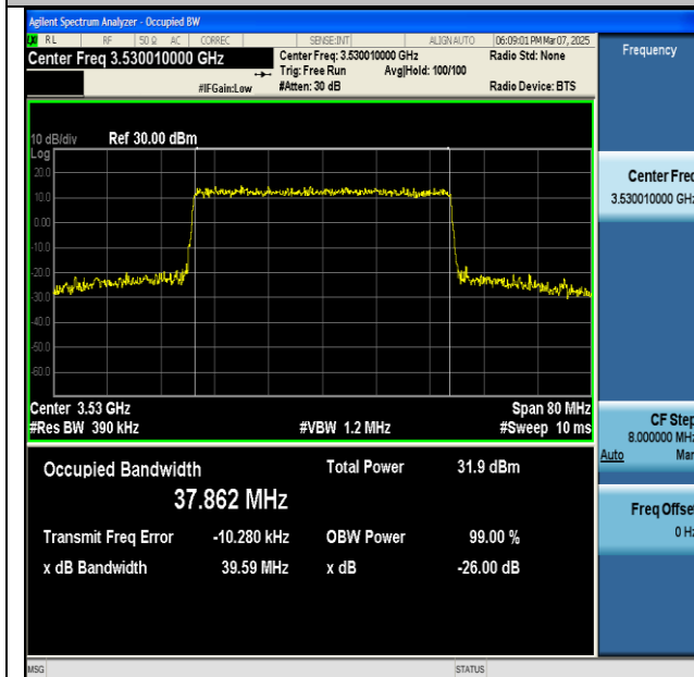
NTNV-n77(3450-3550)-PC2-30-40-H-CP-64QAM- Outer_Full-Ant1-PASS
