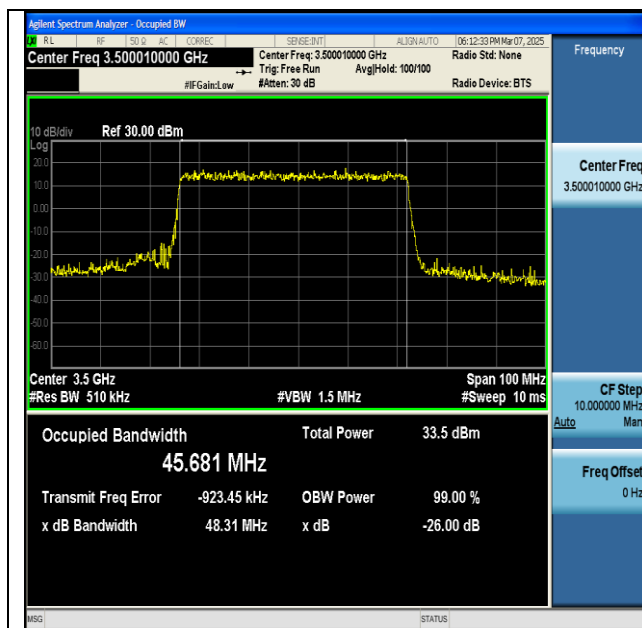
NTNV-n77(3450-3550)-PC2-30-50-M-DFT-64QAM- Outer_Full-Ant1-PASS
