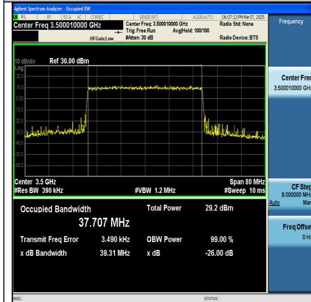
NTNV-n77(3450-3550)-PC2-30-40-M-CP-256QAM- Outer_Full-Ant1-PASS
