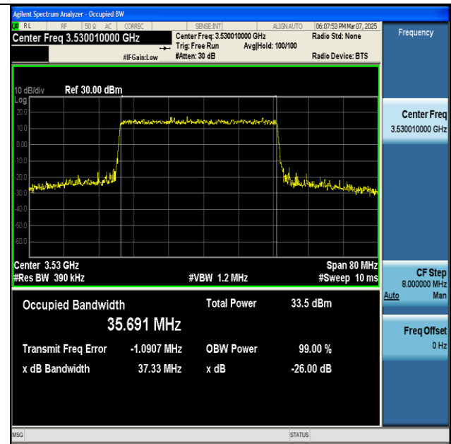
NTNV-n77(3450-3550)-PC2-30-40-H-DFT-16QAM- Outer_Full-Ant1-PASS
