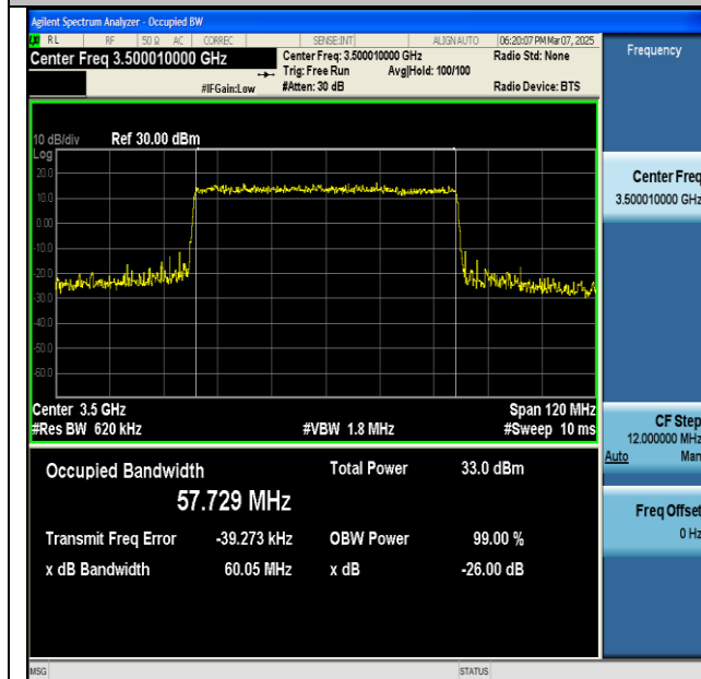
NTNV-n77(3450-3550)-PC2-30-60-M-CP-16QAM- Outer_Full-Ant1-PASS
