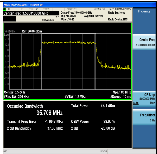
NTNV-n77(3450-3550)-PC2-30-40-M-DFT-64QAM- Outer_Full-Ant1-PASS
