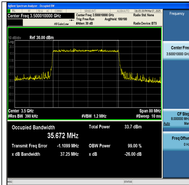
NTNV-n77(3450-3550)-PC2-30-40-M-DFT-16QAM- Outer_Full-Ant1-PASS
