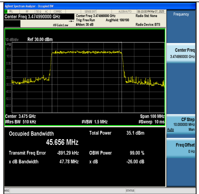
NTNV-n77(3450-3550)-PC2-30-50-L-DFT-QPSK- Outer_Full-Ant1-PASS
