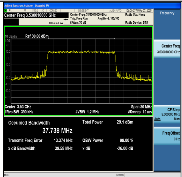
NTNV-n77(3450-3550)-PC2-30-40-H-CP-256QAM- Outer_Full-Ant1-PASS
