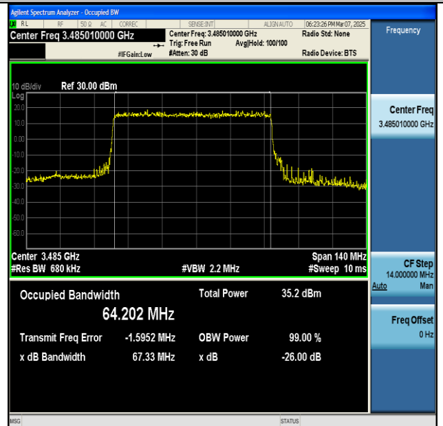
NTNV-n77(3450-3550)-PC2-30-70-L-DFT-QPSK- Outer_Full-Ant1-PASS
