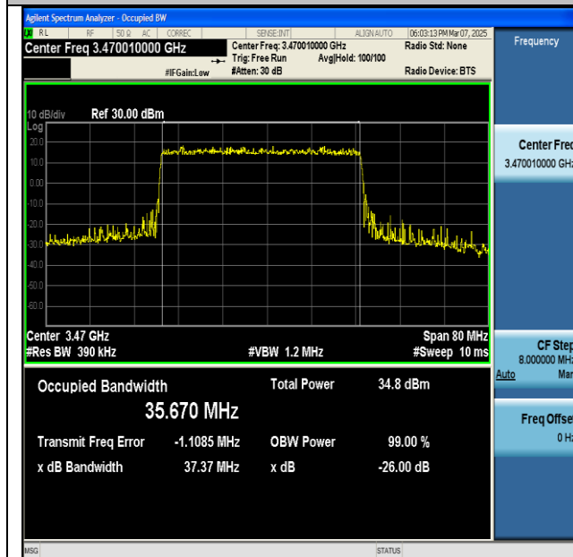
NTNV-n77(3450-3550)-PC2-30-40-L-DFT-QPSK-Outer_Full-Ant1-PASS
