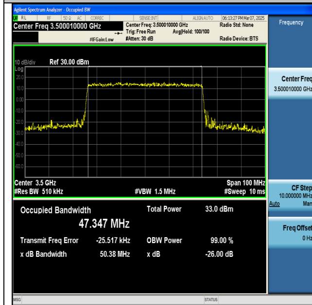
NTNV-n77(3450-3550)-PC2-30-50-M-CP-QPSK- Outer_Full-Ant1-PASS
