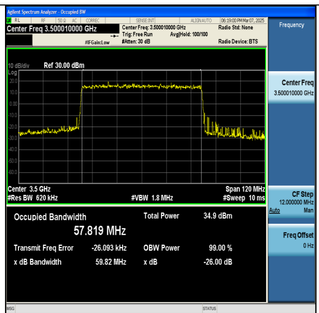
NTNV-n77(3450-3550)-PC2-30-60-M-DFT-QPSK-Outer_Full-Ant1-PASS
