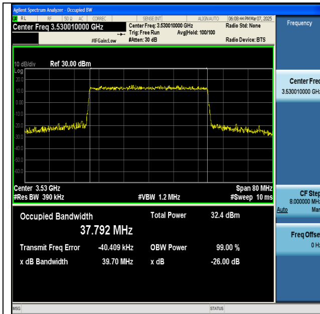
NTNV-n77(3450-3550)-PC2-30-40-H-CP-QPSK- Outer_Full-Ant1-PASS
