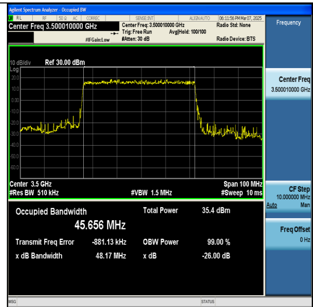
NTNV-n77(3450-3550)-PC2-30-50-M-DFT-BPSK- Outer_Full-Ant1-PASS
