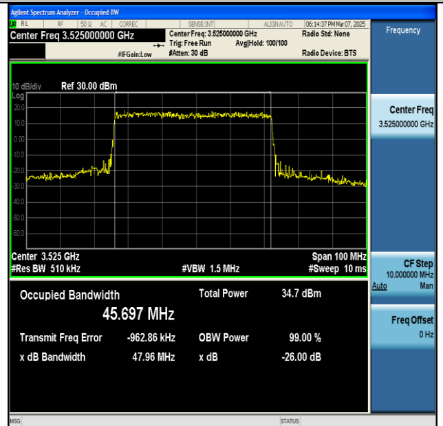
NTNV-n77(3450-3550)-PC2-30-50-H-DFT-QPSK- Outer_Full-Ant1-PASS
