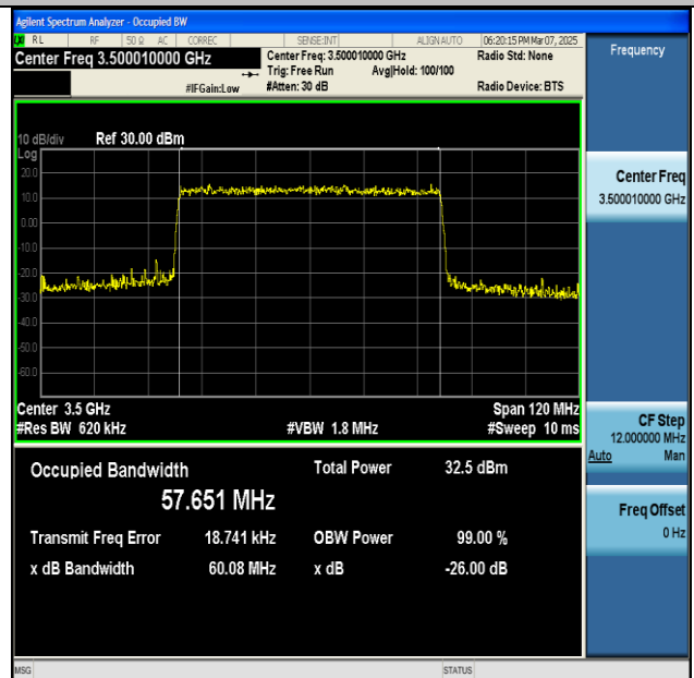
NTNV-n77(3450-3550)-PC2-30-60-M-CP-64QAM- Outer_Full-Ant1-PASS
