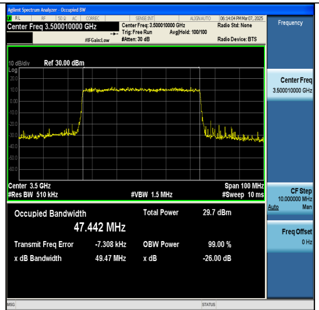
NTNV-n77(3450-3550)-PC2-30-50-M-CP-256QAM- Outer_Full-Ant1-PASS
