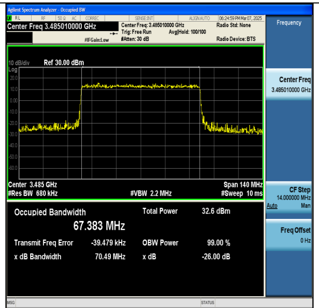
NTNV-n77(3450-3550)-PC2-30-70-L-CP-64QAM- Outer_Full-Ant1-PASS
