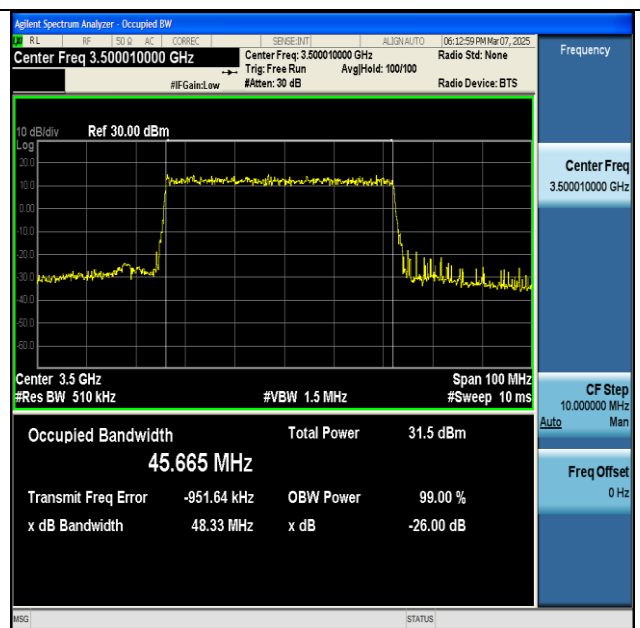
NTNV-n77(3450-3550)-PC2-30-50-M-DFT-256QAM- Outer_Full-Ant1-PASS
