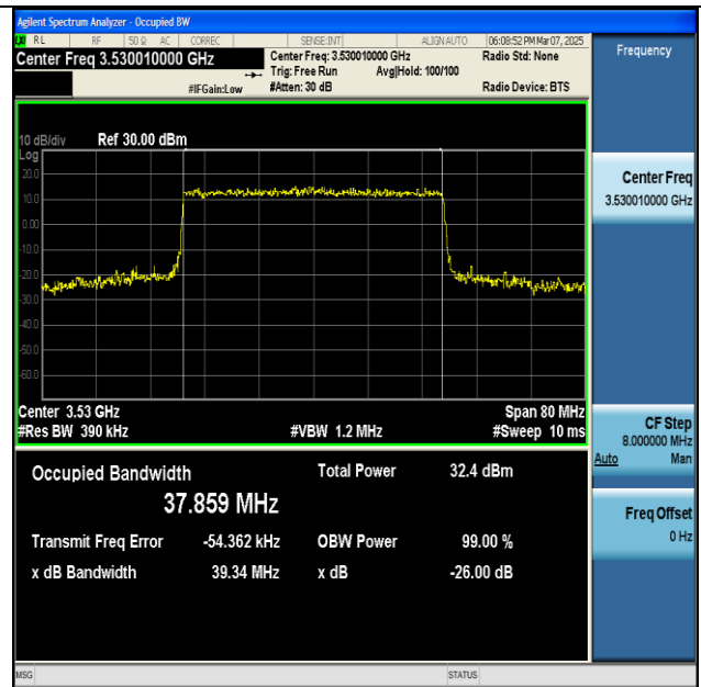
NTNV-n77(3450-3550)-PC2-30-40-H-CP-16QAM- Outer_Full-Ant1-PASS
