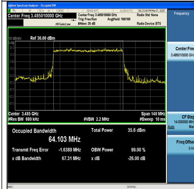
NTNV-n77(3450-3550)-PC2-30-70-L-DFT-BPSK- Outer_Full-Ant1-PASS
