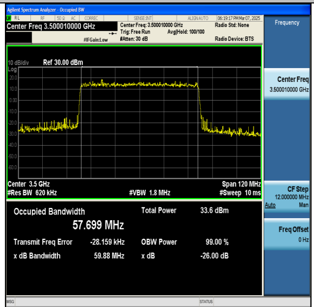
NTNV-n77(3450-3550)-PC2-30-60-M-DFT-64QAM-Outer_Full-Ant1-PASS
