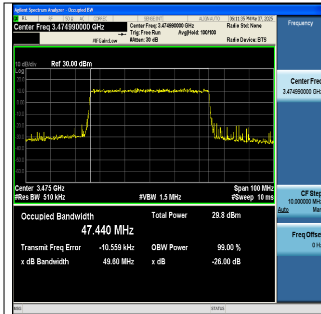
NTNV-n77(3450-3550)-PC2-30-50-L-CP-256QAM- Outer_Full-Ant1-PASS
