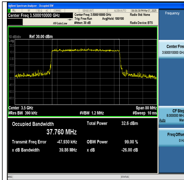
NTNV-n77(3450-3550)-PC2-30-40-M-CP-16QAM- Outer_Full-Ant1-PASS
