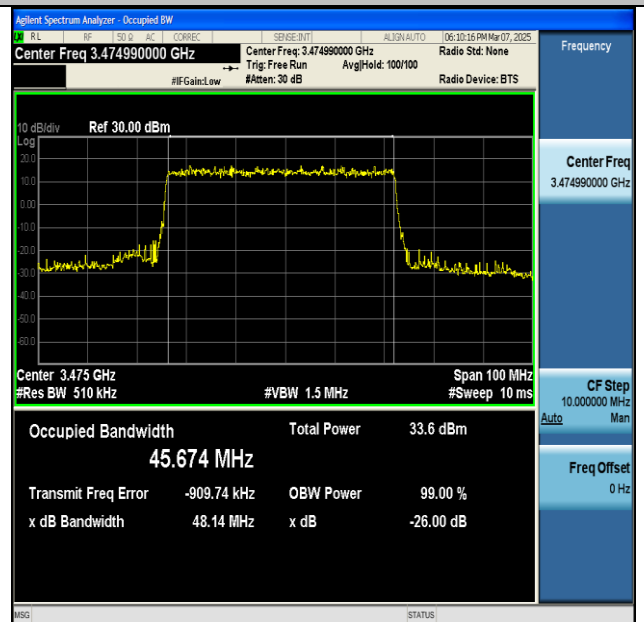
NTNV-n77(3450-3550)-PC2-30-50-L-DFT-64QAM- Outer_Full-Ant1-PASS
