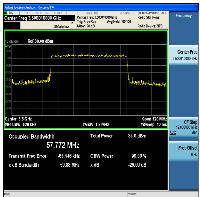
NTNV-n77(3450-3550)-PC2-30-60-M-CP-QPSK- Outer_Full-Ant1-PASS
