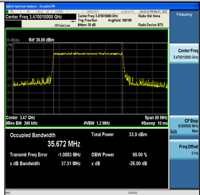
NTNV-n77(3450-3550)-PC2-30-40-L-DFT-16QAM-Outer_Full-Ant1-PASS
