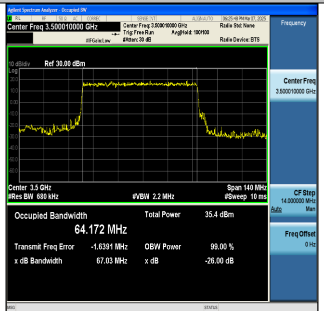
NTNV-n77(3450-3550)-PC2-30-70-M-DFT-BPSK- Outer_Full-Ant1-PASS
