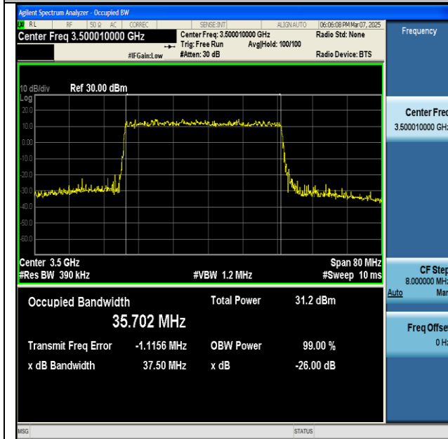
NTNV-n77(3450-3550)-PC2-30-40-M-DFT-256QAM- Outer_Full-Ant1-PASS
