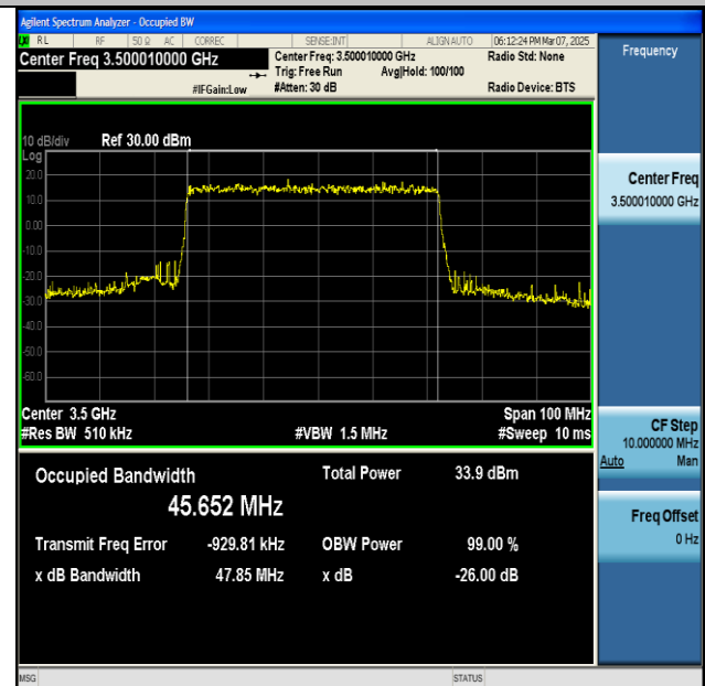
NTNV-n77(3450-3550)-PC2-30-50-M-DFT-16QAM- Outer_Full-Ant1-PASS
