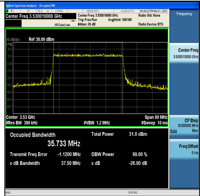
NTNV-n77(3450-3550)-PC2-30-40-H-DFT-256QAM- Outer_Full-Ant1-PASS
