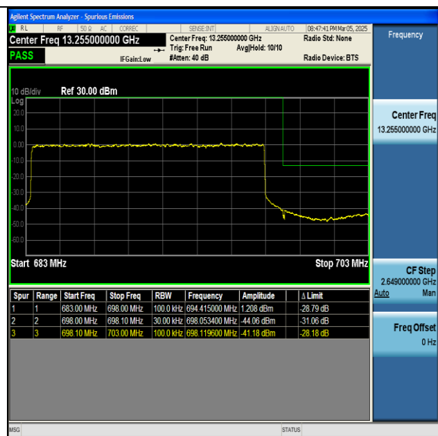
NTNV-n71-PC3-15-15-H-DFT-BPSK-Outer_Full-PASS
