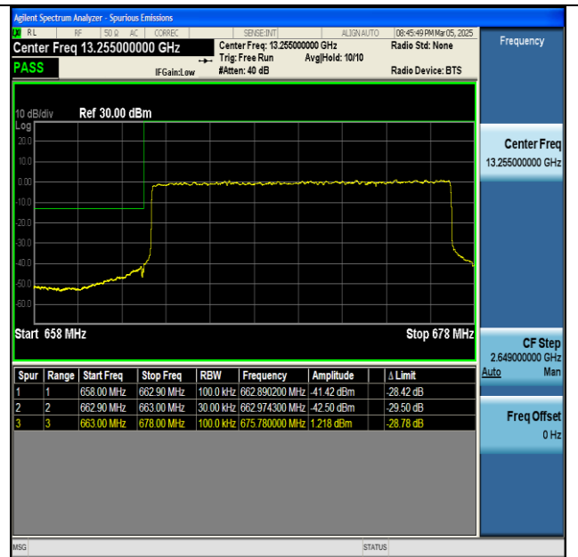
NTNV-n71-PC3-15-15-L-DFT-BPSK-Outer_Full-PASS
