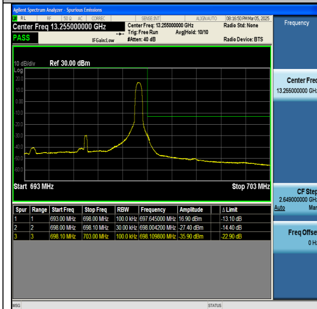
NTNV-n71-PC3-15-5-H-CP-QPSK-Edge_1RB_Right-PASS
