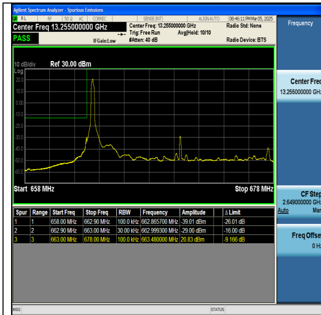
NTNV-n71-PC3-15-15-L-DFT-BPSK-Edge_1RB_Left-PASS
