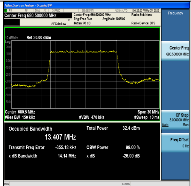
NTNV-n71-PC3-15-15-M-DFT-BPSK-Outer_Full-Ant1- PASS
