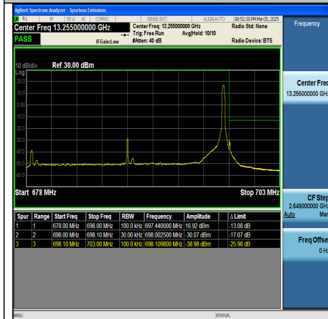
NTNV-n71-PC3-15-20-H-CP-QPSK-Edge_1RB_Right-PASS
