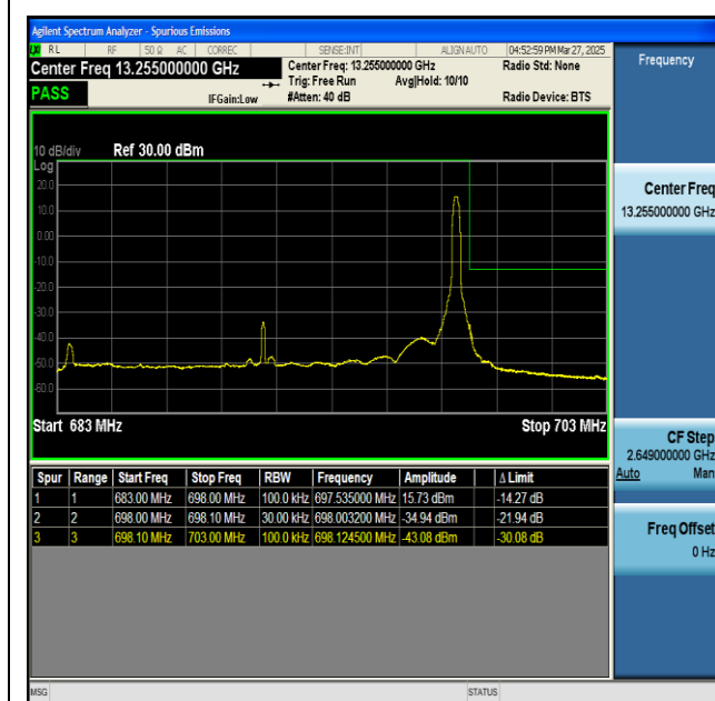
NTNV-n71-PC3-15-15-H-CP-QPSK-Edge_1RB_Right-PASS
