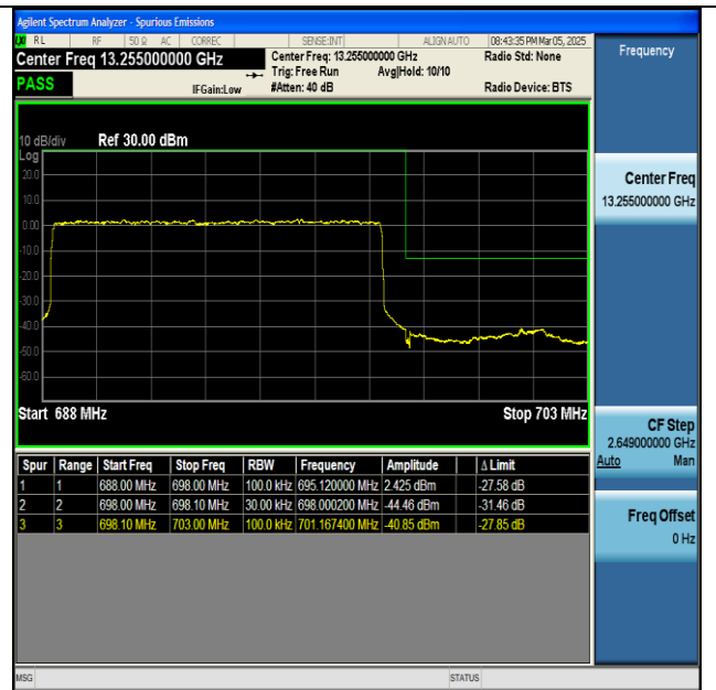
NTNV-n71-PC3-15-10-H-DFT-BPSK-Outer_Full-PASS
