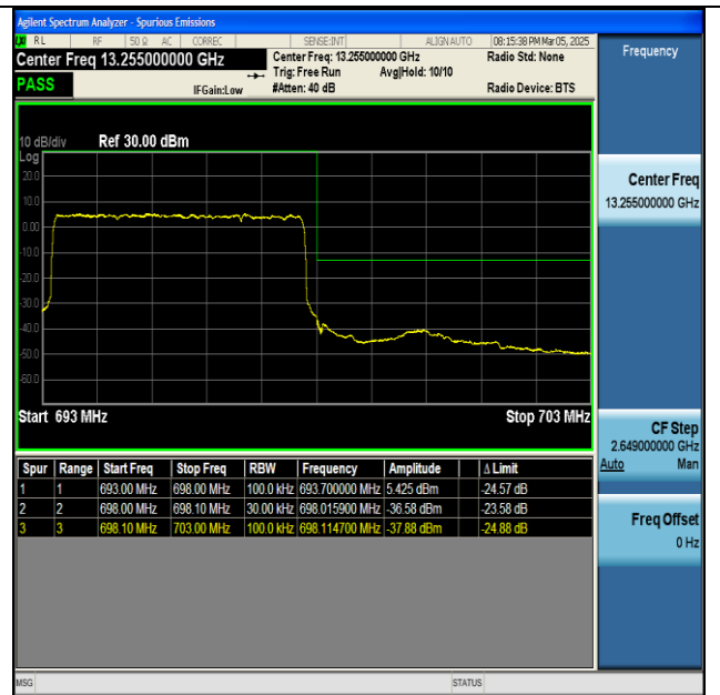
NTNV-n71-PC3-15-5-H-DFT-BPSK-Outer_Full-PASS
