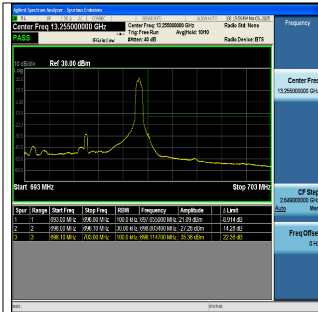
NTNV-n71-PC3-15-5-H-DFT-BPSK-Edge_1RB_Right-PASS
