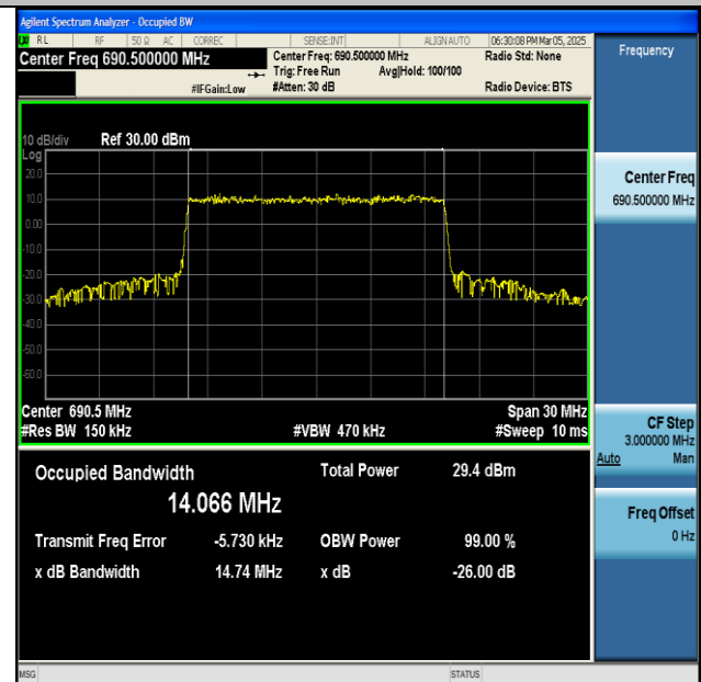
NTNV-n71-PC3-15-15-H-CP-64QAM-Outer_Full-Ant1-PASS
