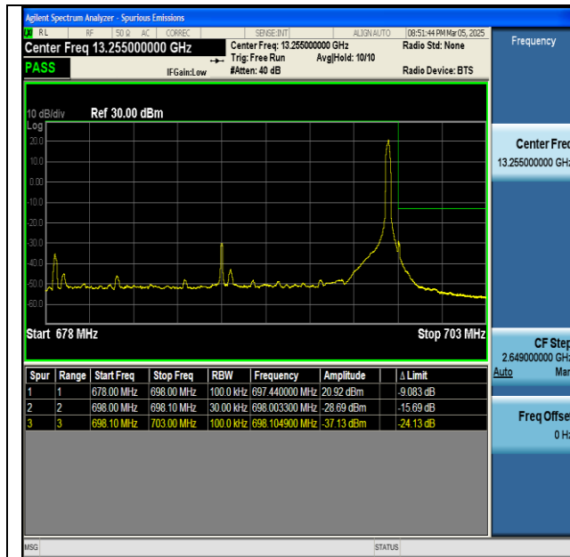
NTNV-n71-PC3-15-20-H-DFT-BPSK-Edge_1RB_Right-PASS
