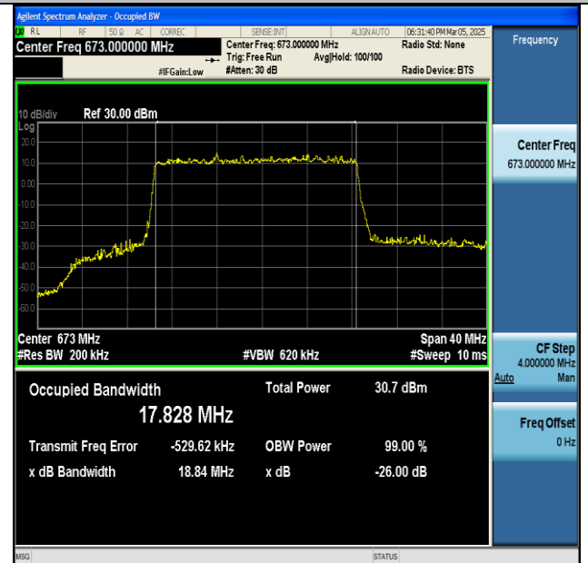
NTVN-n71-PC3-15-20-L-DFT-16QAM-Outer_Full-Ant1- PASS
