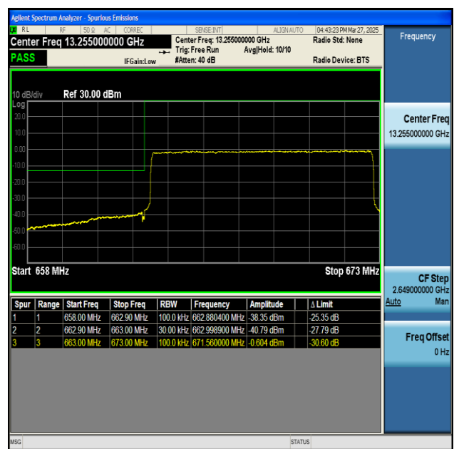
NTNV-n71-PC3-15-10-L-CP-QPSK-Outer_Full-PASS
