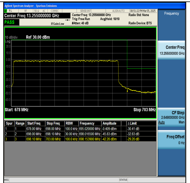
NTNV-n71-PC3-15-20-H-DFT-BPSK-Outer_Full-PASS
