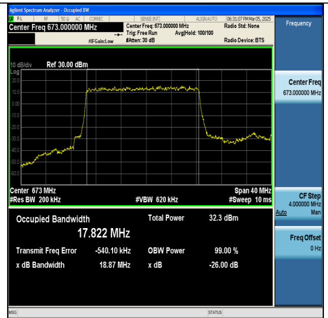
NTVN-n71-PC3-15-20-L-DFT-BPSK-Outer_Full-Ant1- PASS
