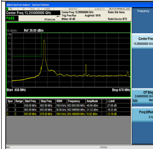
NTNV-n71-PC3-15-15-L-CP-QPSK-Edge_1RB_Left-PASS
