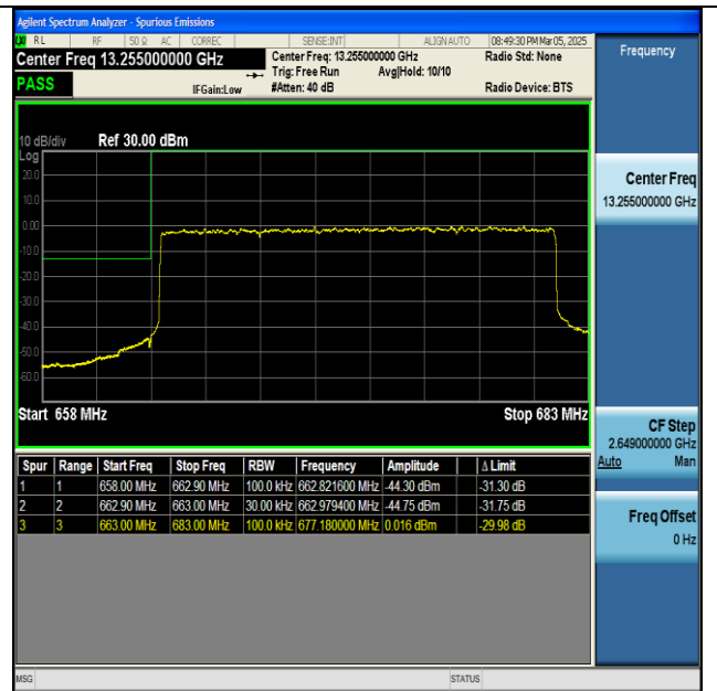
NTNV-n71-PC3-15-20-L-DFT-BPSK-Outer_Full-PASS
