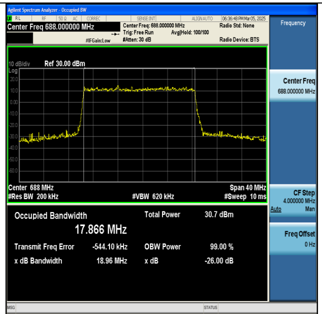
NTNV-n71-PC3-15-20-H-DFT-16QAM-Outer_Full-Ant1- PASS
