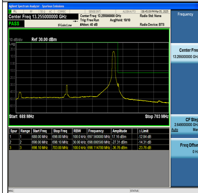
NTNV-n71-PC3-15-10-H-CP-QPSK-Edge_1RB_Right-PASS
