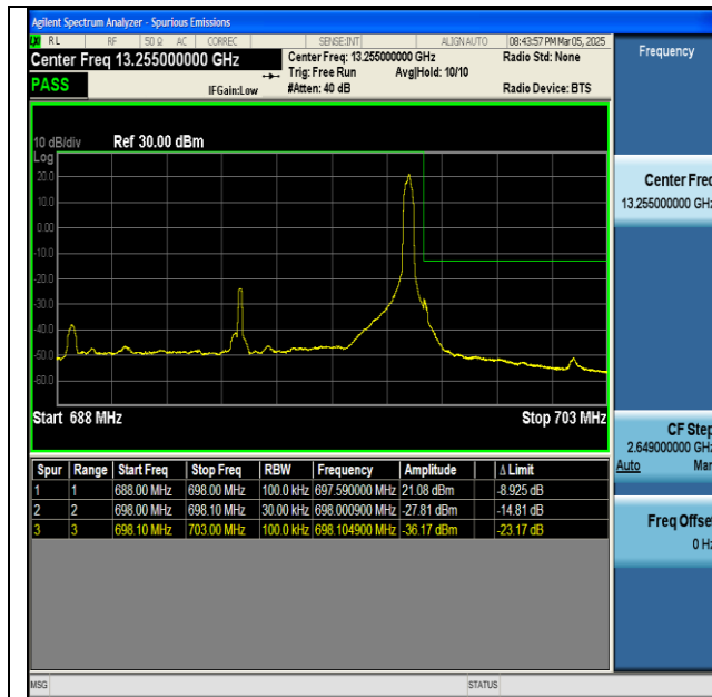
NTNV-n71-PC3-15-10-H-DFT-BPSK-Edge_1RB_Right-PASS
