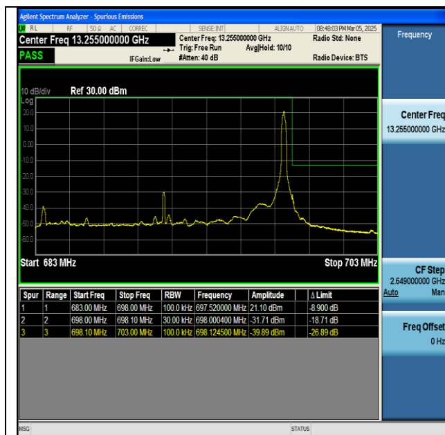
NTNV-n71-PC3-15-15-H-DFT-BPSK-Edge_1RB_Right-PASS
