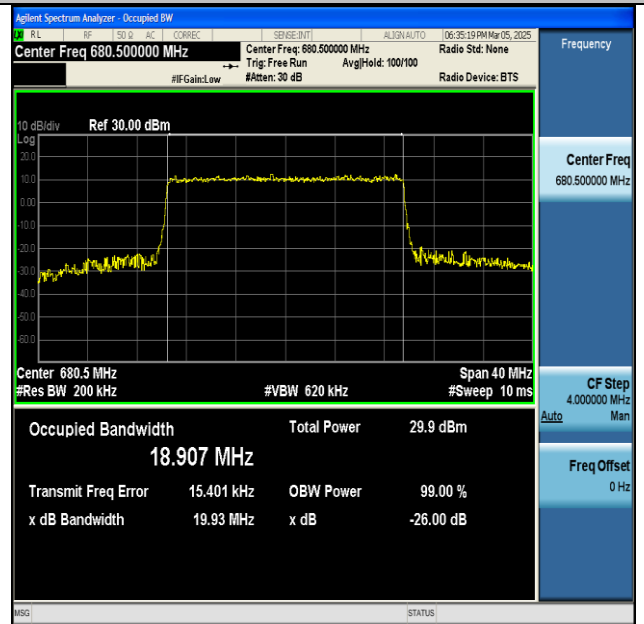
NTVN-n71-PC3-15-20-M-CP-QPSK-Outer_Full-Ant1-PASS
