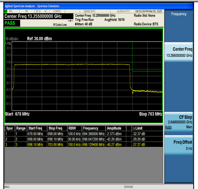
NTNV-n71-PC3-15-20-H-CP-QPSK-Outer_Full-PASS
