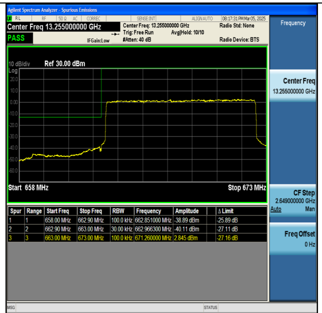
NTNV-n71-PC3-15-10-L-DFT-BPSK-Outer_Full-PASS
