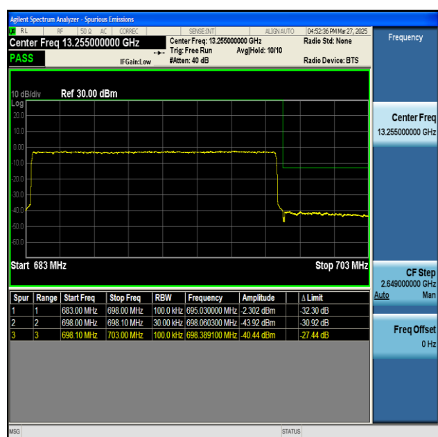
NTNV-n71-PC3-15-15-H-CP-QPSK-Outer_Full-PASS
