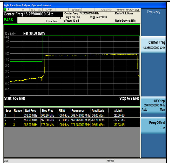
NTNV-n71-PC3-15-15-L-CP-QPSK-Outer_Full-PASS
