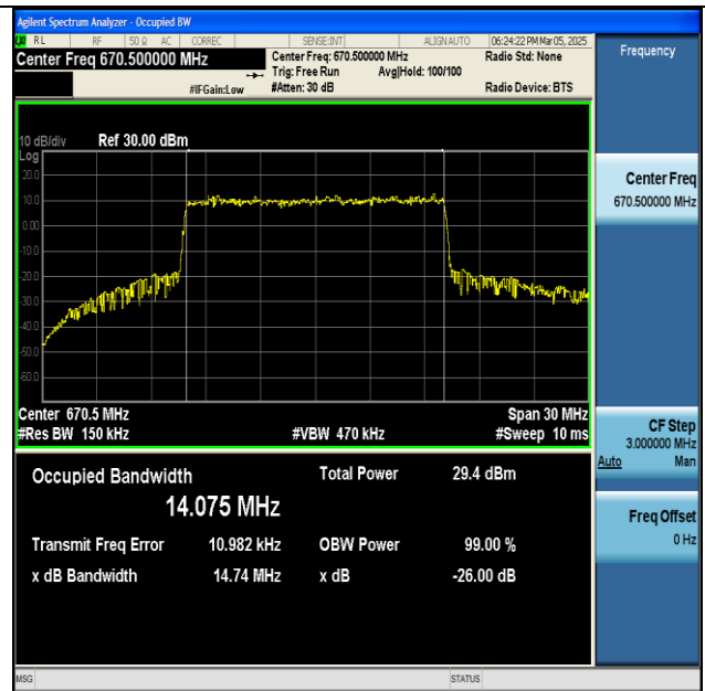
NTNV-n71-PC3-15-15-L-CP-64QAM-Outer_Full-Ant1- PASS
