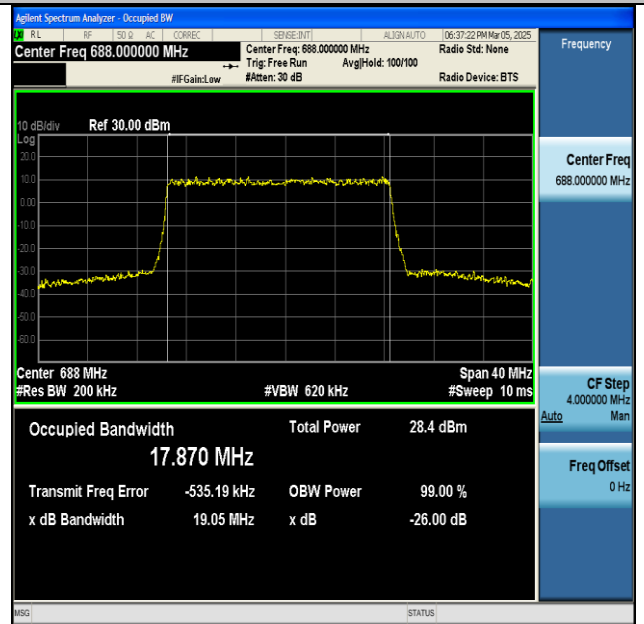
NTNV-n71-PC3-15-20-H-DFT-256QAM-Outer_Full-Ant1- PASS
