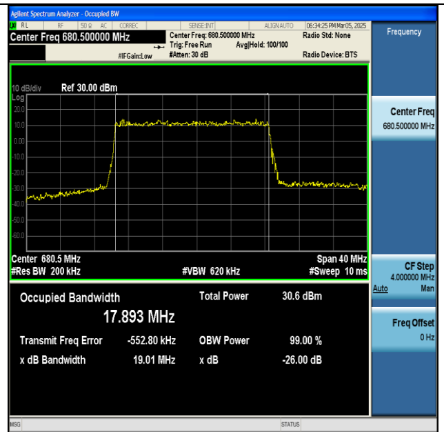
NTVN-n71-PC3-15-20-M-DFT-64QAM-Outer_Full-Ant1- PASS
