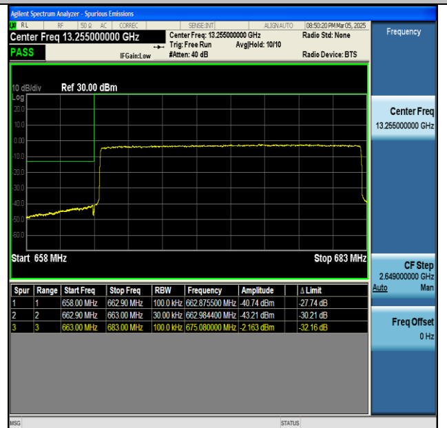
NTNV-n71-PC3-15-20-L-CP-QPSK-Outer_Full-PASS
