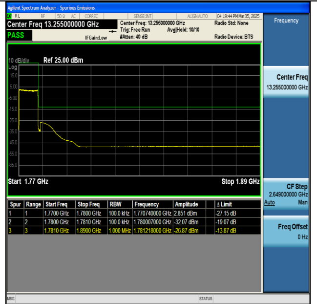
NTNV-n66-PC3-15-10-H-CP-QPSK-Outer_Full-PASS
