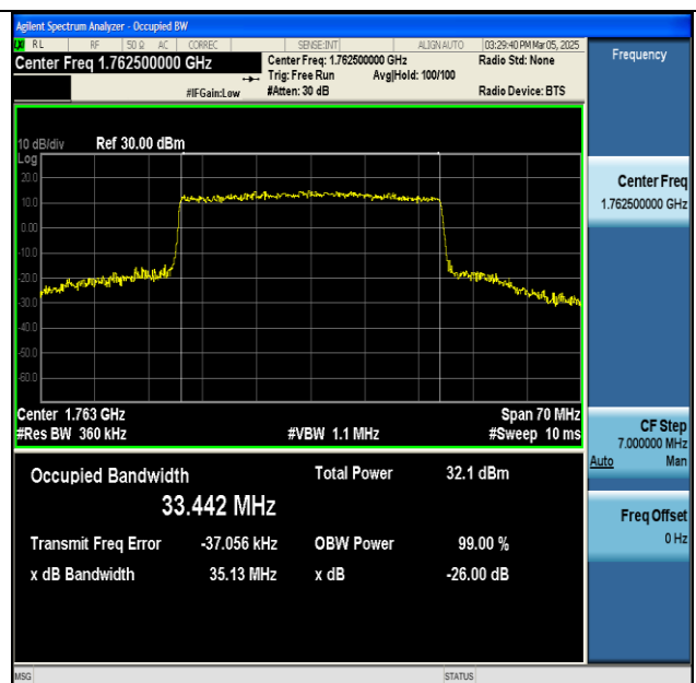
NTNV-n66-PC3-15-35-H-CP-QPSK-Outer_Full-Ant1-PASS
