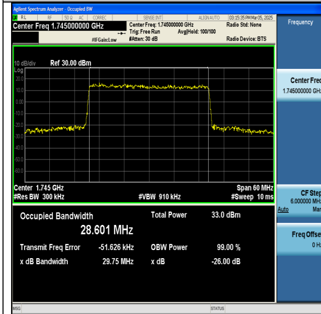
NTNV-n66-PC3-15-30-M-DFT-16QAM-Outer_Full-Ant1- PASS
