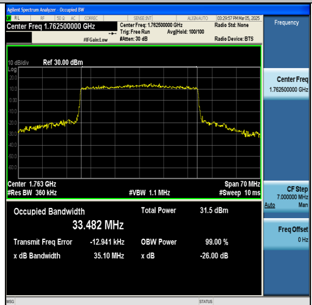
NTNV-n66-PC3-15-35-H-CP-64QAM-Outer_Full-Ant1-PASS
