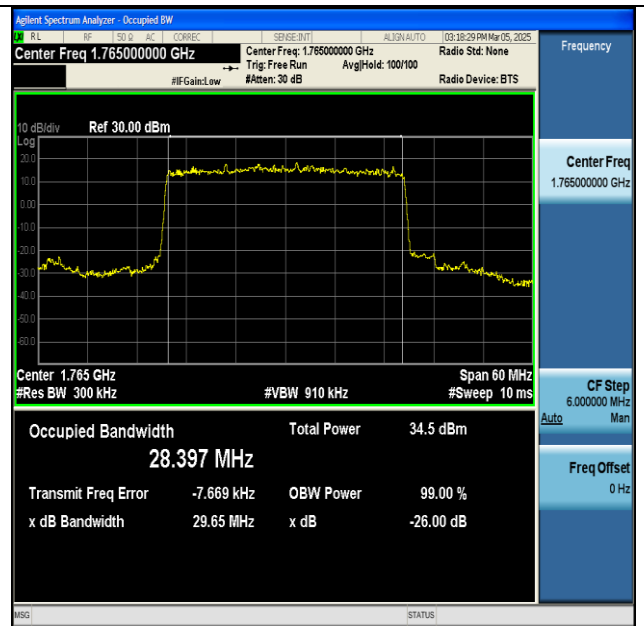
NTNV-n66-PC3-15-30-H-DFT-BPSK-Outer_Full-Ant1- PASS
