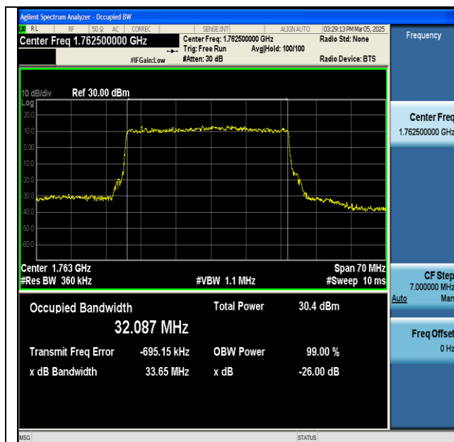
NTNV-n66-PC3-15-35-H-DFT-256QAM-Outer_Full-Ant1-PASS
