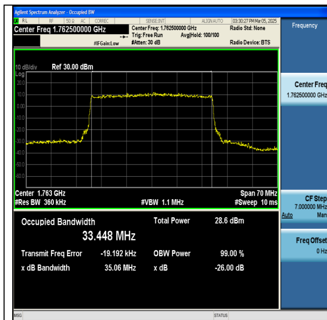
NTNV-n66-PC3-15-35-H-CP-256QAM-Outer_Full-Ant1- PASS
