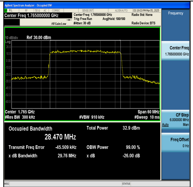
NTNV-n66-PC3-15-30-H-DFT-16QAM-Outer_Full-Ant1- PASS
