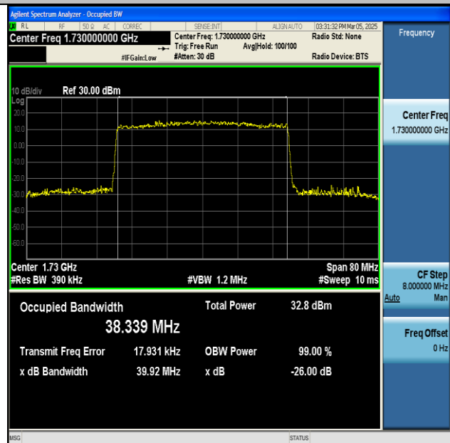
NTNV-n66-PC3-15-40-L-DFT-16QAM-Outer_Full-Ant1- PASS
