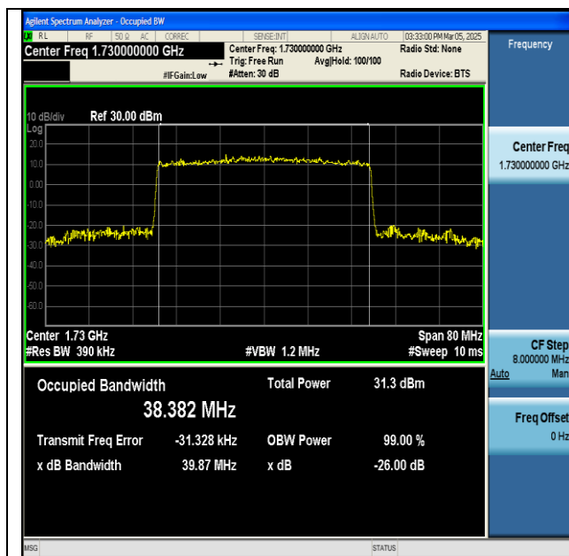
NTNV-n66-PC3-15-40-L-CP-64QAM-Outer_Full-Ant1-1 PASS
