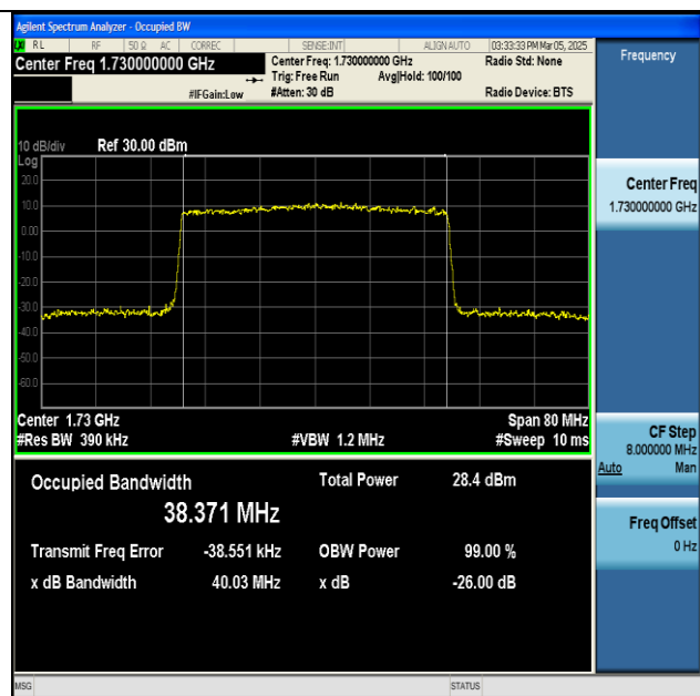
NTNV-n66-PC3-15-40-L-CP-256QAM-Outer_Full-Ant1-1 PASS
