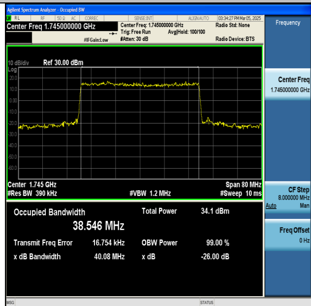
NTNV-n66-PC3-15-40-M-DFT-QPSK-Outer_Full-Ant1-1 PASS
