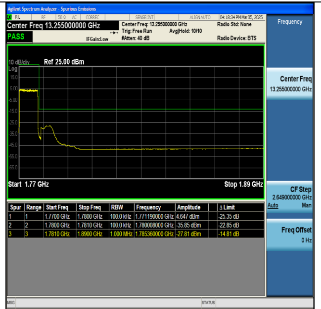
NTNV-n66-PC3-15-10-H-DFT-BPSK-Outer_Full-PASS
