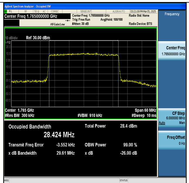
NTNV-n66-PC3-15-30-H-CP-256QAM-Outer_Full-Ant1- PASS
