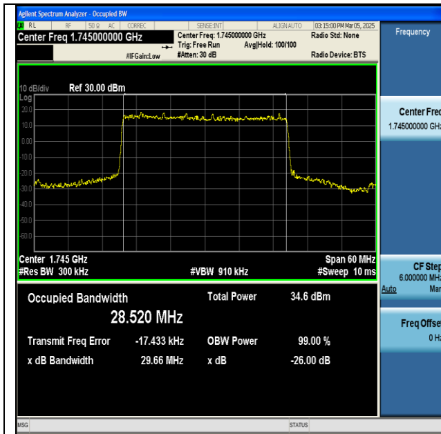
NTNV-n66-PC3-15-30-M-DFT-BPSK-Outer_Full-Ant1- PASS
