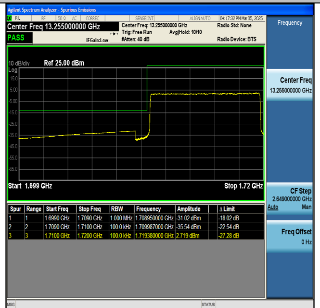
NTNV-n66-PC3-15-10-L-CP-QPSK-Outer_Full-PASS
