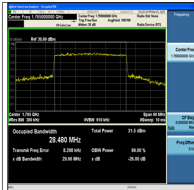
NTNV-n66-PC3-15-30-H-CP-64QAM-Outer_Full-Ant1- PASS
