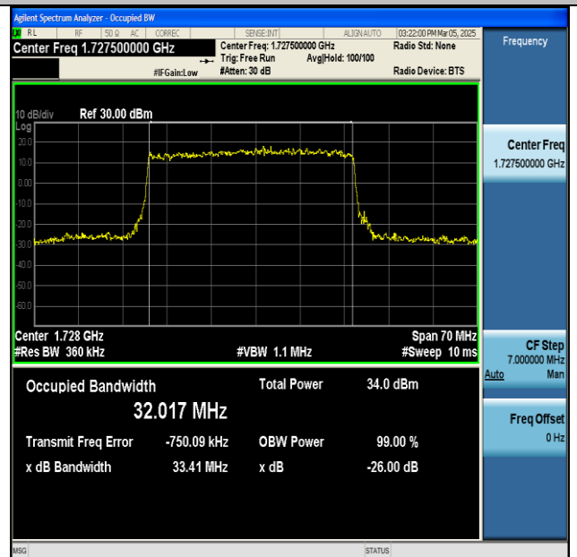
NTNV-n66-PC3-15-35-L-DFT-QPSK-Outer_Full-Ant1- PASS
