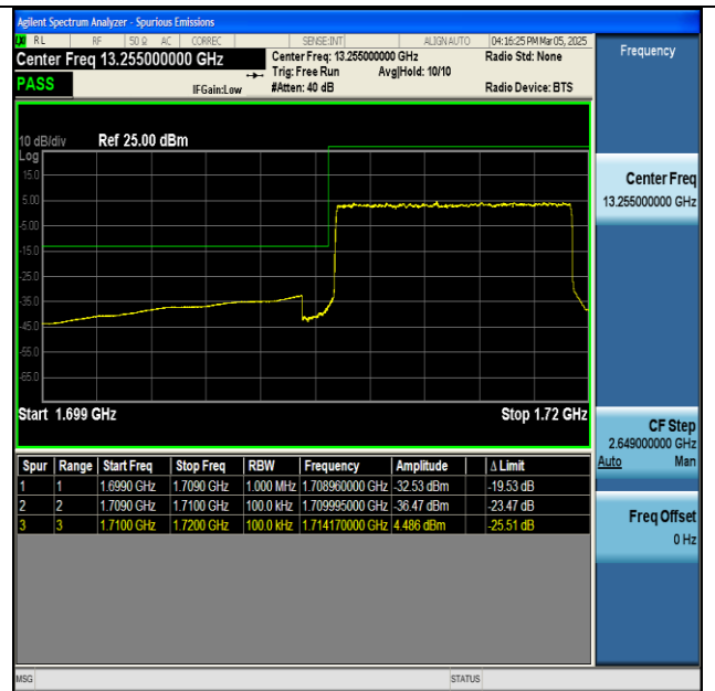
NTNV-n66-PC3-15-10-L-DFT-BPSK-Outer_Full-PASS
