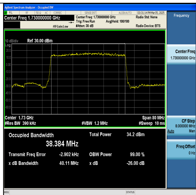
NTNV-n66-PC3-15-40-L-DFT-BPSK-Outer_Full-Ant1- PASS
