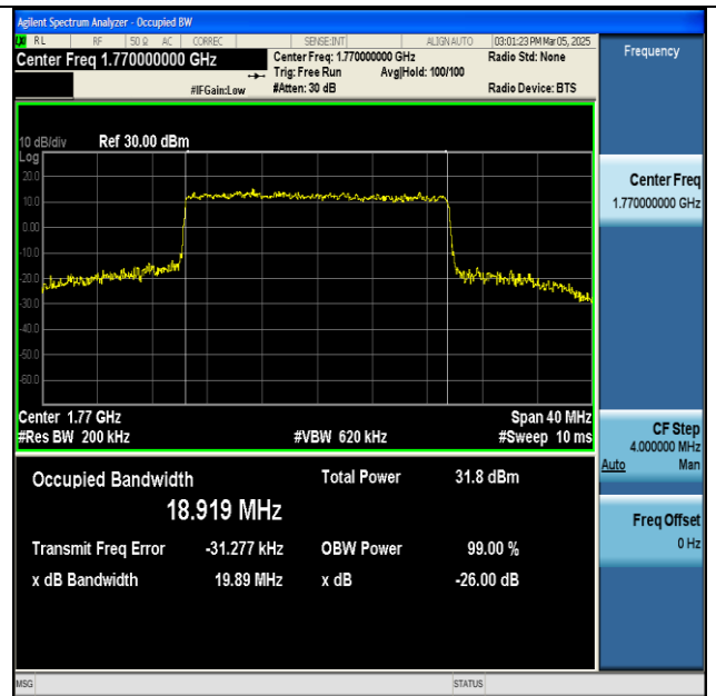
NTNV-n66-PC3-15-20-H-CP-16QAM-Outet_Full-Ant1-PASS
