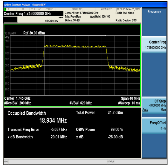
NTNV-n66-PC3-15-20-M-CP-64QAM-Outer_Full-Ant1- PASS
