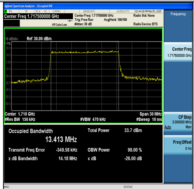
NTNV-n66-PC3-15-15-L-DFT-QPSK-Outer_Full-Ant1- PASS
