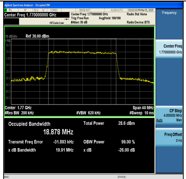
NTNV-n66-PC3-15-20-H-CP-256QAM-Outet_Full-Ant1-PASS
