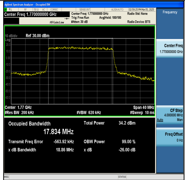
NTNV-n66-PC3-15-20-H-DFT-BPSK-Outer_Full-Ant1- PASS
