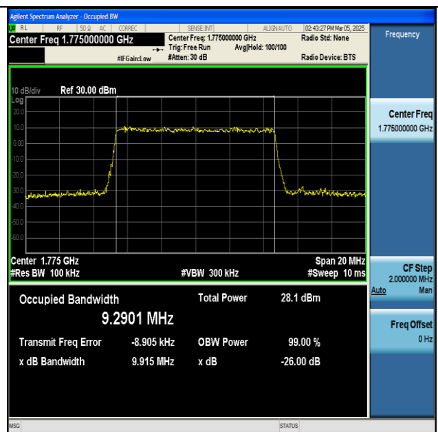
NTNV-n66-PC3-15-10-H-CP-256QAM-Outer_Full-Ant1- PASS
