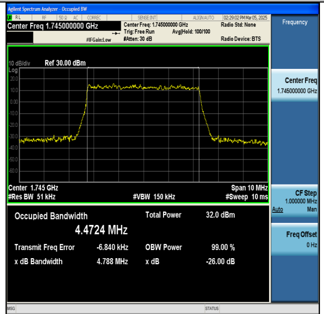
NTNV-n66-PC3-15-5-M-DFT-16QAM-Outer_Full-Ant1-PASS
