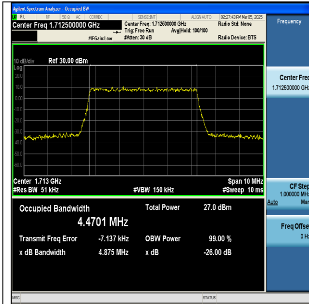
NTNV-n66-PC3-15-5-L-CP-256QAM-Outer_Full-Ant1-PASS
