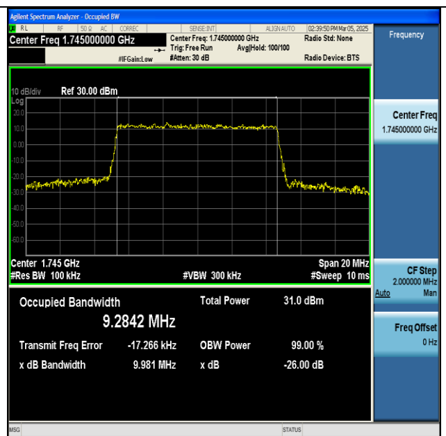
NTNV-n66-PC3-15-10-M-CP-QPSK-Outer_Full-Ant1-PASS
