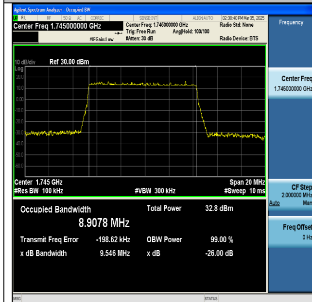
NTNV-n66-PC3-15-10-M-DFT-16QAM-Outer_Full-Ant1- PASS
