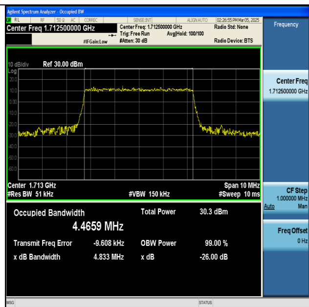
NTNV-n66-PC3-15-5-L-CP-QPSK-Outer_Full-Ant1-PASS
