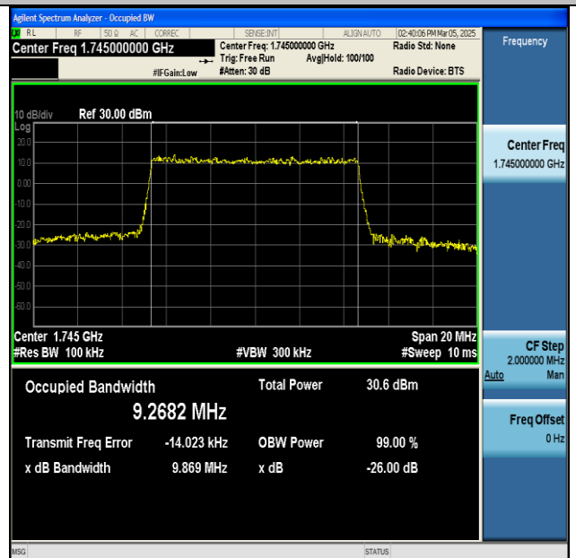
NTNV-n66-PC3-15-10-M-CP-64QAM-Outer_Full-Ant1-PASS
