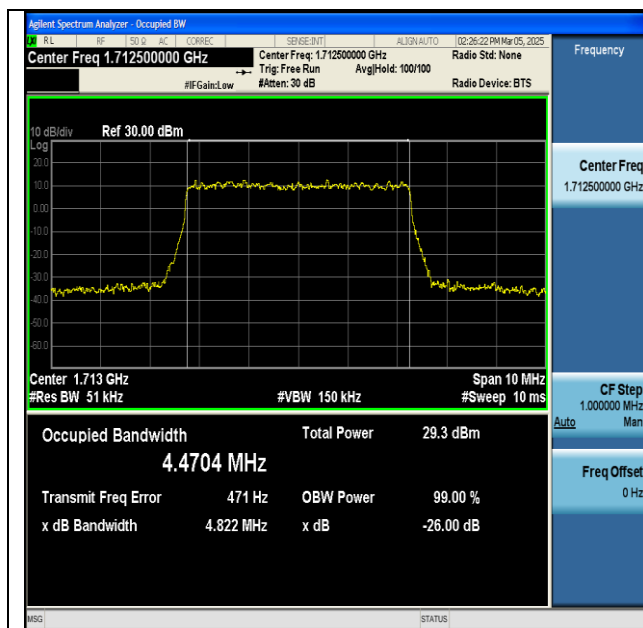
NTNV-n66-PC3-15-5-L-DFT-256QAM-Outer_Full-Ant1-PASS
