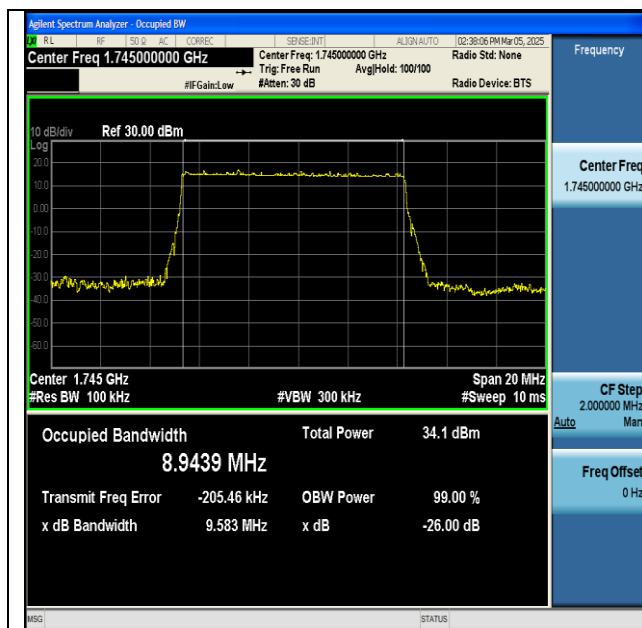
NTNV-n66-PC3-15-10-M-DFT-BPSK-Outer_Full-Ant1- PASS
