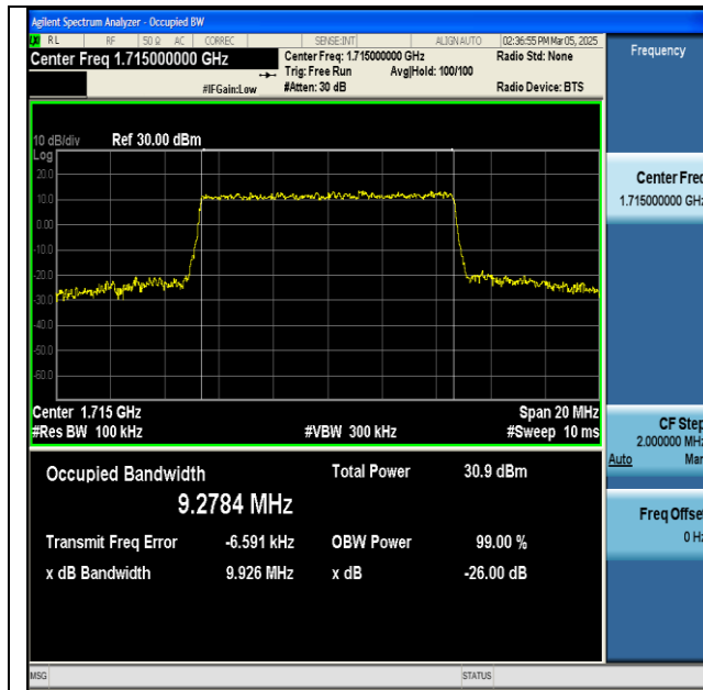
NTNV-n66-PC3-15-10-L-CP-QPSK-Outer_Full-Ant1-PASS
