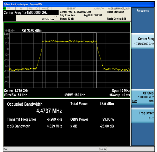
NTNV-n66-PC3-15-5-M-DFT-BPSK-Outer_Full-Ant1-PASS
