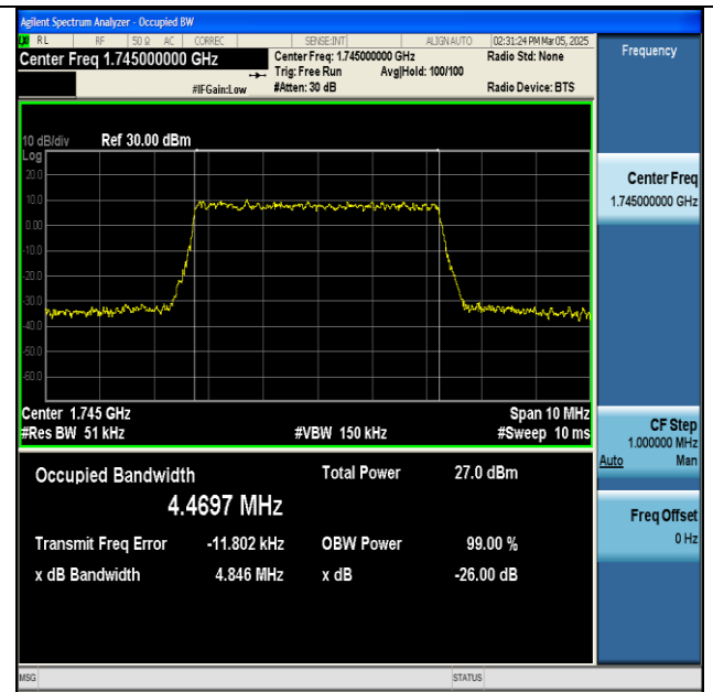
NTNV-n66-PC3-15-5-M-CP-256QAM-Outer_Full-Ant1-PASS
