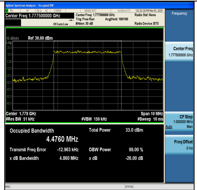
NTNV-n66-PC3-15-5-H-DFT-QPSK-Outer_Full-Ant1-PASS
