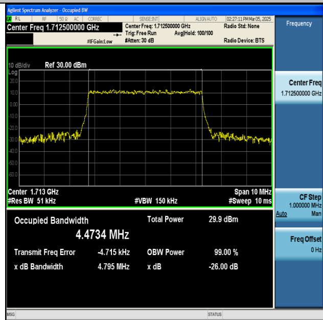
NTNV-n66-PC3-15-5-L-CP-64QAM-Outer_Full-Ant1-PASS
