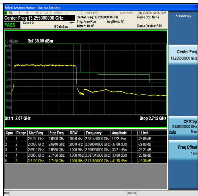
NTNV-n41-PC2-30-20-H-DFT-BPSK-Outer_Full-PASS
