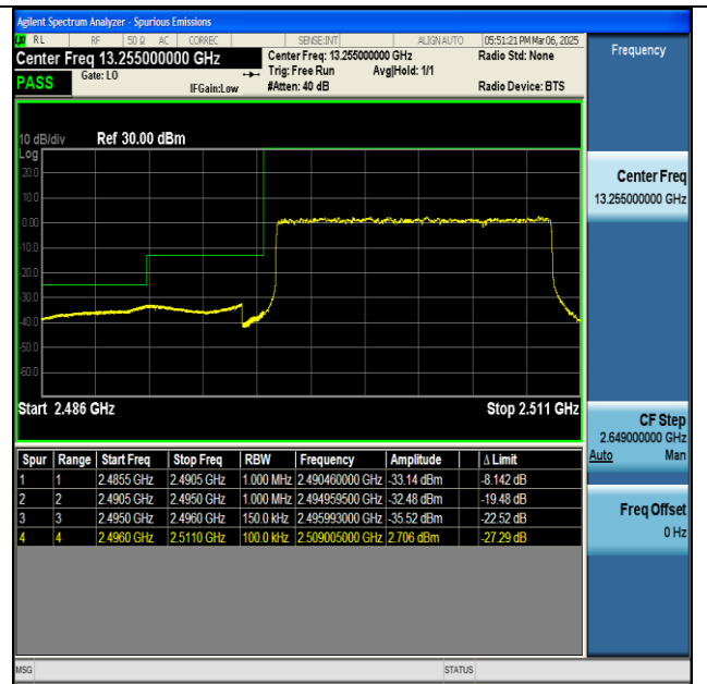
NTNV-n41-PC2-30-15-L-DFT-BPSK-Outer_Full-PASS
