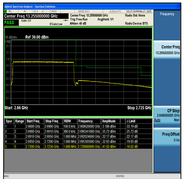
NTNV-n41-PC2-30-30-H-CP-QPSK-Outer_Full-PASS
