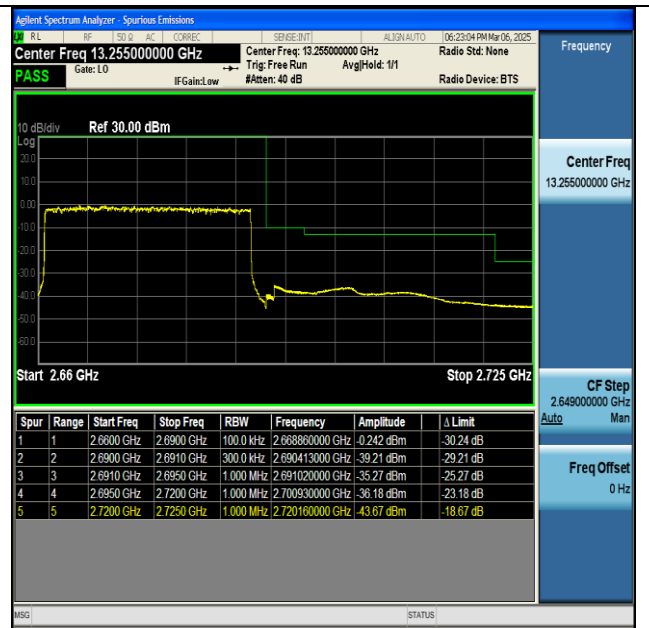
NTNV-n41-PC2-30-30-H-DFT-BPSK-Outer_Full-PASS
