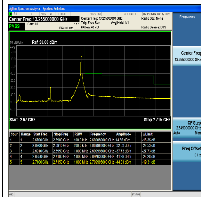
NTNV-n41-PC2-30-20-H-CP-QPSK-Edge_1RB_Right-PASS
