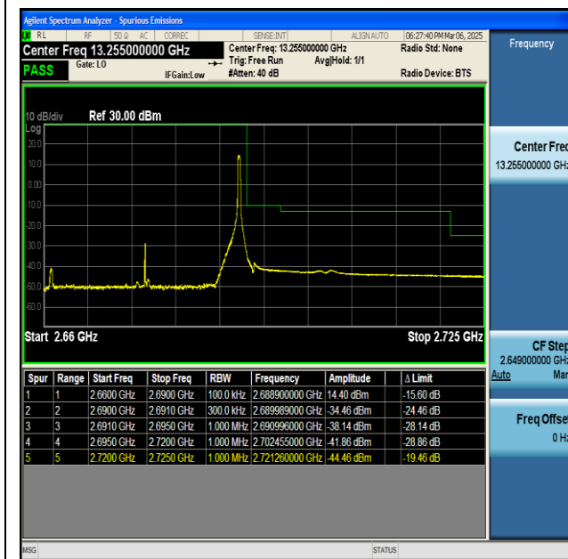
NTNV-n41-PC2-30-30-H-CP-QPSK-Edge_1RB_Right-PASS
