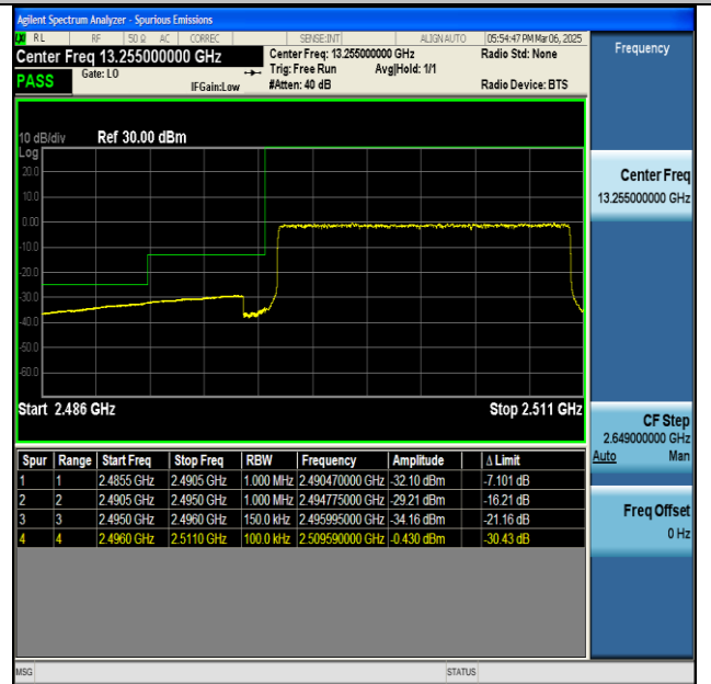
NTNV-n41-PC2-30-15-L-CP-QPSK-Outer_Full-PASS
