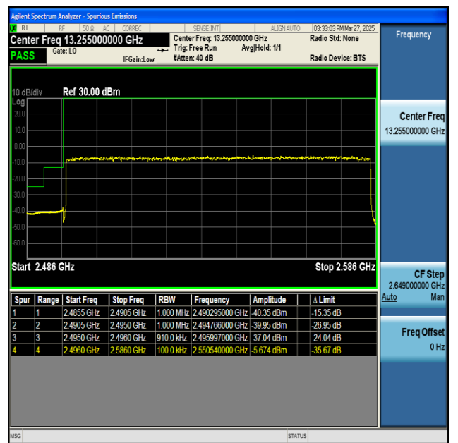
NTNV-n41-PC2-30-90-L-CP-QPSK-Outer_Full-PASS
