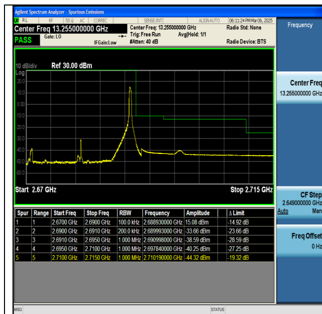
NTNV-n41-PC2-30-20-H-DFT-BPSK-Edge_1RB_Right-PASS
