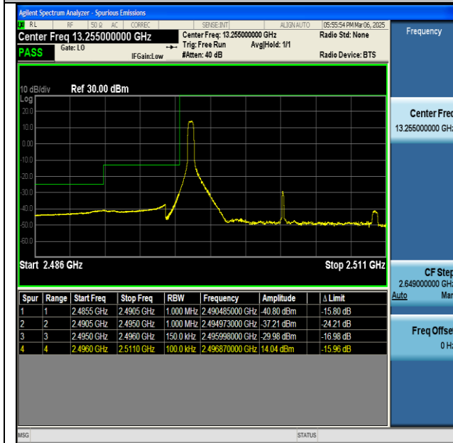
NTNV-n41-PC2-30-15-L-CP-QPSK-Edge_1RB_Left-PASS
