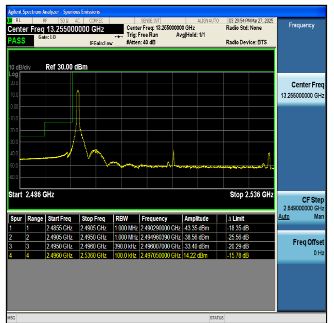
NTNV-n41-PC2-30-40-L-CP-QPSK-Outer_Full-PASS
