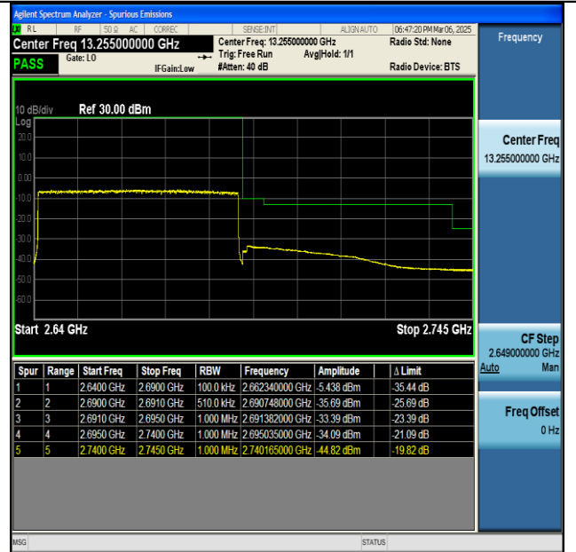
NTNV-n41-PC2-30-50-H-CP-QPSK-Outer_Full-PASS
