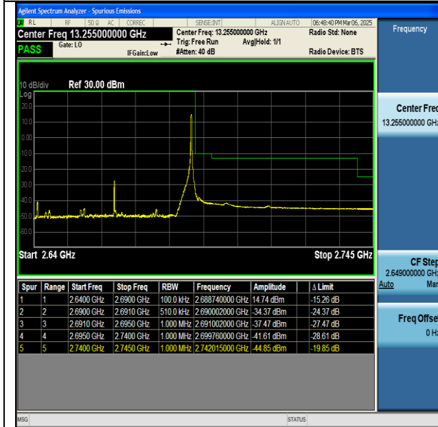
NTNV-n41-PC2-30-50-H-CP-QPSK-Edge_1RB_Right-PASS
