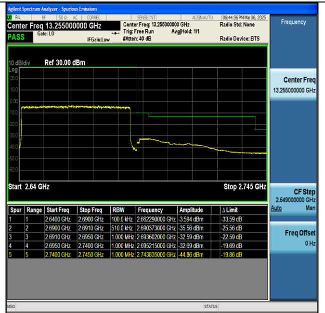
NTNV-n41-PC2-30-50-H-DFT-BPSK-Outer_Full-PASS
