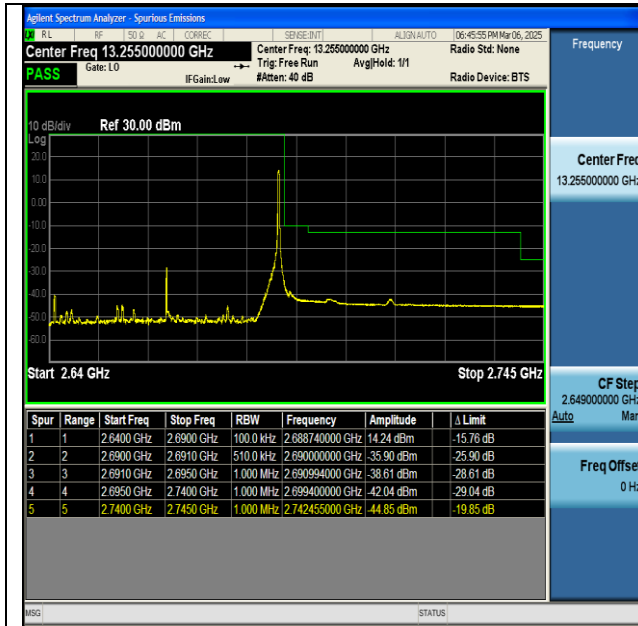
NTNV-n41-PC2-30-50-H-DFT-BPSK-Edge_1RB_Right-PASS
