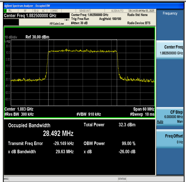
NTNV-n25-PC3-15-30-M-DFT-64QAM-Outer_Full-Ant1- PASS
