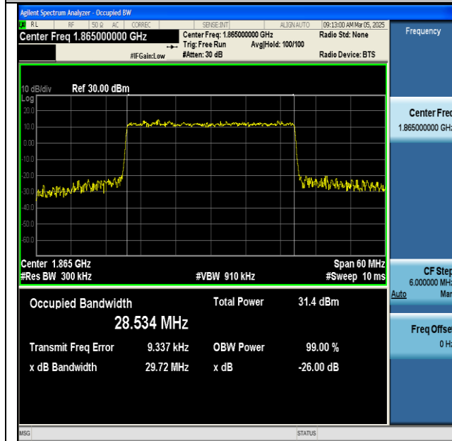
NTNV-n25-PC3-15-30-L-CP-64QAM-Outer_Full-Ant1-PASS
