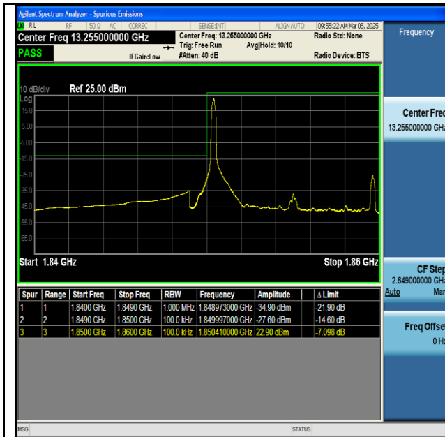
NTNV-n25-PC3-15-10-L-DFT-BPSK-Edge_1RB_Left-PASS
