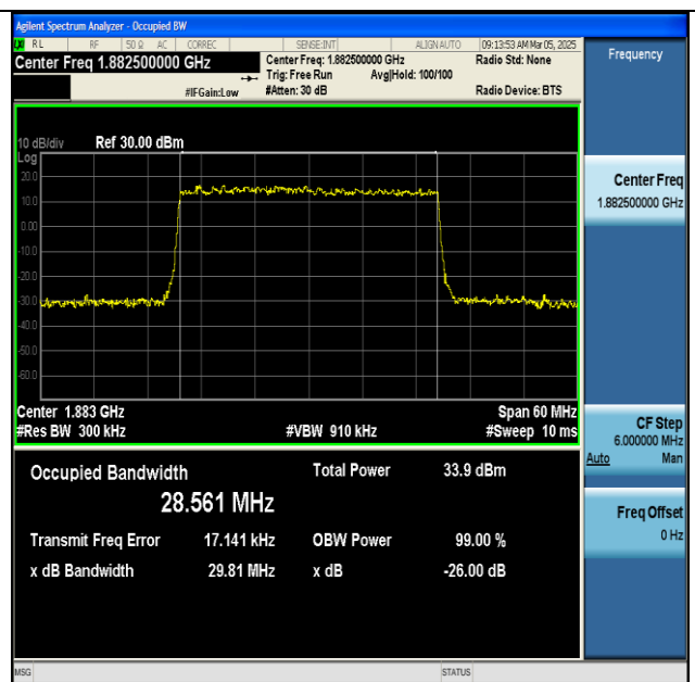
NTNV-n25-PC3-15-30-M-DFT-QPSK-Outer_Full-Ant1- PASS
