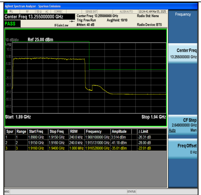
NTNV-n25-PC3-15-25-H-DFT-BPSK-Outer_Full-PASS
