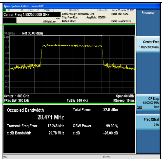
NTNV-n25-PC3-15-30-M-CP-QPSK-Outer_Full-Ant1-PASS
