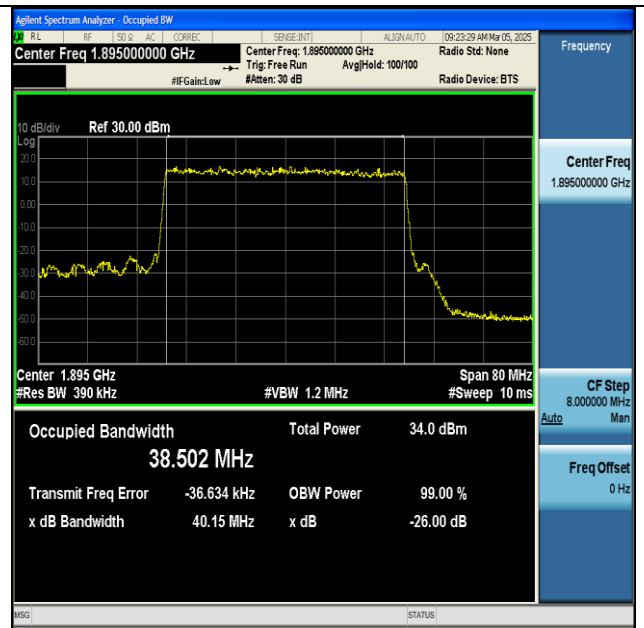
NTNV-n25-PC3-15-40-H-DFT-QPSK-Outer_Full-Ant1- PASS
