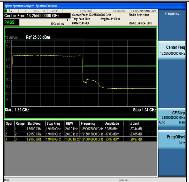
NTNV-n25-PC3-15-25-H-CP-QPSK-Outer_Full-PASS
