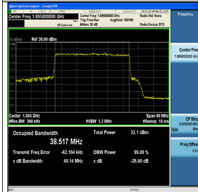
NTNV-n25-PC3-15-40-H-CP-16QAM-Outer_Full-Ant1-PASS
