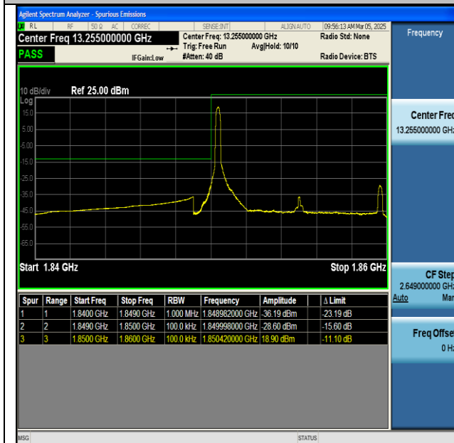
NTNV-n25-PC3-15-10-L-CP-QPSK-Edge_1RB_Left-PASS
