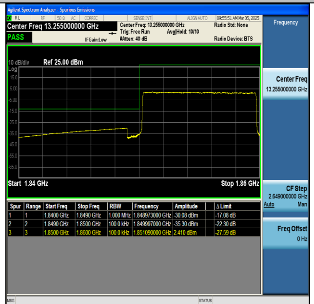
NTNV-n25-PC3-15-10-L-CP-QPSK-Outer_Full-PASS
