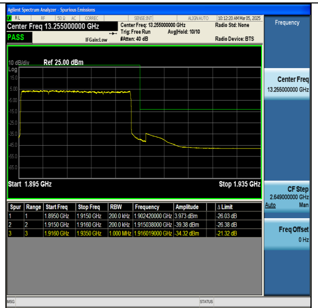
NTNV-n25-PC3-15-20-H-DFT-BPSK-Outer_Full-PASS
