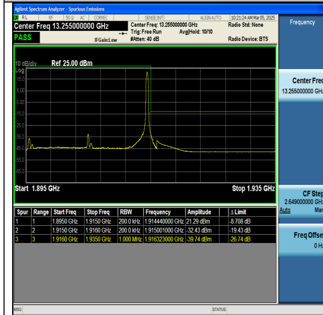
NTNV-n25-PC3-15-20-H-CP-QPSK-Edge_1RB_Right-PASS
