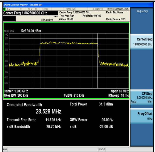
NTNV-n25-PC3-15-30-M-CP-64QAM-Outer_Full-Ant1-PASS
