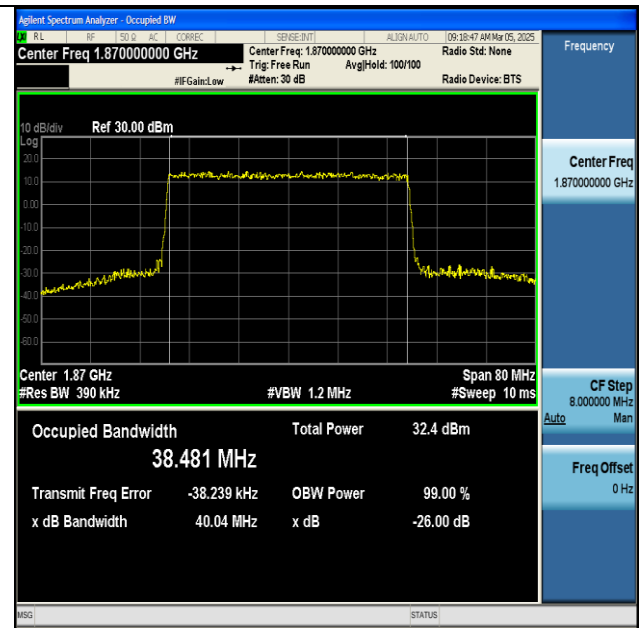
NTNV-n25-PC3-15-40-L-DFT-64QAM-Outer_Full-Ant1- PASS
