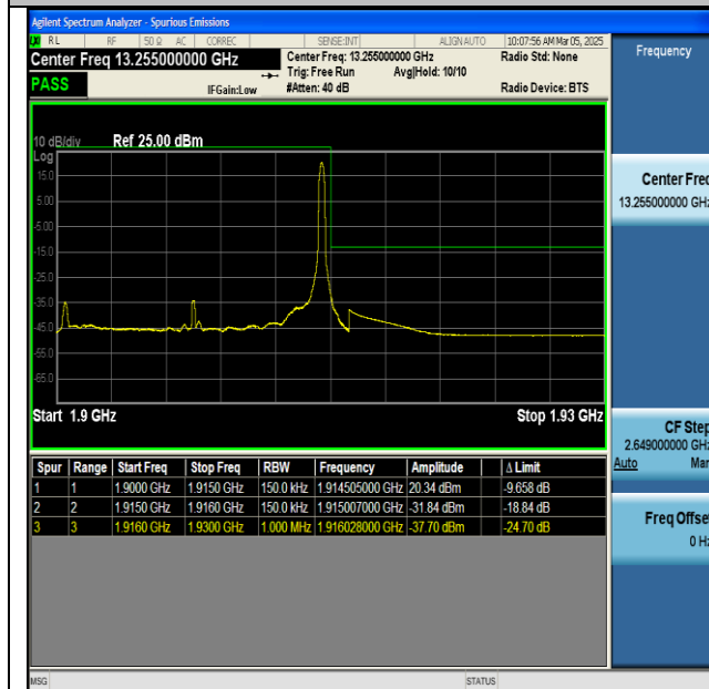
NTNV-n25-PC3-15-15-H-CP-QPSK-Edge_1RB_Right-PASS
