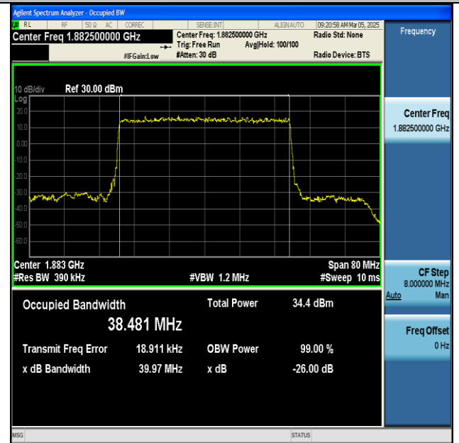
NTNV-n25-PC3-15-40-M-DFT-BPSK-Outer_Full-Ant1- PASS
