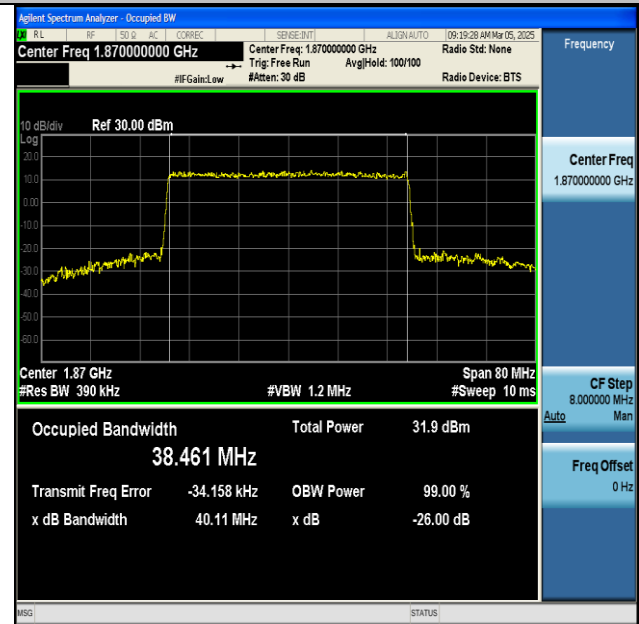
NTNV-n25-PC3-15-40-L-CP-QPSK-Outer_Full-Ant1-PASS
