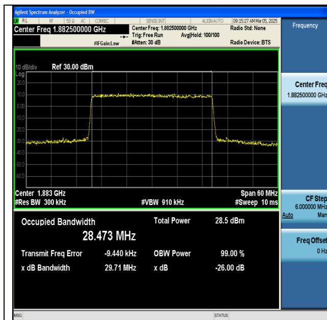
NTNV-n25-PC3-15-30-M-CP-256QAM-Outer_Full-Ant1- PASS
