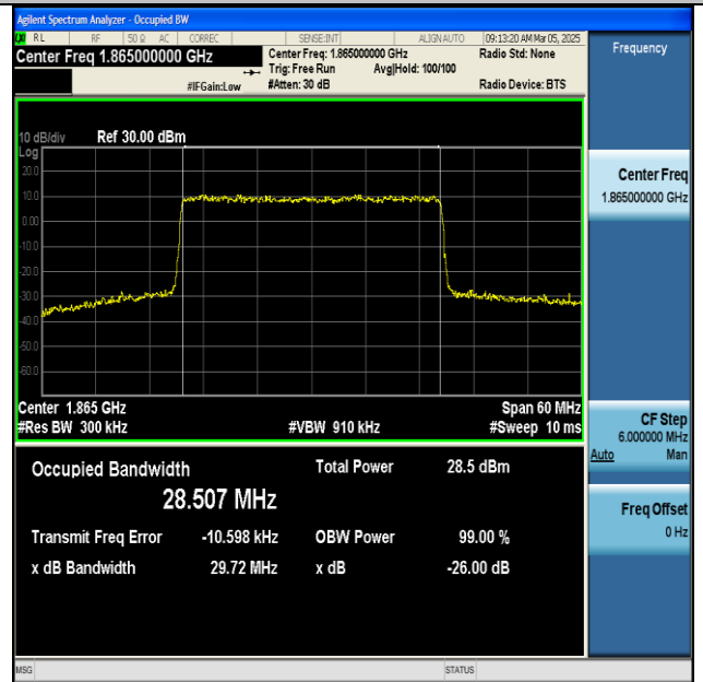
NTNV-n25-PC3-15-30-L-CP-256QAM-Outer_Full-Ant1-PASS
