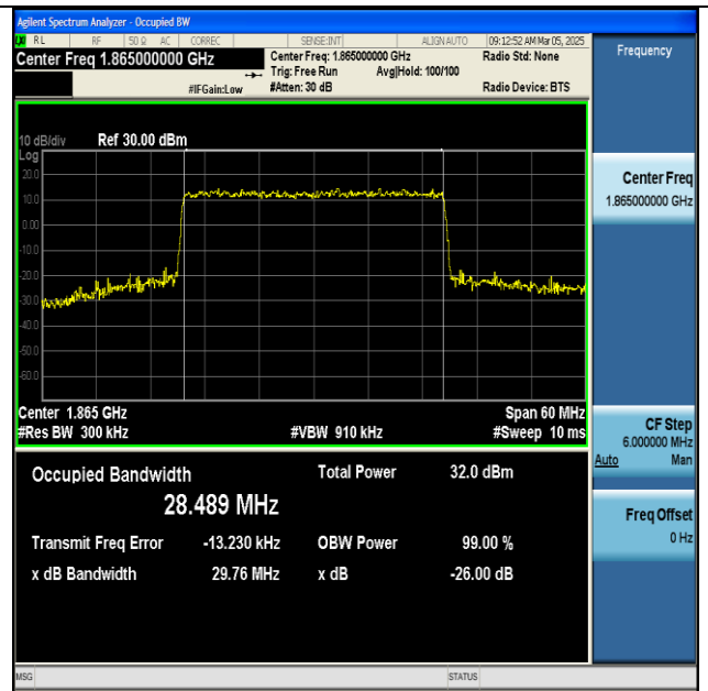
NTNV-n25-PC3-15-30-L-CP-16QAM-Outer_Full-Ant1-PASS
