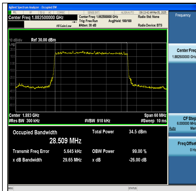
NTNV-n25-PC3-15-30-M-DFT-BPSK-Outer_Full-Ant1- PASS
