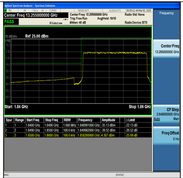
NTNV-n25-PC3-15-10-L-DFT-BPSK-Outer_Full-PASS
