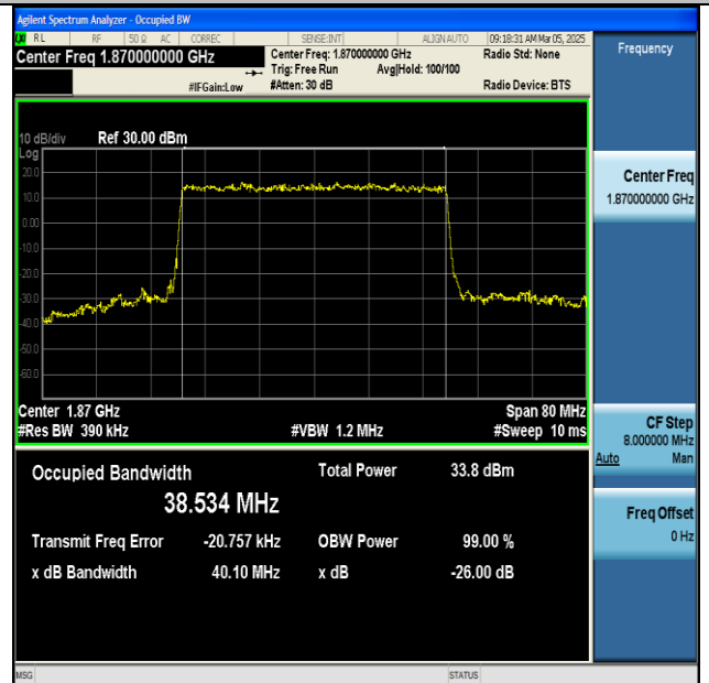
NTNV-n25-PC3-15-40-L-DFT-QPSK-Outer_Full-Ant1- PASS
