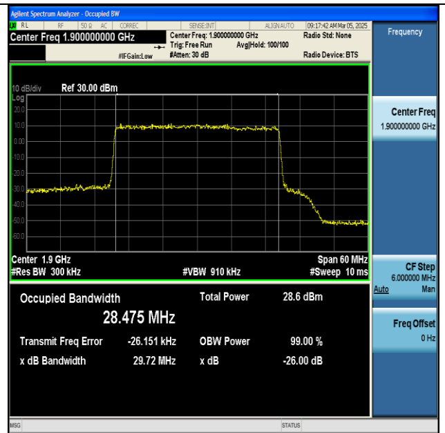
NTNV-n25-PC3-15-30-H-CP-256QAM-Outer_Full-Ant1- PASS
