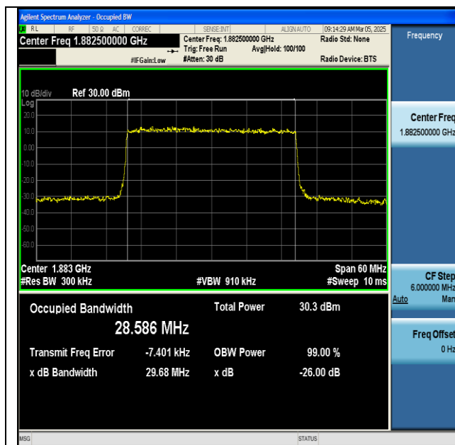
NTNV-n25-PC3-15-30-M-DFT-256QAM-Outer_Full-Ant1-PASS
