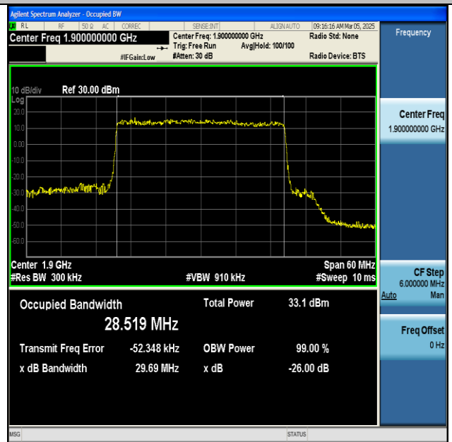
NTNV-n25-PC3-15-30-H-DFT-16QAM-Outer_Full-Ant1- PASS
