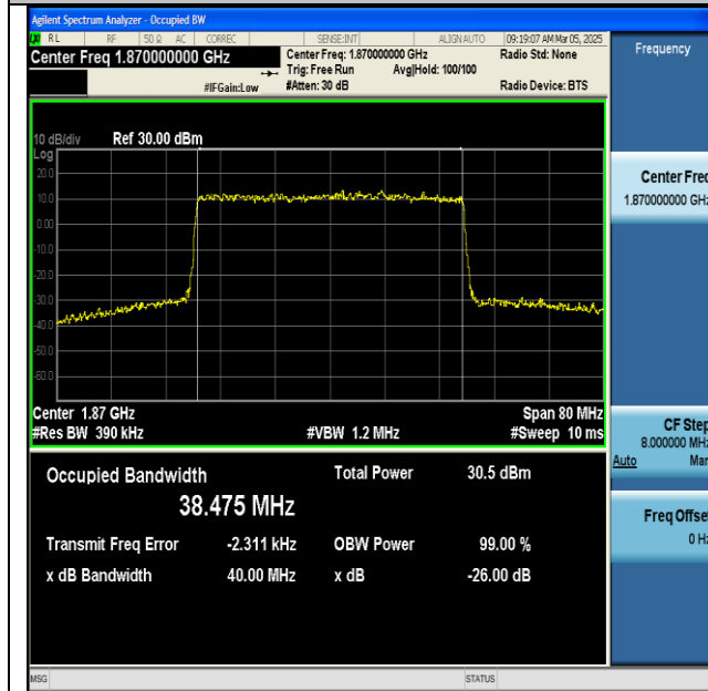
NTNV-n25-PC3-15-40-L-DFT-256QAM-Outer_Full-Ant1- PASS
