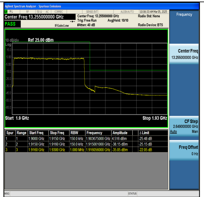
NTNV-n25-PC3-15-15-H-DFT-BPSK-Outer_Full-PASS
