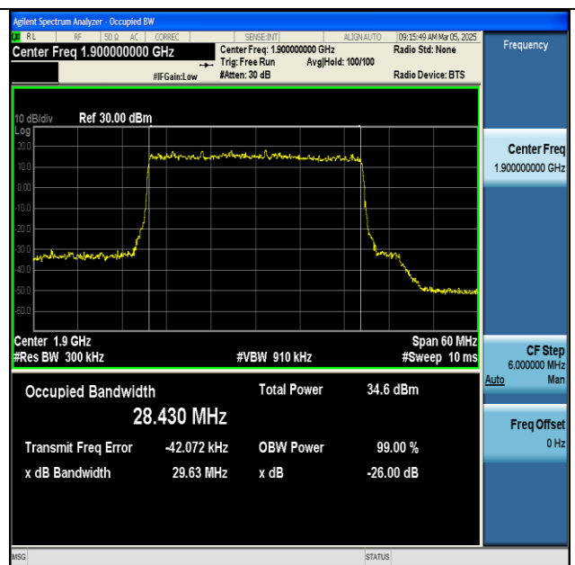
NTNV-n25-PC3-15-30-H-DFT-BPSK-Outer_Full-Ant1- PASS
