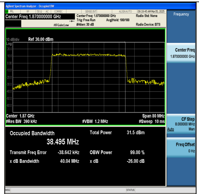
NTNV-n25-PC3-15-40-L-CP-64QAM-Outer_Full-Ant1- PASS
