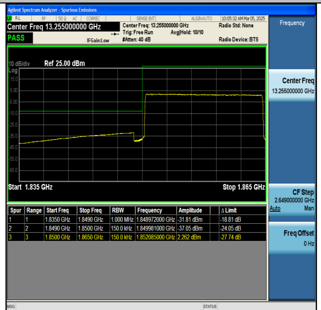
NTNV-n25-PC3-15-15-L-CP-QPSK-Outer_Full-PASS
