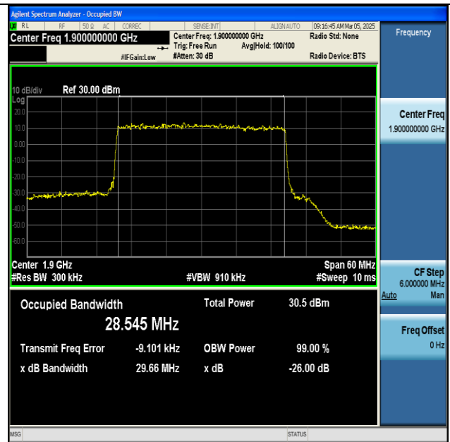
NTNV-n25-PC3-15-30-H-DFT-256QAM-Outer_Full-Ant1- PASS
