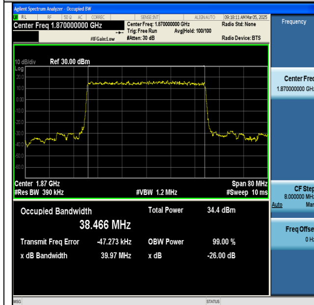
NTNV-n25-PC3-15-40-L-DFT-BPSK-Outer_Full-Ant1- PASS
