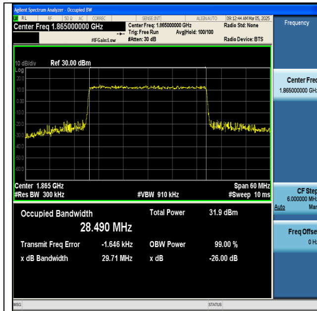
NTNV-n25-PC3-15-30-L-CP-QPSK-Outer_Full-Ant1-PASS
