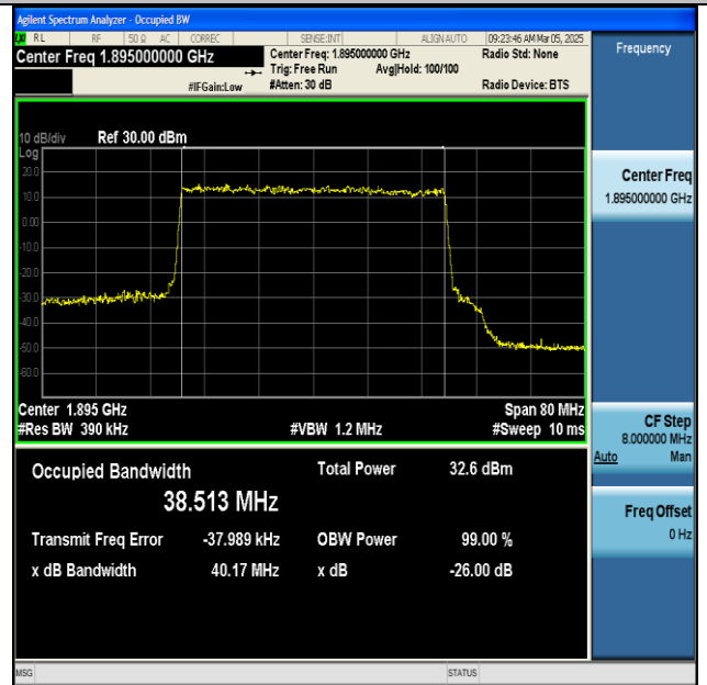
NTNV-n25-PC3-15-40-H-DFT-64QAM-Outer_Full-Ant1- PASS
