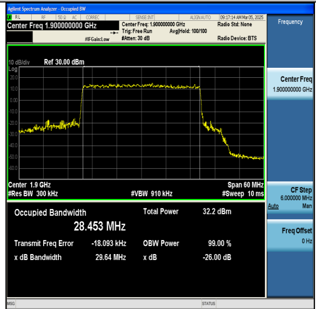
NTNV-n25-PC3-15-30-H-CP-16QAM-Outer_Full-Ant1- PASS
