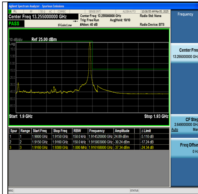
NTNV-n25-PC3-15-15-H-DFT-BPSK-Edge_1RB_Right-PASS
