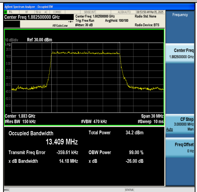
NTNV-n25-PC3-15-15-M-DFT-BPSK-Outer_Full-Ant1- PASS
