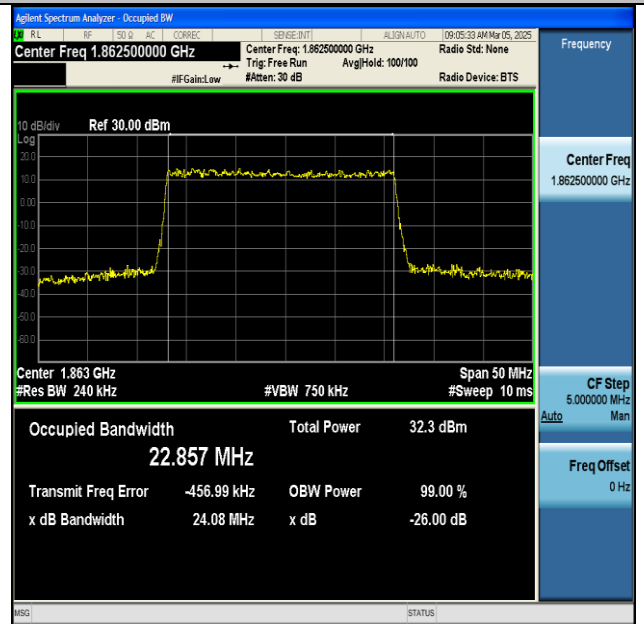
NTNV-n25-PC3-15-25-L-DFT-64QAM-Outer_Full-Ant1- PASS
