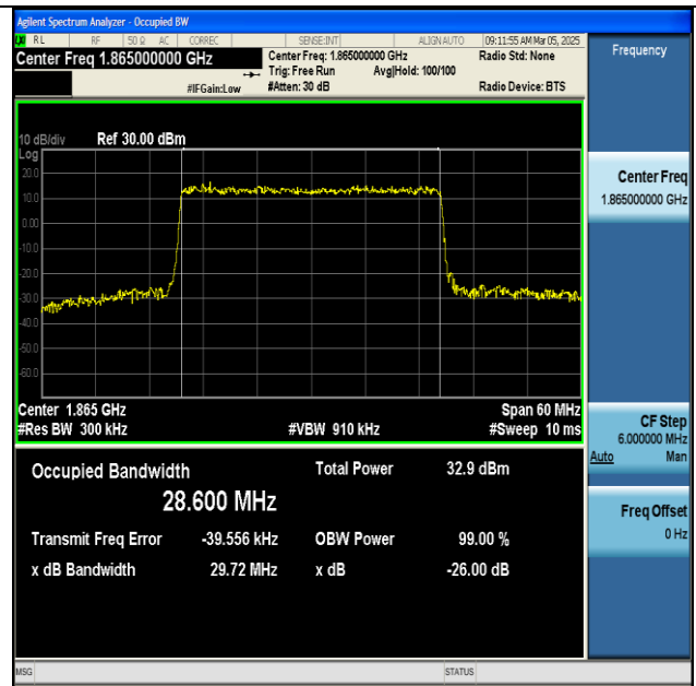
NTNV-n25-PC3-15-30-L-DFT-16QAM-Outer_Full-Ant1- PASS
