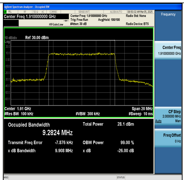
NTNV-n25-PC3-15-10-H-CP-256QAM-Outer_Full-Ant1- PASS
