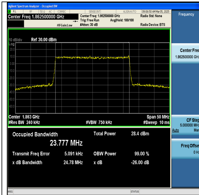
NTNV-n25-PC3-15-25-L-CP-256QAM-Outer_Full-Ant1- PASS
