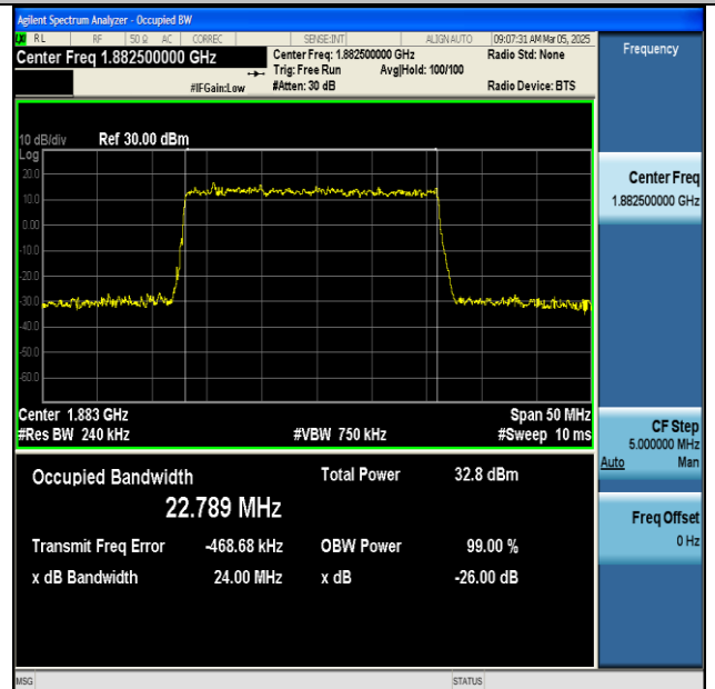
NTNV-n25-PC3-15-25-M-DFT-16QAM-Outer_Full-Ant1- PASS
