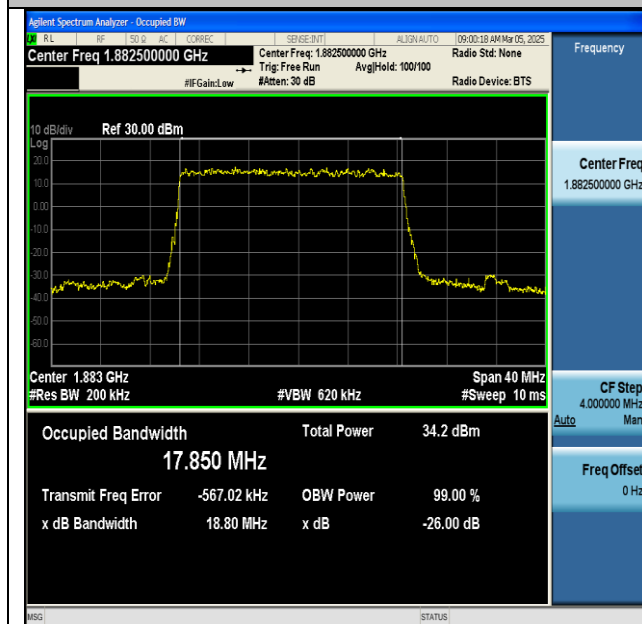
NTNV-n25-PC3-15-20-M-DFT-BPSK-Outer_Full-Ant1- PASS
