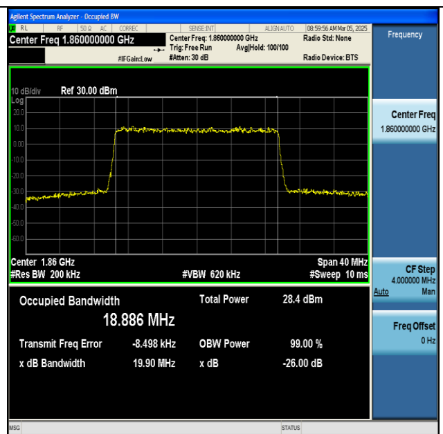
NTNV-n25-PC3-15-20-L-CP-256QAM-Outer_Full-Ant1- PASS
