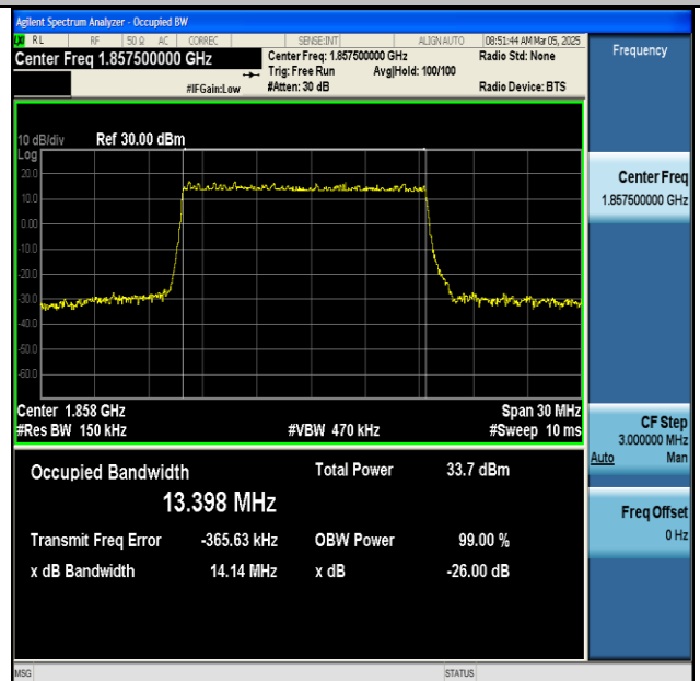
NTNV-n25-PC3-15-15-L-DFT-QPSK-Outer_Full-Ant1- PASS
