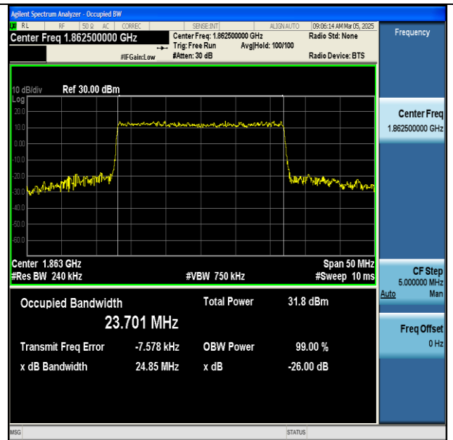
NTNV-n25-PC3-15-25-L-CP-QPSK-Outer_Full-Ant1-PASS
