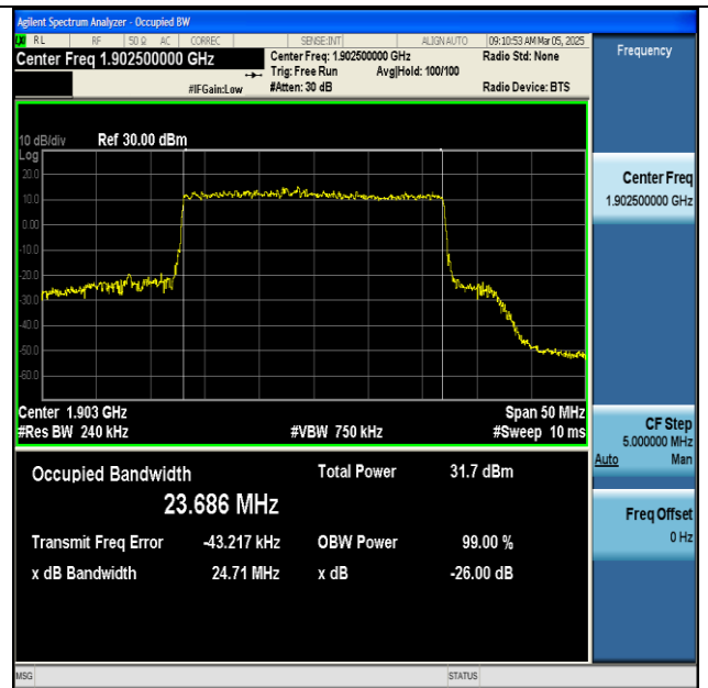
NTNV-n25-PC3-15-25-H-CP-64QAM-Outer_Full-Ant1- PASS
