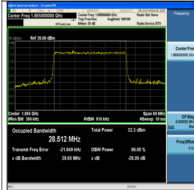
NTNV-n25-PC3-15-30-L-DFT-64QAM-Outer_Full-Ant1- PASS
