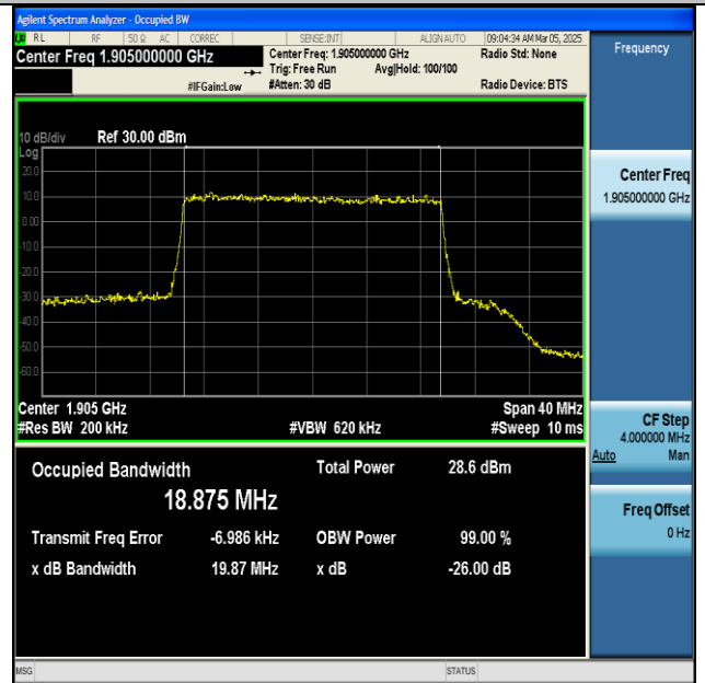
NTNV-n25-PC3-15-20-H-CP-256QAM-Outer_Full-Ant1-PASS
