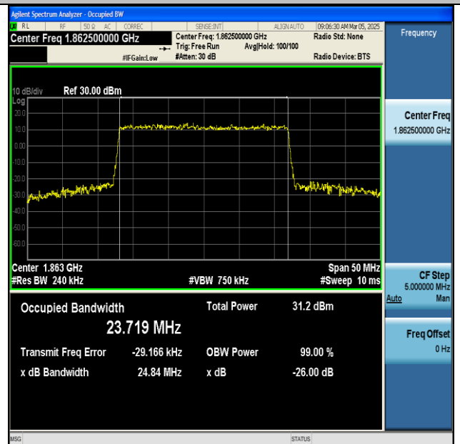
NTNV-n25-PC3-15-25-L-CP-64QAM-Outer_Full-Ant1-PASS
