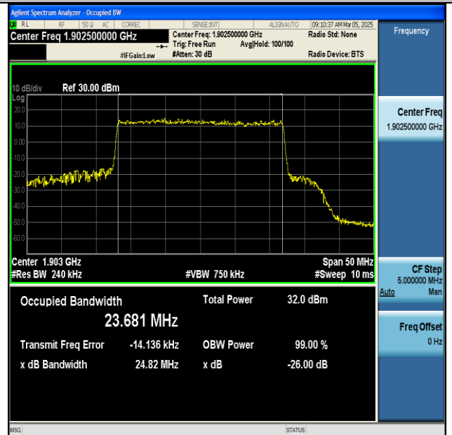
NTNV-n25-PC3-15-25-H-CP-QPSK-Outer_Full-Ant1-PASS
