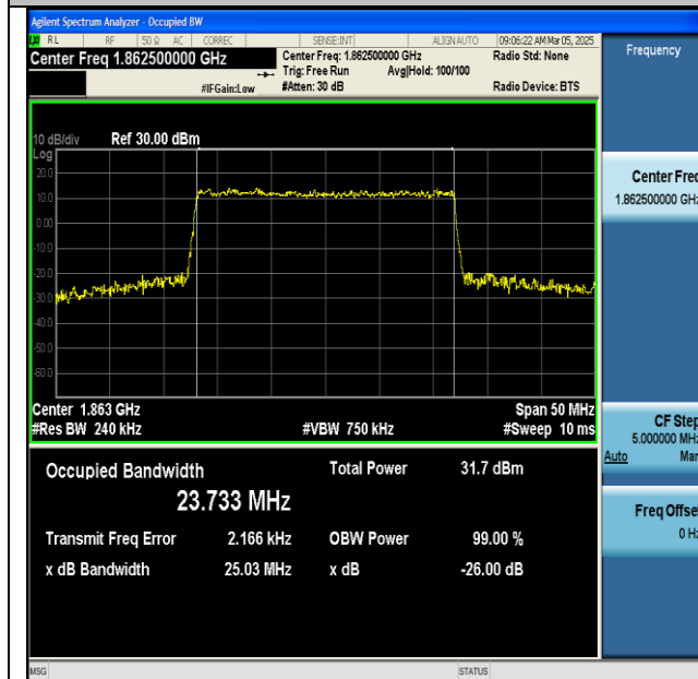
NTNV-n25-PC3-15-25-L-CP-16QAM-Outer_Full-Ant1-PASS
