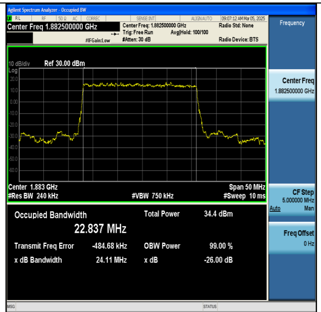
NTNV-n25-PC3-15-25-M-DFT-BPSK-Outer_Full-Ant1- PASS
