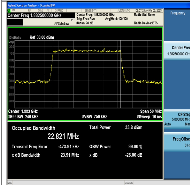
NTNV-n25-PC3-15-25-M-DFT-QPSK-Outer_Full-Ant1- PASS
