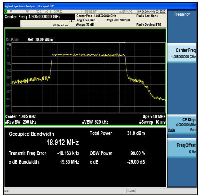
NTNV-n25-PC3-15-20-H-CP-16QAM-Outer_Full-Ant1-PASS
