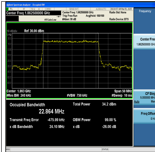
NTNV-n25-PC3-15-25-L-DFT-BPSK-Outer_Full-Ant1- PASS
