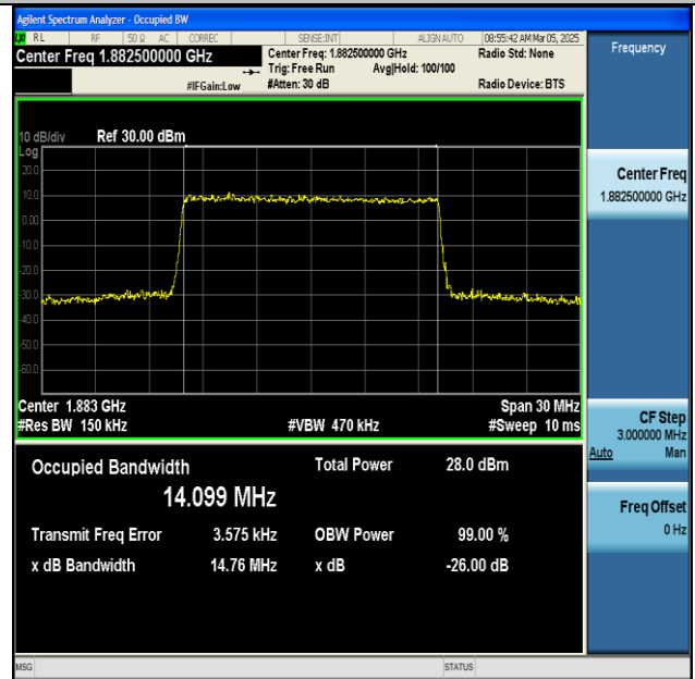
NTNV-n25-PC3-15-15-M-CP-256QAM-Outer_Full-Ant1-PASS
