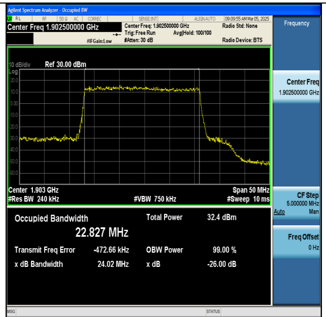
NTNV-n25-PC3-15-25-H-DFT-64QAM-Outer_Full-Ant1- PASS
