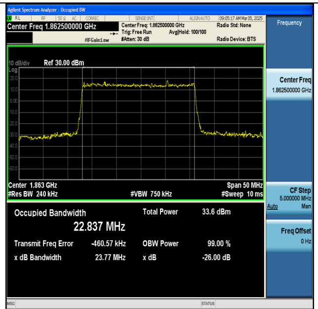
NTNV-n25-PC3-15-25-L-DFT-QPSK-Outer_Full-Ant1- PASS
