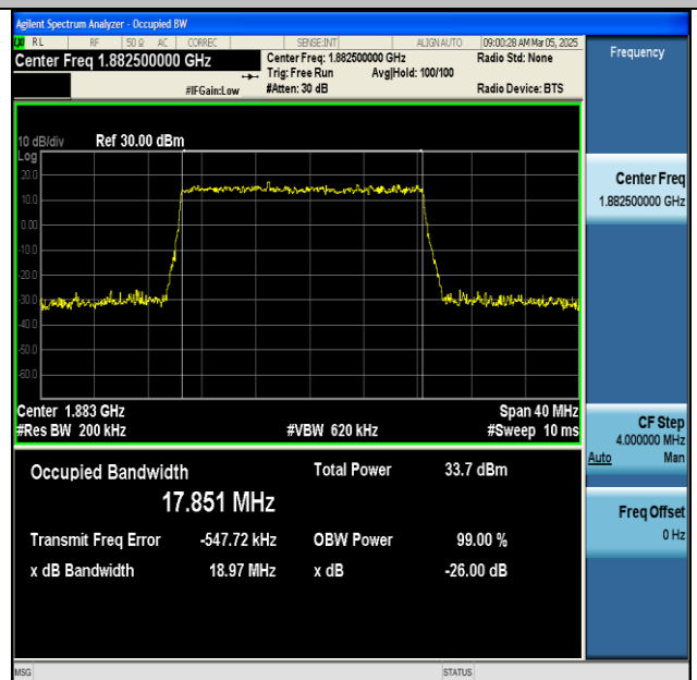
NTNV-n25-PC3-15-20-M-DFT-QPSK-Outer_Full-Ant1- PASS
