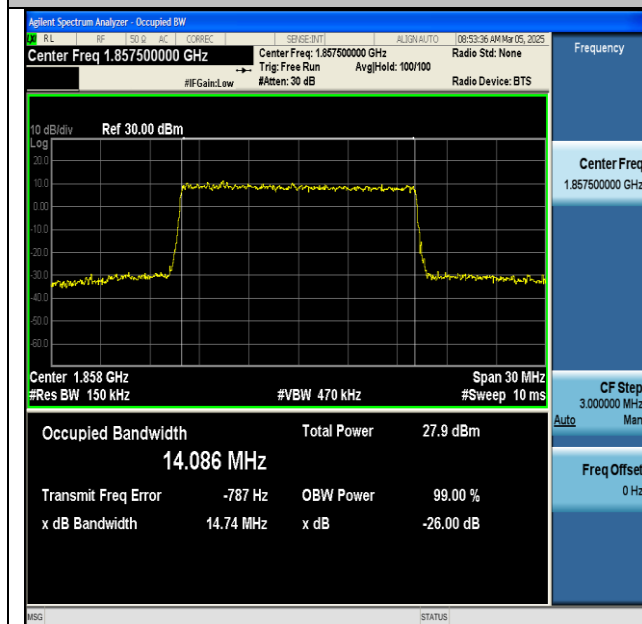
NTNV-n25-PC3-15-15-L-CP-256QAM-Outer_Full-Ant1- PASS
