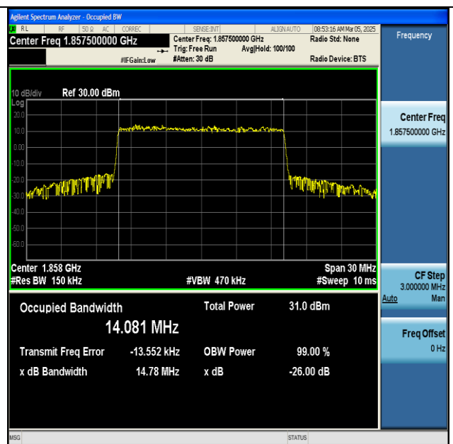
NTNV-n25-PC3-15-15-L-CP-64QAM-Outer_Full-Ant1- PASS
