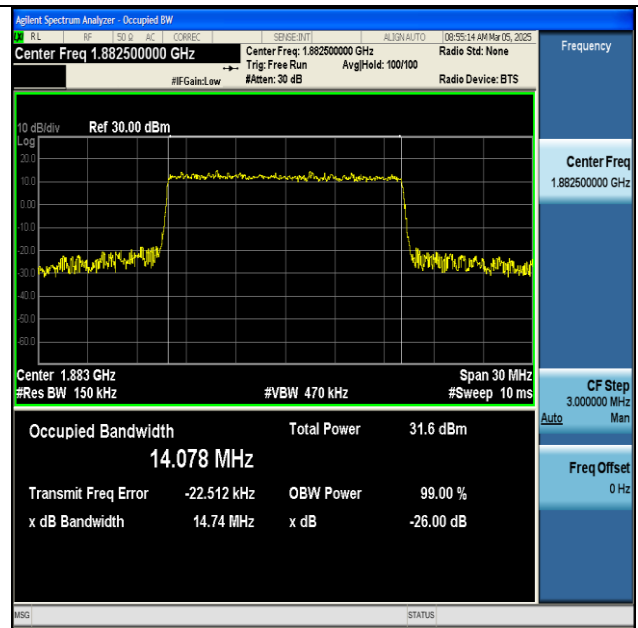
NTNV-n25-PC3-15-15-M-CP-16QAM-Outer_Full-Ant1-PASS
