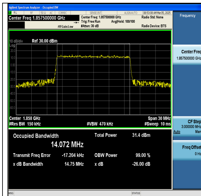
NTNV-n25-PC3-15-15-L-CP-16QAM-Outer_Full-Ant1- PASS
