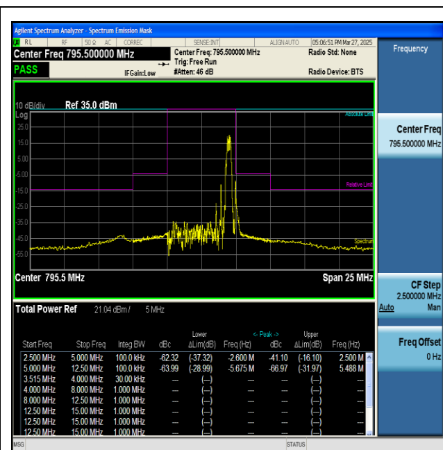
NTNT-n14-PC3-15-5-H-CP-QPSK-Inner_1RB_Right-PASS
