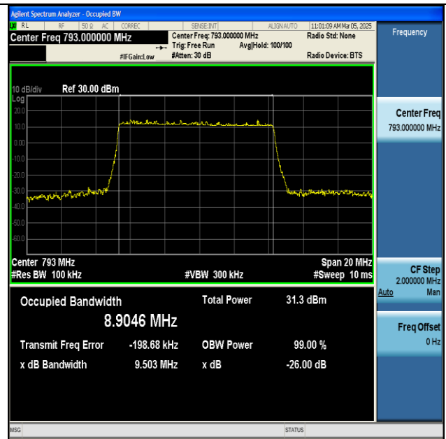
NTNV-n14-PC3-15-10-L-DFT-16QAM-Outer_Full-Ant1- PASS
