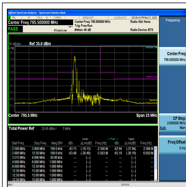
NTNT-n14-PC3-15-5-H-CP-QPSK-Inner_1RB_Left-PASS
