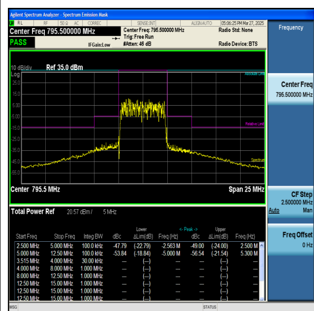
NTNT-n14-PC3-15-5-H-CP-QPSK-Outer_Full-PASS
