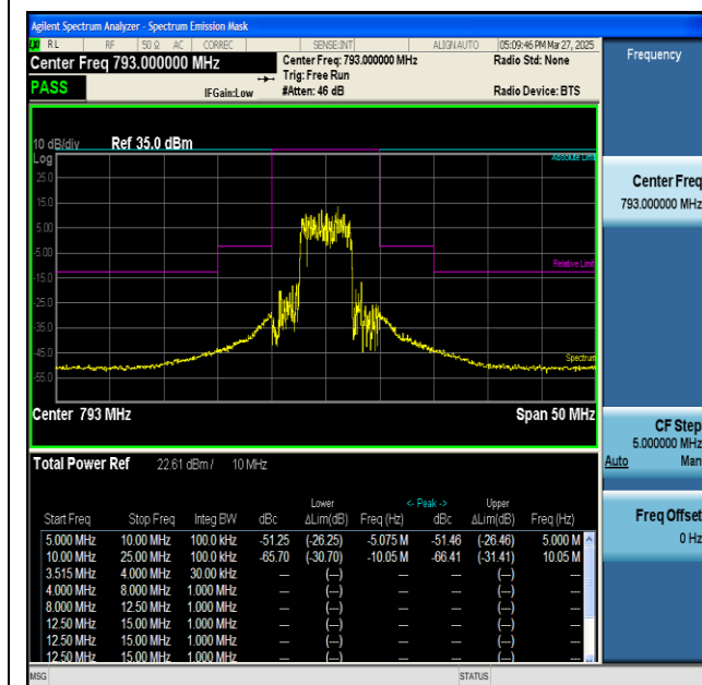
NTNT-n14-PC3-15-10-H-CP-QPSK-Inner_Full-PASS
