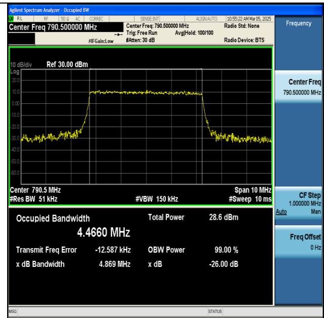
NTNV-n14-PC3-15-5-L-CP-QPSK-Outer_Full-Ant1-PASS
