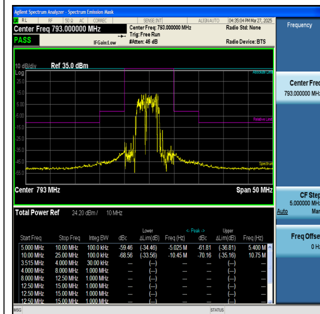
NTNT-n14-PC3-15-10-L-DFT-BPSK-Inner_Full-PASS
