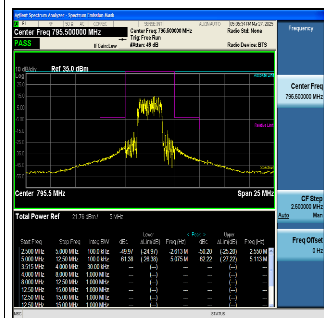
NTNT-n14-PC3-15-5-H-CP-QPSK-Inner_Full-PASS
