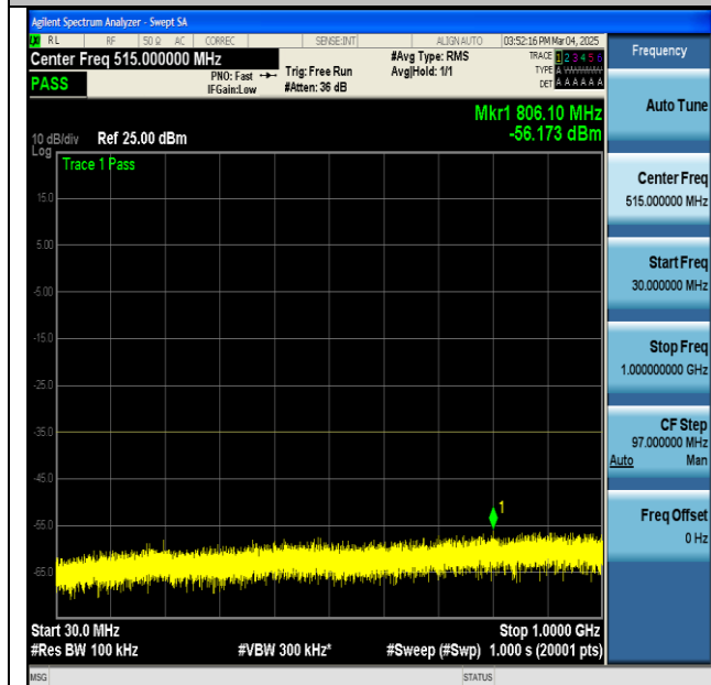
NTNV-n7-PC3-15-20-H-DFT-BPSK-Edge_1RB_Left-30-1000-PASS
