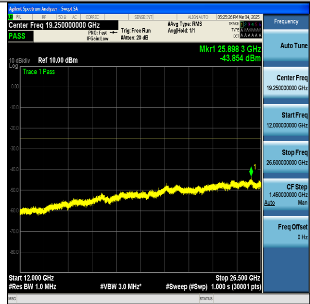
NTNV-n7-PC3-15-20-M-CP-QPSK-Edge_1RB_Left-12000-26500-PASS
