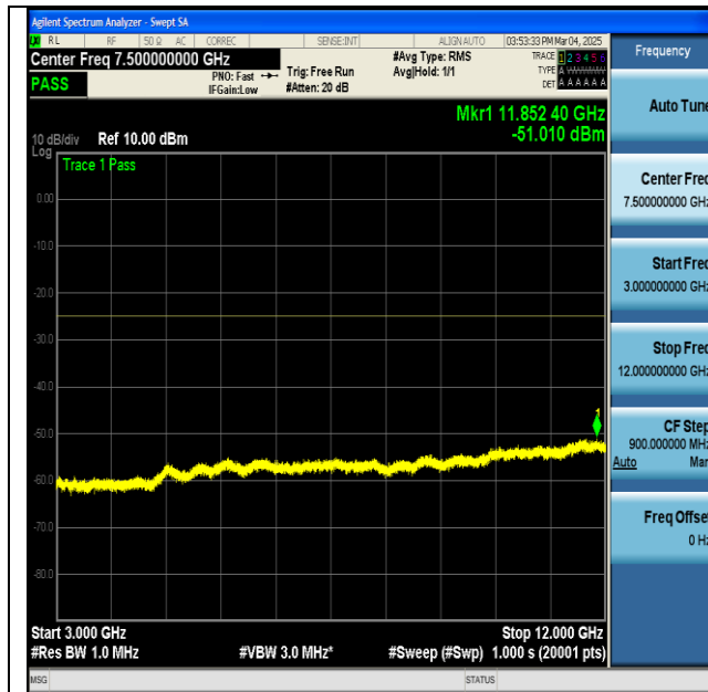
NTNV-n7-PC3-15-20-H-CP-QPSK-Edge_1RB_Left-3000-12000-PASS
