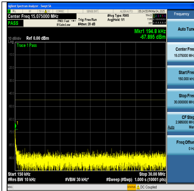
NTNV-n7-PC3-15-20-M-CP-QPSK-Edge_1RB_Left-0.15-30-PASS
