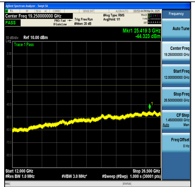
NTNV-n7-PC3-15-20-H-CP-QPSK-Edge_1RB_Left-12000-26500-PASS
