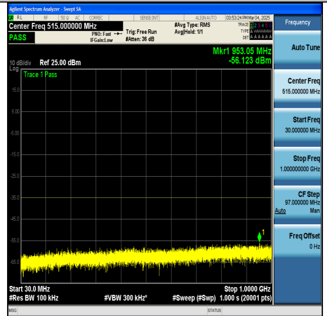
NTNV-n7-PC3-15-20-H-CP-QPSK-Edge_1RB_Left-30-1000-PASS
