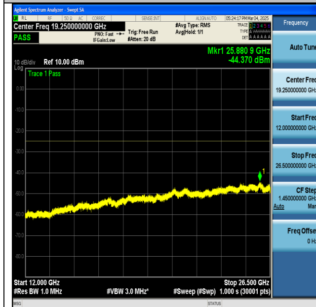
NTNV-n7-PC3-15-20-M-DFT-BPSK-Edge_1RB_Left-12000-26500-PASS
