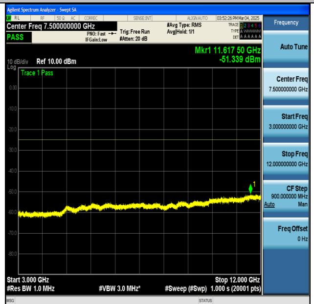
NTNV-n7-PC3-15-20-H-DFT-BPSK-Edge_1RB_Left-3000-12000-PASS
