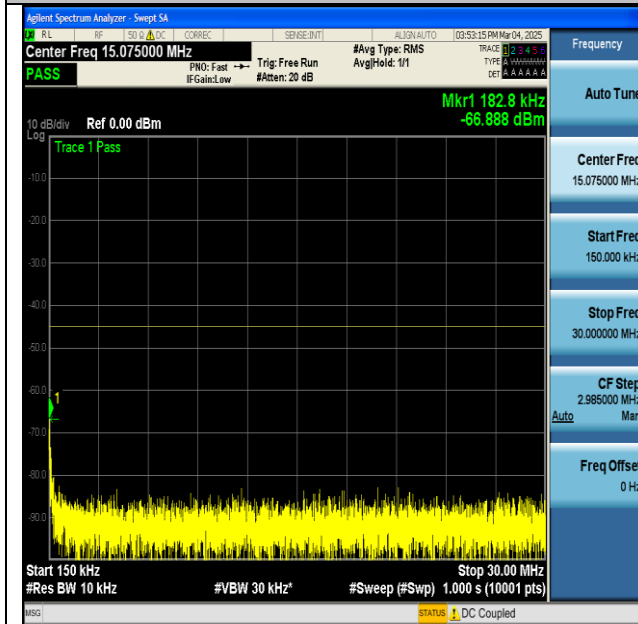
NTNV-n7-PC3-15-20-H-CP-QPSK-Edge_1RB_Left-0.15-30-PASS
