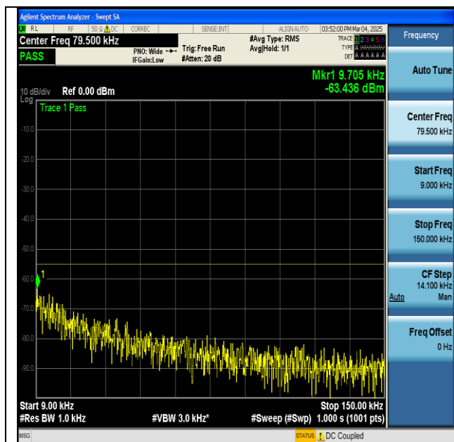
NTNV-n7-PC3-15-20-H-DFT-BPSK-Edge_1RB_Left-0.009-0.15-PASS
