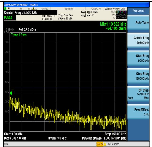
NTNV-n7-PC3-15-20-H-CP-QPSK-Edge_1RB_Left-0.009-0.15-PASS
