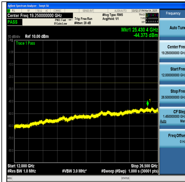
NTNV-n7-PC3-15-20-H-DFT-BPSK-Edge_1RB_Left-12000-26500-PASS
