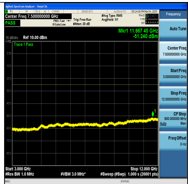
NTNV-n7-PC3-15-20-M-DFT-BPSK-Edge_1RB_Left-3000-12000-PASS
