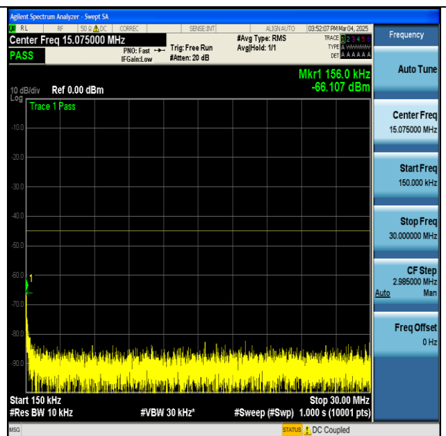
NTNV-n7-PC3-15-20-H-DFT-BPSK-Edge_1RB_Left-0.15-30-PASS
