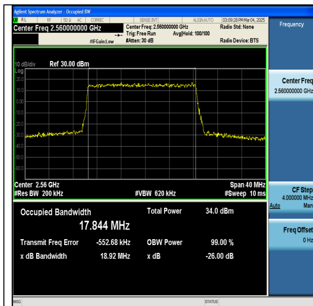
NTNV-n7-PC3-15-20-H-DFT-QPSK-Outer_Full-Ant1-PASS
