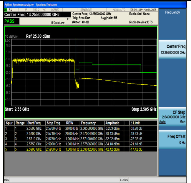
NTNV-n7-PC3-15-20-H-CP-QPSK-Outer_Full-PASS
