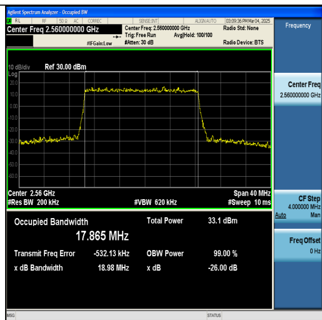
NTNV-n7-PC3-15-20-H-DFT-16QAM-Outer_Full-Ant1-PASS
