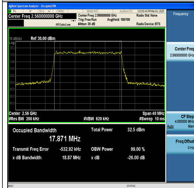
NTNV-n7-PC3-15-20-H-DFT-64QAM-Outer_Full-Ant1-PASS
