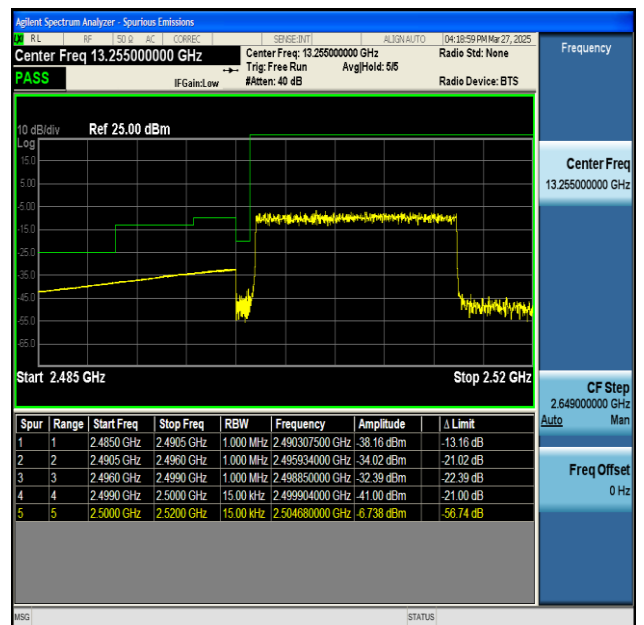
NTNV-n7-PC3-15-15-L-CP-QPSK-Outer_Full-PASS
