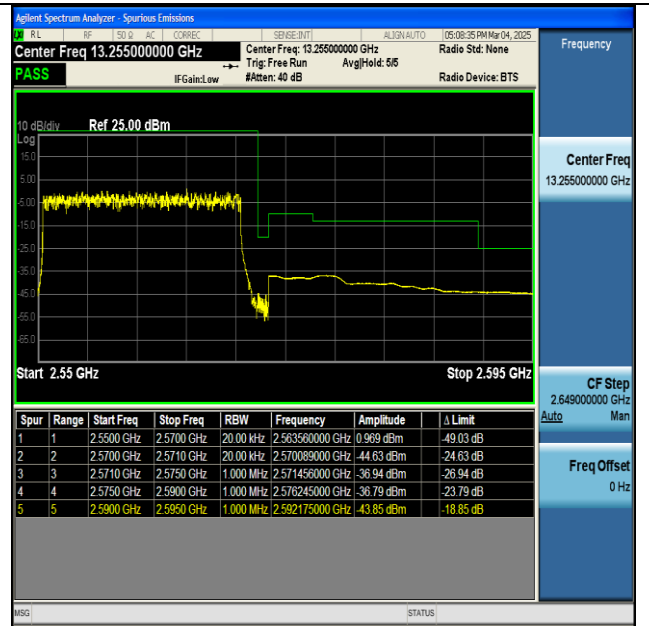
NTNV-n7-PC3-15-20-H-DFT-BPSK-Outer_Full-PASS
