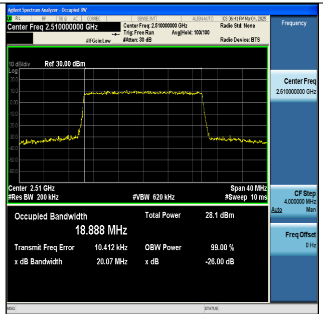
NTNV-n7-PC3-15-20-L-CP-256QAM-Outer_Full-Ant1-PASS
