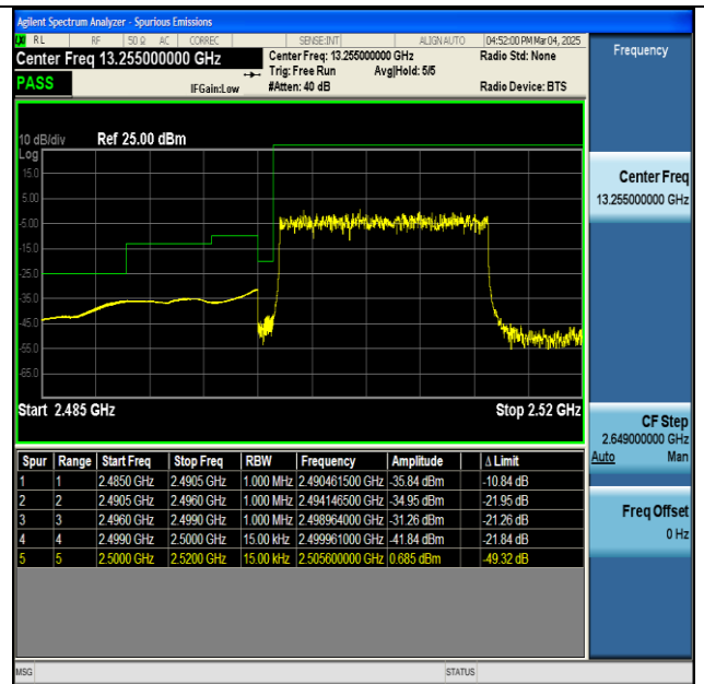
NTNV-n7-PC3-15-15-L-DFT-BPSK-Outer_Full-PASS
