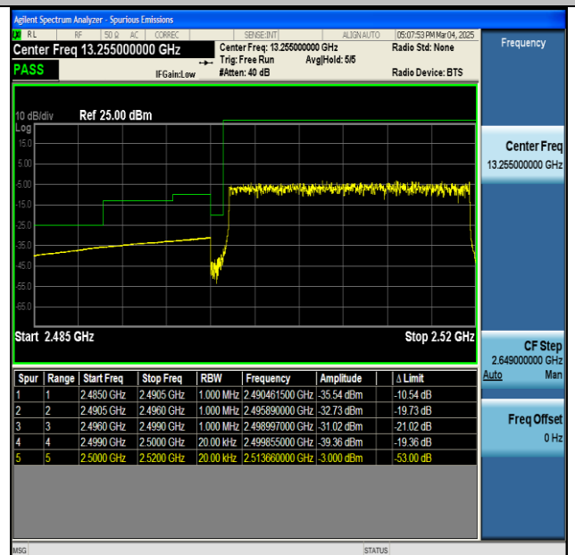
NTNV-n7-PC3-15-20-L-CP-QPSK-Outer_Full-PASS
