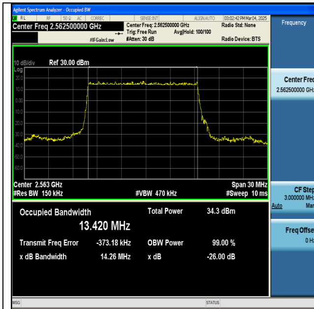
NTNV-n7-PC3-15-15-H-DFT-BPSK-Outer_Full-Ant1-PASS
