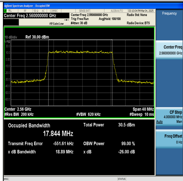
NTNV-n7-PC3-15-20-H-DFT-256QAM-Outer_Full-Ant1-PASS
