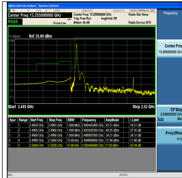
NTNV-n7-PC3-15-15-L-DFT-BPSK-Edge_1RB_Left-PASS
