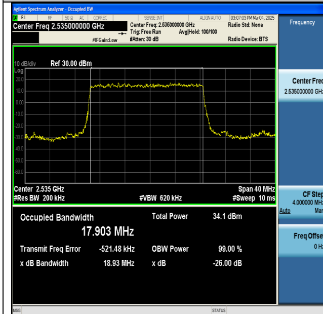
NTNV-n7-PC3-15-20-M-DFT-BPSK-Outer_Full-Ant1-PASS
