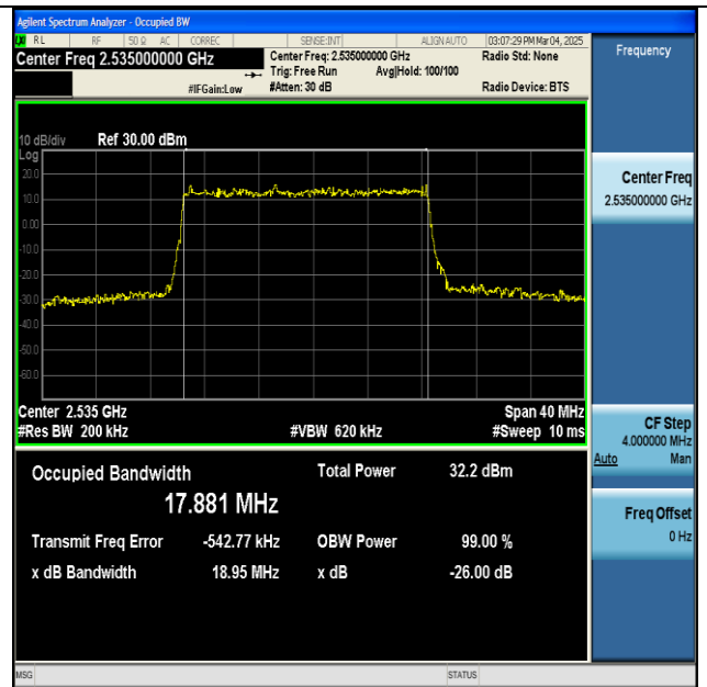
NTNV-n7-PC3-15-20-M-DFT-64QAM-Outer_Full-Ant1- PASS
