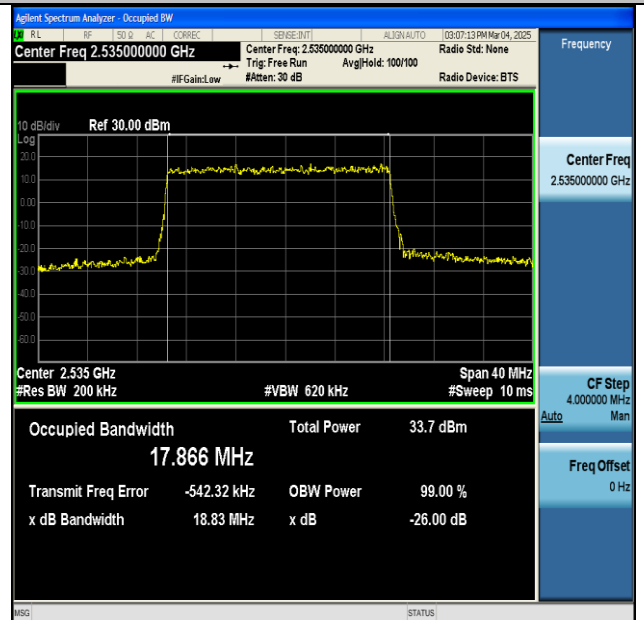
NTNV-n7-PC3-15-20-M-DFT-QPSK-Outer_Full-Ant1-PASS
