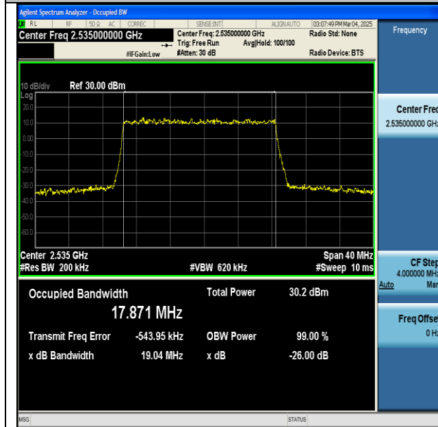
NTNV-n7-PC3-15-20-M-DFT-256QAM-Outer_Full-Ant1- PASS
