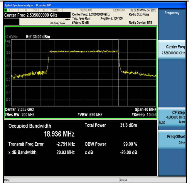
NTNV-n7-PC3-15-20-M-CP-QPSK-Outer_Full-Ant1-PASS
