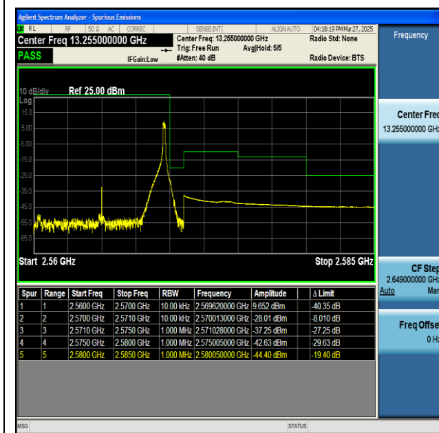
NTNV-n7-PC3-15-10-H-CP-QPSK-Edge_1RB_Right-PASS
