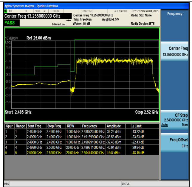
NTNV-n7-PC3-15-20-L-DFT-BPSK-Outer_Full-PASS
