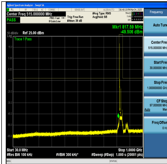
NTNV-n5-PC3-15-20-M-CP-QPSK-Edge_1RB_Left-30-1000-PASS
