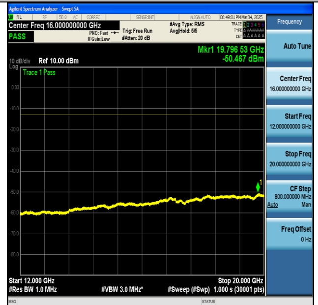
NTNV-n5-PC3-15-20-M-CP-QPSK-Edge_1RB_Left-12000-20000-PASS
