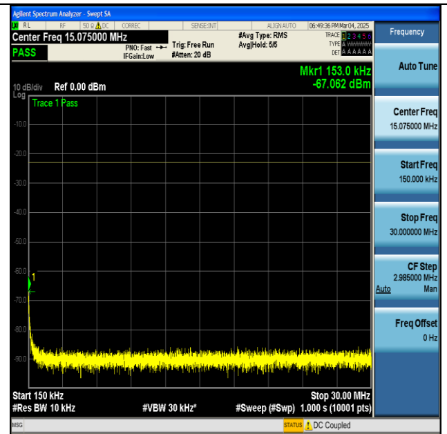
NTNV-n5-PC3-15-20-H-DFT-BPSK-Edge_1RB_Left-0.15-30-PASS
