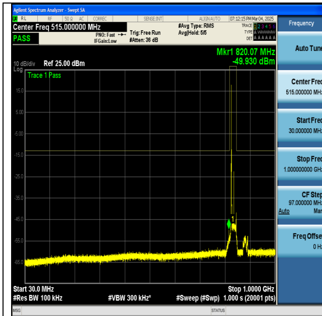
NTNV-n5-PC3-15-20-H-CP-QPSK-Edge_1RB_Left-30-1000-PASS
