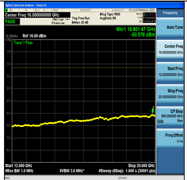
NTNV-n5-PC3-15-20-H-CP-QPSK-Edge_1RB_Left-12000-20000-PASS
