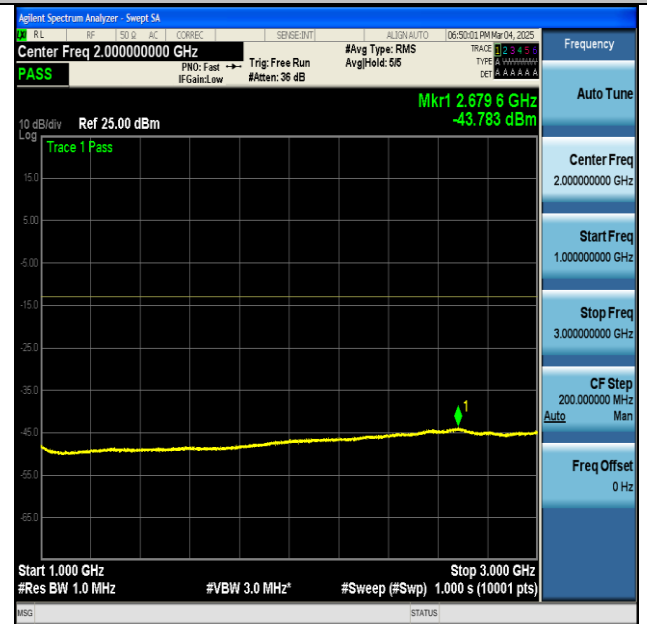
NTNV-n5-PC3-15-20-H-DFT-BPSK-Edge_1RB_Left-1000-3000-PASS
