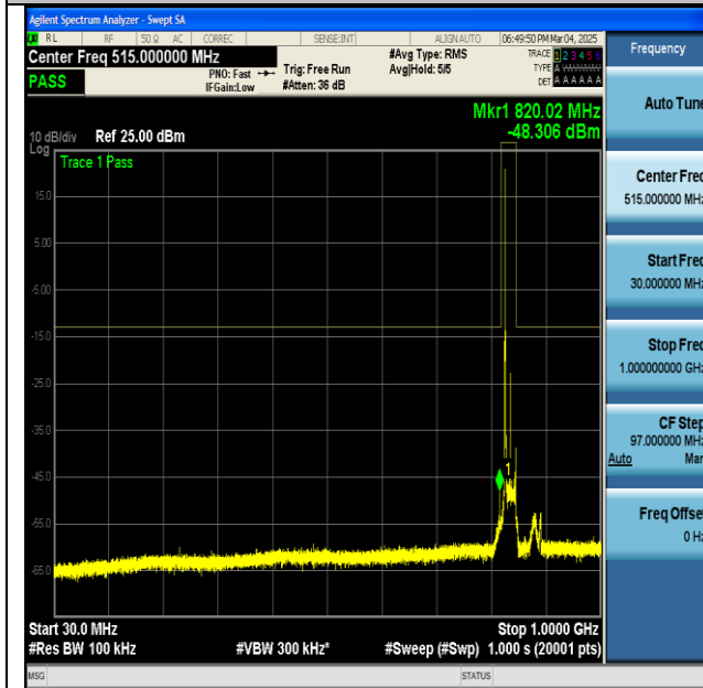
NTNV-n5-PC3-15-20-H-DFT-BPSK-Edge_1RB_Left-30-1000-PASS
