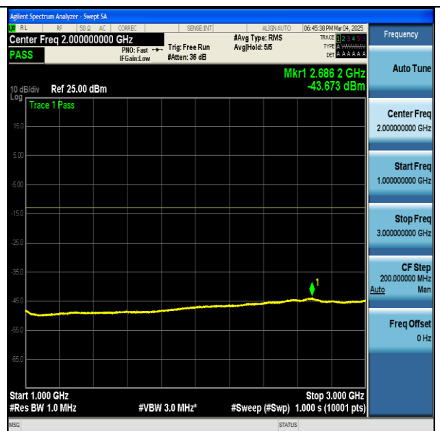
NTNV-n5-PC3-15-20-L-CP-QPSK-Edge_1RB_Left-1000-3000-PASS
