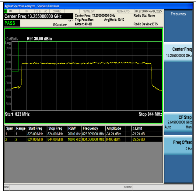
NTNV-n5-PC3-15-20-L-DFT-BPSK-Outer_Full-PASS
