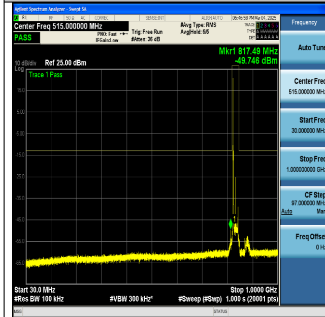
NTNV-n5-PC3-15-20-M-DFT-BPSK-Edge_1RB_Left-30-1000-PASS
