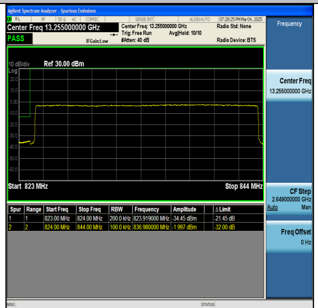
NTNV-n5-PC3-15-20-L-CP-QPSK-Outer_Full-PASS
