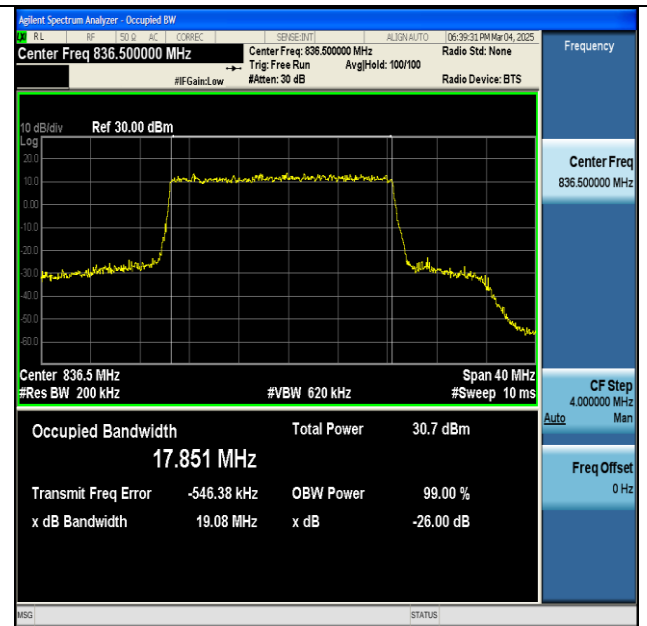
NTNV-n5-PC3-15-20-M-DFT-64QAM-Outer_Full-Ant1- PASS
