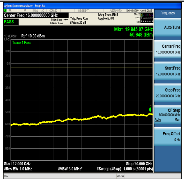
NTNV-n5-PC3-15-20-L-CP-QPSK-Edge_1RB_Left-12000-20000-PASS
