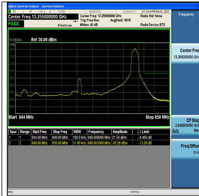
NTNV-n5-PC3-15-5-H-DFT-BPSK-Edge_1RB_Right-PASS
