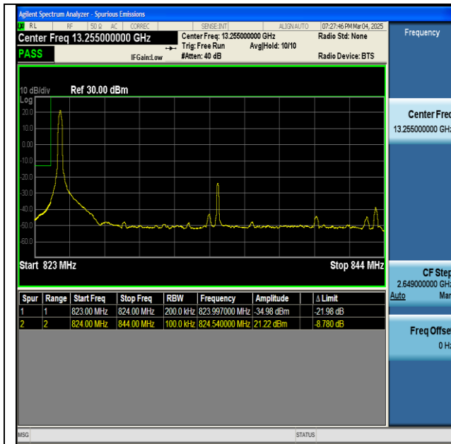
NTNV-n5-PC3-15-20-L-DFT-BPSK-Edge_1RB_Left-PASS
