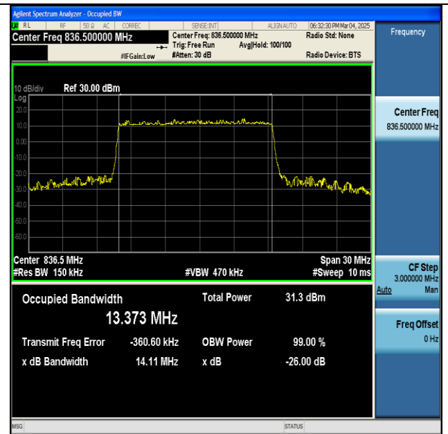
NTNV-n5-PC3-15-15-M-DFT-16QAM-Outet_Full-Ant1-PASS
