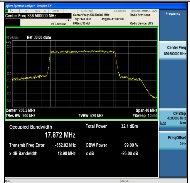
NTNV-n5-PC3-15-20-M-DFT-QPSK-Outer_Full-Ant1-PASS
