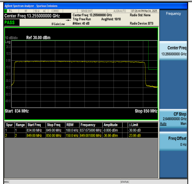
NTNV-n5-PC3-15-15-H-CP-QPSK-Outer_Full-PASS
