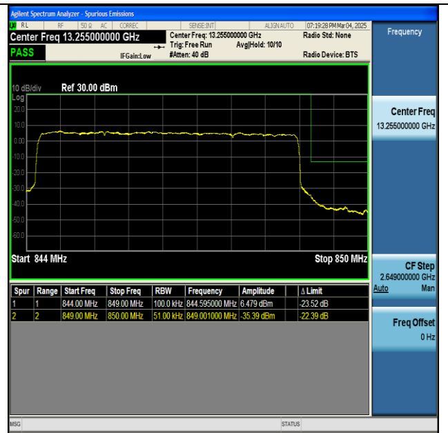
NTNV-n5-PC3-15-5-H-DFT-BPSK-Outer_Full-PASS
