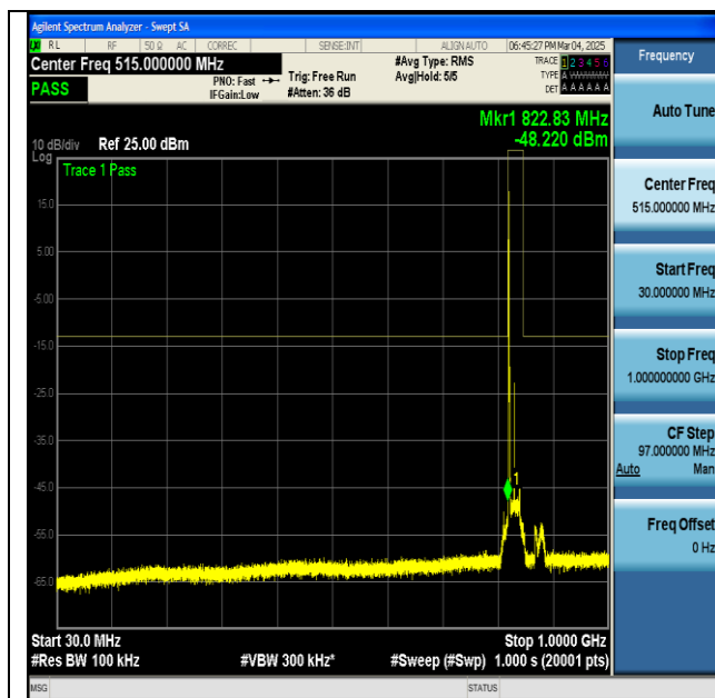
NTNV-n5-PC3-15-20-L-CP-QPSK-Edge_1RB_Left-30-1000-PASS
