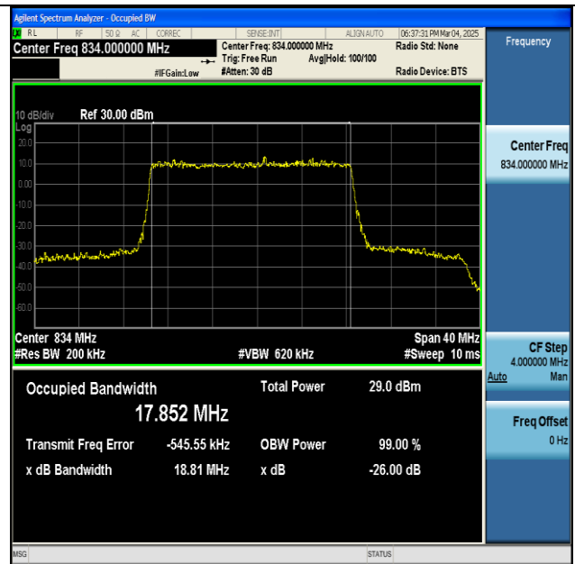
NTNV-n5-PC3-15-20-L-DFT-256QAM-Outer_Full-Ant1- PASS
