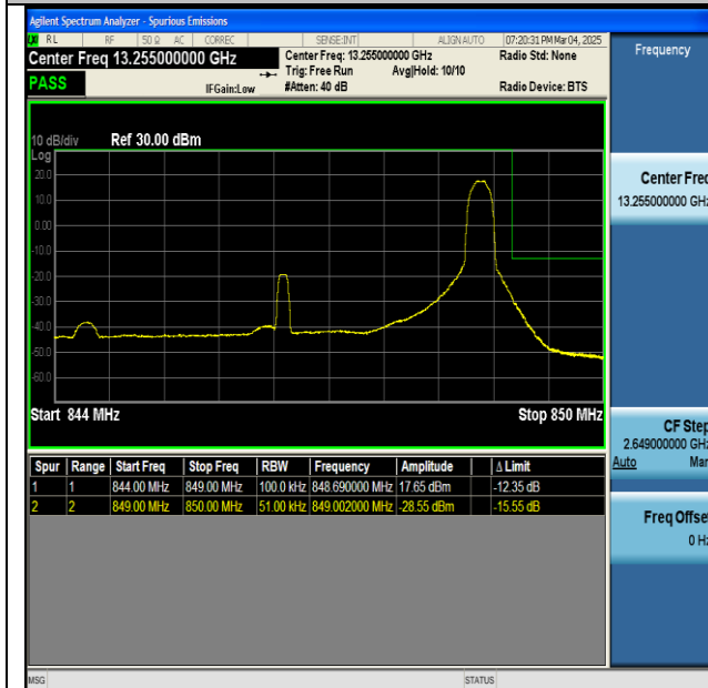
NTNV-n5-PC3-15-5-H-CP-QPSK-Edge_1RB_Right-PASS
