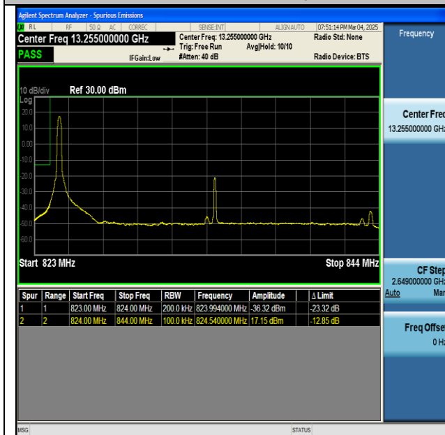
NTNV-n5-PC3-15-20-L-CP-QPSK-Edge_1RB_Left-PASS
