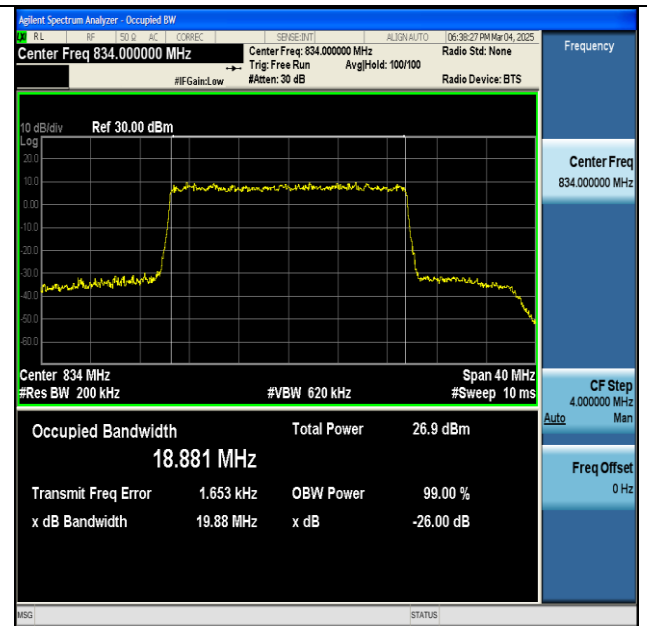
NTNV-n5-PC3-15-20-L-CP-256QAM-Outer_Full-Ant1-PASS
