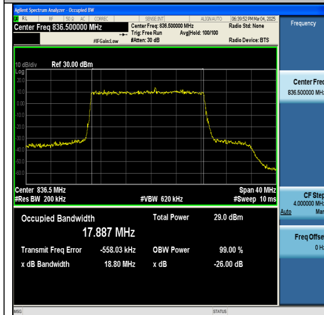
NTNV-n5-PC3-15-20-M-DFT-256QAM-Outer_Full-Ant1- PASS
