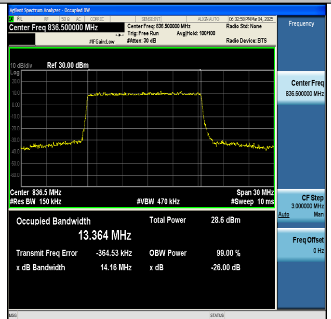
NTNV-n5-PC3-15-15-M-DFT-256QAM-Outet_Full-Ant1-PASS
