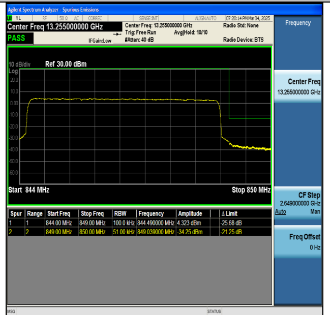
NTNV-n5-PC3-15-5-H-CP-QPSK-Outer_Full-PASS
