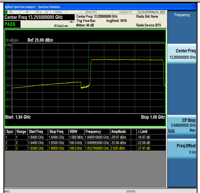
NTNV-n2-PC3-15-10-L-CP-QPSK-Outer_Full-PASS
