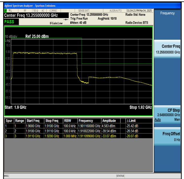
NTNV-n2-PC3-15-10-H-DFT-BPSK-Outer_Full-PASS
