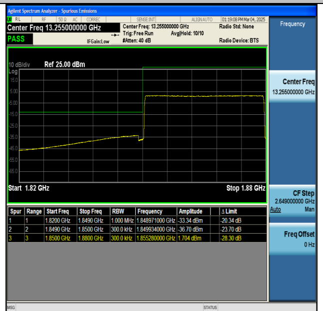
NTNV-n2-PC3-15-30-L-CP-QPSK-Outer_Full-PASS
