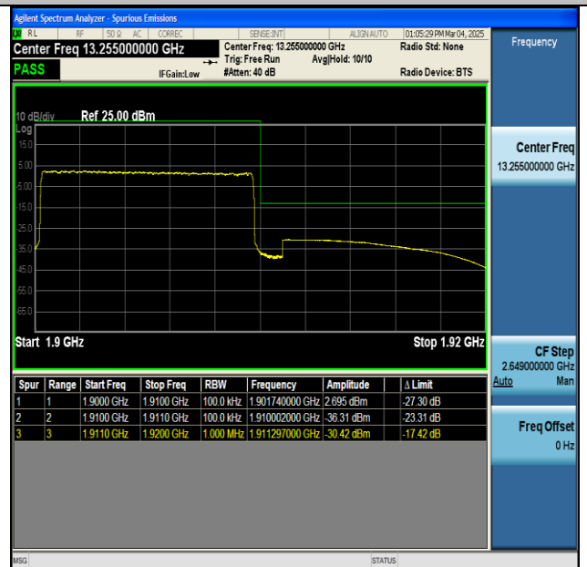
NTNV-n2-PC3-15-10-H-CP-QPSK-Outer_Full-PASS
