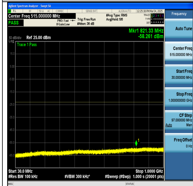
NTNV-n2-PC3-15-30-M-DFT-BPSK-Edge_1RB_Left-30- 1000-PASS
