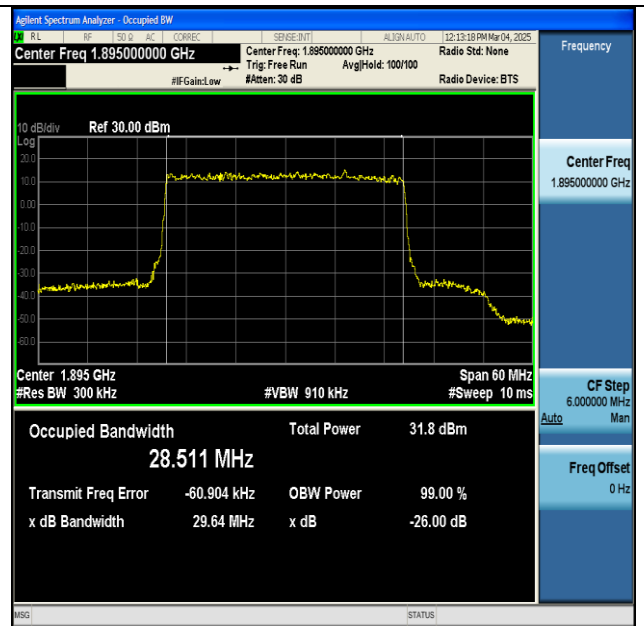
NTNV-n2-PC3-15-30-H-DFT-BPSK-Outet_Full-Ant1-PASS
