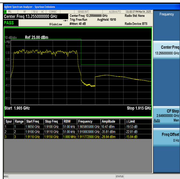
NTNV-n2-PC3-15-5-H-DFT-BPSK-Outer_Full-PASS
