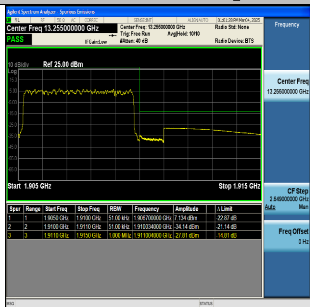
NTNV-n2-PC3-15-5-H-CP-QPSK-Outer_Full-PASS
