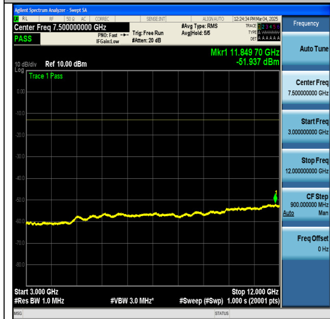
NTNV-n2-PC3-15-30-L-CP-QPSK-Edge_1RB_Left-3000-12000-PASS
