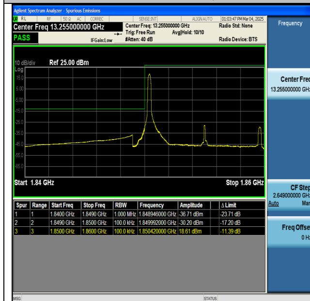
NTNV-n2-PC3-15-10-L-CP-QPSK-Edge_1RB_Left-PASS
