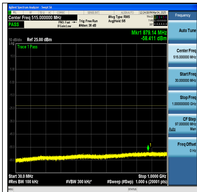
NTNV-n2-PC3-15-30-L-CP-QPSK-Edge_1RB_Left-30-1000-PASS
