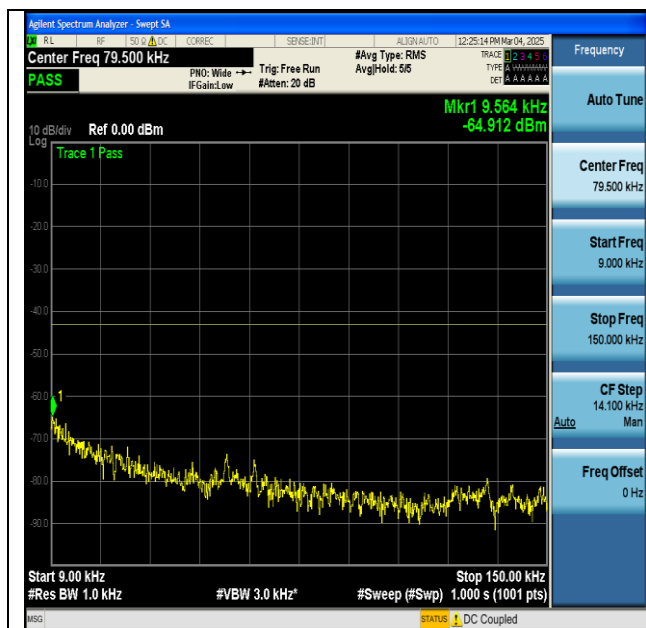
NTNV-n2-PC3-15-30-M-DFT-BPSK-Edge_1RB_Left- 0.009-0.15-PASS
