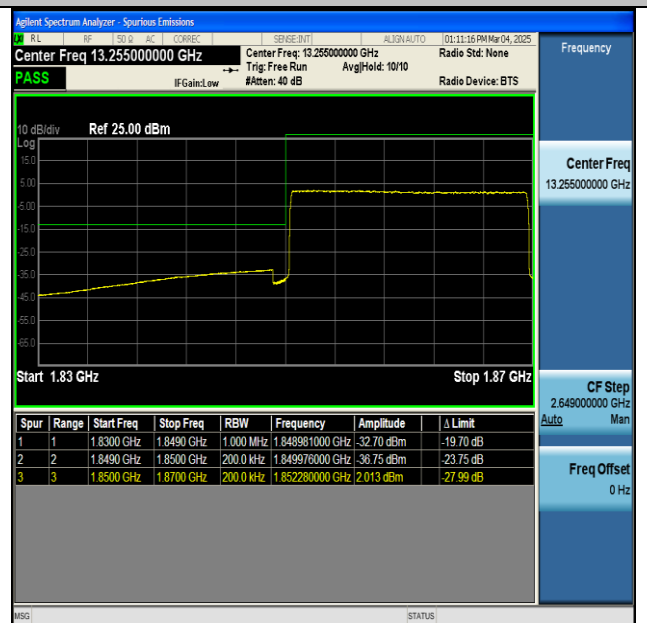
NTNV-n2-PC3-15-20-L-CP-QPSK-Outer_Full-PASS
