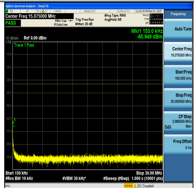
NTNV-n2-PC3-15-30-M-CP-QPSK-Edge_1RB_Left-0.15-30-PASS
