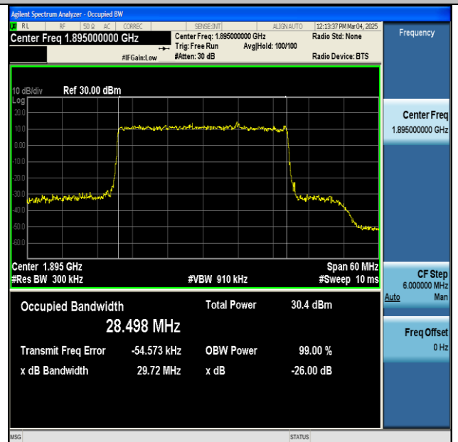
NTNV-n2-PC3-15-30-H-DFT-16QAM-Outet_Full-Ant1-PASS
