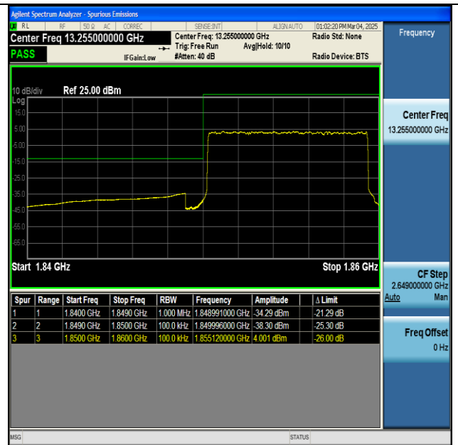
NTNV-n2-PC3-15-10-L-DFT-BPSK-Outer_Full-PASS
