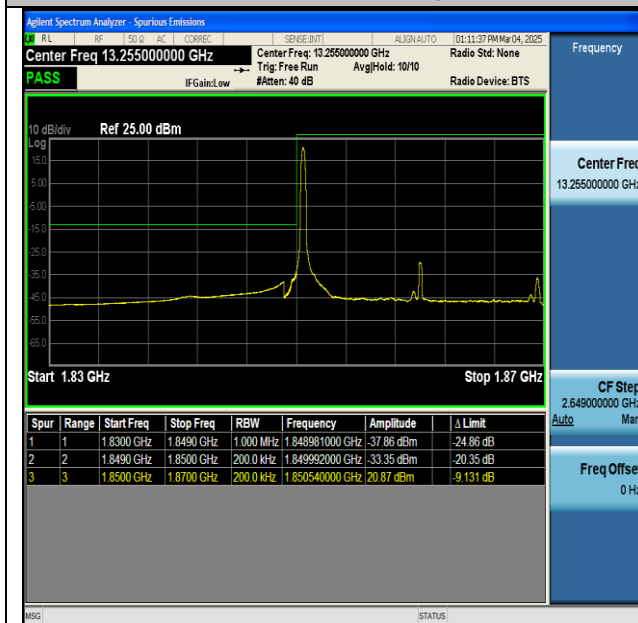
NTNV-n2-PC3-15-20-L-CP-QPSK-Edge_1RB_Left-PASS
