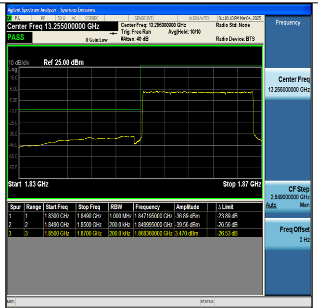
NTNV-n2-PC3-15-20-L-DFT-BPSK-Outer_Full-PASS
