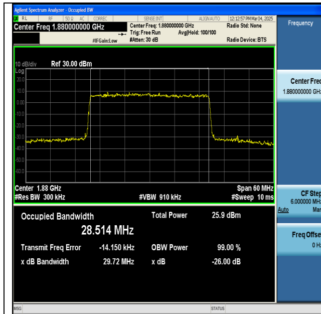
NTNV-n2-PC3-15-30-M-CP-256QAM-Outet_Full-Ant1-PASS
