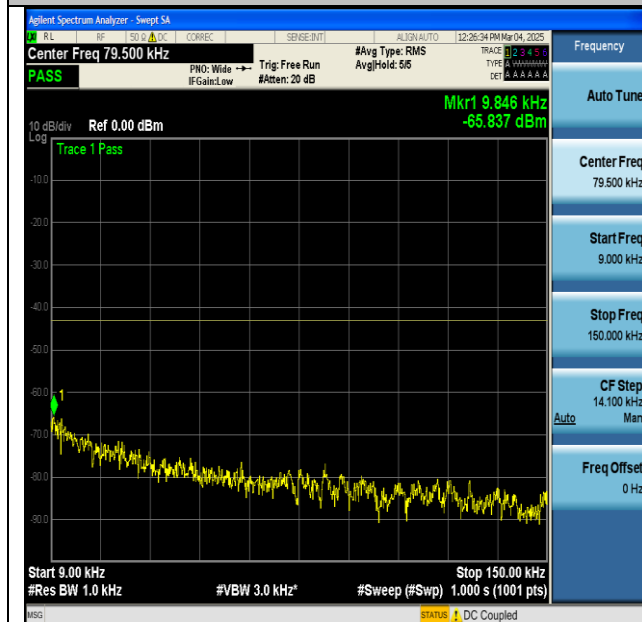
NTNV-n2-PC3-15-30-M-CP-QPSK-Edge_1RB_Left-0.009-0.15-PASS
