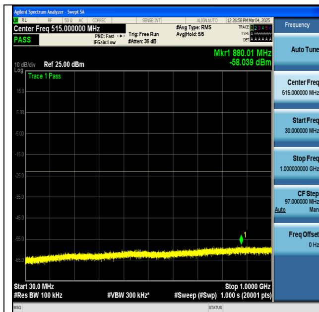
NTNV-n2-PC3-15-30-M-CP-QPSK-Edge_1RB_Left-30-1000-PASS
