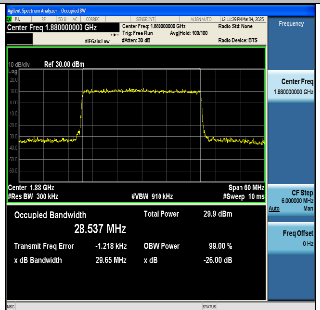
NTNV-n2-PC3-15-30-M-DFT-64QAM-Outer_Full-Ant1-PASS
