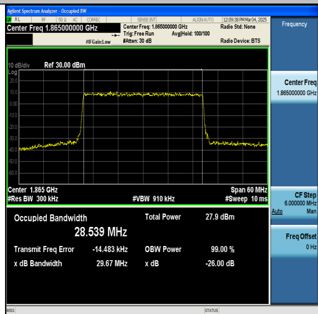
NTNV-n2-PC3-15-30-L-DFT-256QAM-Outer_Full-Ant1-PASS
