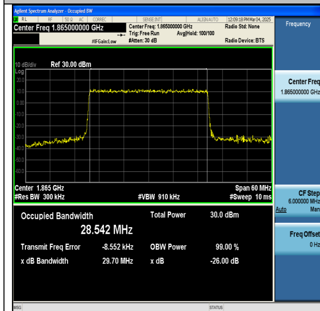
NTNV-n2-PC3-15-30-L-DFT-64QAM-Outer_Full-Ant1-PASS
