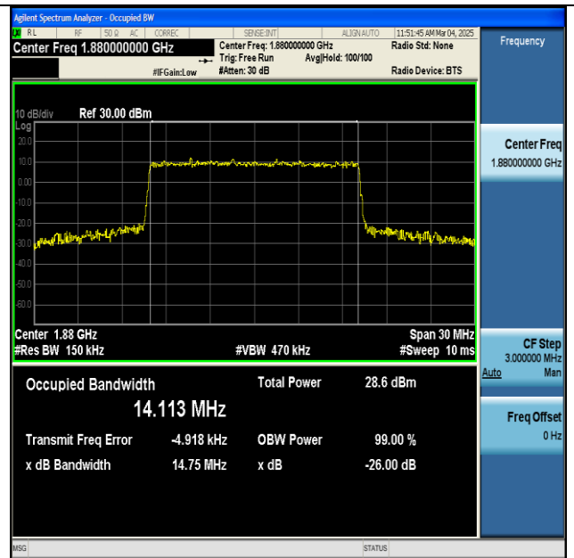
NTNV-n2-PC3-15-15-M-CP-16QAM-Outer_Full-Ant1-PASS
