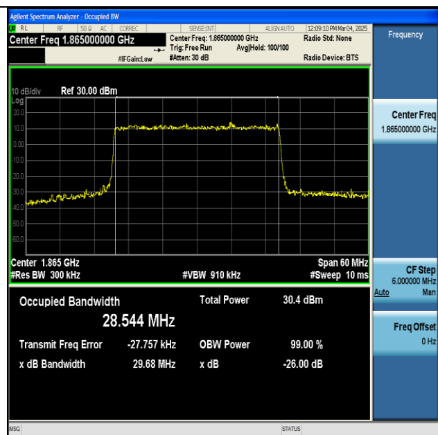
NTNV-n2-PC3-15-30-L-DFT-16QAM-Outer_Full-Ant1-PASS
