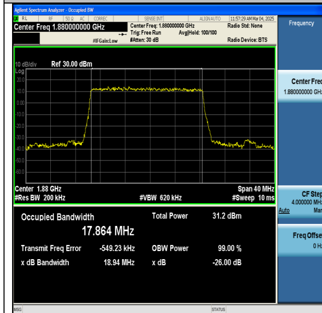
NTNV-n2-PC3-15-20-M-DFT-BPSK-Outer_Full-Ant1-PASS
