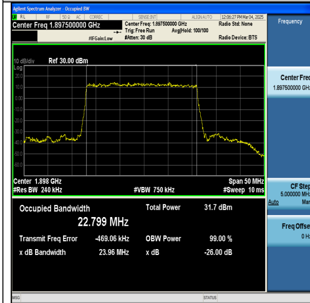
NTNV-n2-PC3-15-25-H-DFT-BPSK-Outer_Full-Ant1-PASS
