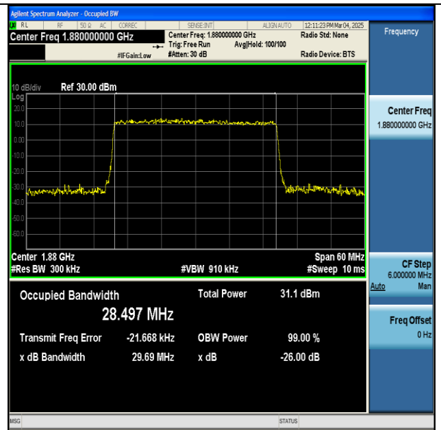
NTNV-n2-PC3-15-30-M-DFT-QPSK-Outer_Full-Ant1-PASS
