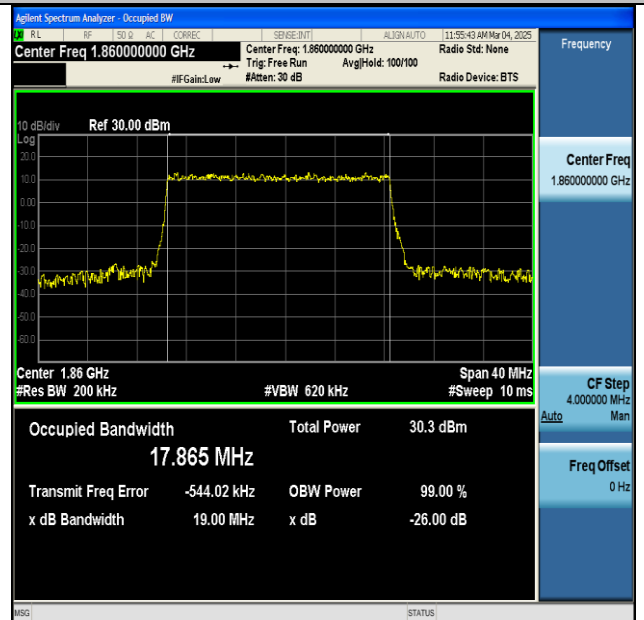
NTNV-n2-PC3-15-20-L-DFT-16QAM-Outet_Full-Ant1-PASS
