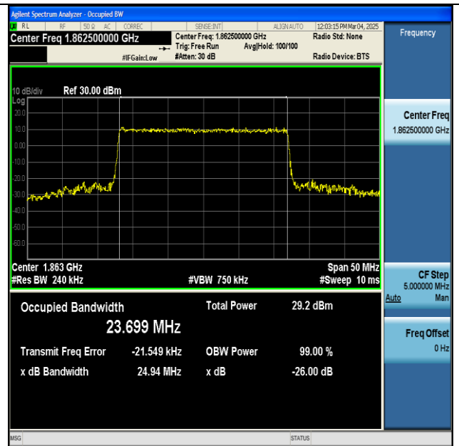
NTNV-n2-PC3-15-25-L-CP-QPSK-Outer_Full-Ant1-PASS
