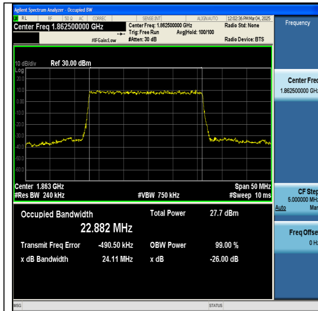
NTNV-n2-PC3-15-25-L-DFT-256QAM-Outer_Full-Ant1-PASS
