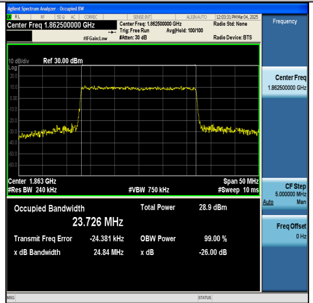
NTNV-n2-PC3-15-25-L-CP-64QAM-Outer_Full-Ant1-PASS
