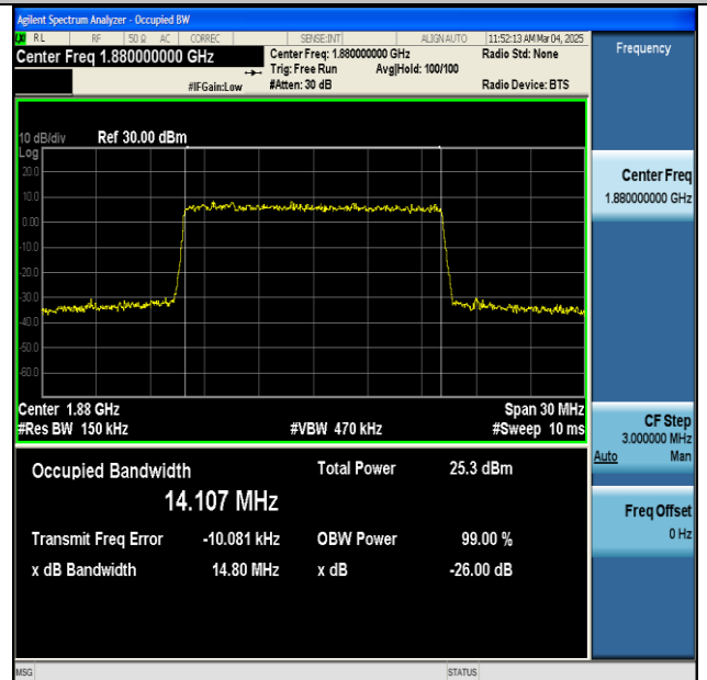
NTNV-n2-PC3-15-15-M-CP-256QAM-Outer_Full-Ant1-PASS
