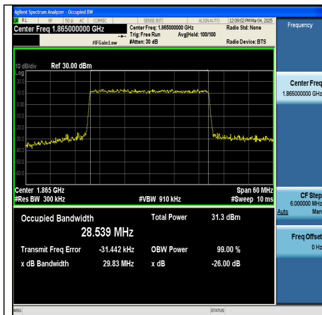
NTNV-n2-PC3-15-30-L-DFT-QPSK-Outer_Full-Ant1-PASS
