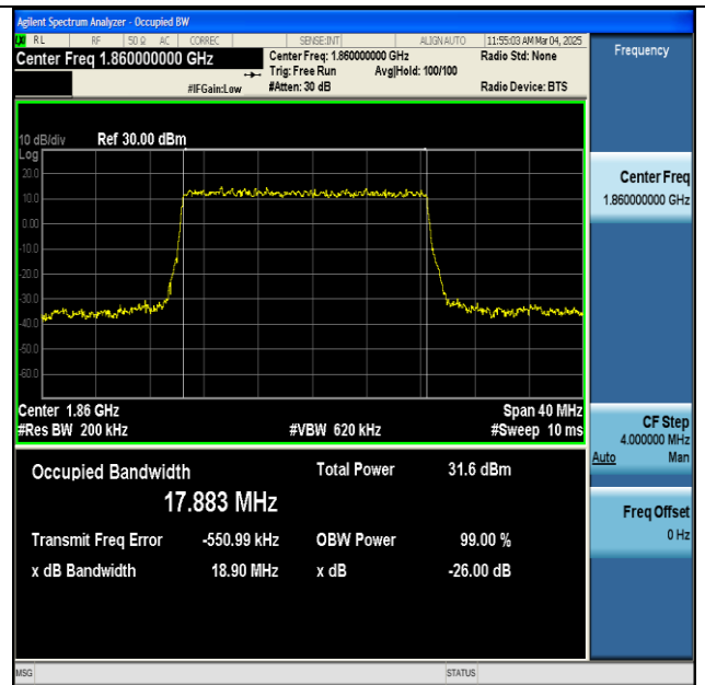
NTNV-n2-PC3-15-20-L-DFT-BPSK-Outet_Full-Ant1-PASS
