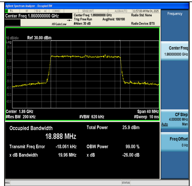
NTNV-n2-PC3-15-20-L-CP-256QAM-Outer_Full-Ant1-PASS
