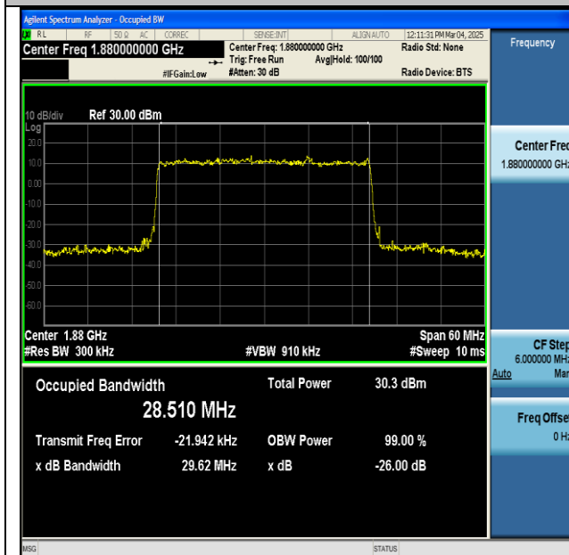
NTNV-n2-PC3-15-30-M-DFT-16QAM-Outer_Full-Ant1-PASS
