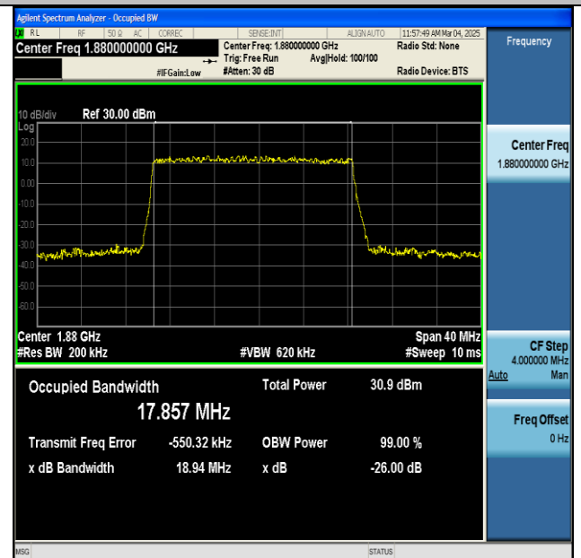
NTNV-n2-PC3-15-20-M-DFT-QPSK-Outer_Full-Ant1-PASS
