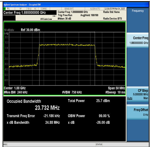
NTNV-n2-PC3-15-25-M-CP-256QAM-Outer_Full-Ant1- PASS
