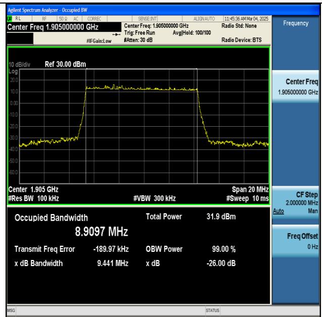
NTNV-n2-PC3-15-10-H-DFT-BPSK-Outer_Full-Ant1-PASS
