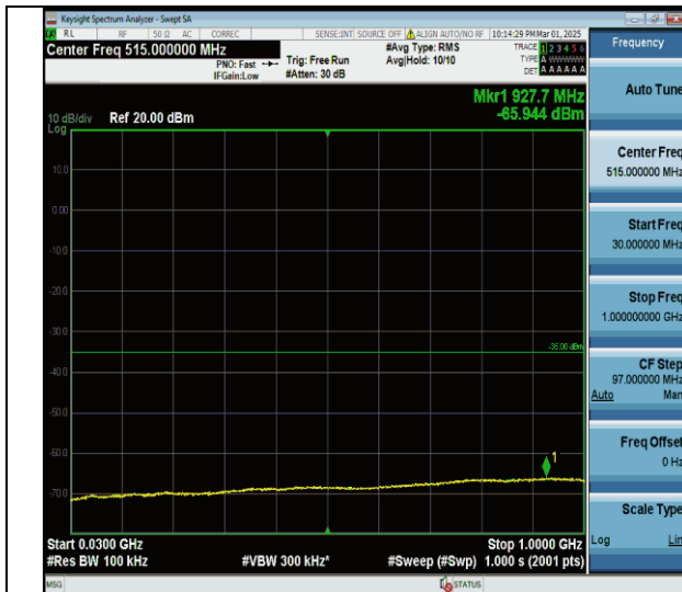
Band7-20MHz-QPSK-21350-1RB#0-30~1000-PASS
