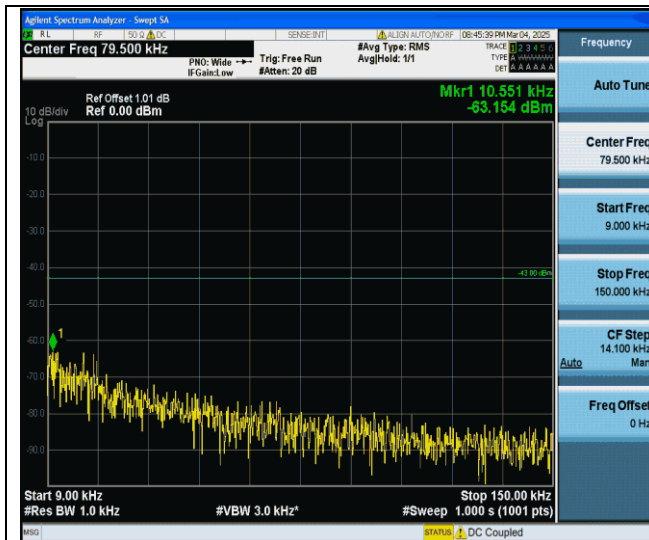
Band IV-1312-0.009~0.15MHz-PASS
