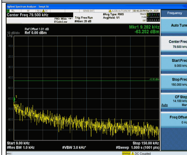
Band IV-1413-0.009~0.15MHz-PASS
