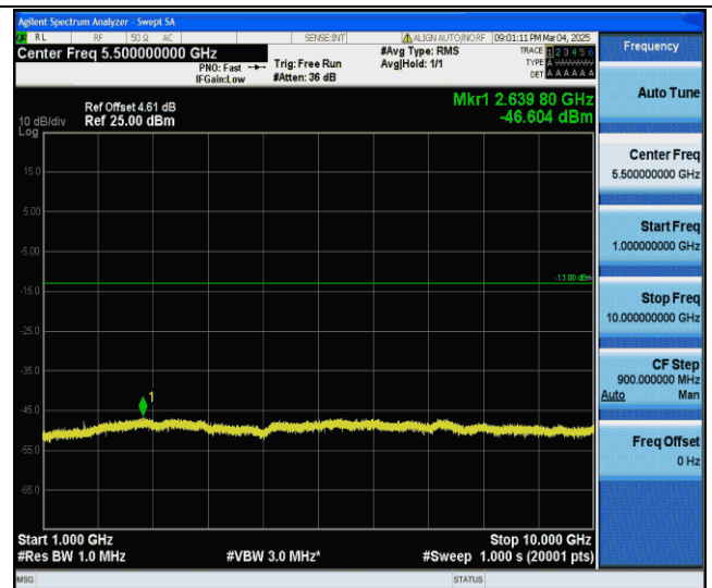
Band V-4182-1000~10000MHz-PASS
