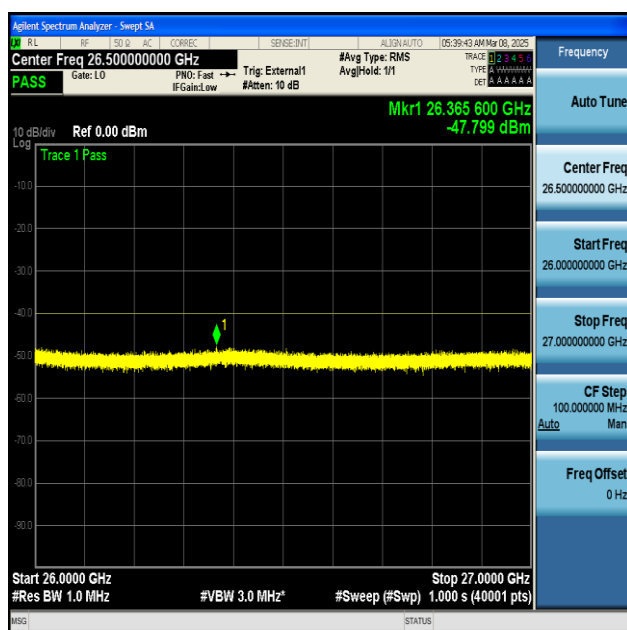
NTNV-n48-PC3-30-100-L-DFT-BPSK-Edge_1RB_Left- 26000-27000-PASS
