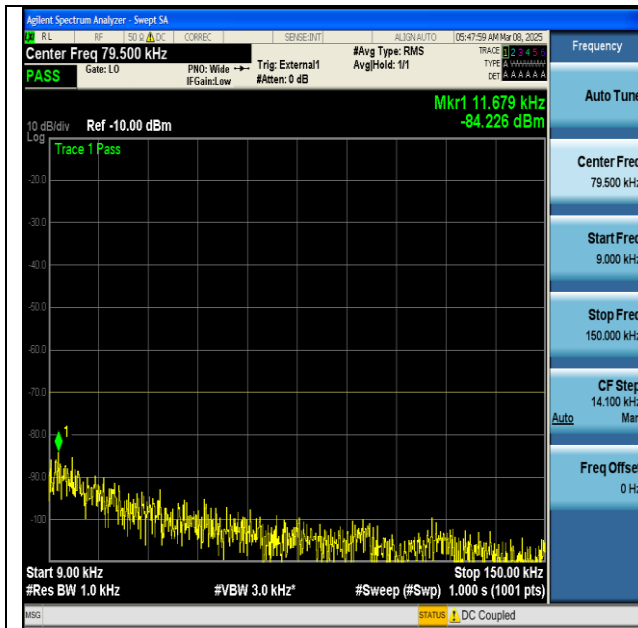
NTNV-n48-PC3-30-100-H-DFT-BPSK-Edge_1RB_Left- 0.009-0.15-PASS
