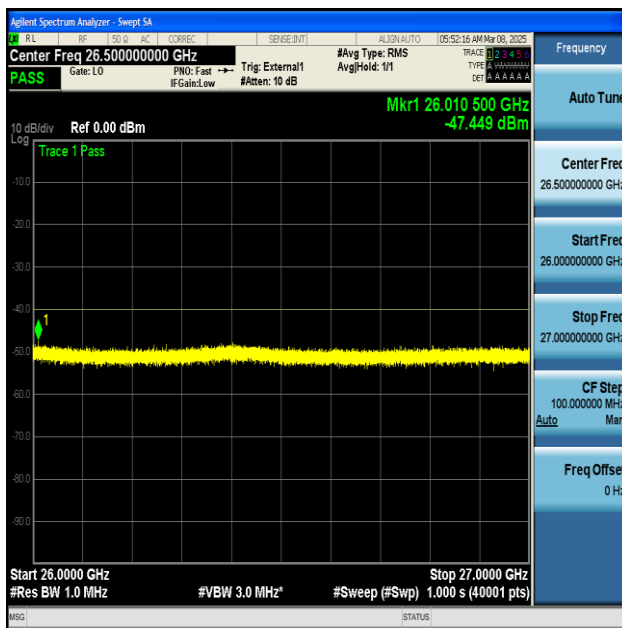
NTNV-n48-PC3-30-100-H-CP-QPSK-Edge_1RB_Left- 26000-27000-PASS
