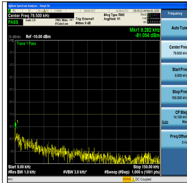
NTNV-n48-PC3-30-100-M-CP-QPSK-Edge_1RB_Left- 0.009-0.15-PASS
