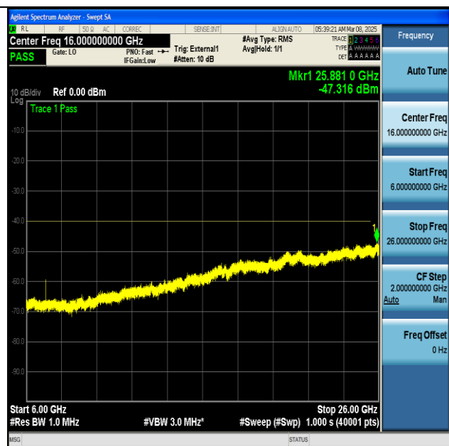
NTNV-n48-PC3-30-100-L-DFT-BPSK-Edge_1RB_Left- 6000-26000-PASS
