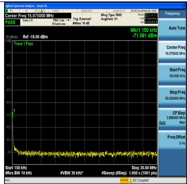
NTNV-n48-PC3-30-100-L-CP-QPSK-Edge_1RB_Left-0.15- 30-PASS
