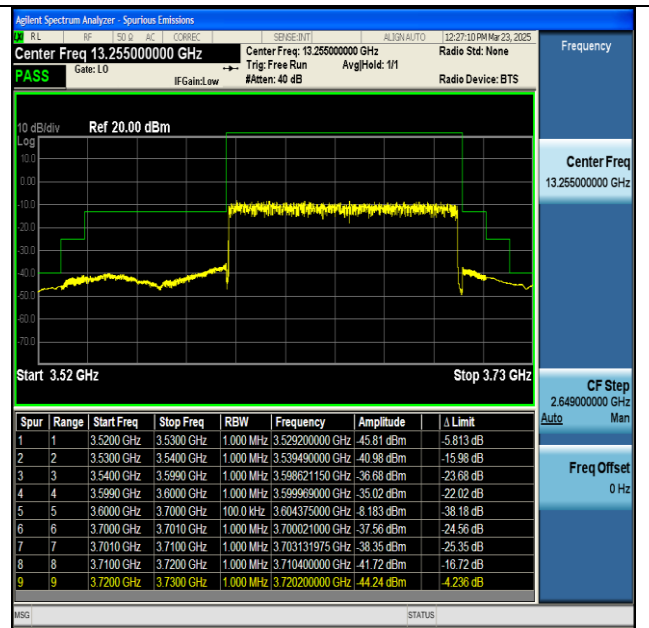
NTNV-n48-PC3-30-100-H-DFT-BPSK-Outer_Full-PASS
