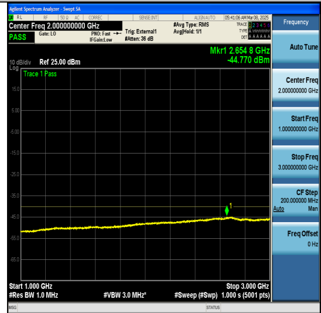
NTNV-n48-PC3-30-100-L-CP-QPSK-Edge_1RB_Left- 1000-3000-PASS
