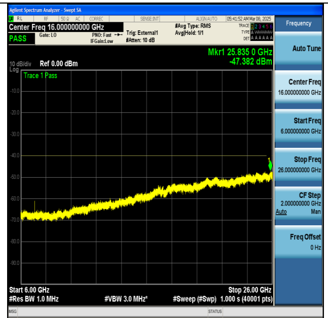
NTNV-n48-PC3-30-100-L-CP-QPSK-Edge_1RB_Left- 6000-26000-PASS
