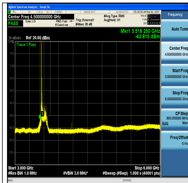
NTNV-n48-PC3-30-100-L-DFT-BPSK-Edge_1RB_Left- 3000-6000-PASS
