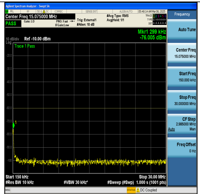
NTNV-n48-PC3-30-100-H-DFT-BPSK-Edge_1RB_Left- 0.15-30-PASS
