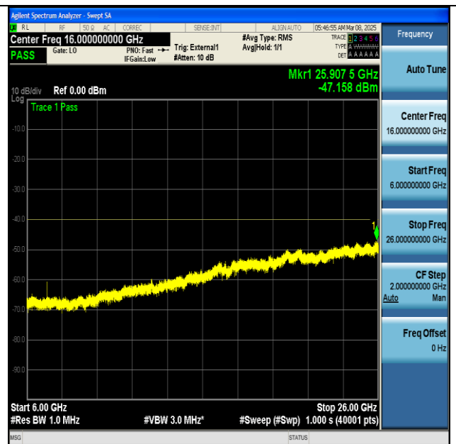
NTNV-n48-PC3-30-100-M-CP-QPSK-Edge_1RB_Left- 6000-26000-PASS
