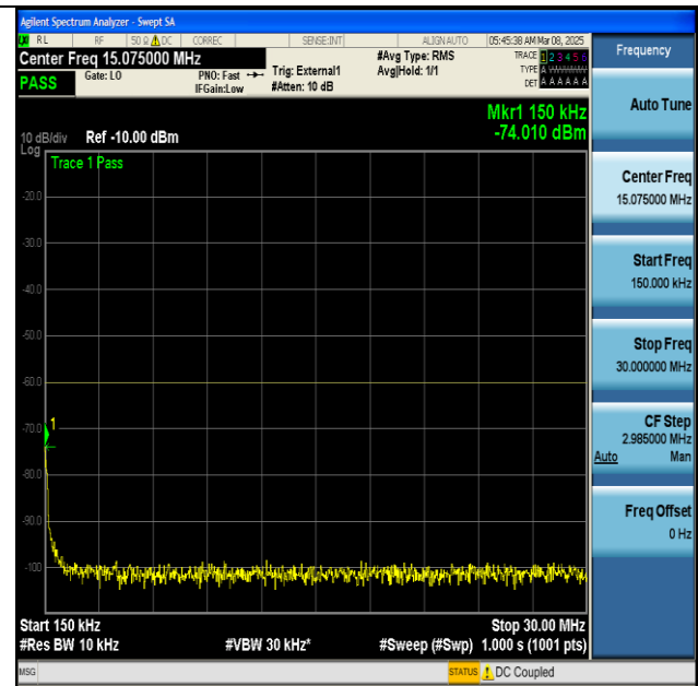
NTNV-n48-PC3-30-100-M-CP-QPSK-Edge_1RB_Left- 0.15-30-PASS
