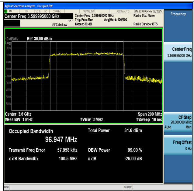
NTNV-n48-PC3-30-100-L-CP-16QAM-Outer_Full-Ant1- PASS
