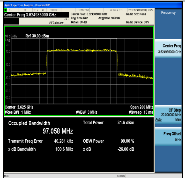
NTVN-n48-PC3-30-100-M-CP-64QAM-Outer_Full-Ant1- PASS
