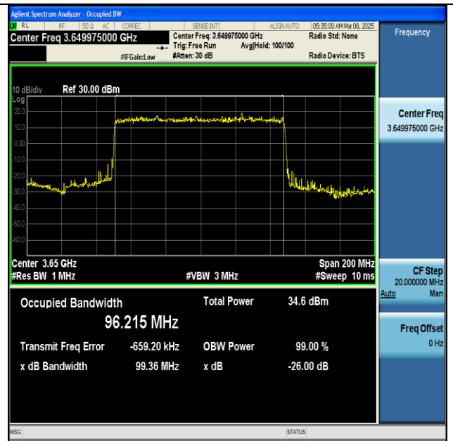
NTNV-n48-PC3-30-100-H-DFT-BPSK-Outer_Full-Ant1- PASS
