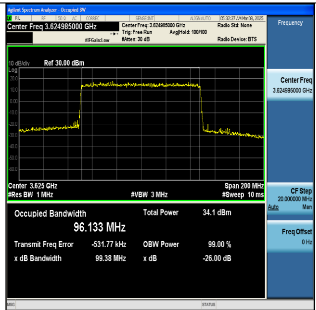
NTNV-n48-PC3-30-100-M-DFT-QPSK-Outer_Full-Ant1- PASS
