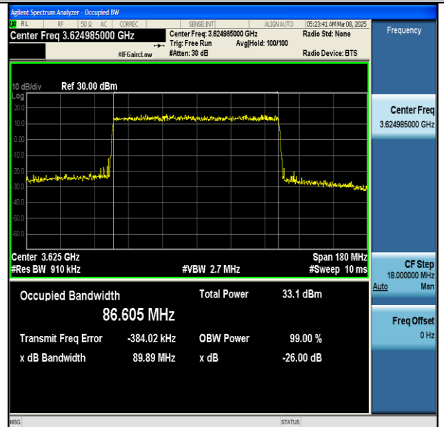
NTNV-n48-PC3-30-90-M-DFT-16QAM-Outer_Full-Ant1- PASS
