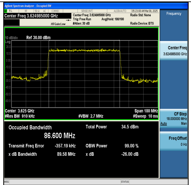
NTNV-n48-PC3-30-90-M-DFT-BPSK-Outer_Full-Ant1- PASS
