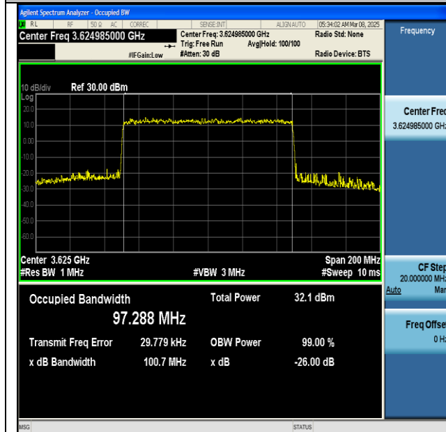
NTVN-n48-PC3-30-100-M-CP-16QAM-Outer_Full-Ant1- PASS
