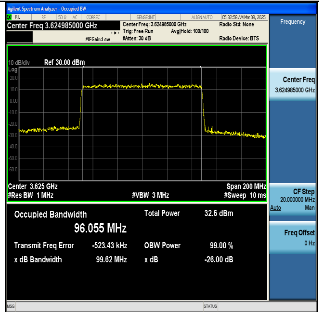
NTNV-n48-PC3-30-100-M-DFT-64QAM-Outer_Full-Ant1- PASS
