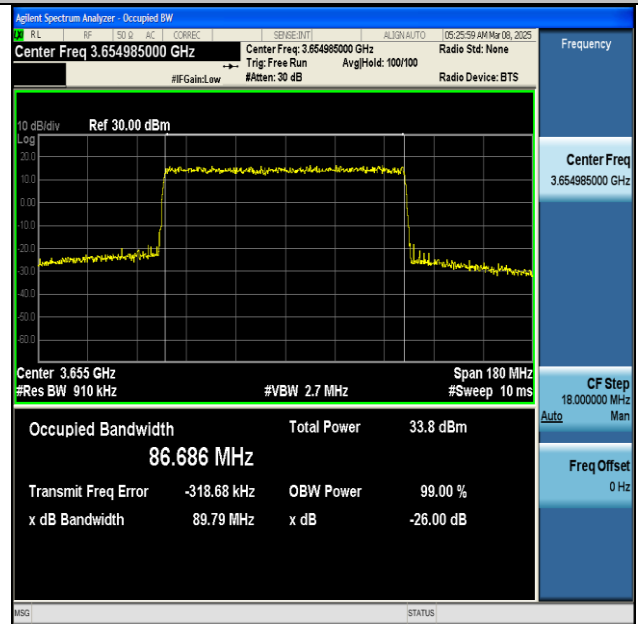
NTNV-n48-PC3-30-90-H-DFT-QPSK-Outer_Full-Ant1- PASS
