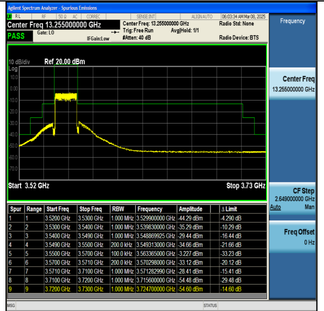
NTNV-n48-PC3-30-20-L-CP-QPSK-Outer_Full-PASS
