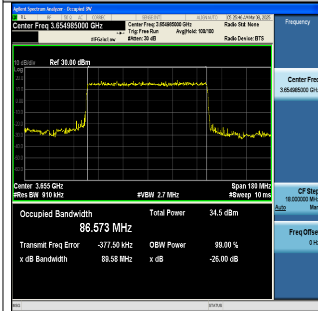
NTNV-n48-PC3-30-90-H-DFT-BPSK-Outer_Full-Ant1- PASS
