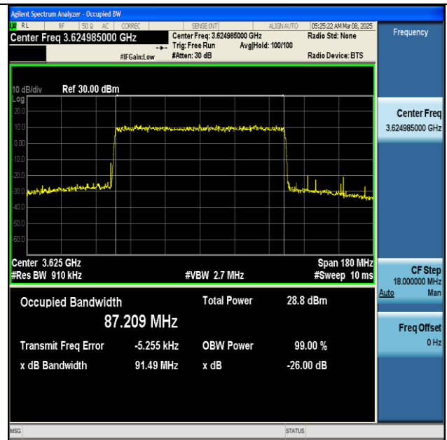
NTNV-n48-PC3-30-90-M-CP-256QAM-Outer_Full-Ant1- PASS
