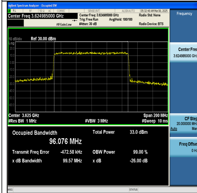
NTNV-n48-PC3-30-100-M-DFT-16QAM-Outer_Full-Ant1- PASS
