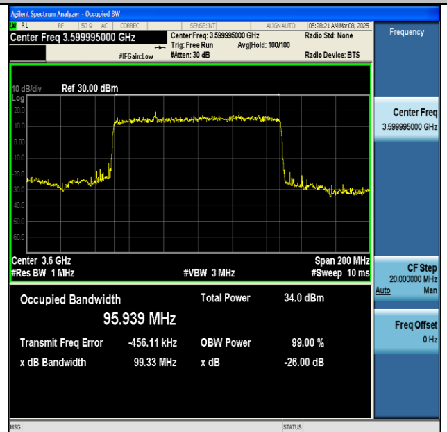
NTNV-n48-PC3-30-100-L-DFT-BPSK-Outer_Full-Ant1- PASS
