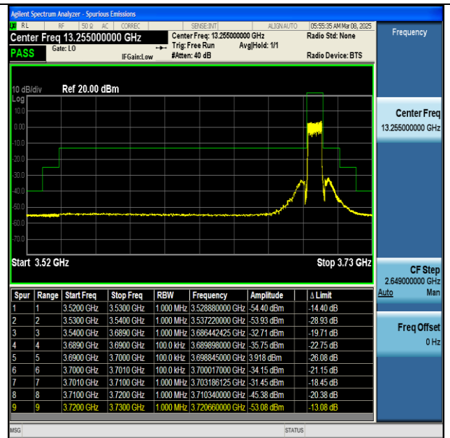
NTNV-n48-PC3-30-10-H-DFT-BPSK-Outer_Full-PASS
