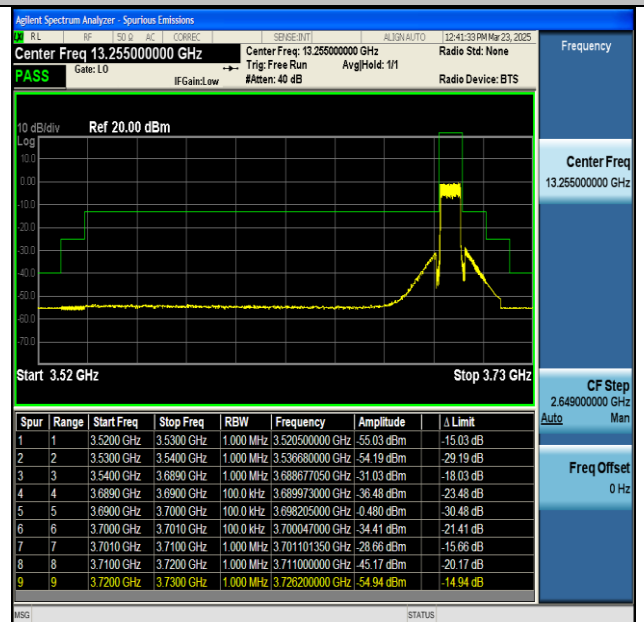
NTNV-n48-PC3-30-10-H-CP-QPSK-Outer_Full-PASS
