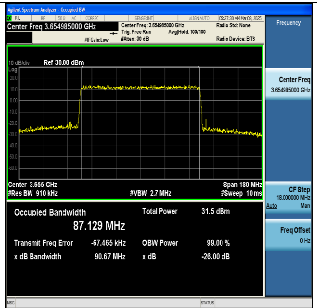
NTNV-n48-PC3-30-90-H-CP-64QAM-Outer_Full-Ant1- PASS
