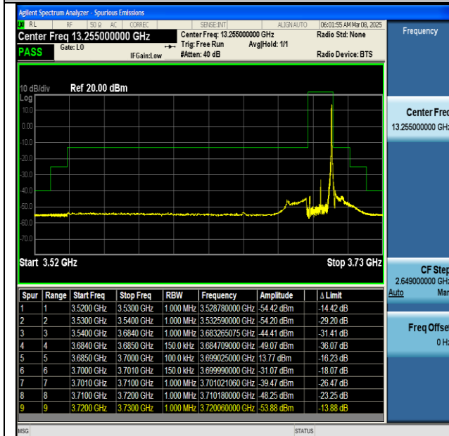
NTNV-n48-PC3-30-15-H-CP-QPSK-Edge_1RB_Right-PASS
