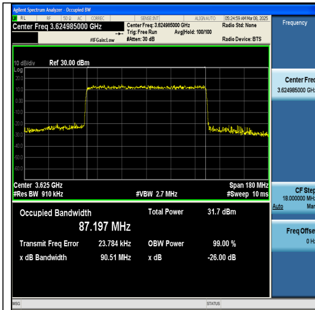
NTNV-n48-PC3-30-90-M-CP-64QAM-Outer_Full-Ant1- PASS
