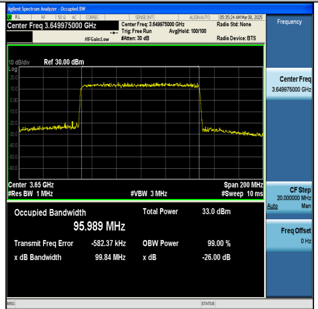
NTNV-n48-PC3-30-100-H-DFT-16QAM-Outer_Full-Ant1- PASS
