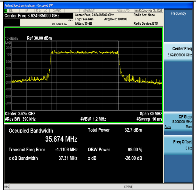
NTNV-n48-PC3-30-40-M-DFT-16QAM-Outer_Full-Ant1- PASS
