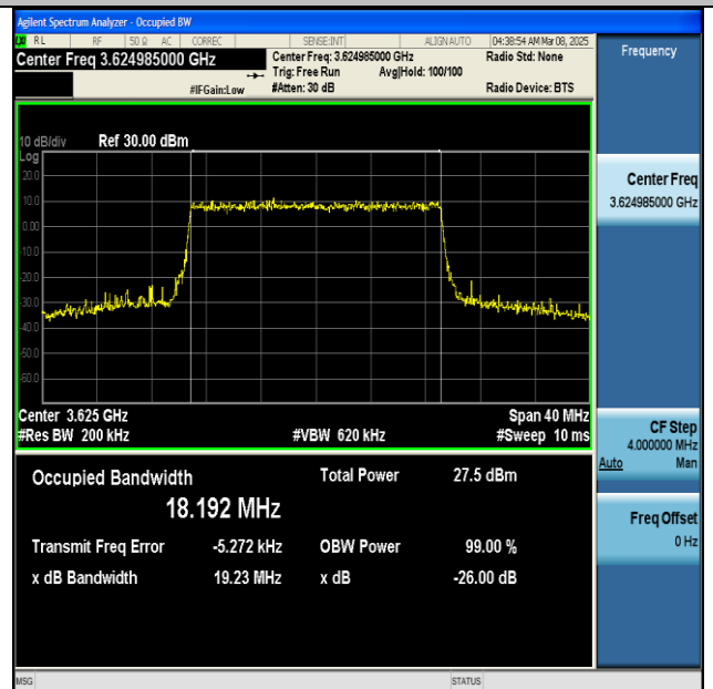
NTNV-n48-PC3-30-20-M-CP-256QAM-Outet_Full-Ant1-PASS
