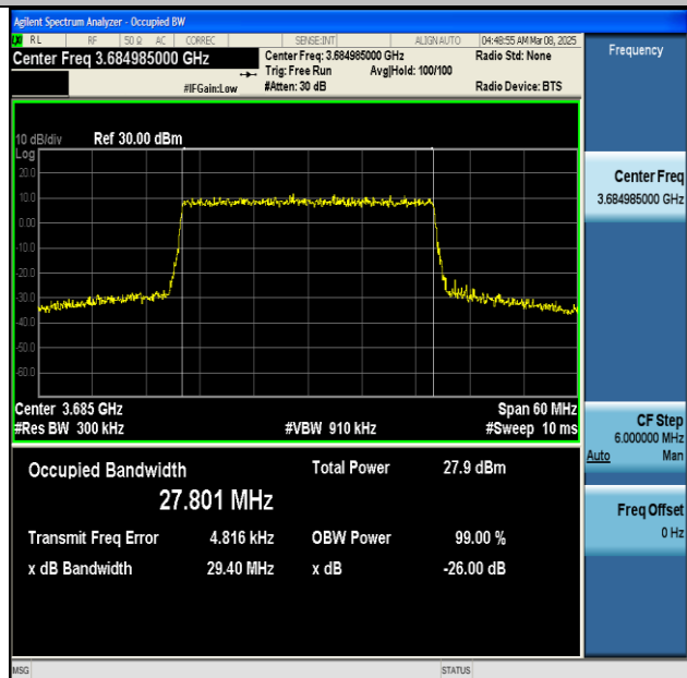
NTNV-n48-PC3-30-30-H-CP-256QAM-Outet_Full-Ant1-PASS
