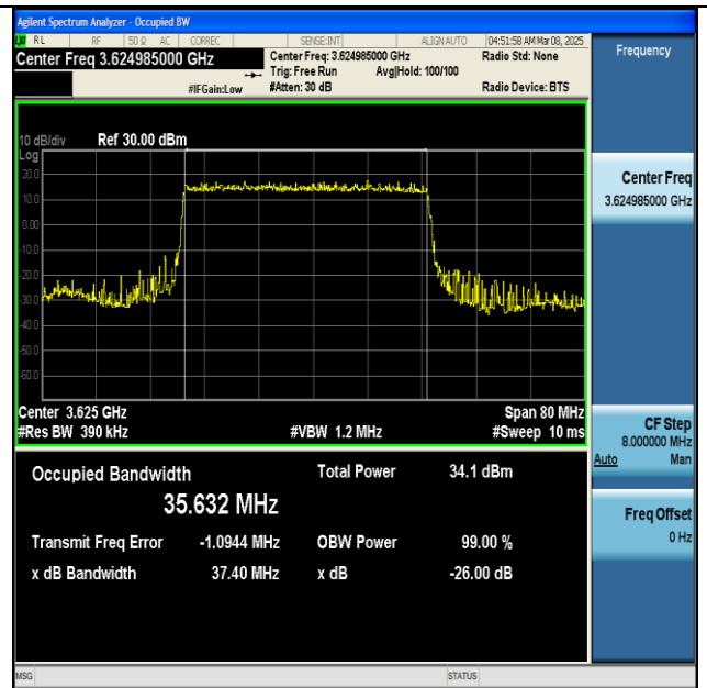
NTNV-n48-PC3-30-40-M-DFT-BPSK-Outer_Full-Ant1- PASS
