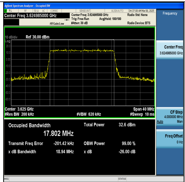
NTNV-n48-PC3-30-20-M-DFT-16QAM-Outer_Full-Ant1- PASS
