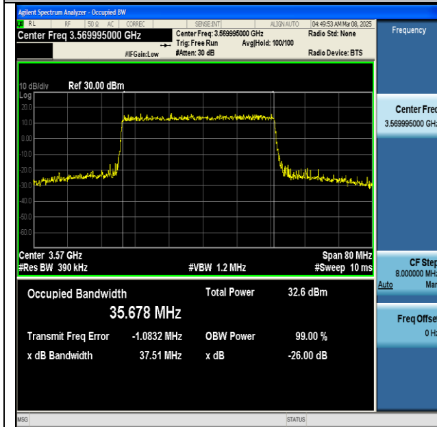
NTNV-n48-PC3-30-40-L-DFT-16QAM-Outer_Full-Ant1- PASS
