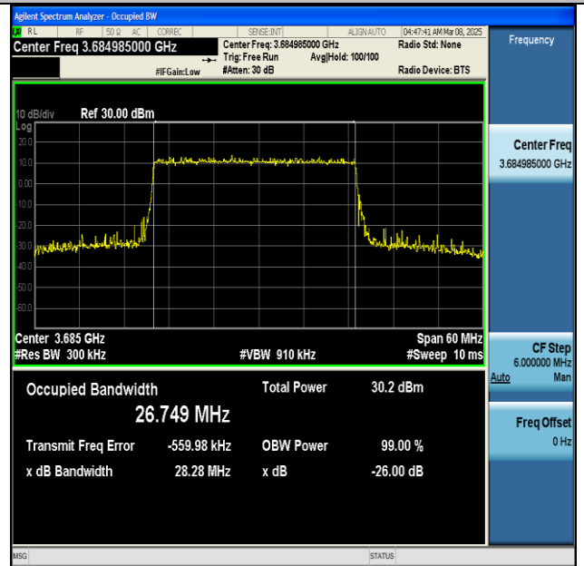
NTNV-n48-PC3-30-30-H-DFT-256QAM-Outer_Full-Ant1- PASS
