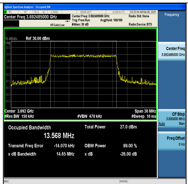
NTNV-n48-PC3-30-15-H-CP-256QAM-Outer_Full-Ant1- PASS
