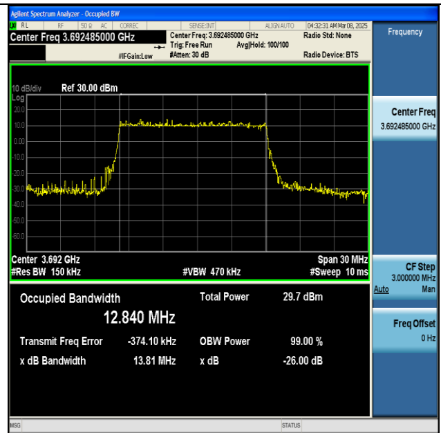
NTNV-n48-PC3-30-15-H-DFT-256QAM-Outer_Full-Ant1-1- PASS
