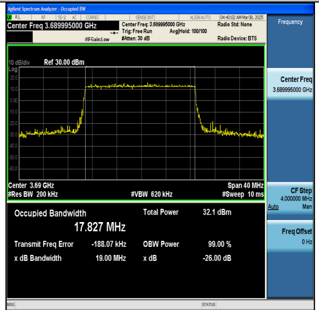
NTNV-n48-PC3-30-20-H-DFT-64QAM-Outer_Full-Ant1- PASS
