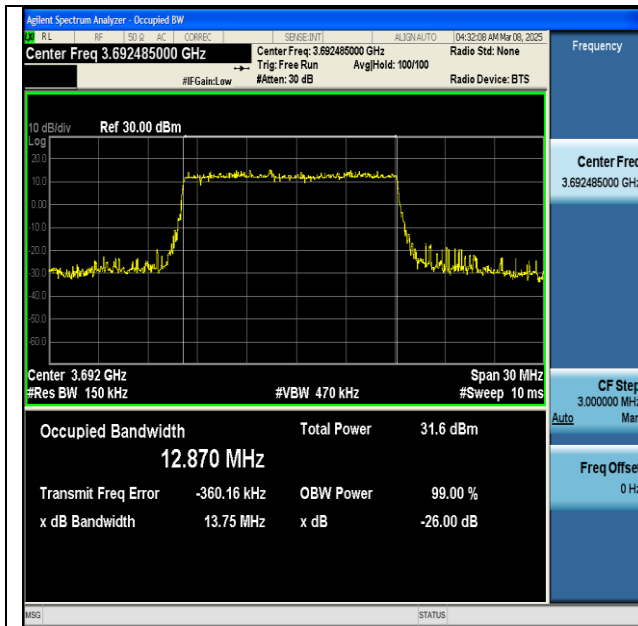
NTNV-n48-PC3-30-15-H-DFT-64QAM-Outer_Full-Ant1-1- PASS
