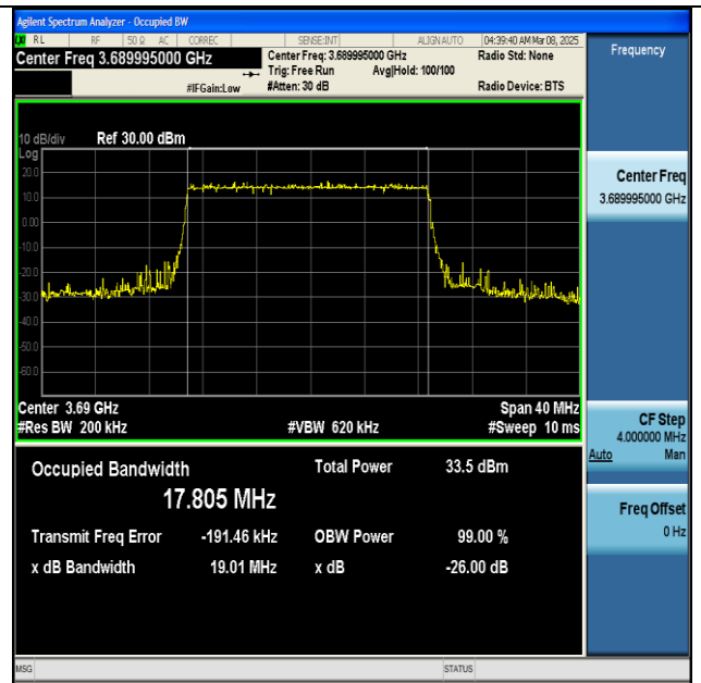
NTNV-n48-PC3-30-20-H-DFT-QPSK-Outer_Full-Ant1- PASS
