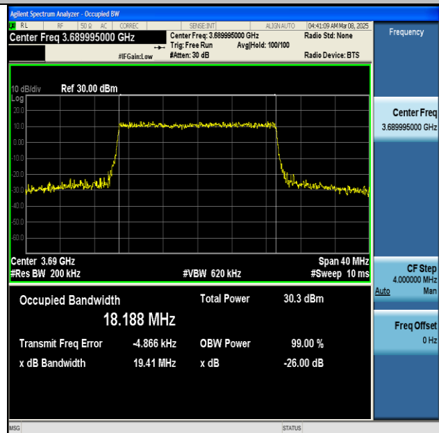
NTNV-n48-PC3-30-20-H-CP-64QAM-Outer_Full-Ant1-PASS
