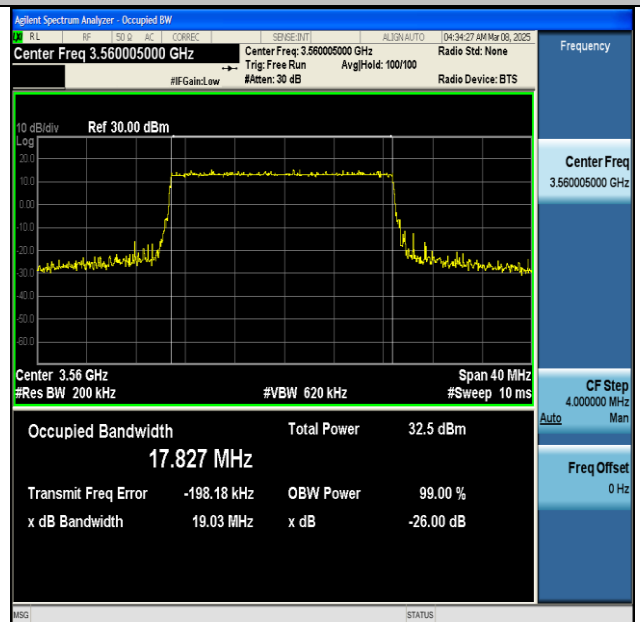
NTNV-n48-PC3-30-20-L-DFT-QPSK-Outer_Full-Ant1- PASS
