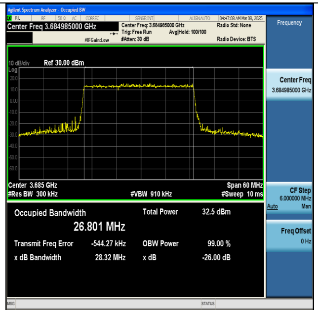
NTNV-n48-PC3-30-30-H-DFT-16QAM-Outer_Full-Ant1- PASS
