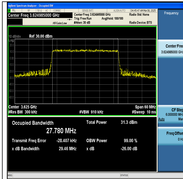
NTNV-n48-PC3-30-30-M-CP-16QAM-Outer_Full-Ant1- PASS
