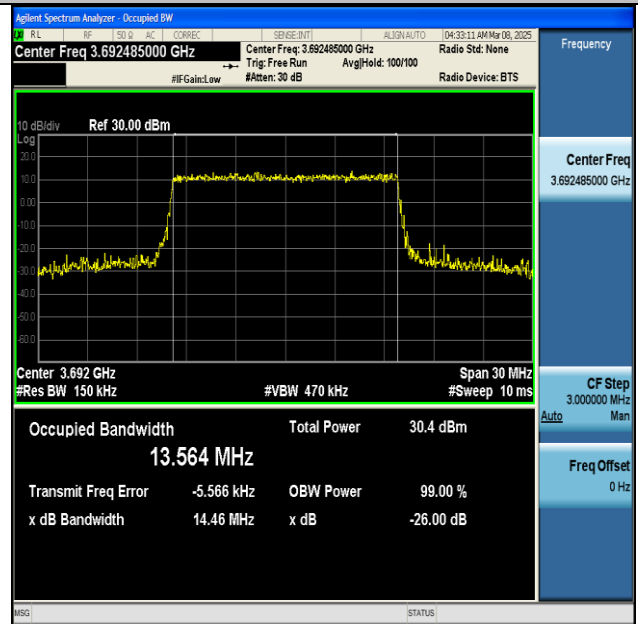
NTNV-n48-PC3-30-15-H-CP-16QAM-Outer_Full-Ant1-1- PASS
