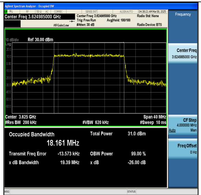
NTNV-n48-PC3-30-20-M-CP-16QAM-Outet_Full-Ant1-PASS
