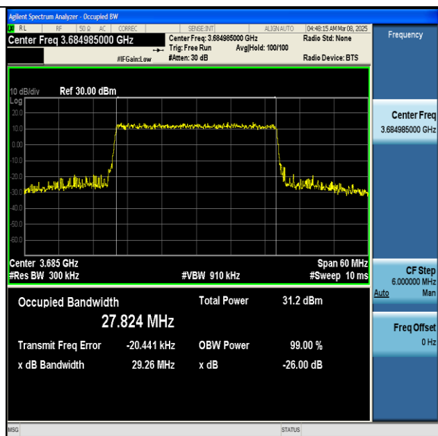
NTNV-n48-PC3-30-30-H-CP-16QAM-Outet_Full-Ant1-PASS
