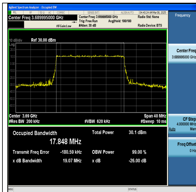
NTNV-n48-PC3-30-20-H-DFT-256QAM-Outer_Full-Ant1-PASS
