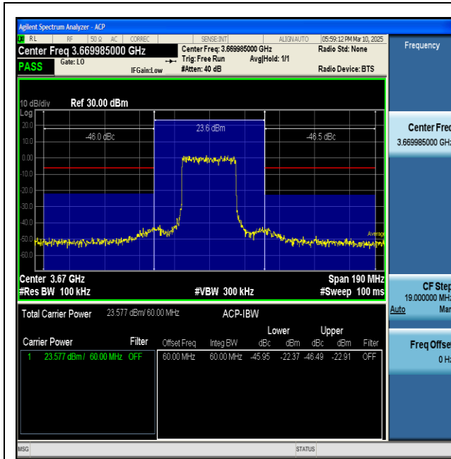
NTNV-n48-PC3-30-60-H-DFT-BPSK-Inner_Full-PASS
