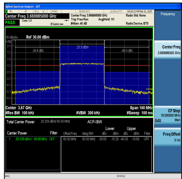
NTNV-n48-PC3-30-60-H-CP-QPSK-Outer_Full-PASS
