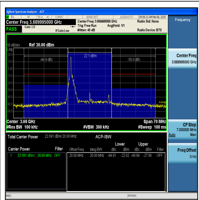
NTVN-n48-PC3-30-20-H-CP-QPSK-Inner_1RB_Left-PASS
