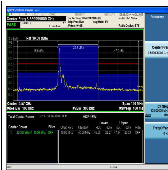
NTNV-n48-PC3-30-40-L-CP-QPSK-Inner_1RB_Left-PASS
