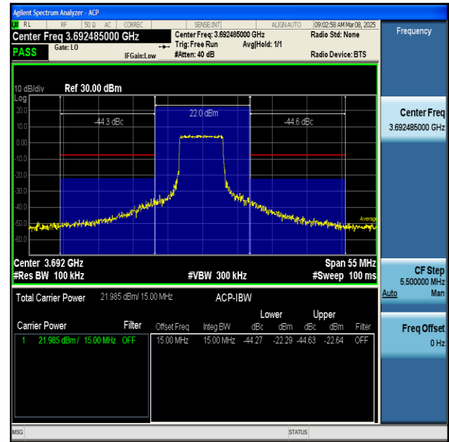
NTNV-n48-PC3-30-15-H-CP-QPSK-Inner_Full-PASS
