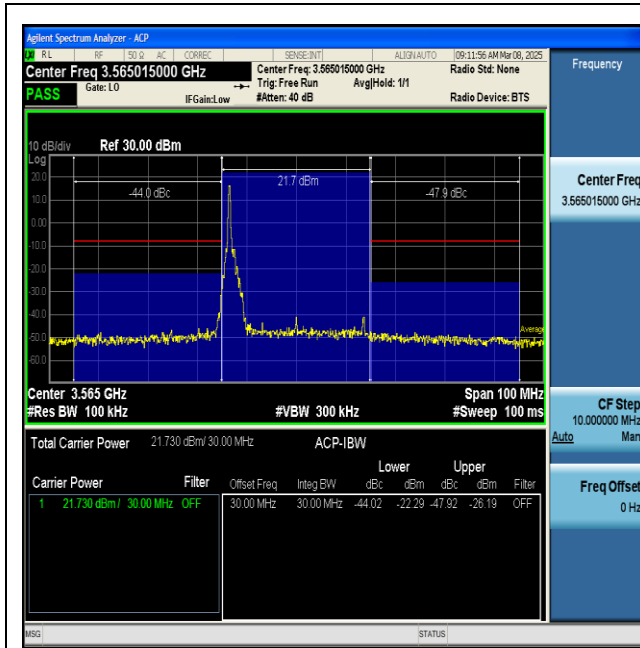
NTNV-n48-PC3-30-30-L-CP-QPSK-Inner_1RB_Left-PASS
