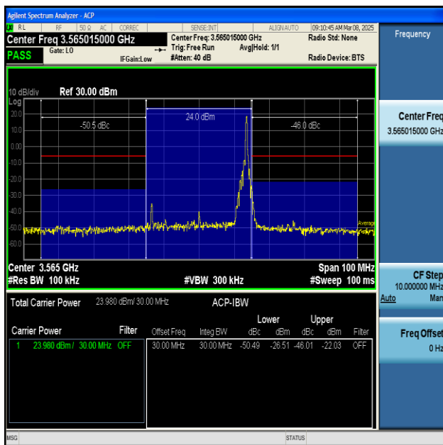
NTNV-n48-PC3-30-30-L-DFT-BPSK-Inner_1RB_Right PASS
