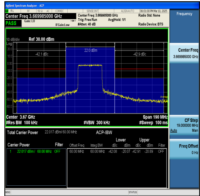
NTNV-n48-PC3-30-60-H-CP-QPSK-Inner_Full-PASS
