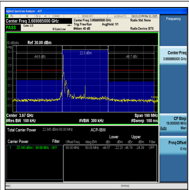
NTNV-n48-PC3-30-60-H-CP-QPSK-Inner_1RB_Left-PASS
