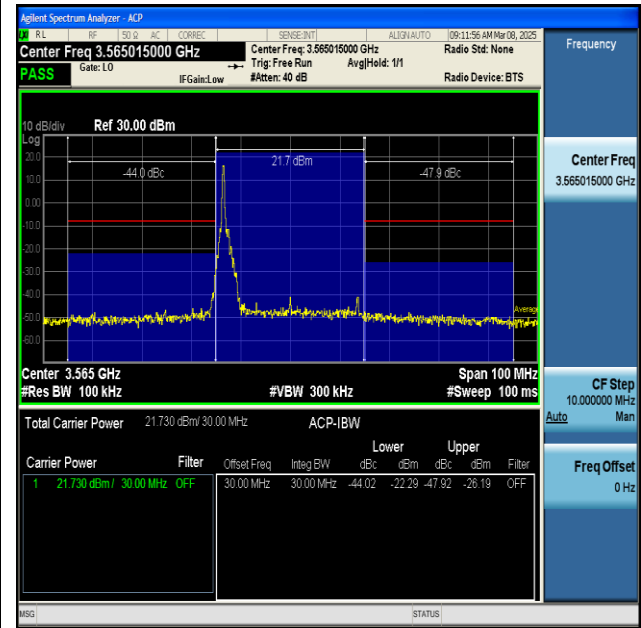
NTNV-n48-PC3-30-30-L-CP-QPSK-Inner_1RB_Left-PASS
