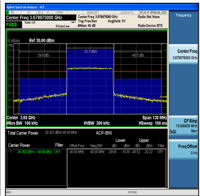
NTNV-n48-PC3-30-40-H-CP-QPSK-Outer_Full-PASS
