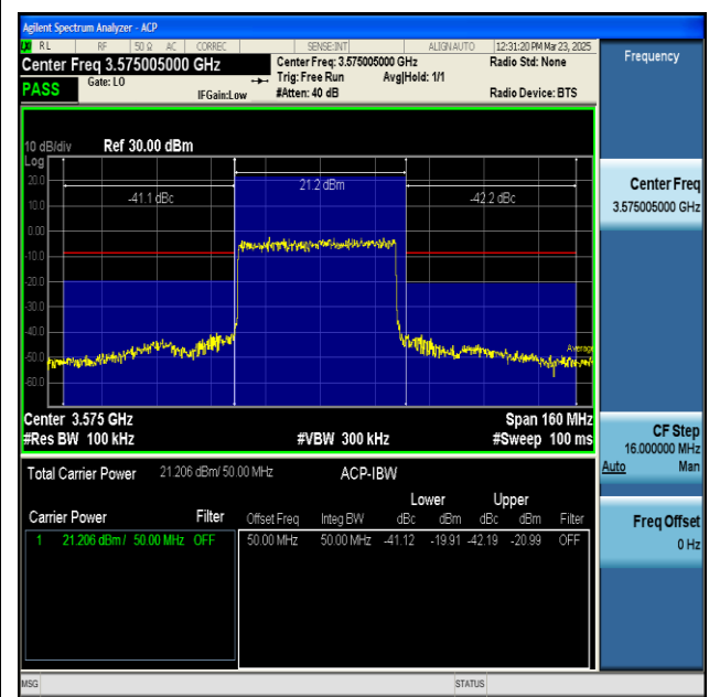
NTNV-n48-PC3-30-50-L-DFT-BPSK-Outer_Full-PASS
