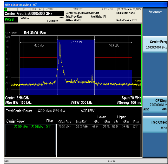
NTNV-n48-PC3-30-20-L-DFT-BPSK-Inner_1RB_Left- PASS
