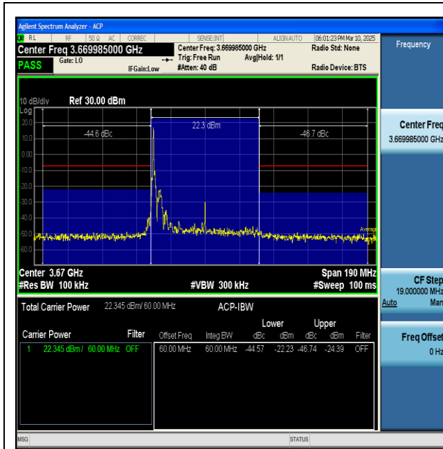
NTNV-n48-PC3-30-60-H-CP-QPSK-Inner_1RB_Left-PASS
