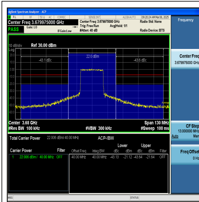
NTNV-n48-PC3-30-40-H-CP-QPSK-Inner_Full-PASS
