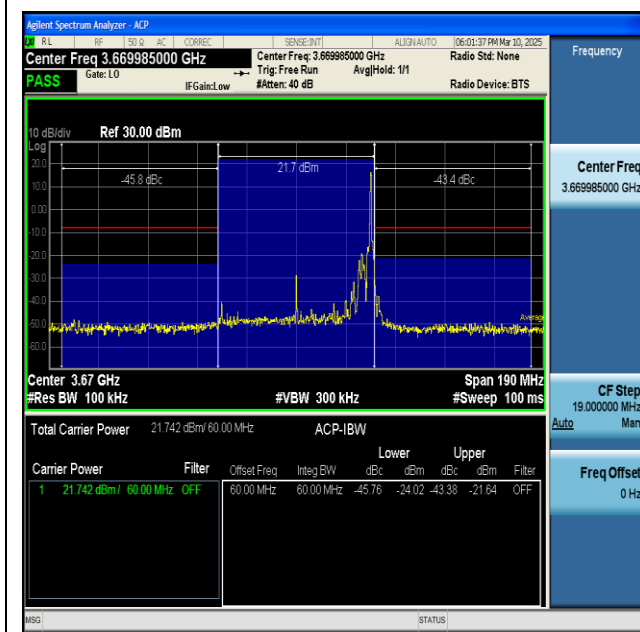
NTNV-n48-PC3-30-60-H-CP-QPSK-Inner_1RB_Right-PASS
