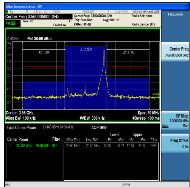
NTNV-n48-PC3-30-20-L-DFT-BPSK-Inner_1RB_Right- PASS
