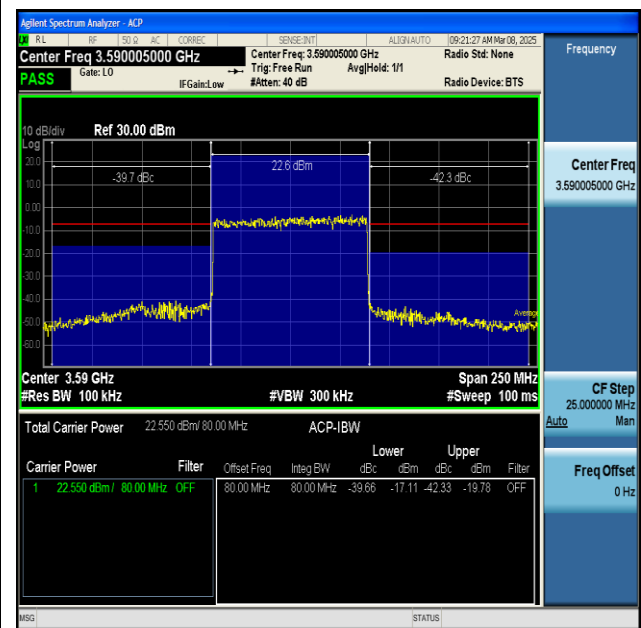
NTNV-n48-PC3-30-80-L-DFT-BPSK-Outer_Full-PASS
