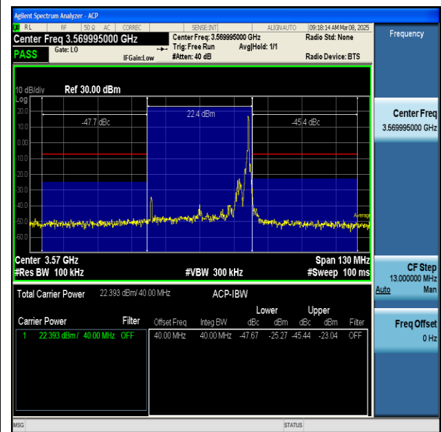
NTNV-n48-PC3-30-40-L-CP-QPSK-Inner_1RB_Right-PASS
