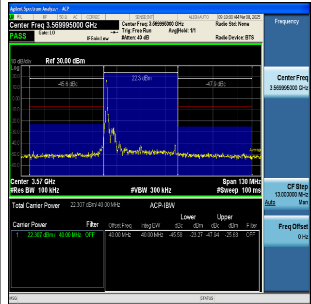
NTNV-n48-PC3-30-40-L-CP-QPSK-Inner_1RB_Left-PASS
