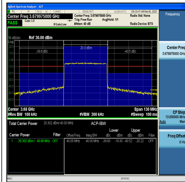
NTNV-n48-PC3-30-40-H-CP-QPSK-Outer_Full-PASS
