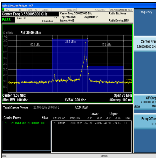
NTNV-n48-PC3-30-20-L-DFT-BPSK-Inner_1RB_Right- PASS
