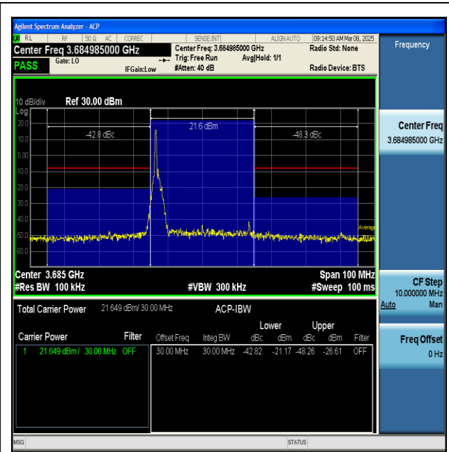
NTNV-n48-PC3-30-30-H-CP-QPSK-Inner_1RB_Left-PASS
