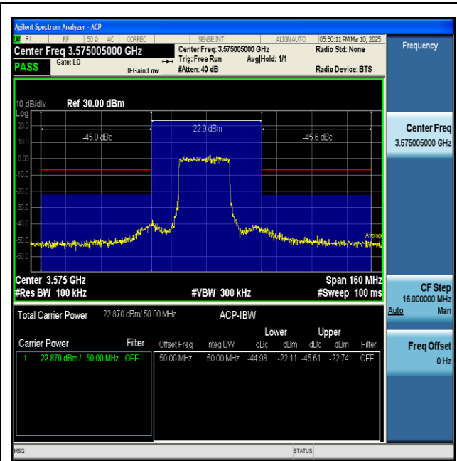
NTNV-n48-PC3-30-50-L-DFT-BPSK-Inner_Full-PASS
