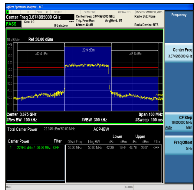
NTNV-n48-PC3-30-50-H-DFT-BPSK-Outer_Full-PASS
