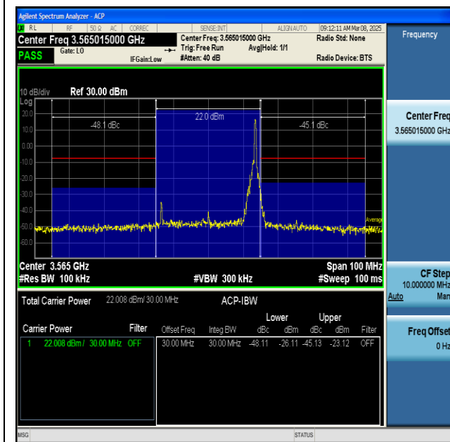
NTNV-n48-PC3-30-30-L-CP-QPSK-Inner_1RB_Right-PASS
