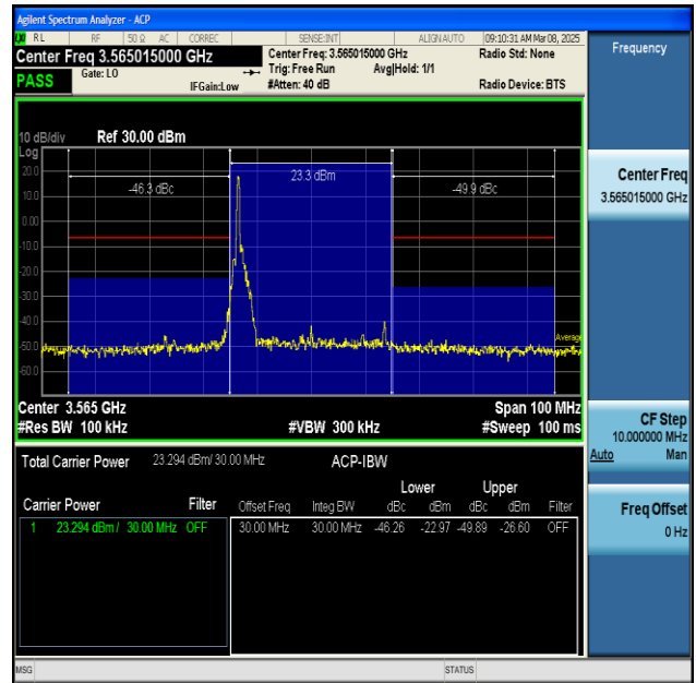
NTNV-n48-PC3-30-30-L-DFT-BPSK-Inner_1RB_Left PASS
