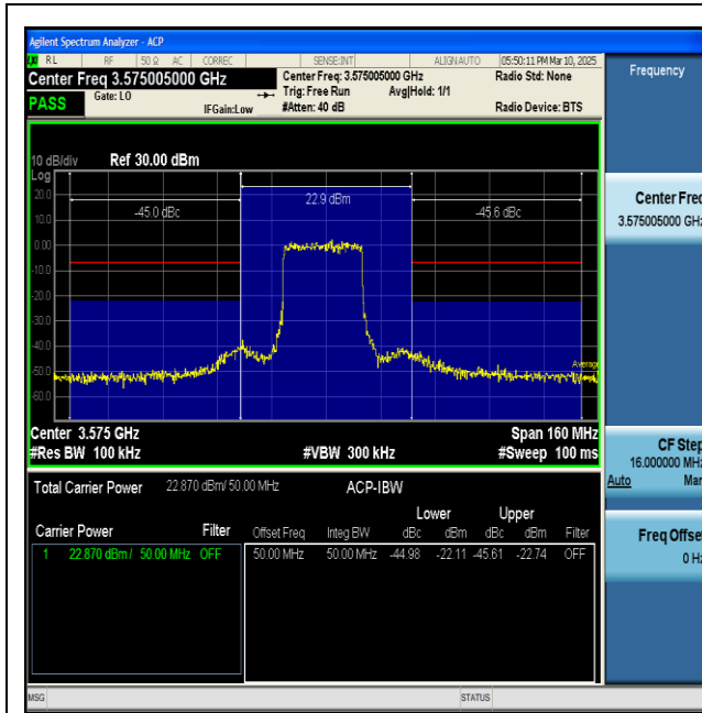
NTNV-n48-PC3-30-50-L-DFT-BPSK-Inner_Full-PASS
