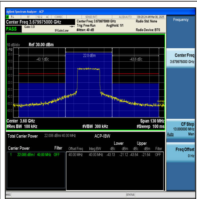
NTNV-n48-PC3-30-40-H-CP-QPSK-Inner_Full-PASS
