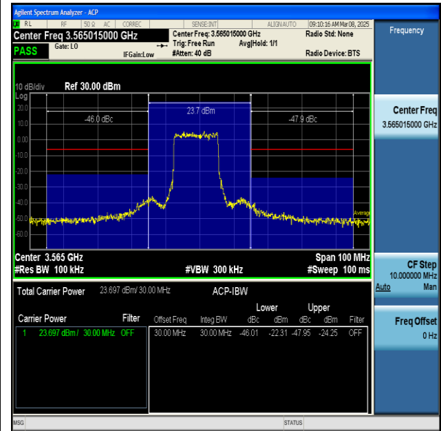
NTNV-n48-PC3-30-30-L-DFT-BPSK-Inner_Full-PASS
