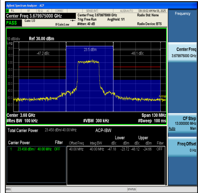
NTNV-n48-PC3-30-40-H-DFT-BPSK-Inner_Full-PASS
