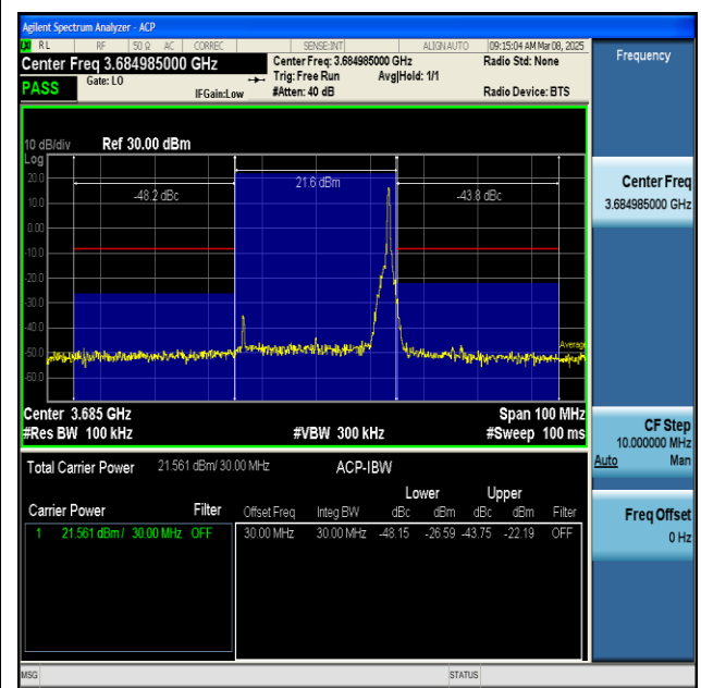
NTNV-n48-PC3-30-30-H-CP-QPSK-Inner_1RB_Right-PASS
