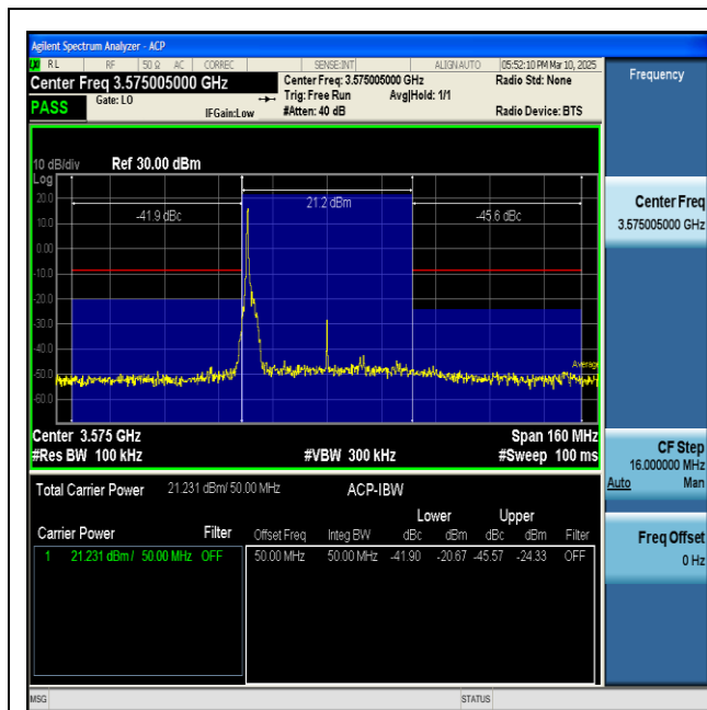
NTNV-n48-PC3-30-50-L-CP-QPSK-Inner 1RB Left-PASS
