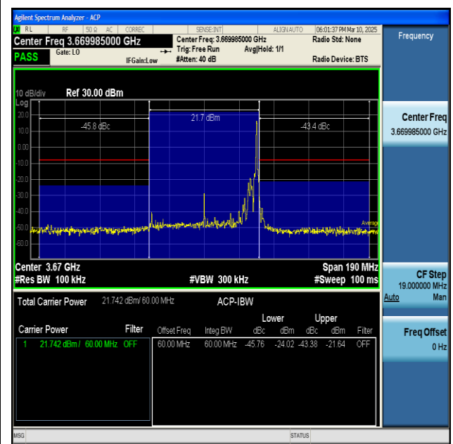
NTNV-n48-PC3-30-60-H-CP-QPSK-Inner_1RB_Right-PASS
