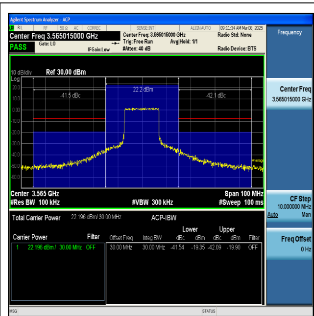
NTNV-n48-PC3-30-30-L-CP-QPSK-Inner Full-PASS
