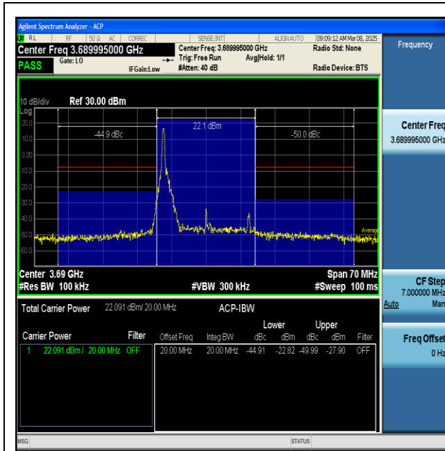
NTVN-n48-PC3-30-20-H-CP-QPSK-Inner_1RB_Left-PASS
