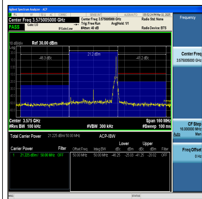
NTNV-n48-PC3-30-50-L-CP-QPSK-Inner_1RB_Right- PASS
