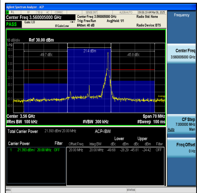
NTVN-n48-PC3-30-20-L-CP-QPSK-Inner_1RB_Right-PASS
