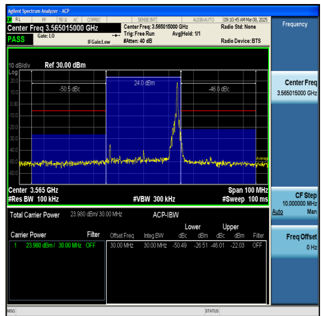
NTNV-n48-PC3-30-30-L-DFT-BPSK-Inner_1RB_Right PASS
