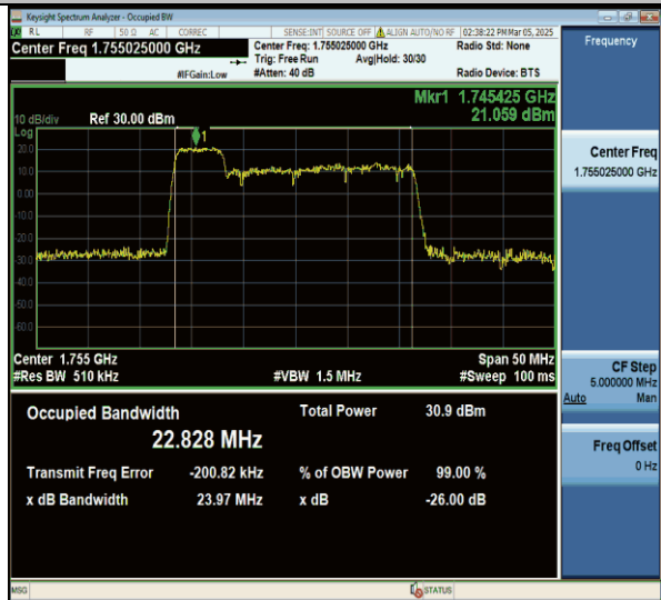
66-66-5MHz-20MHz-64QAM-64QAM-132330-132447- 25RB#0-100RB#0-PASS
