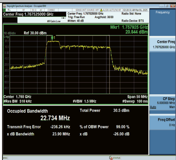
66-66-5MHz-20MHz-16QAM-16QAM-132455-132572- 25RB#0-100RB#0-PASS
