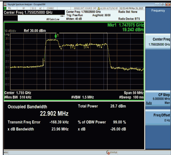
66-66-5MHz-20MHz-256QAM-256QAM-132330-132447- 25RB#0-100RB#0-PASS
