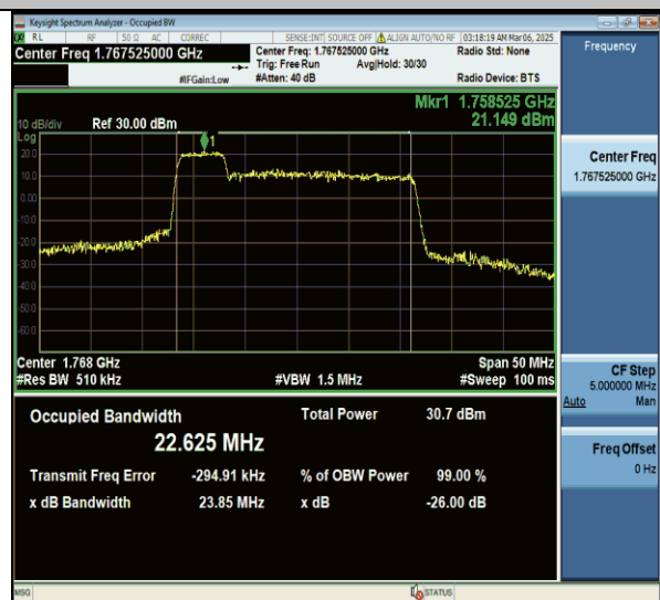
66-66-5MHz-20MHz-64QAM-64QAM-132455-132572- 25RB#0-100RB#0-PASS
