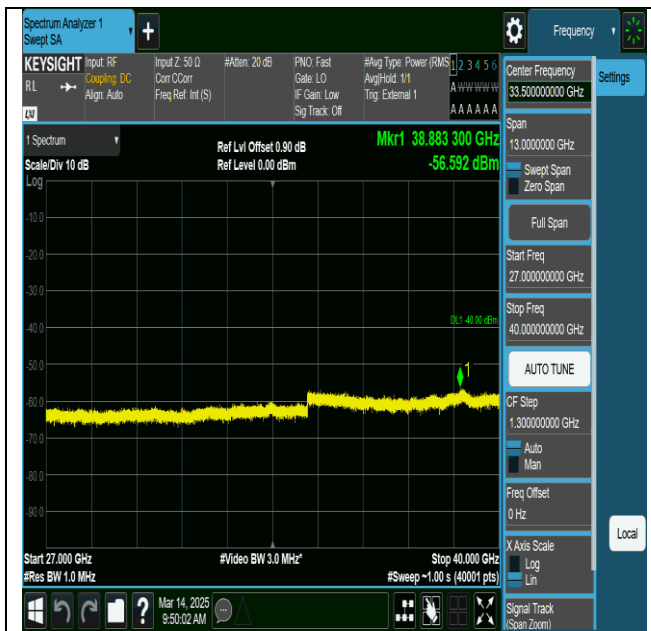
48-48-20MHz-20MHz-QPSK-QPSK-55340-55538-1RB#0- ORB#0-27000~40000MHz-PASS
