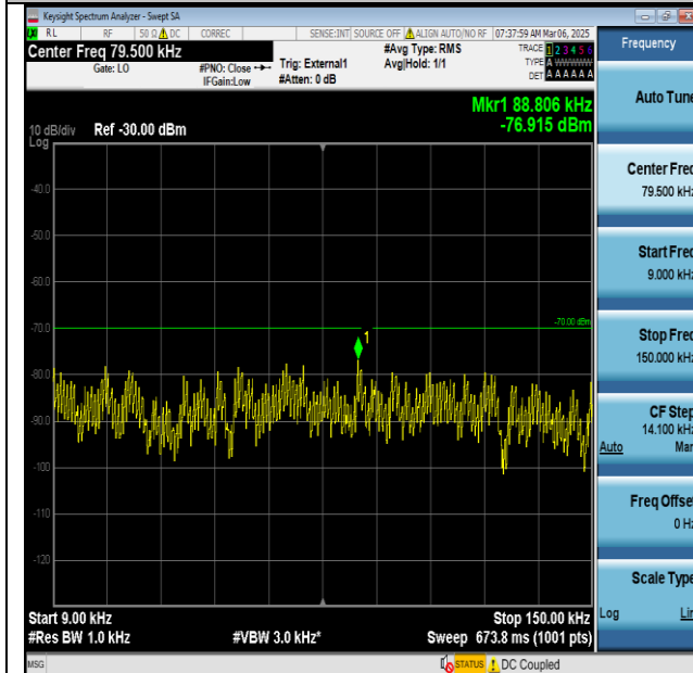
48-48-20MHz-20MHz-QPSK-QPSK-56442-56640-1RB#0- ORB#0-0.009~0.15MHz-PASS
