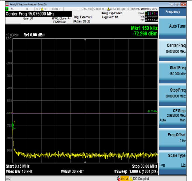
48-48-20MHz-20MHz-QPSK-QPSK-56442-56640-1RB#0- ORB#0-0.15~30MHz-PASS
