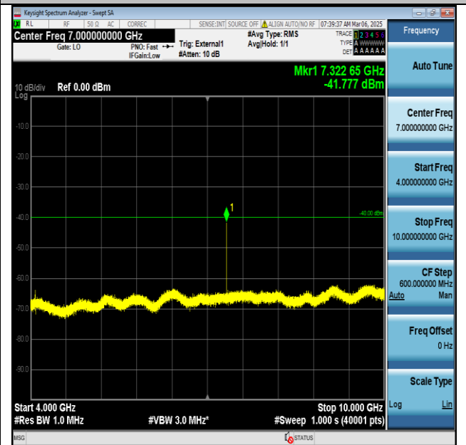
48-48-20MHz-20MHz-QPSK-QPSK-56442-56640-1RB#0-ORB#0-4000~10000MHz-PASS
