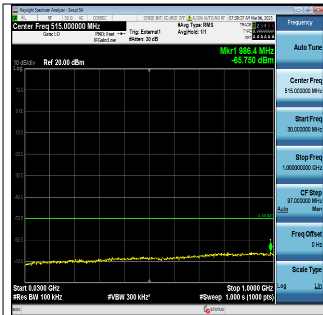
48-48-20MHz-20MHz-QPSK-QPSK-56442-56640-1RB#0-ORB#0-30~1000MHz-PASS
