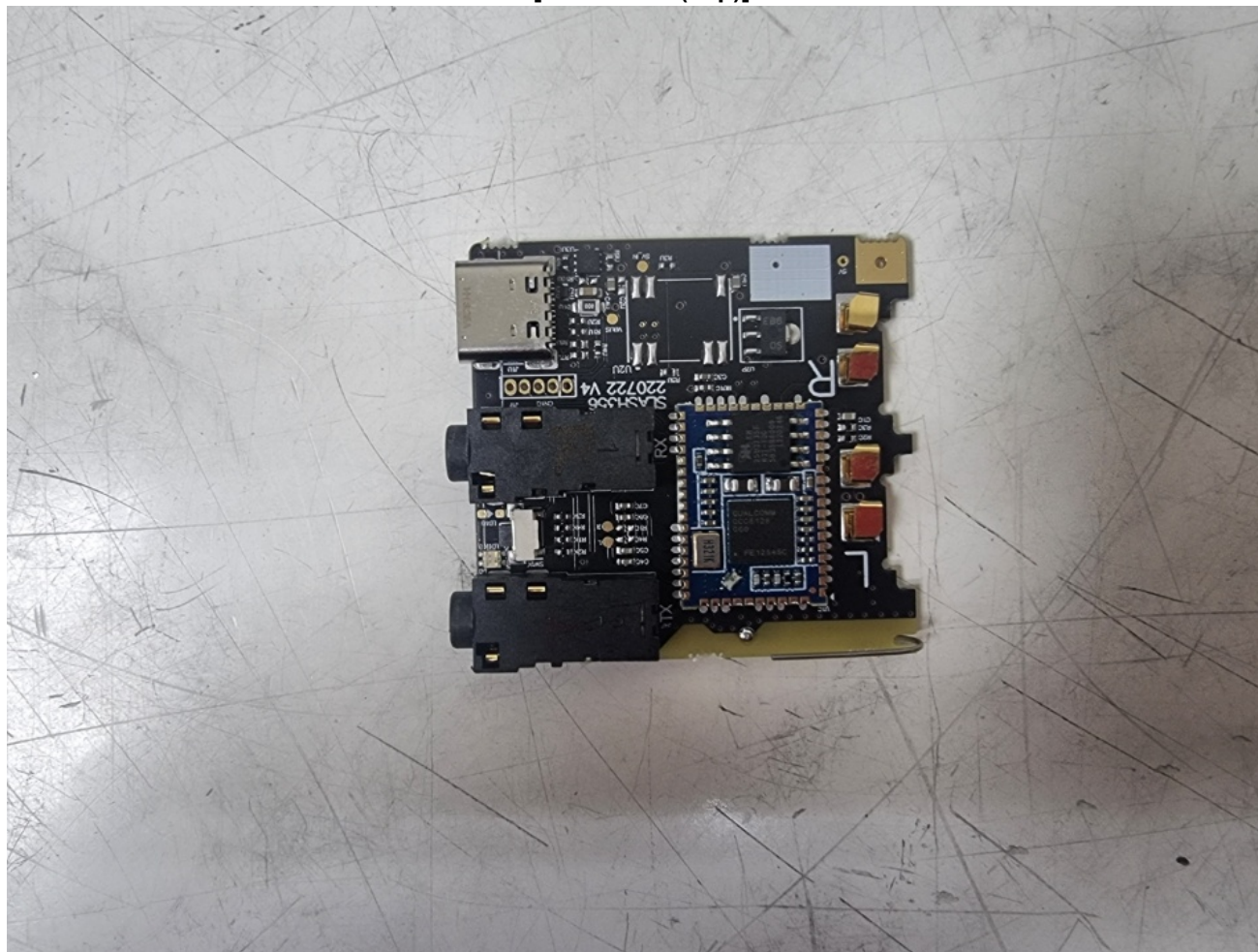
[Main board(Top)]
