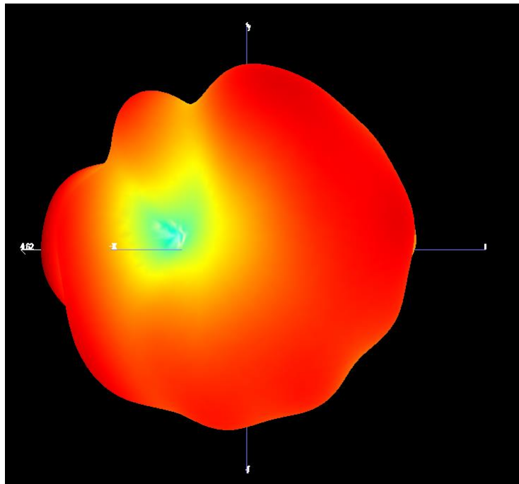
B1.2 3D Pattern for 2450MHz
