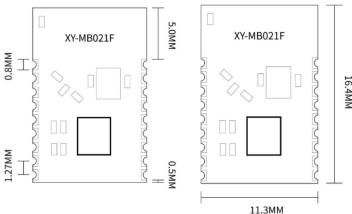
Figure 2-Module dimension Diagram
