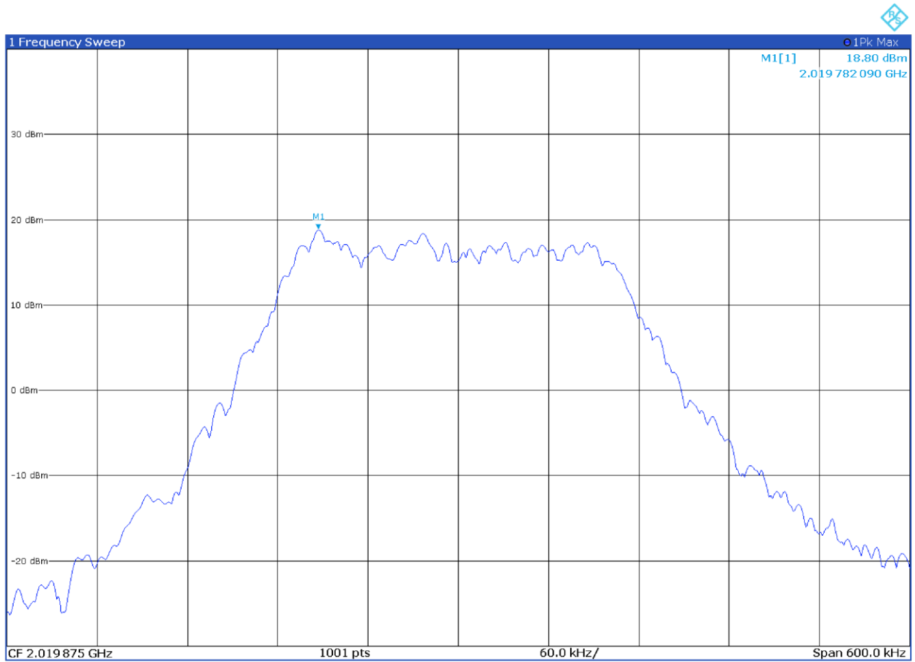
Figure 8.4-6: Output power on high channel - LoRa 250 kHz BW
